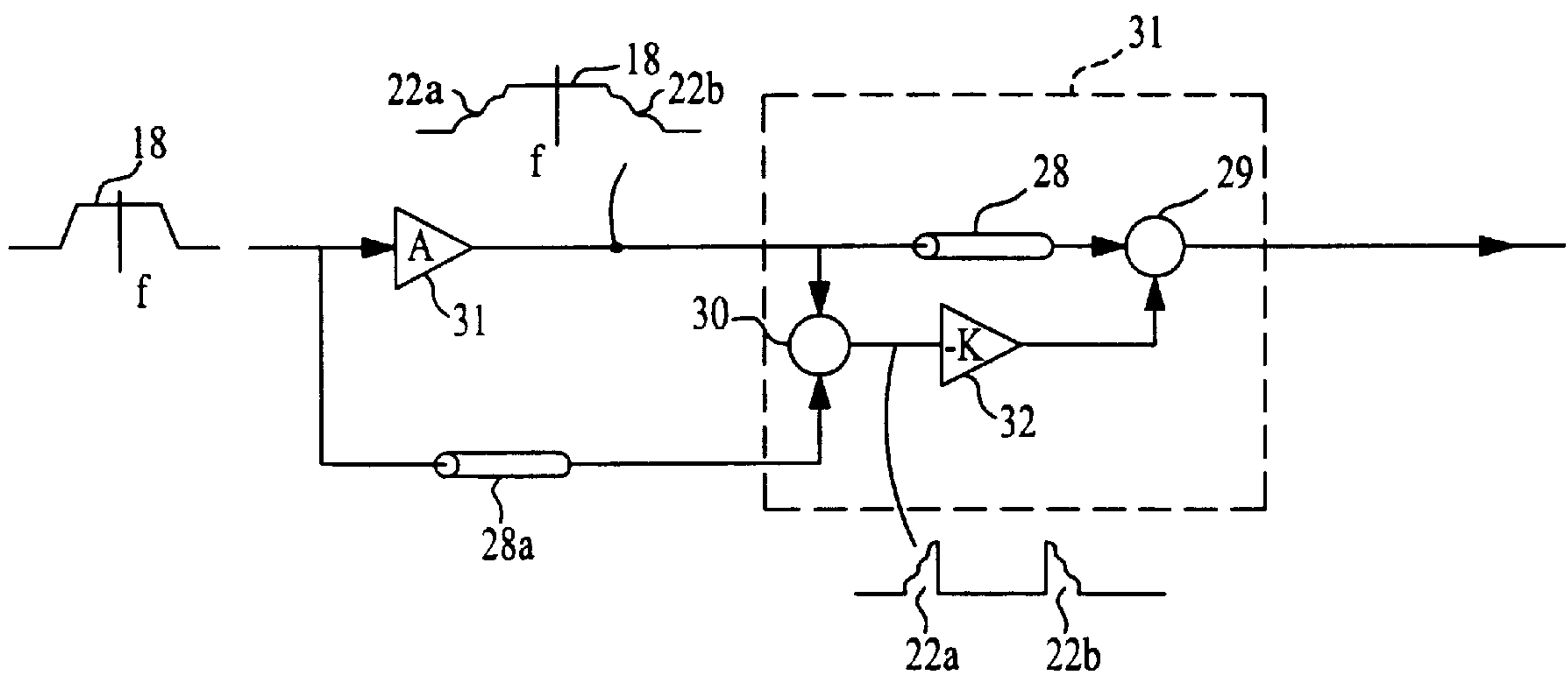
FIG. 4 (PRIOR ART)
