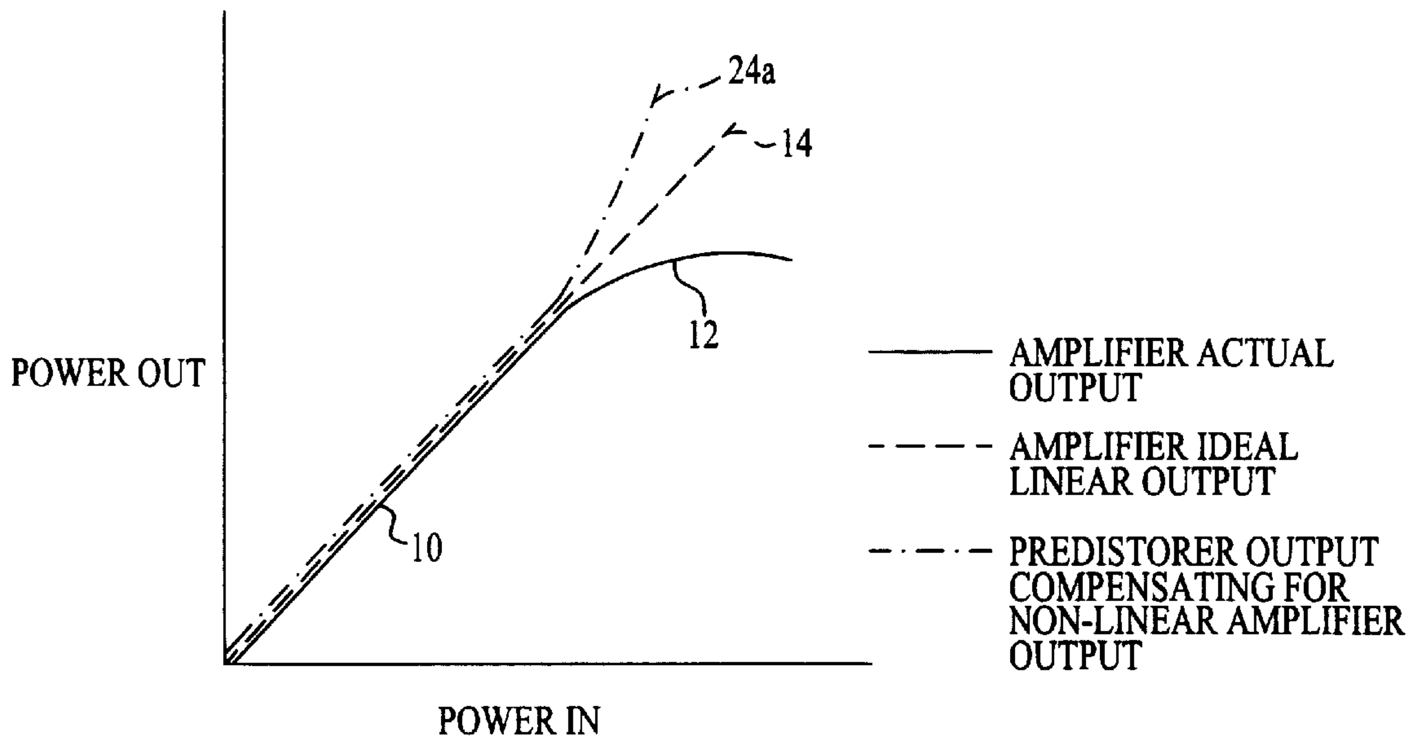
FIG. 1 (PRIOR ART)
