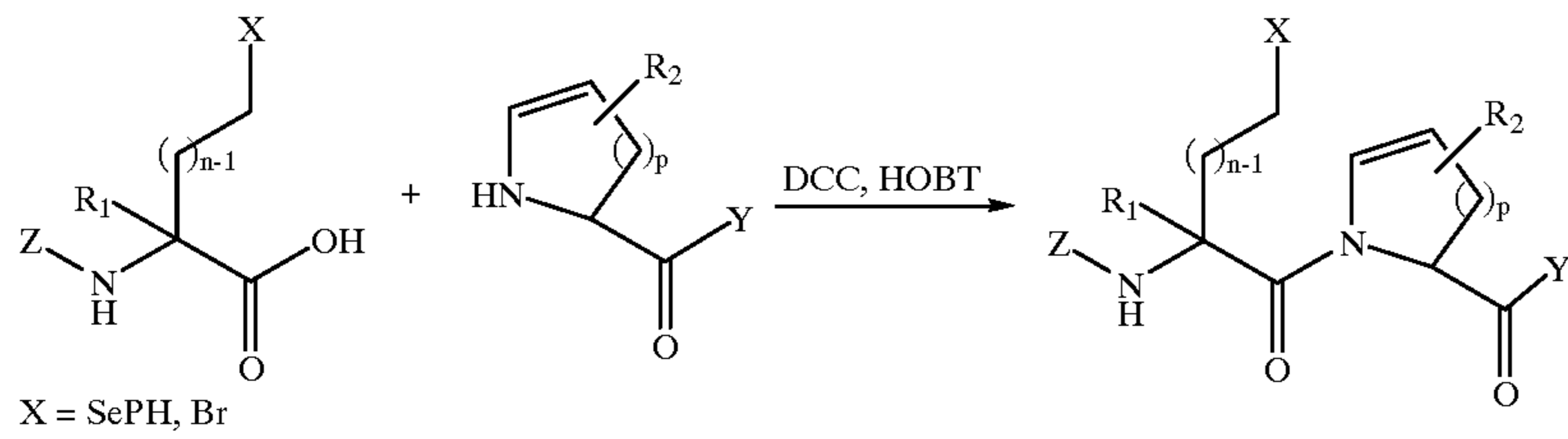
Reaction Scheme (1)
