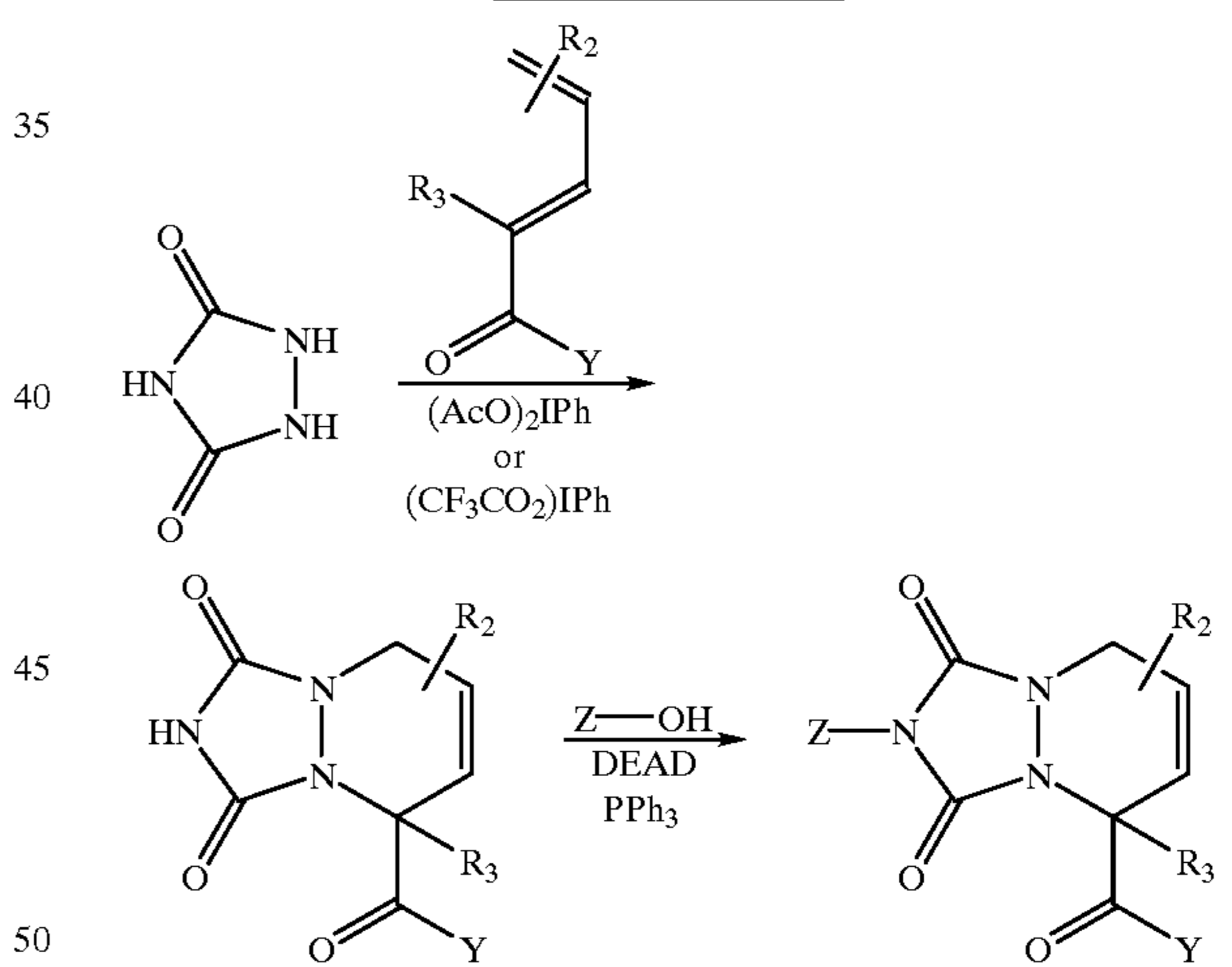
Reaction Scheme (28)
