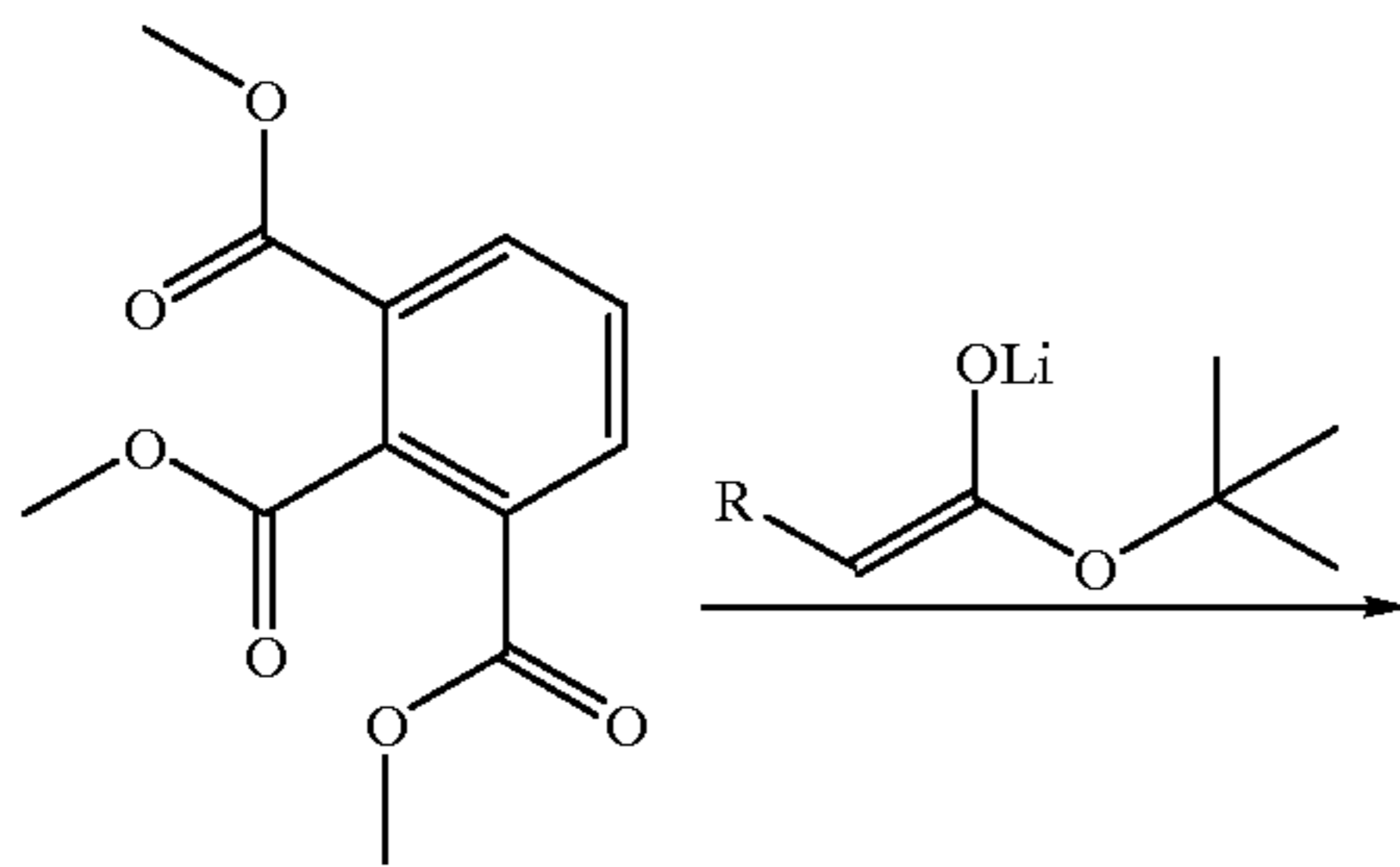
Reaction Scheme (18)
