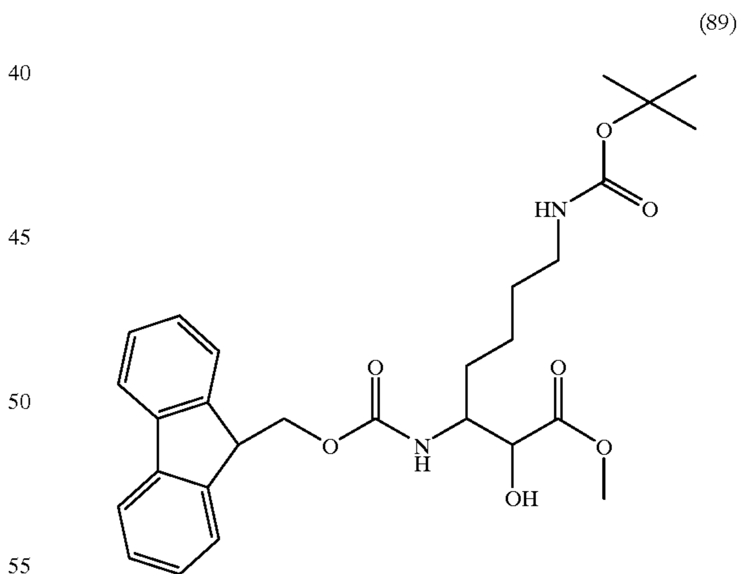
Synthesis of Structure (89)
