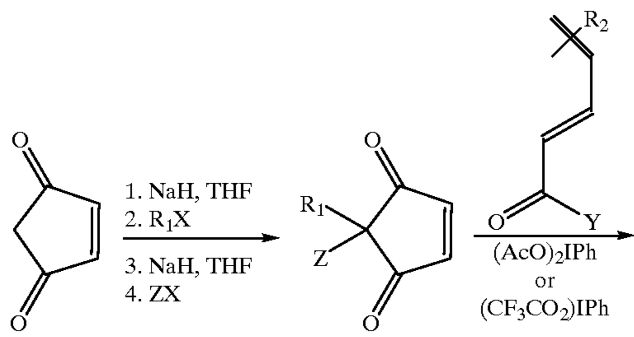
Reaction Scheme (19-1)
