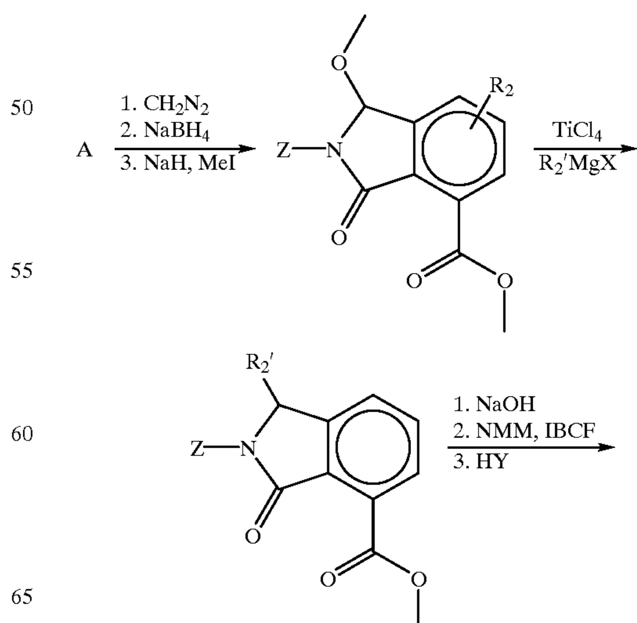
Reaction Scheme (25)
