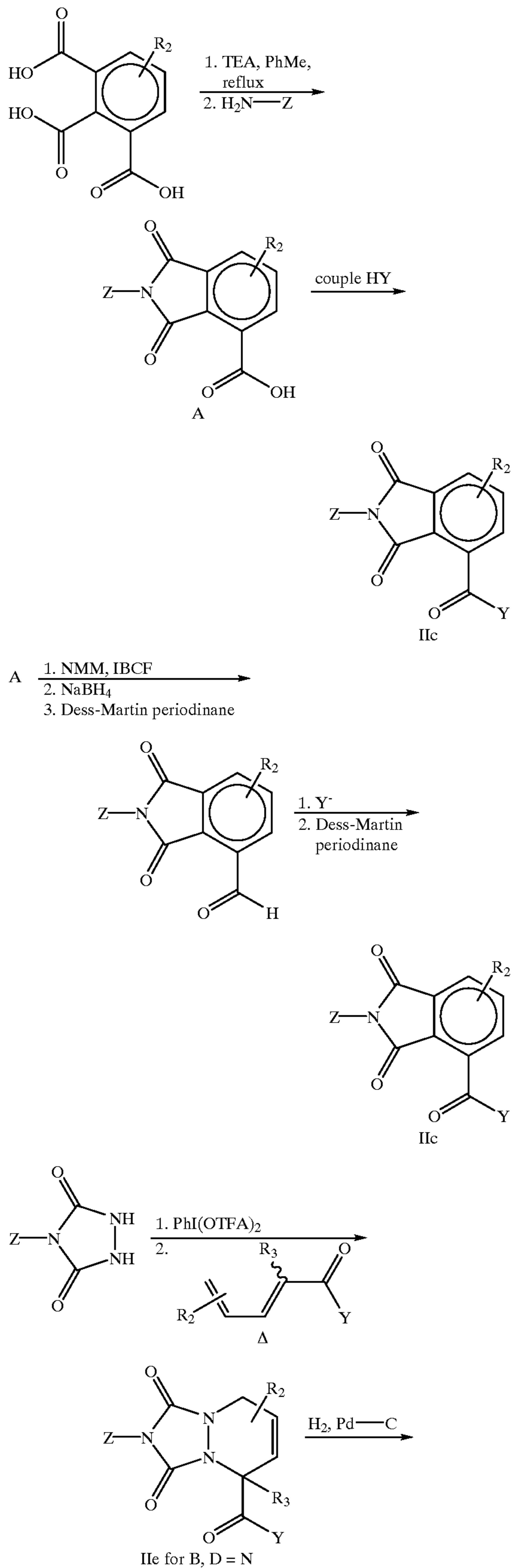
Reaction Scheme (24)
