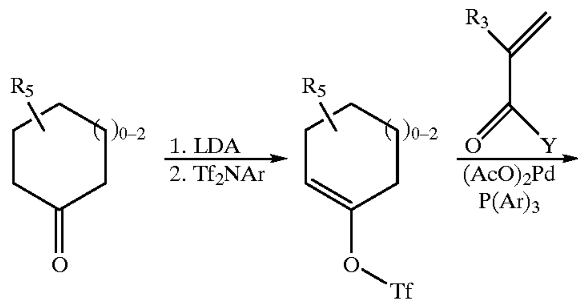
Reaction Scheme (27)
