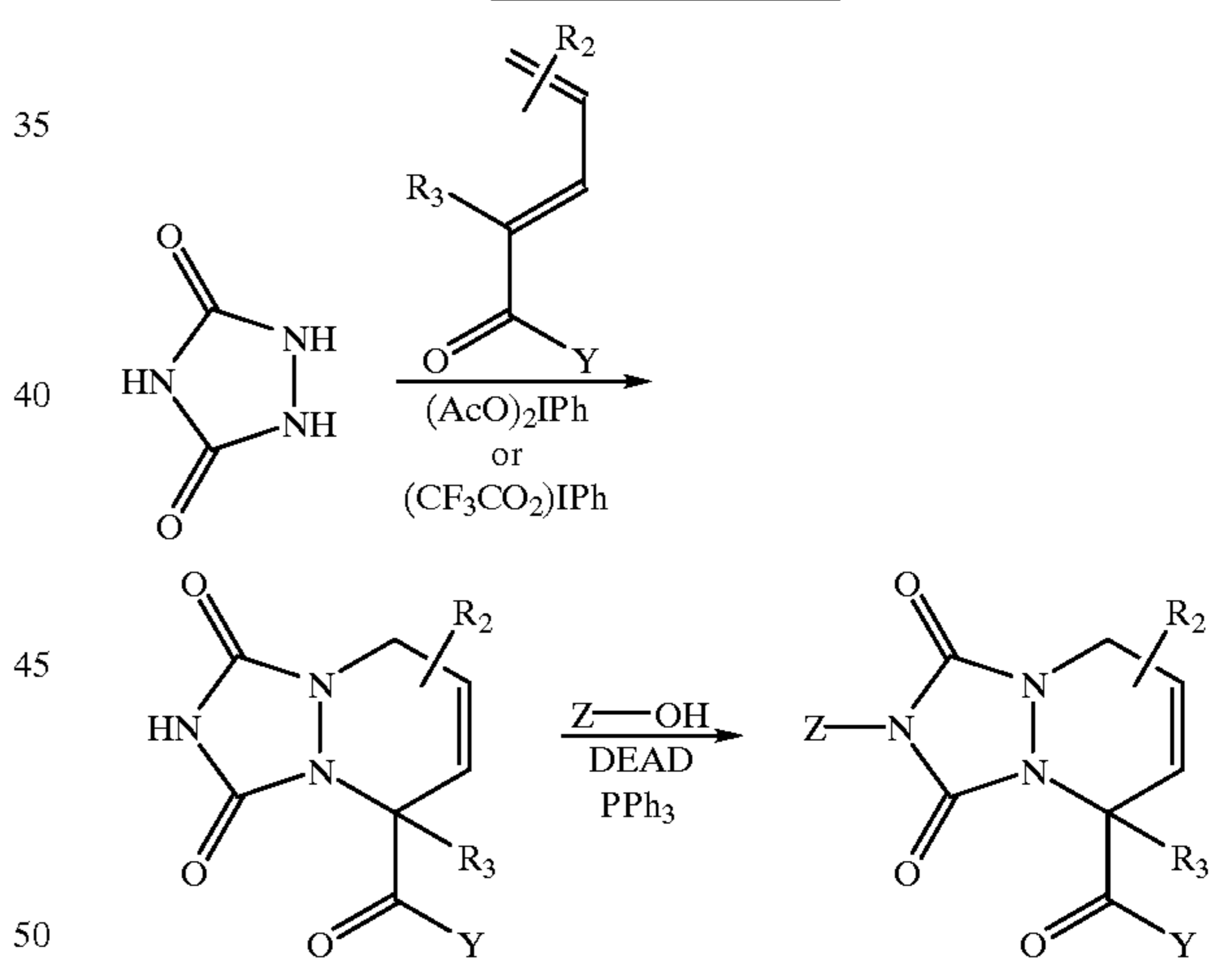
Reaction Scheme (28)
