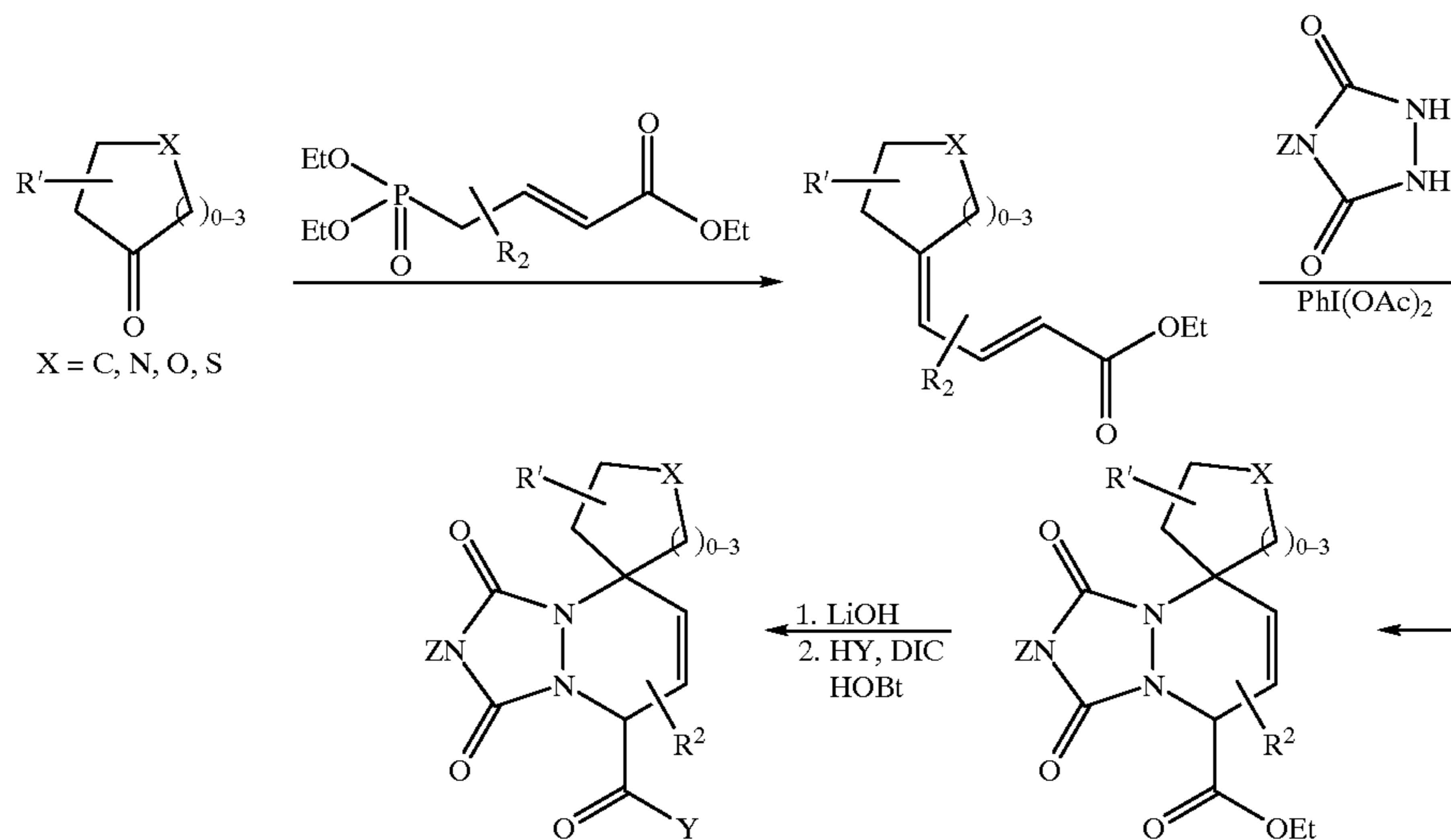
Reaction Scheme (29)
