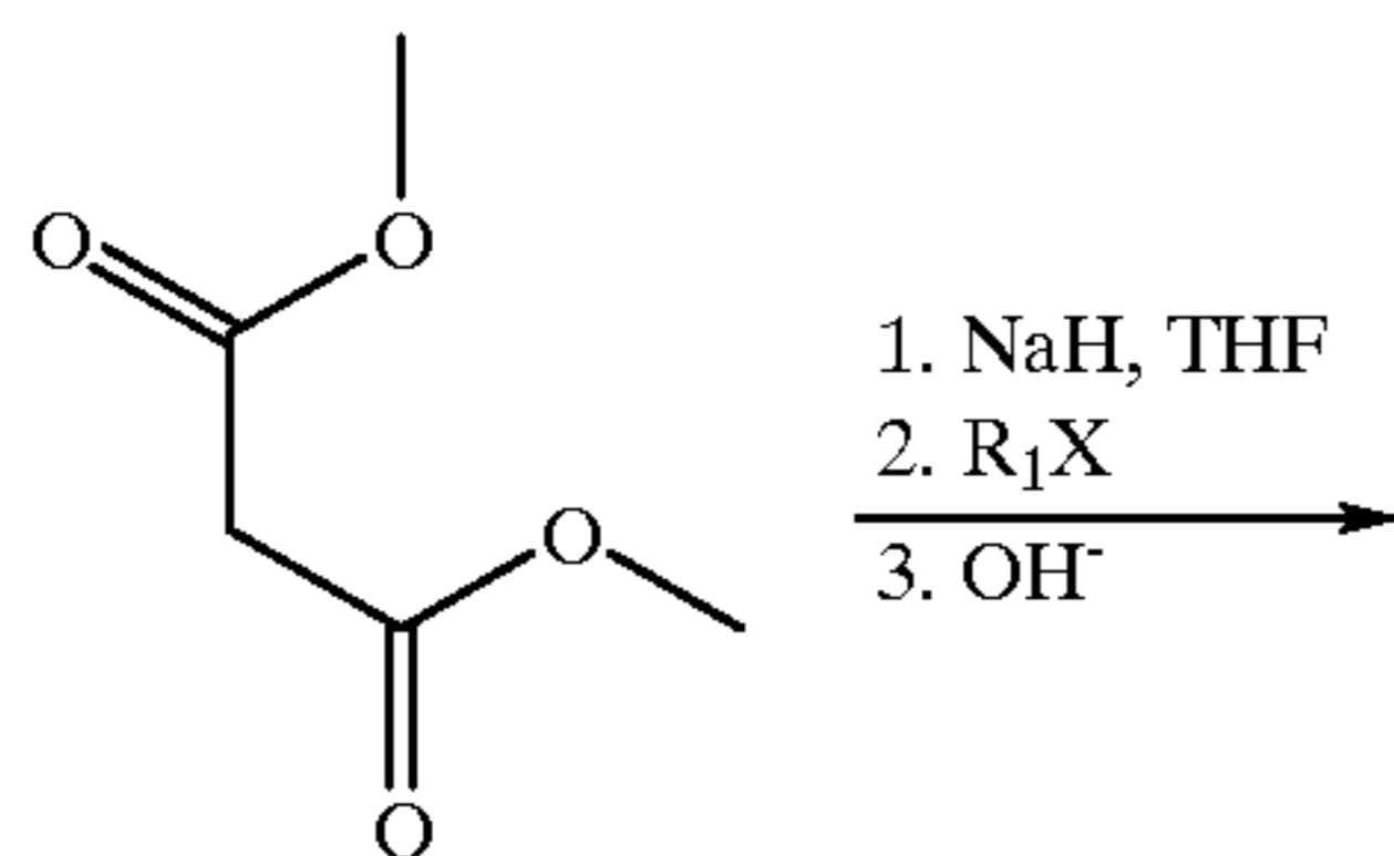
Reaction Scheme (21-1)
