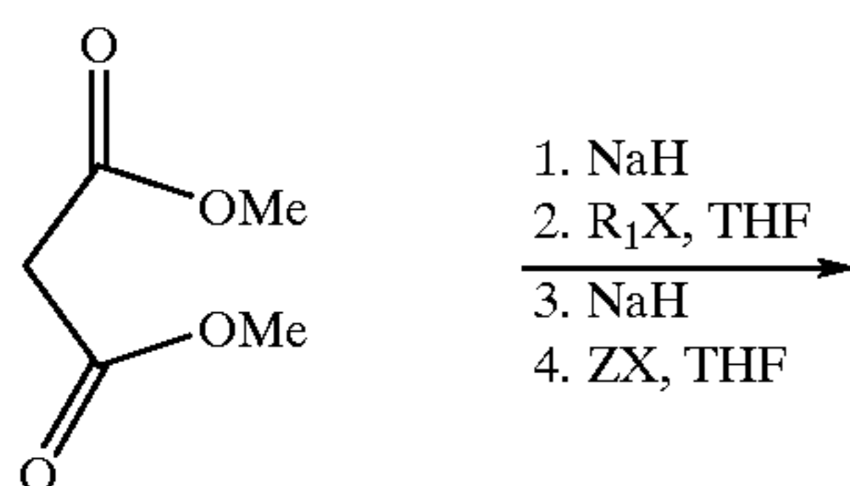
Reaction Scheme (20)
