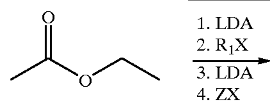
Reaction Scheme (21)
