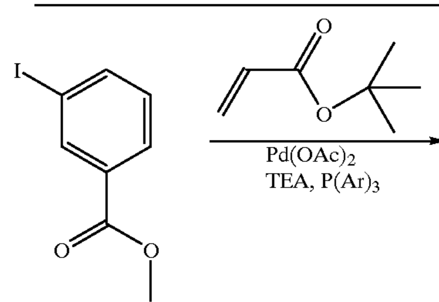
Reaction Scheme (19)
