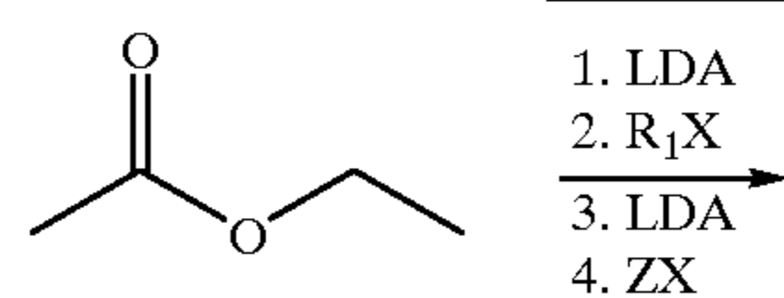
Reaction Scheme (21)
