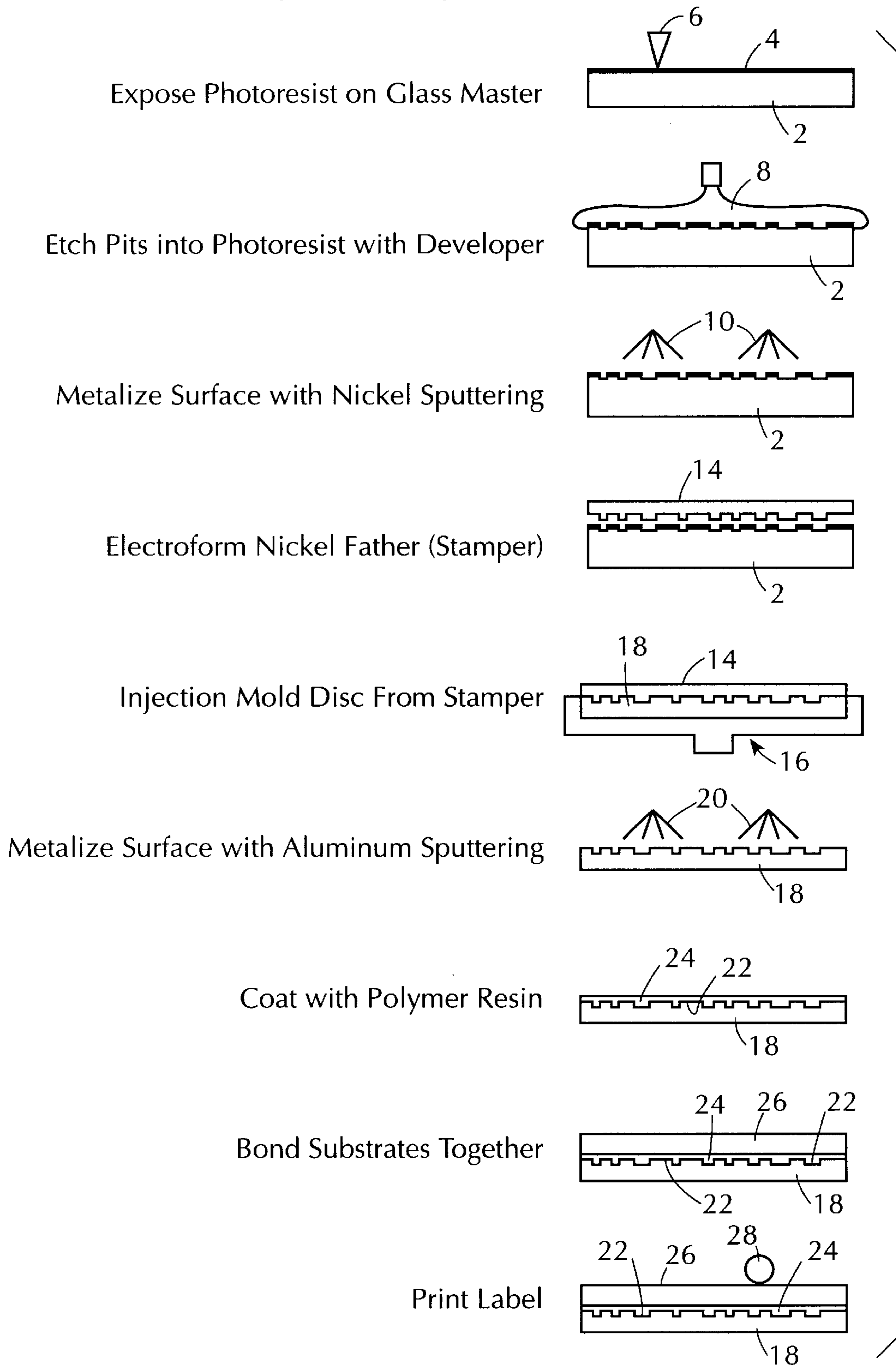
FIG. 1 Prior Art (Single Layer, Single Side: DVD-5)
