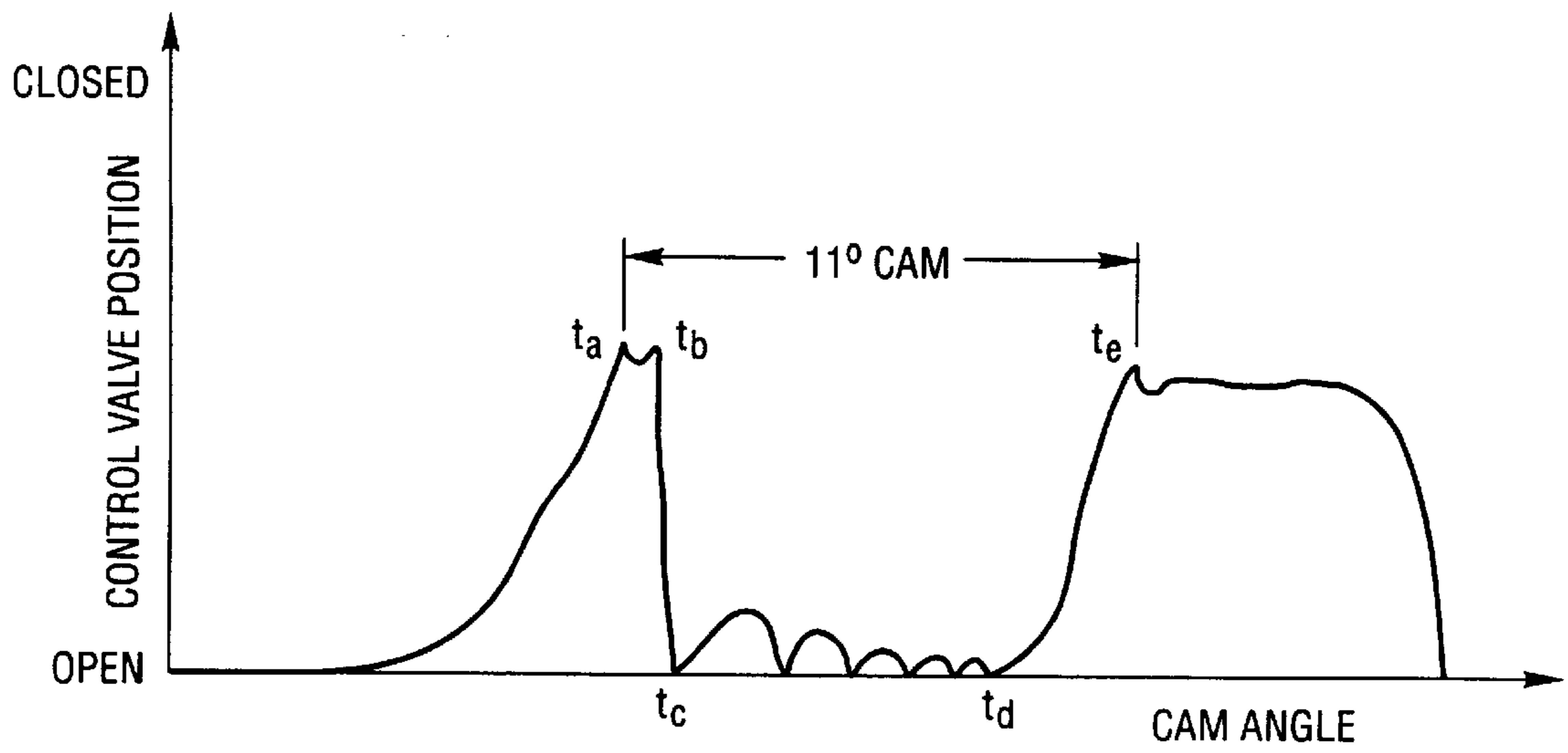
Fig. 1 (PRIOR ART)
