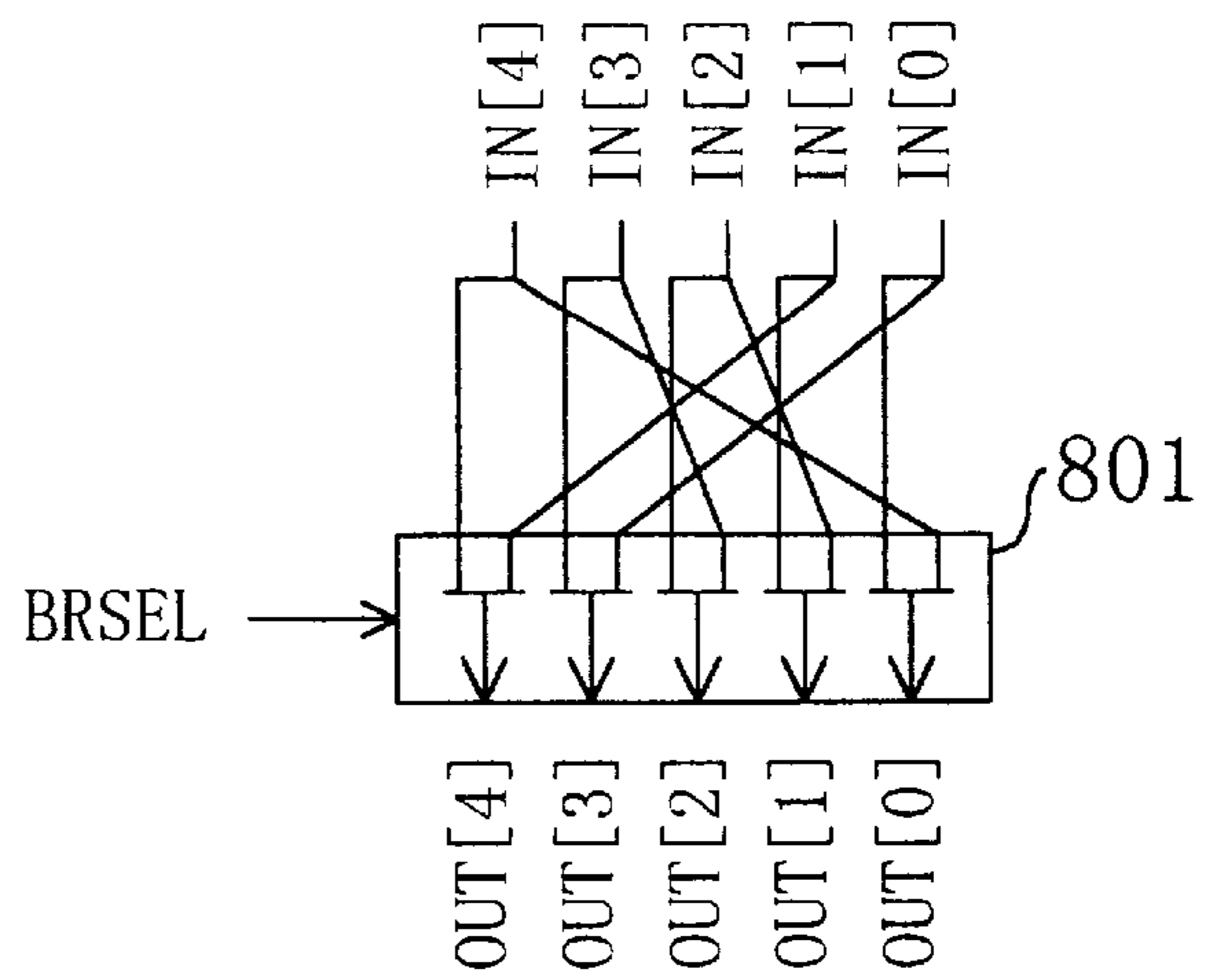
Fig. 24(a) BIT REVERSE CIRCUIT BR
