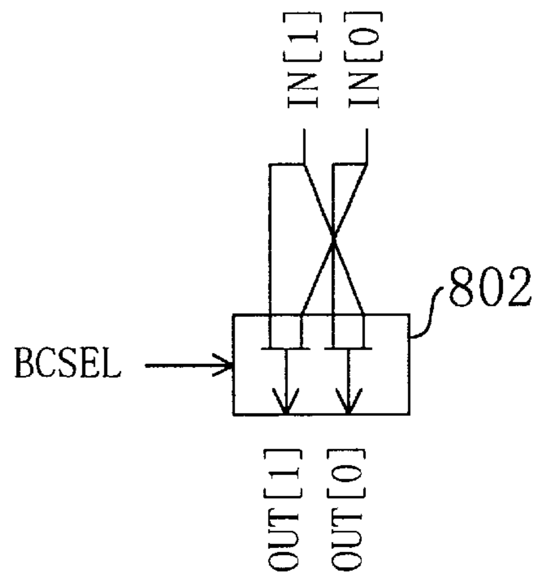
Fig. 24(b) BIT EXCHANGING CIRCUIT BC
