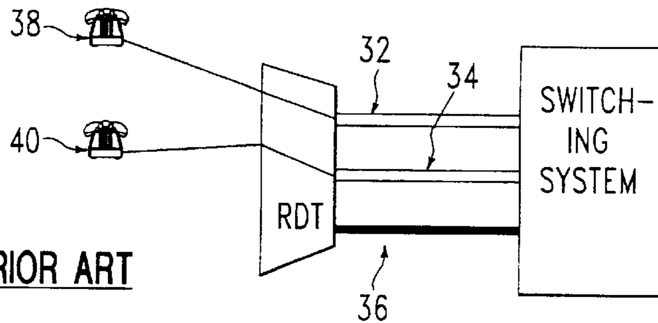
FIG. 1 PRIOR ART
