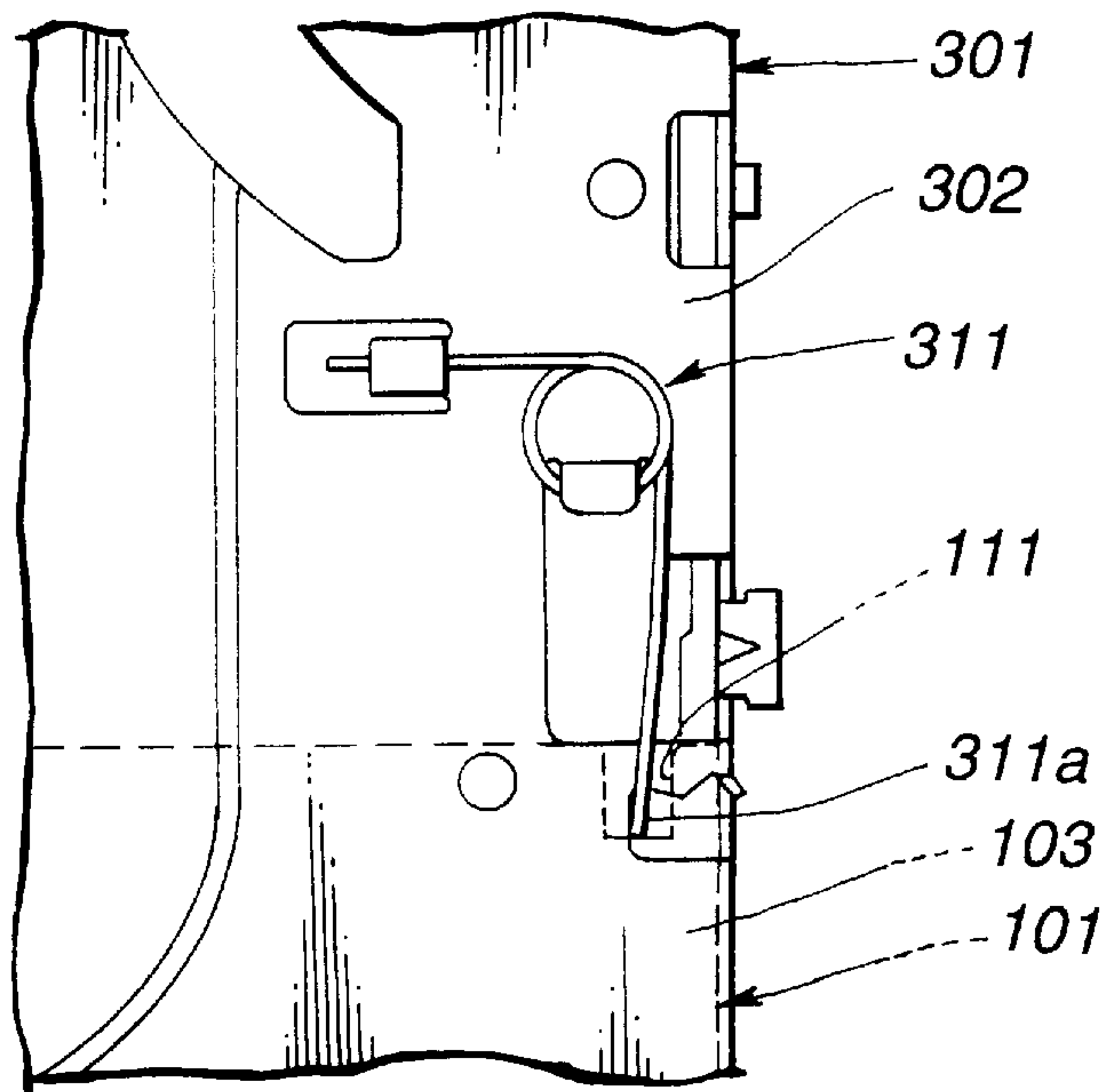
FIG.29 (RELATED ART)
