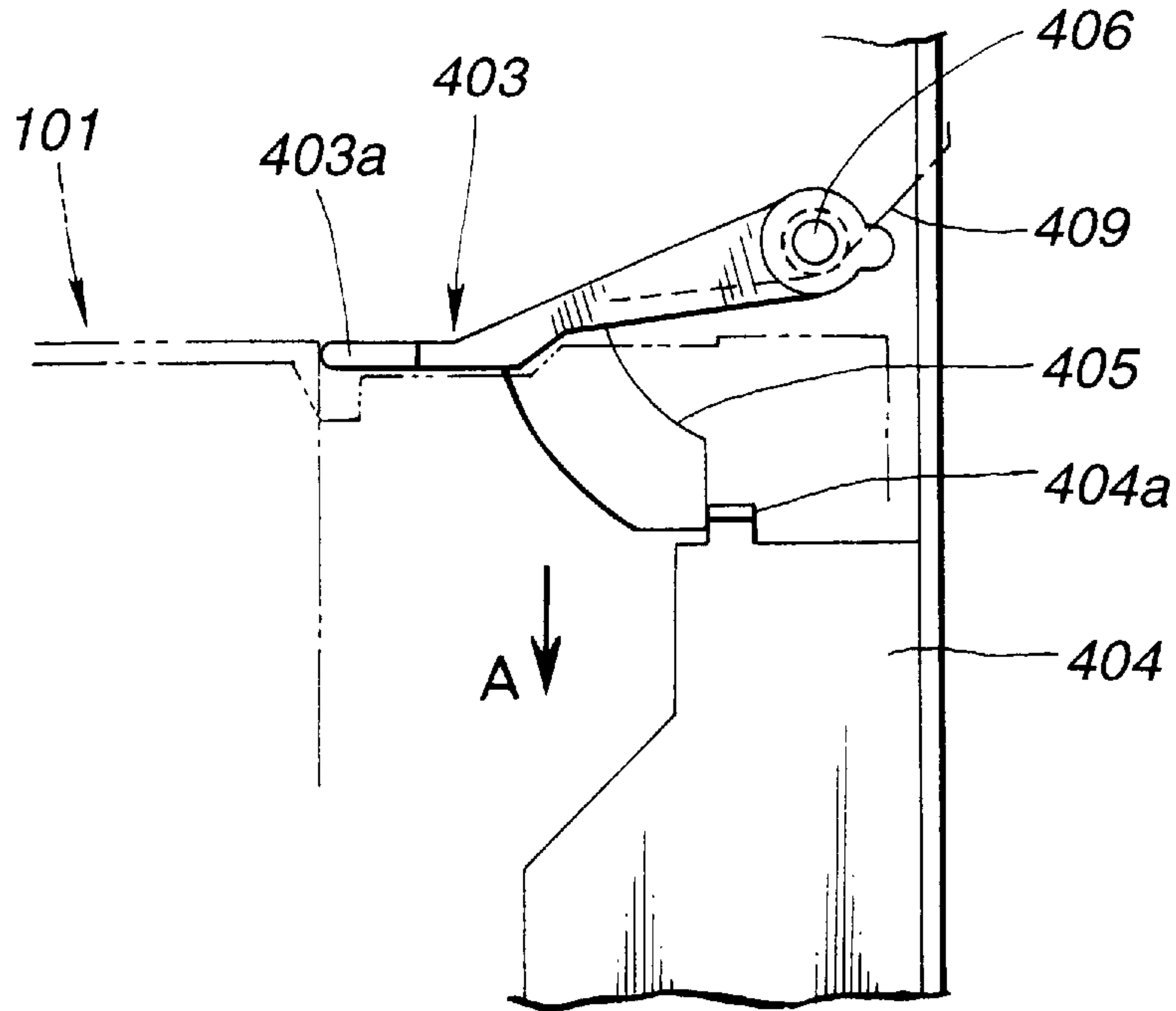
FIG.28 (RELATED ART)
