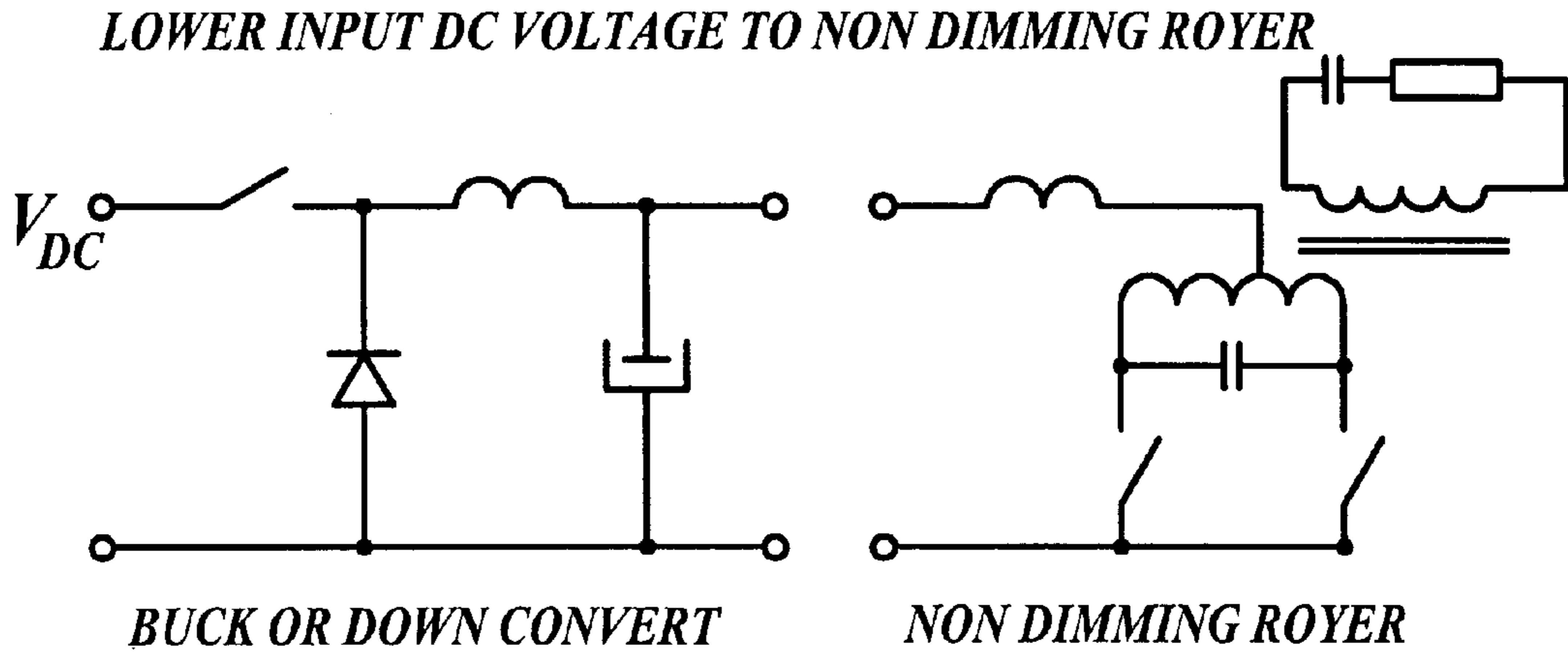
Fig. 2 (PRIOR ART)
