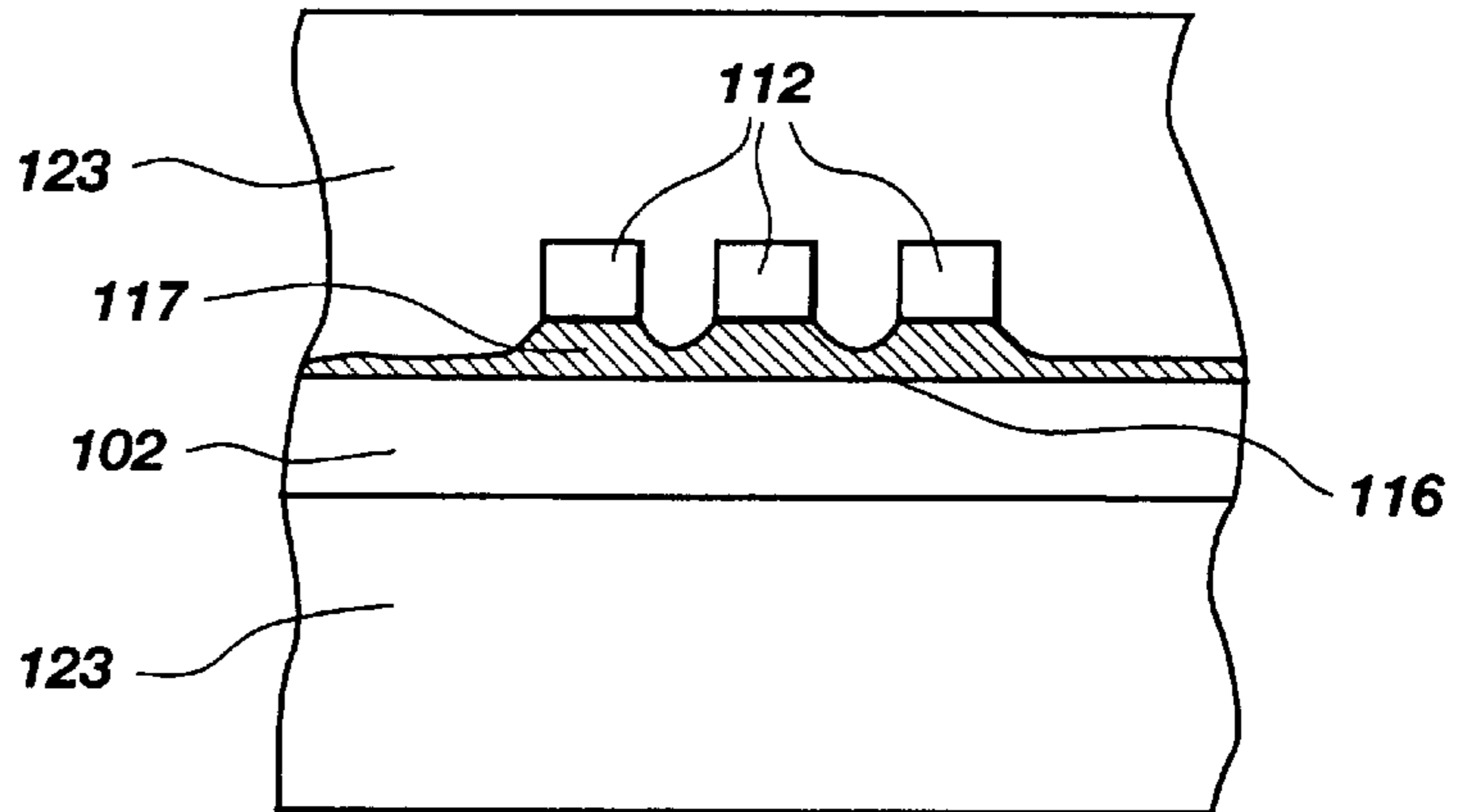
SECTION 10-10
