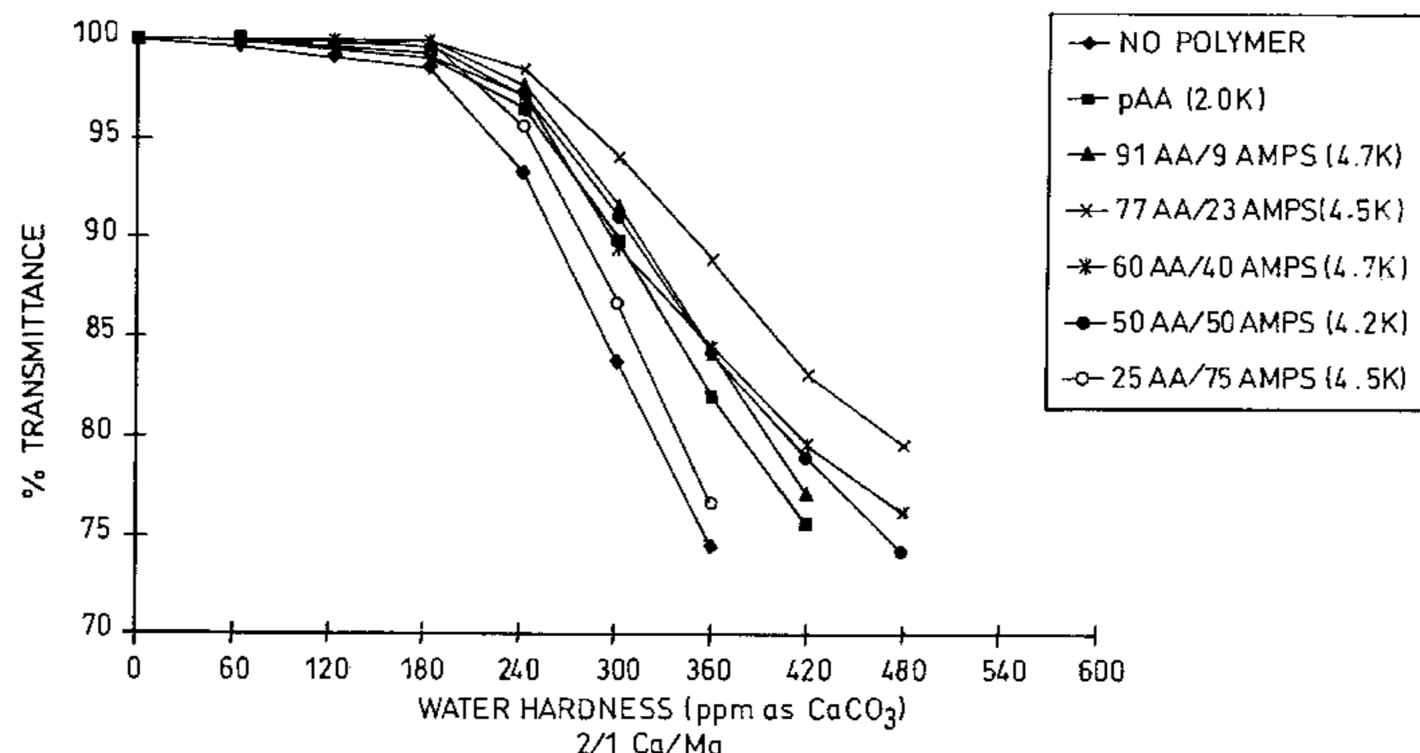
INHIBITION OF CALCIUM TRIPOLYPHOSPHATE AS A FUNCTION OF AMPS COMONOMER CONCENTRATION/WATER HARDNESS
