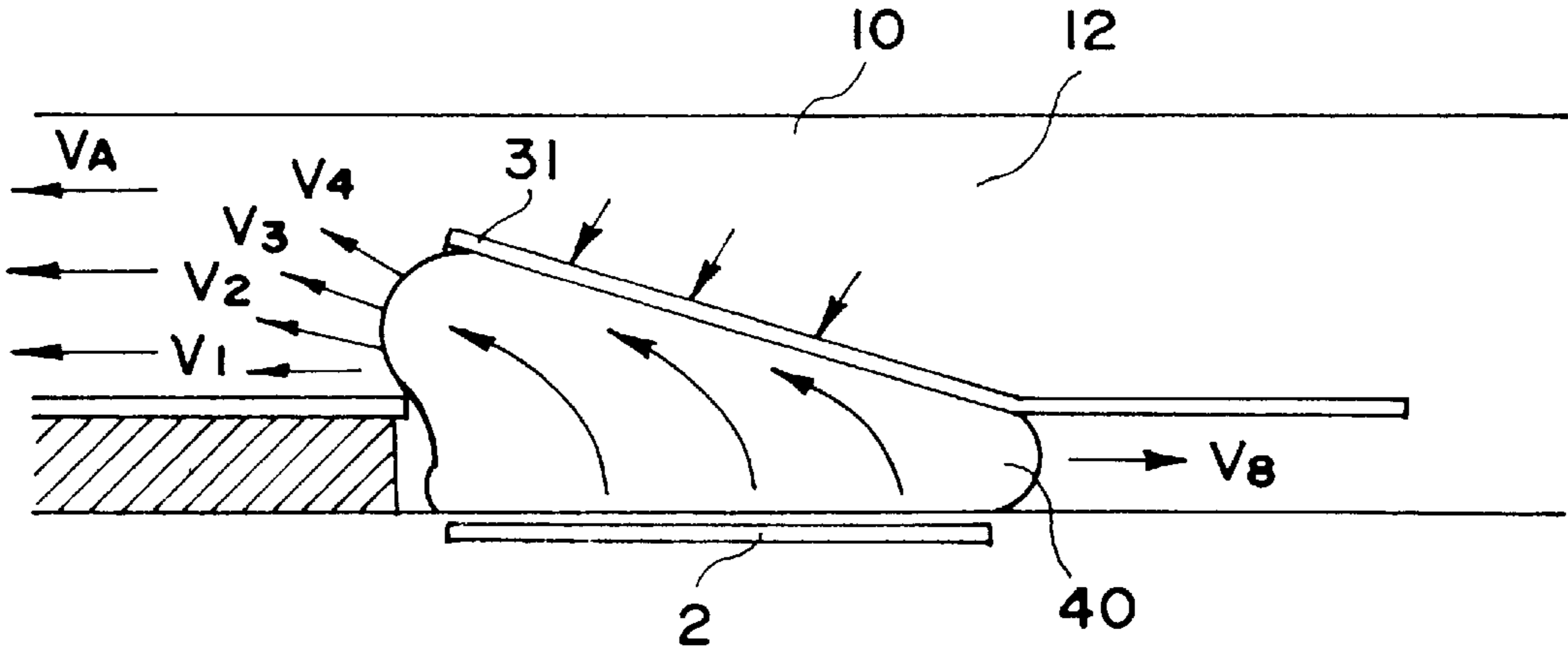
FIG. 6 PRIOR ART
