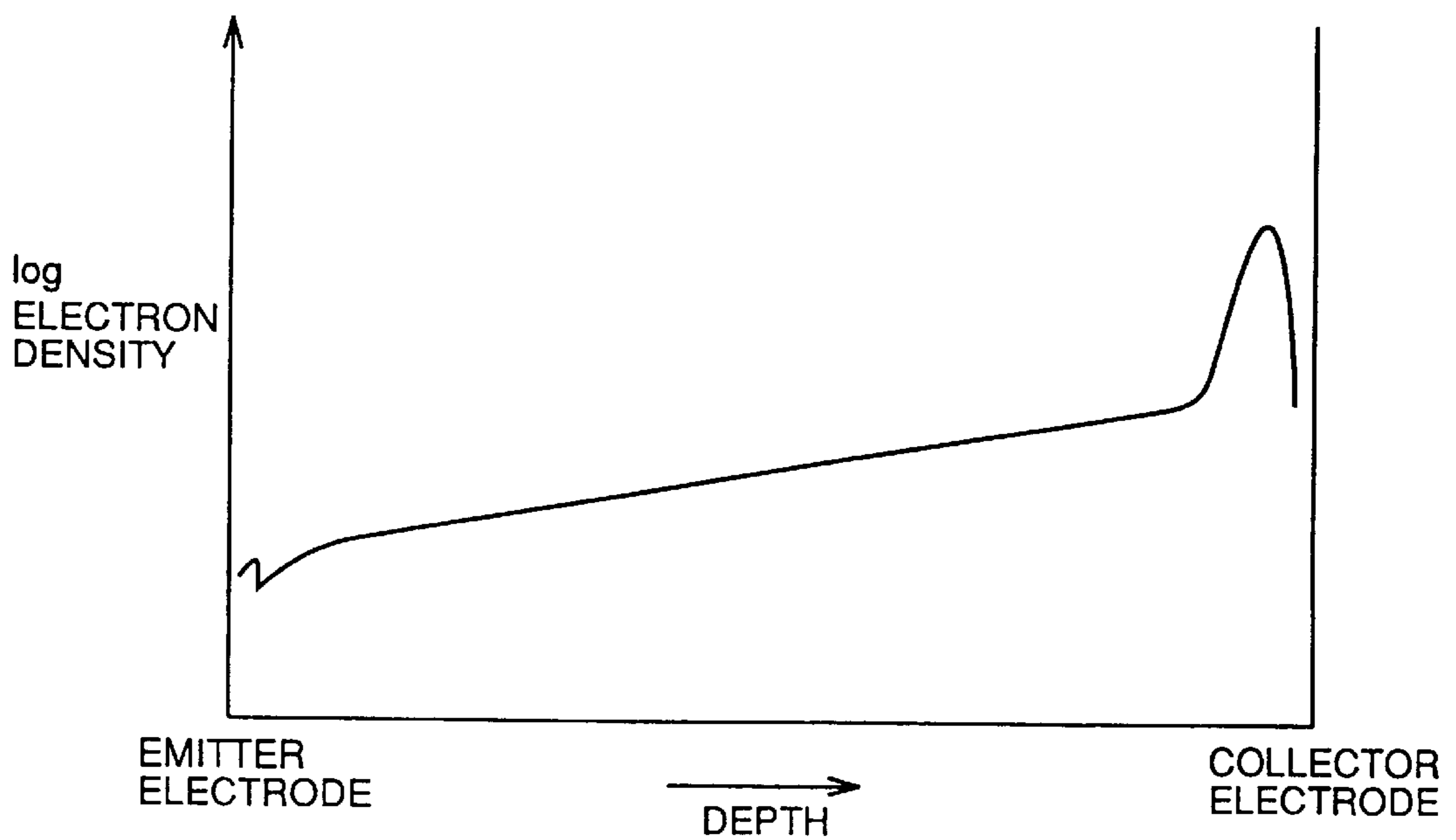
FIG.51 PRIOR ART
