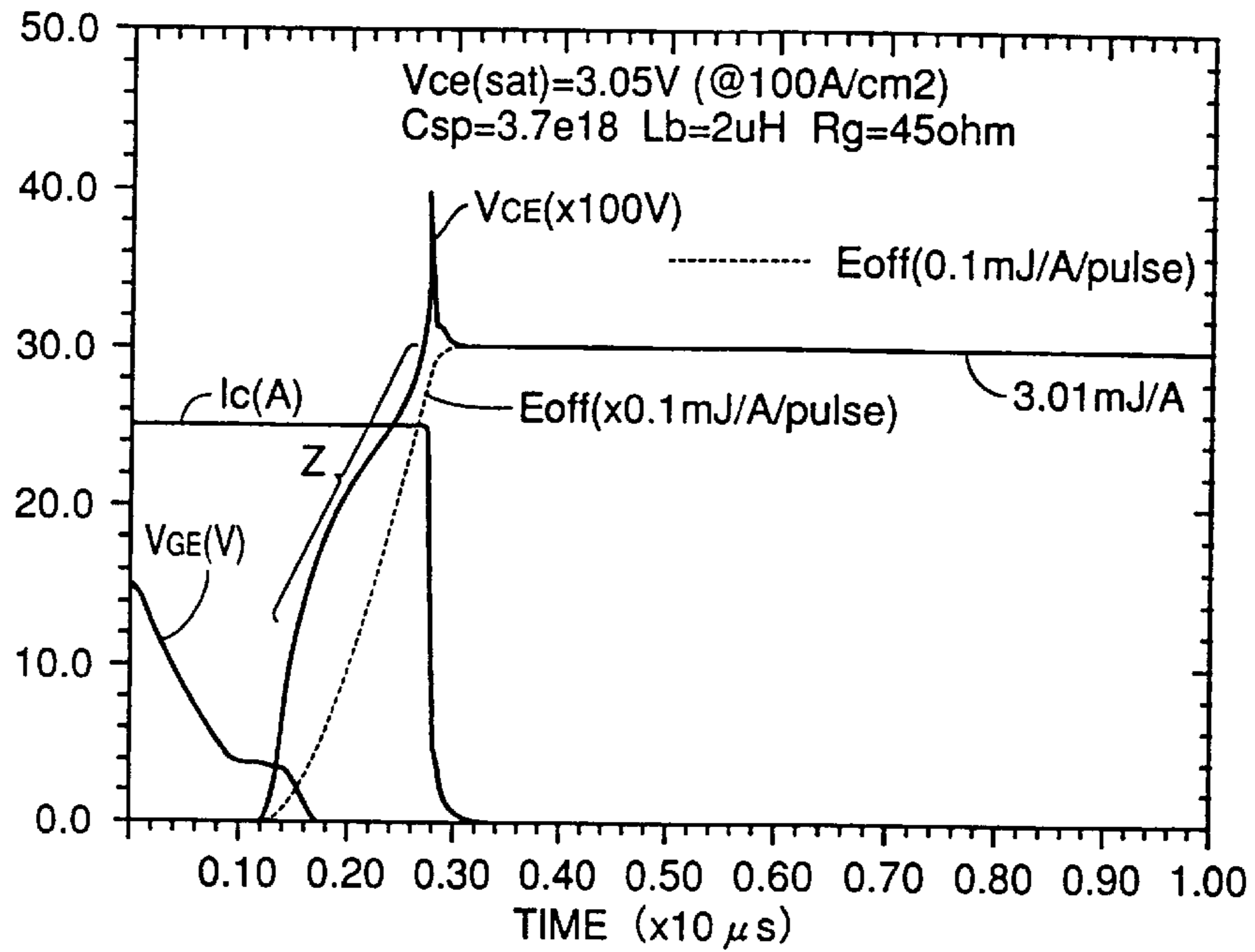
FIG.50 PRIOR ART
