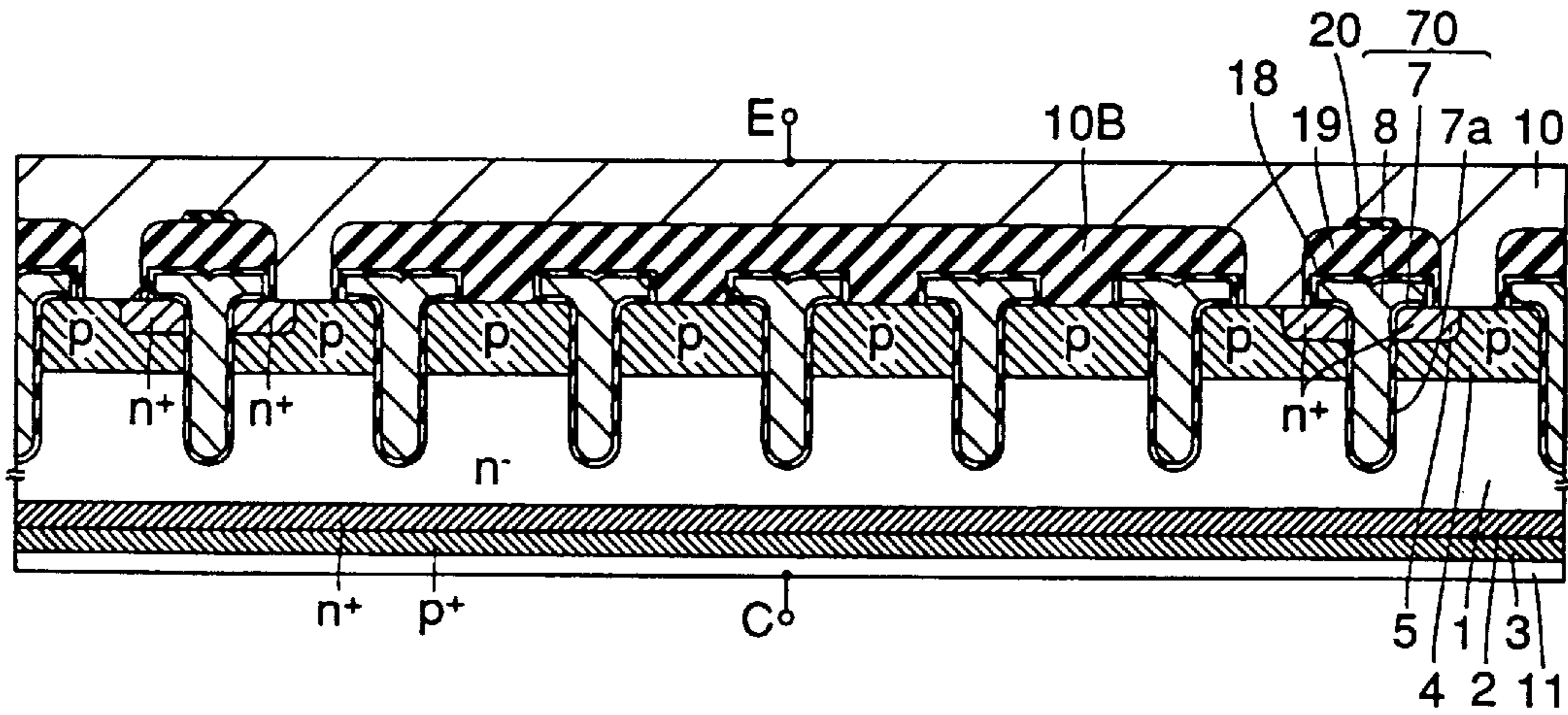
FIG.52 PRIOR ART
