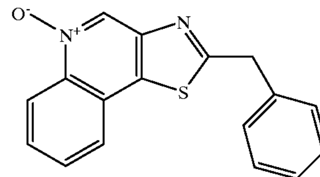
2-Benzylthiazolo[4,5-c]quinoline-5N-oxide
