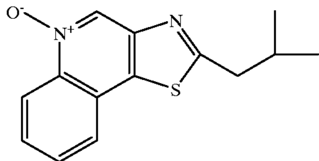
2-(2-Methylpropyl)thiazolo[4,5-c]quinoline-5N-oxide
