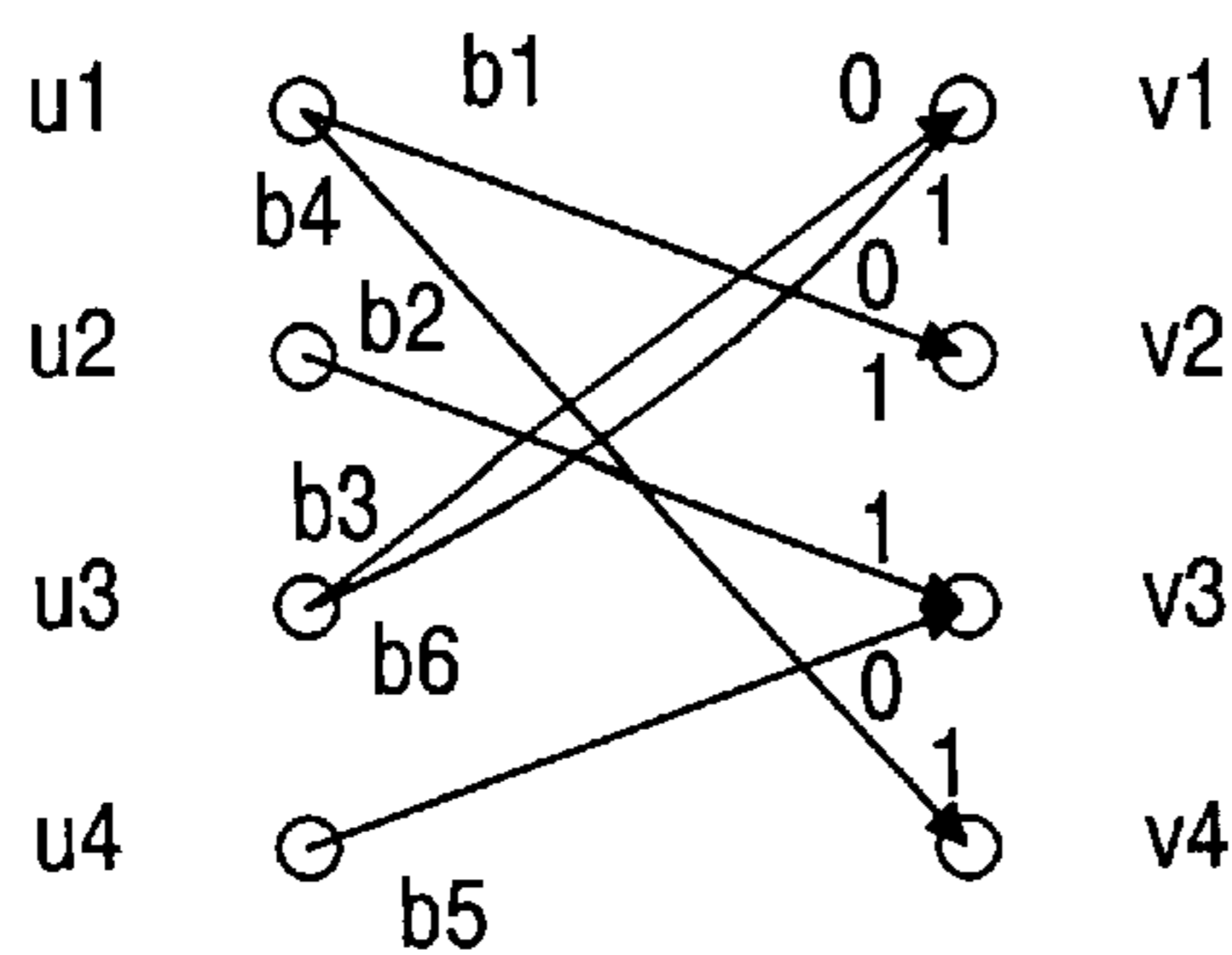
(C) THE BIPARTITE GRAPH G
