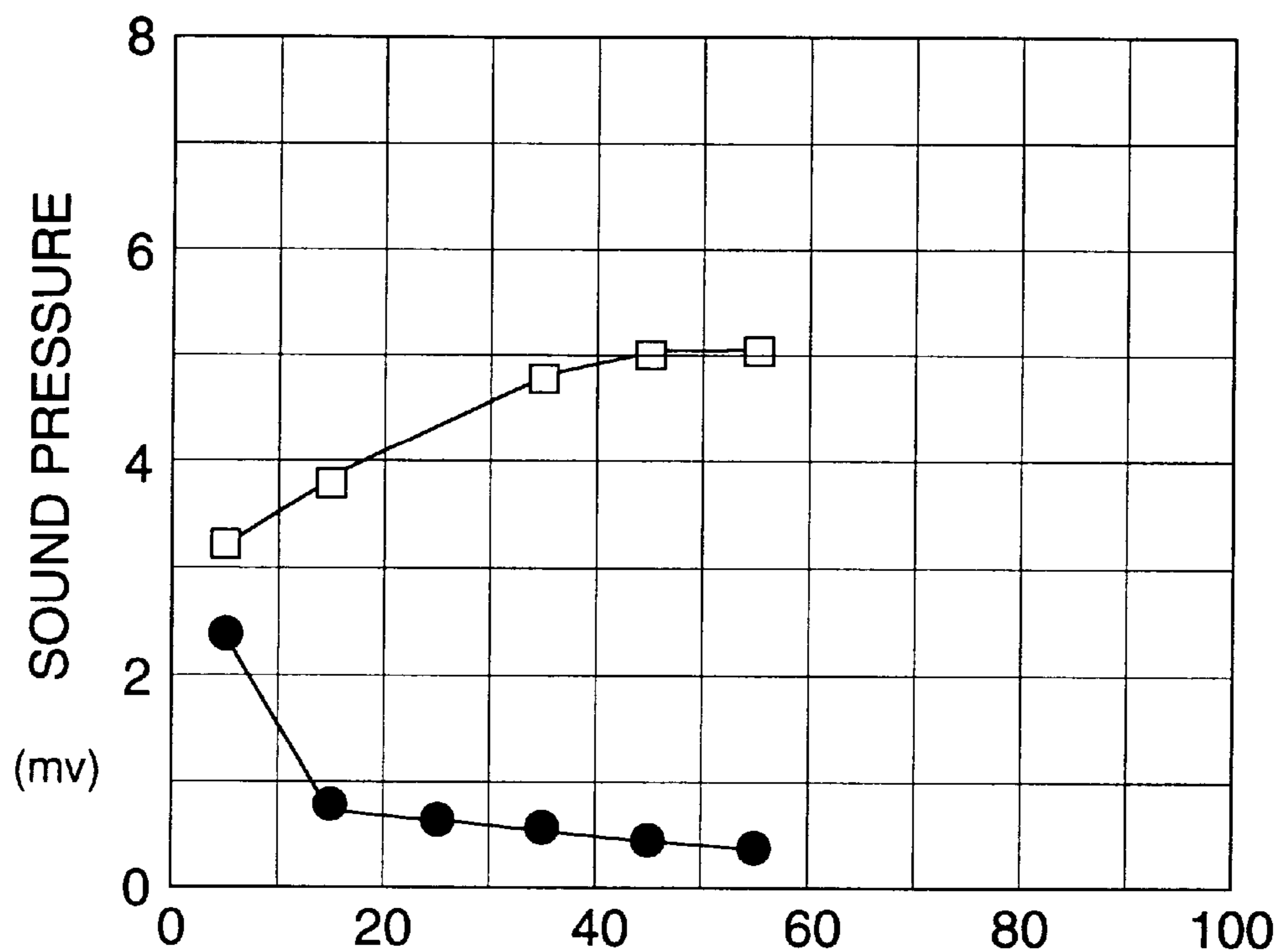
DEGREE OF UNSATURATION OF THE DENSITY OF DISSOLVED AIR IN THE LIQUID FOR TRANSFERRING ULTRASONIC WAVE UNDER USING CONDITIONS (%)
