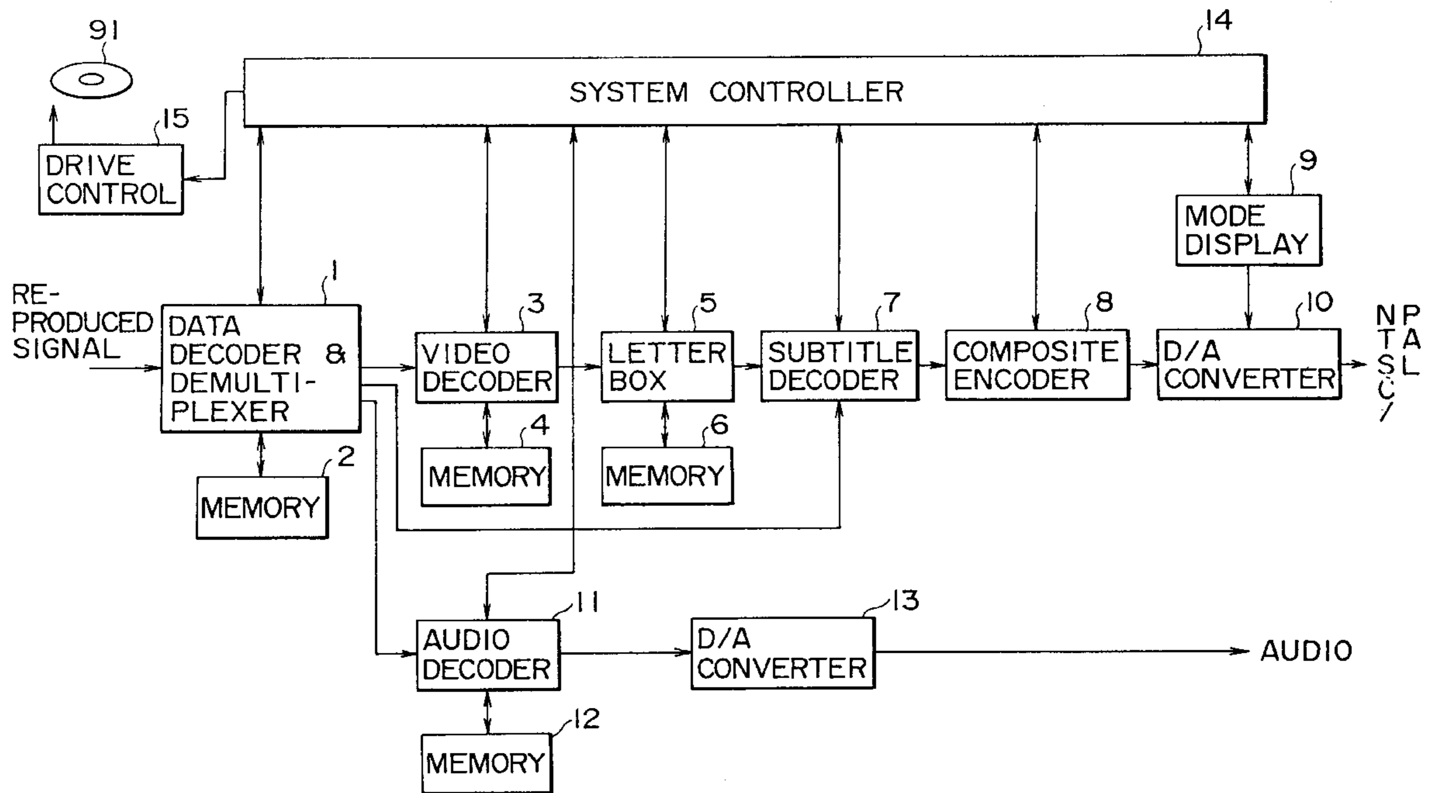
BLOCK DIAGRAM OF INTRA-PLAYER CIRCUITS
