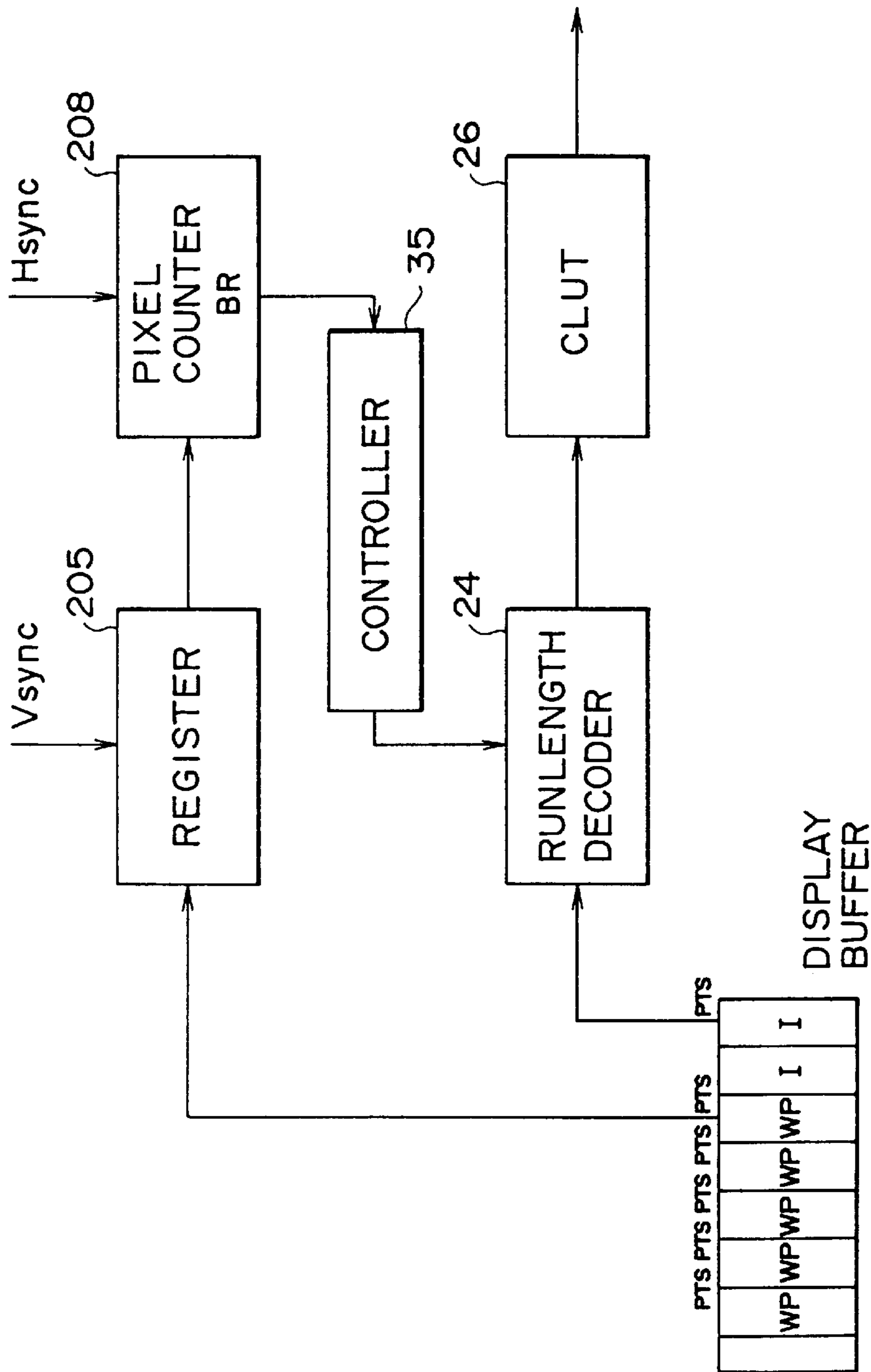
BLOCK DIAGRAM FOR POSITION CONTROL
