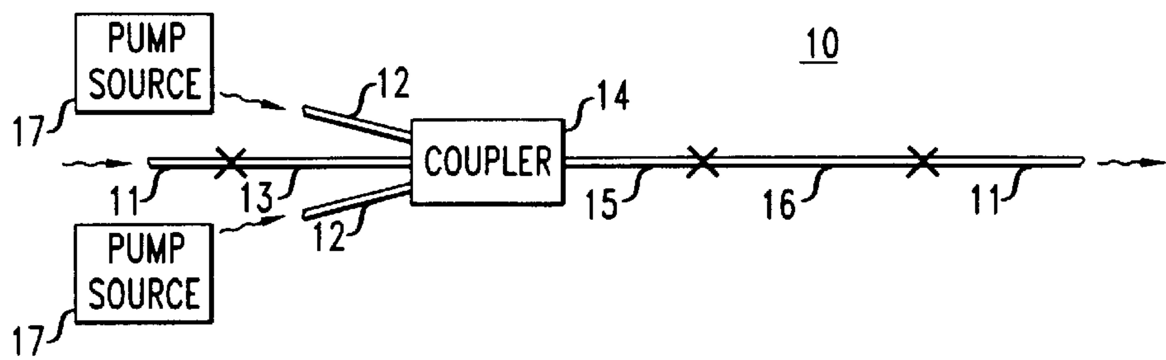
FIG. 1 (PRIOR ART)
