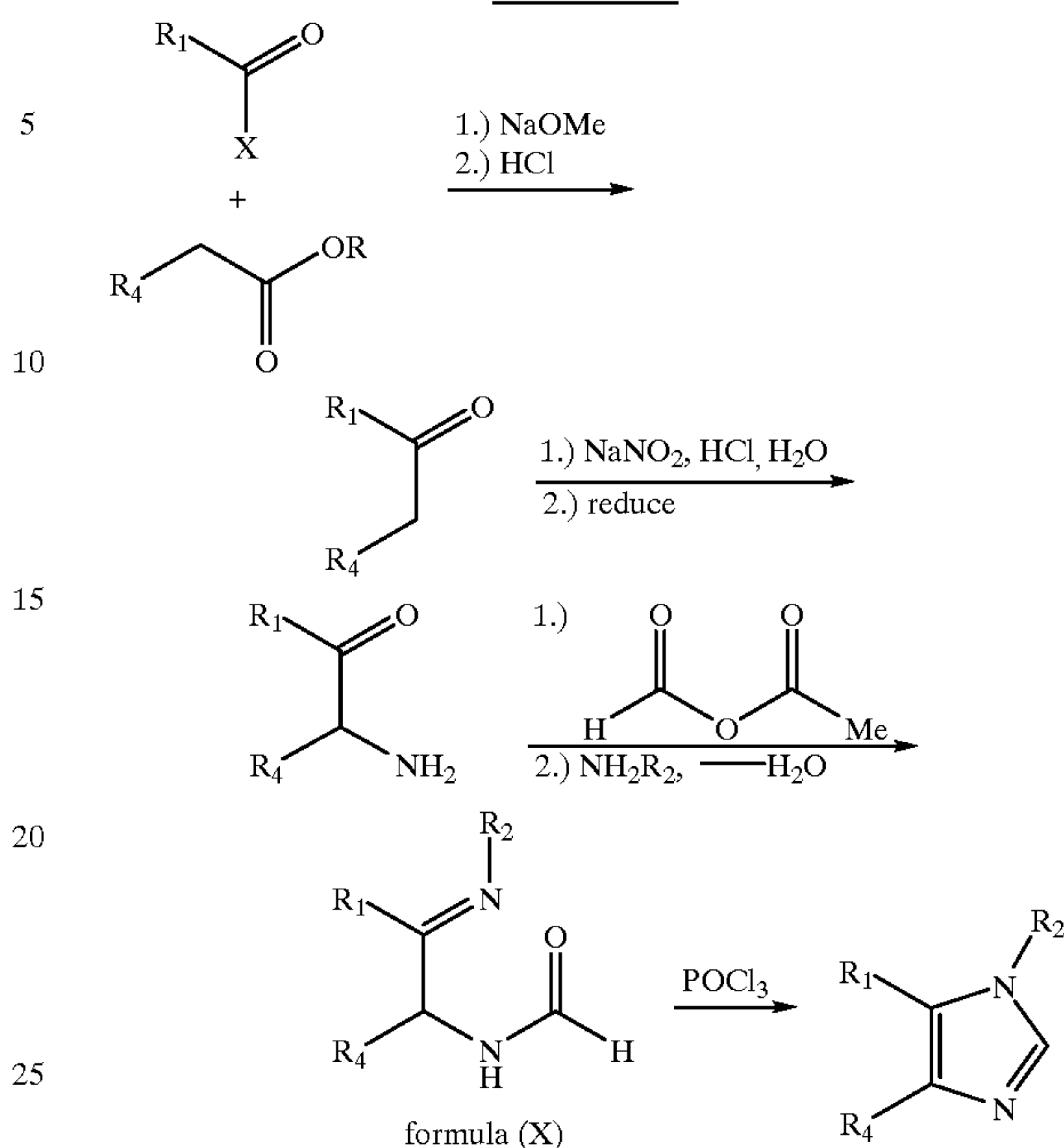
SCHEME III
