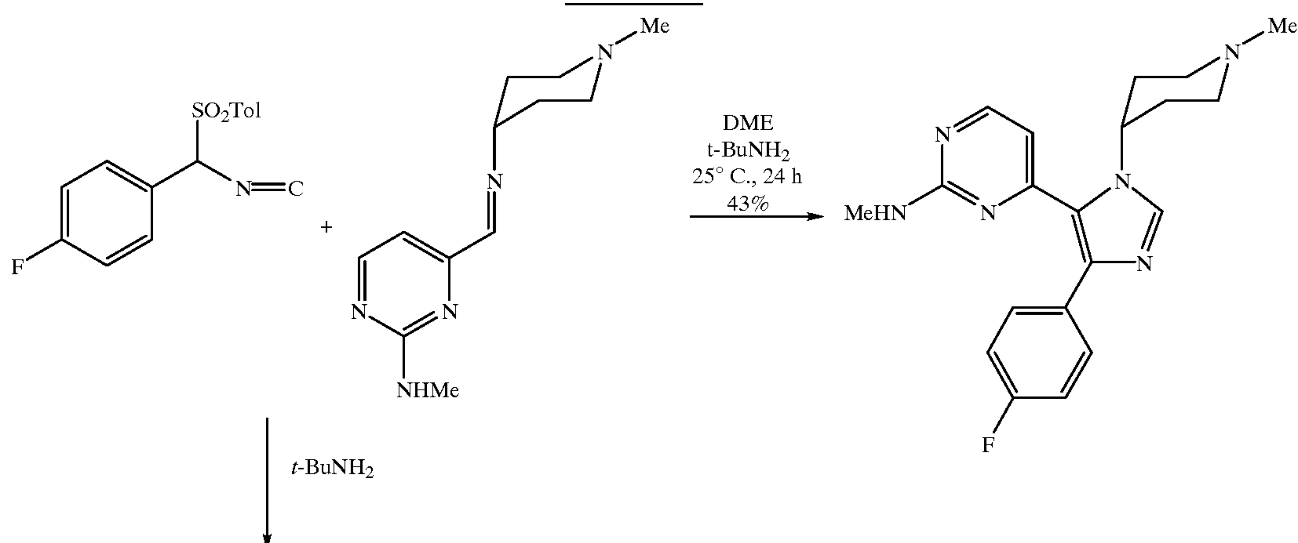
SCHEME VII
