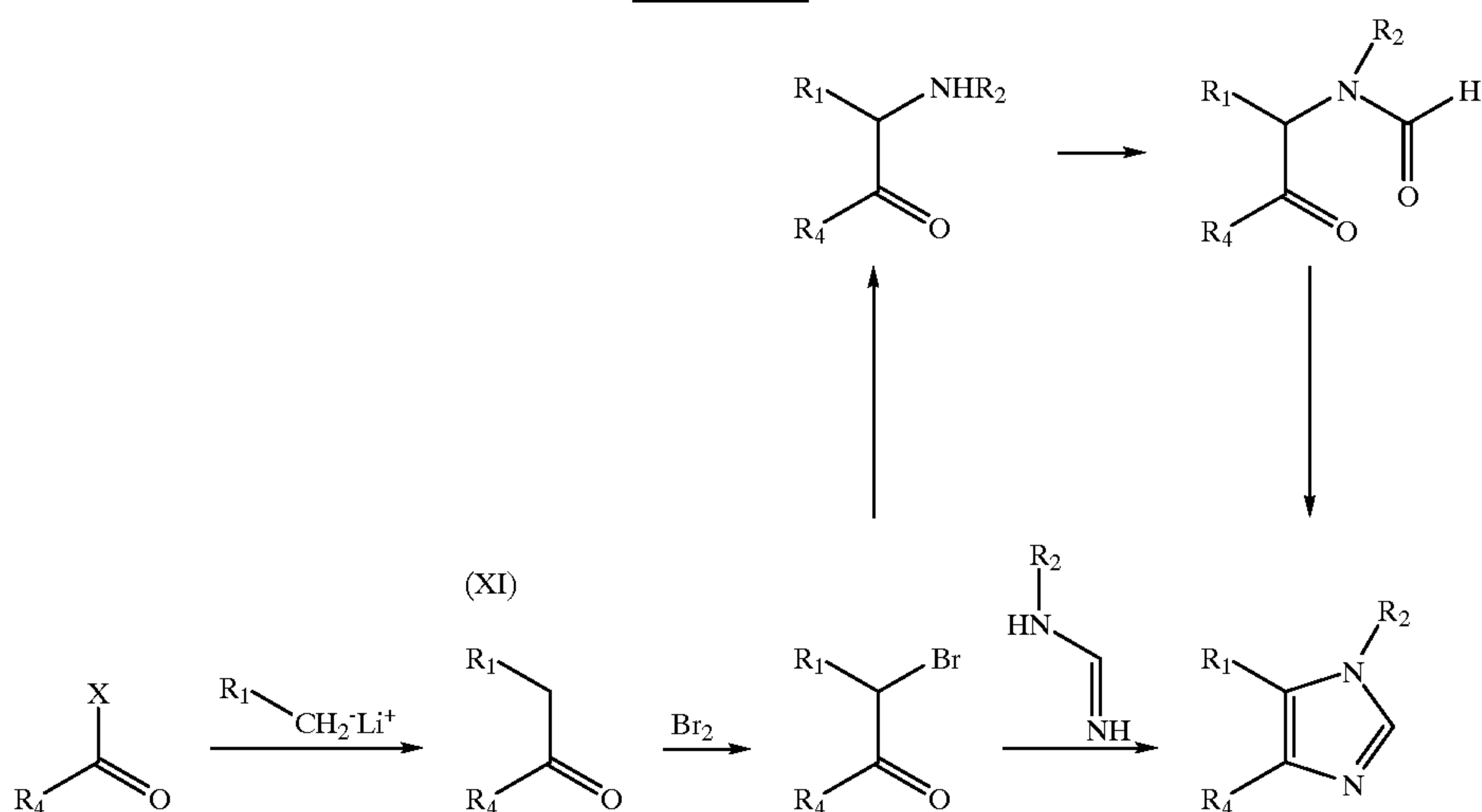
SCHEME IV
