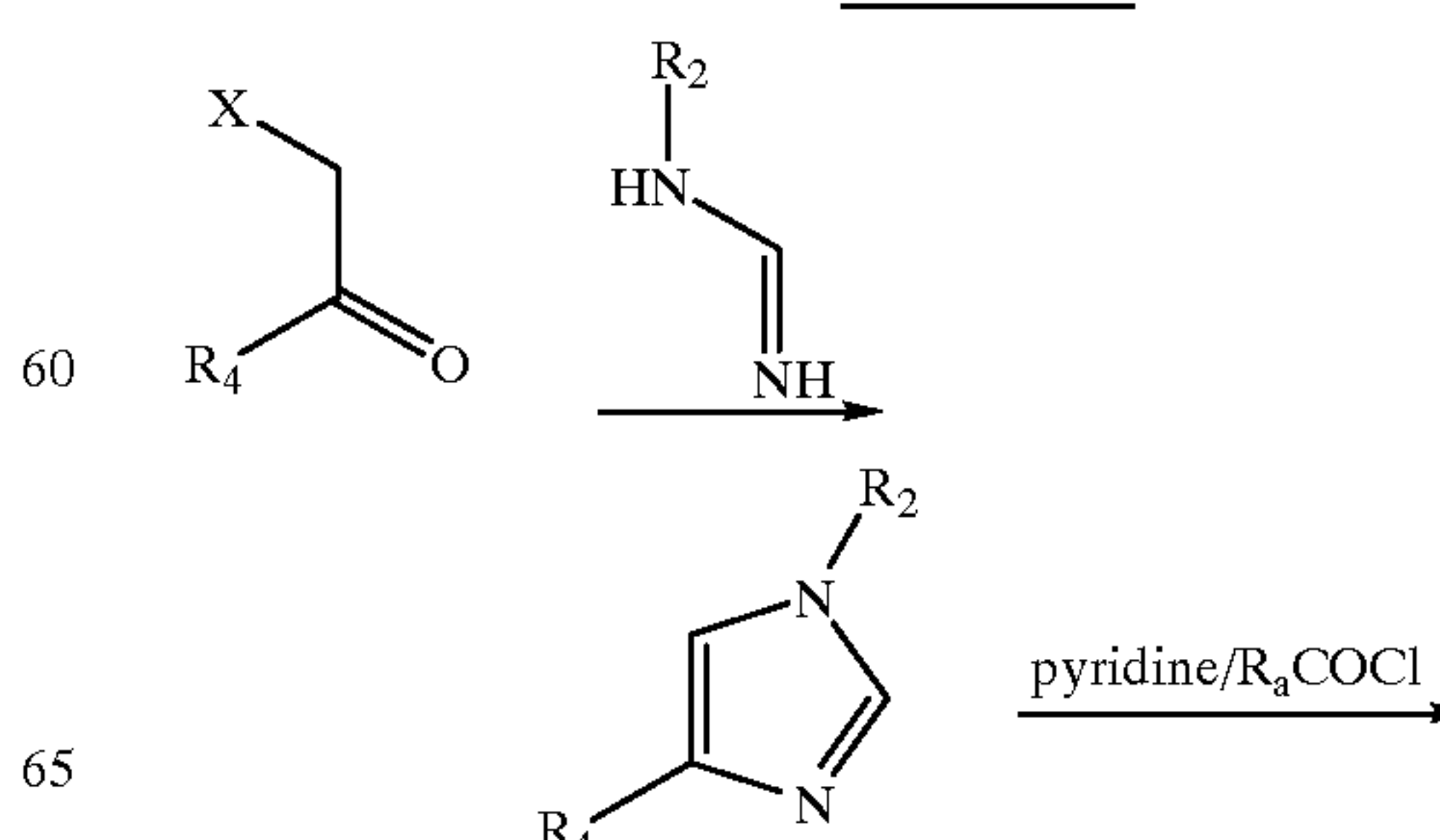
SCHEME II
