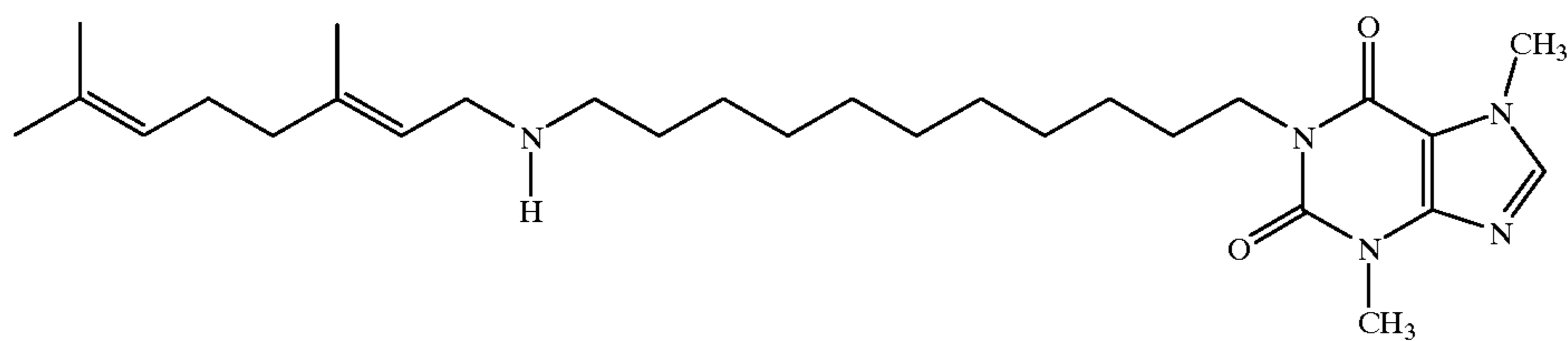
6579 1-[11-(trans-3,7-Dimethyl-2,6-octadienylamino)undecyl]-3,7-dimethylxanthine
