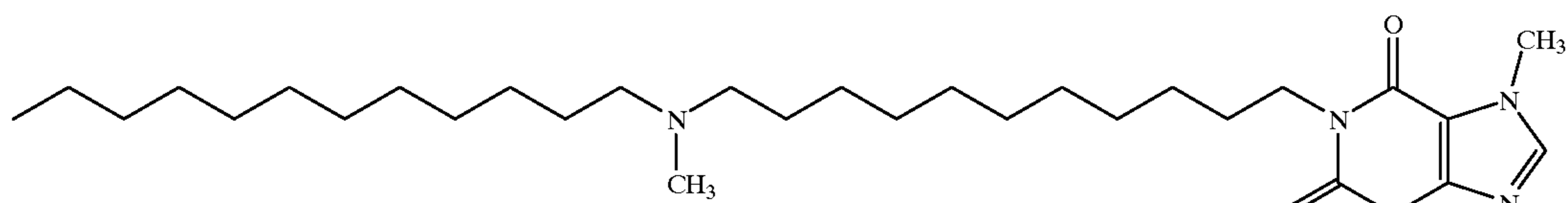
3576 1-[11-(N-Methyl-N-dodecylamino)undecyl]-3,7-dimethylxanthine
