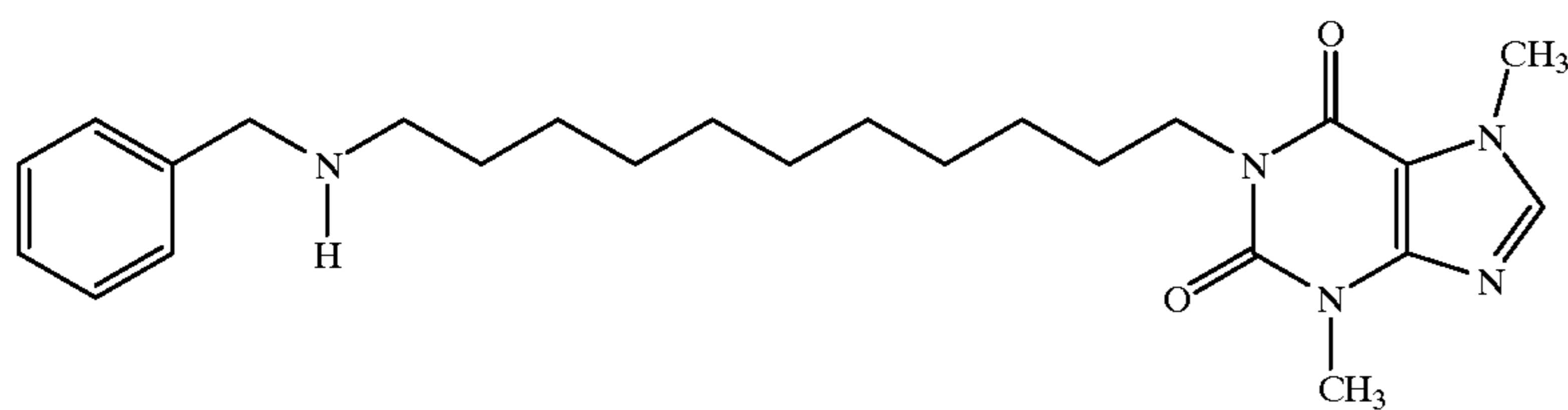
6531 1-[11-Benzylaminoundecyl]-3,7-dimethylxanthine
