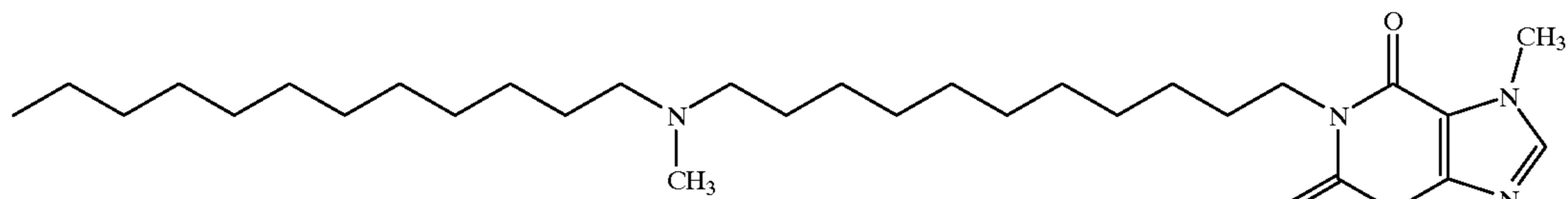
3576 1-[11-(N-Methyl-N-dodecylamino)undecyl]-3,7-dimethylxanthine
