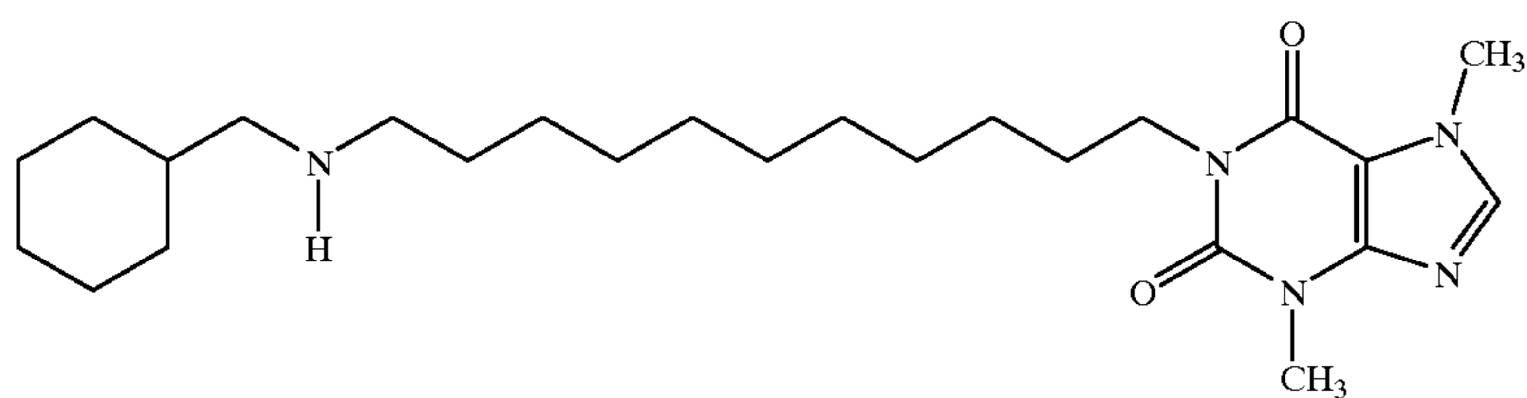
6542 1-[11-(Cyclohexylmethylamino)undecyl]-3,7-dimethylxanthine
