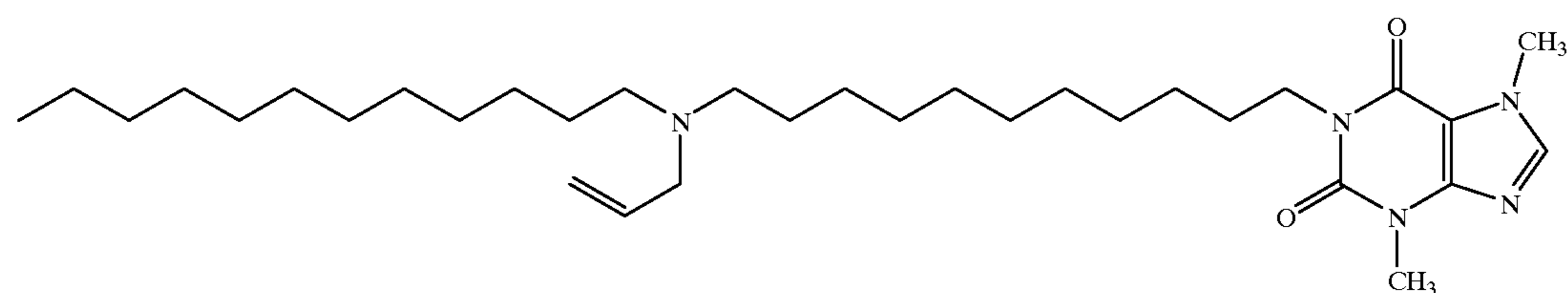
6563 1-(11-Allyldodecylaminoundecyl)-3,7-dimethylxanthine
