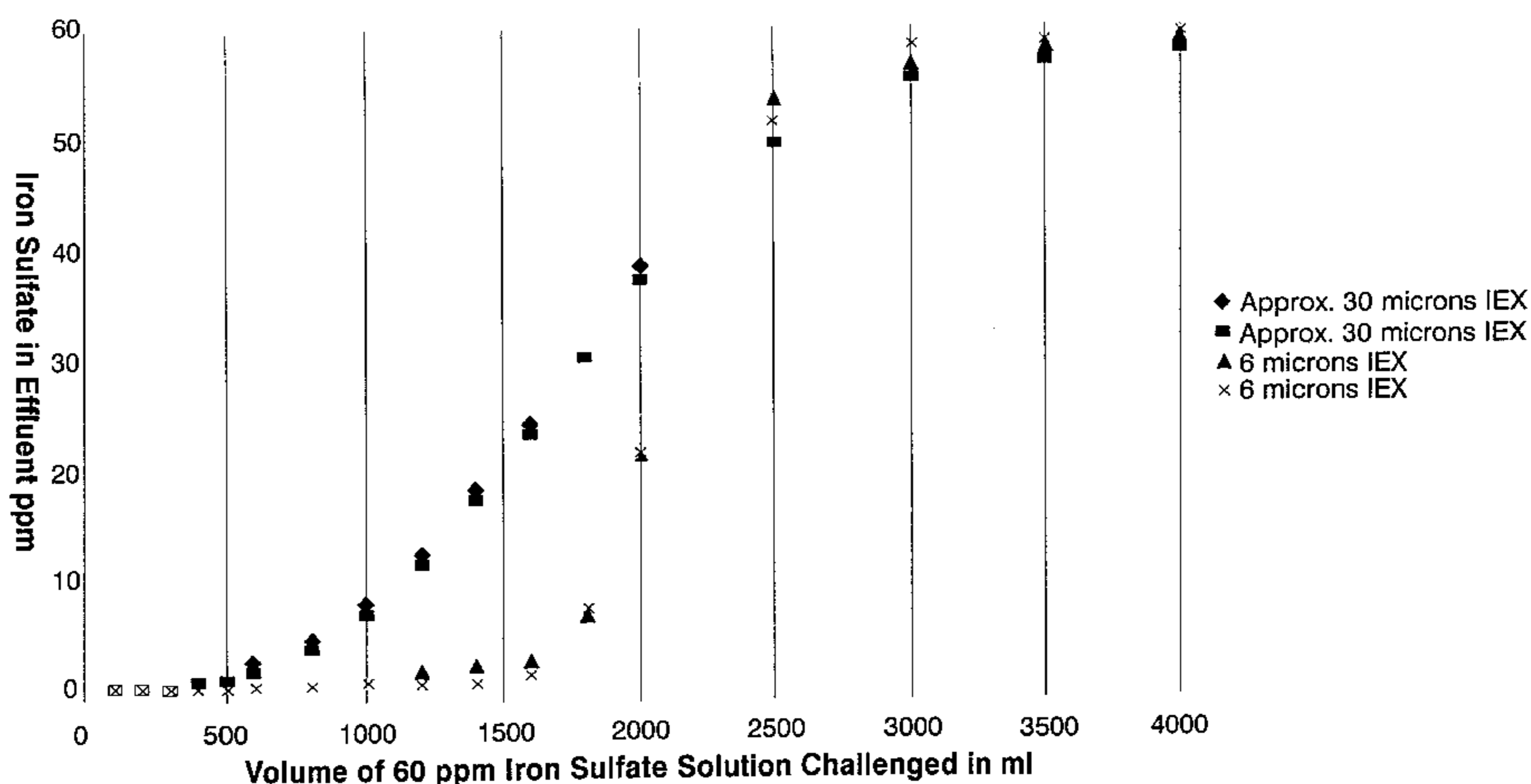
Effect of IEX Particle Size on Performance
