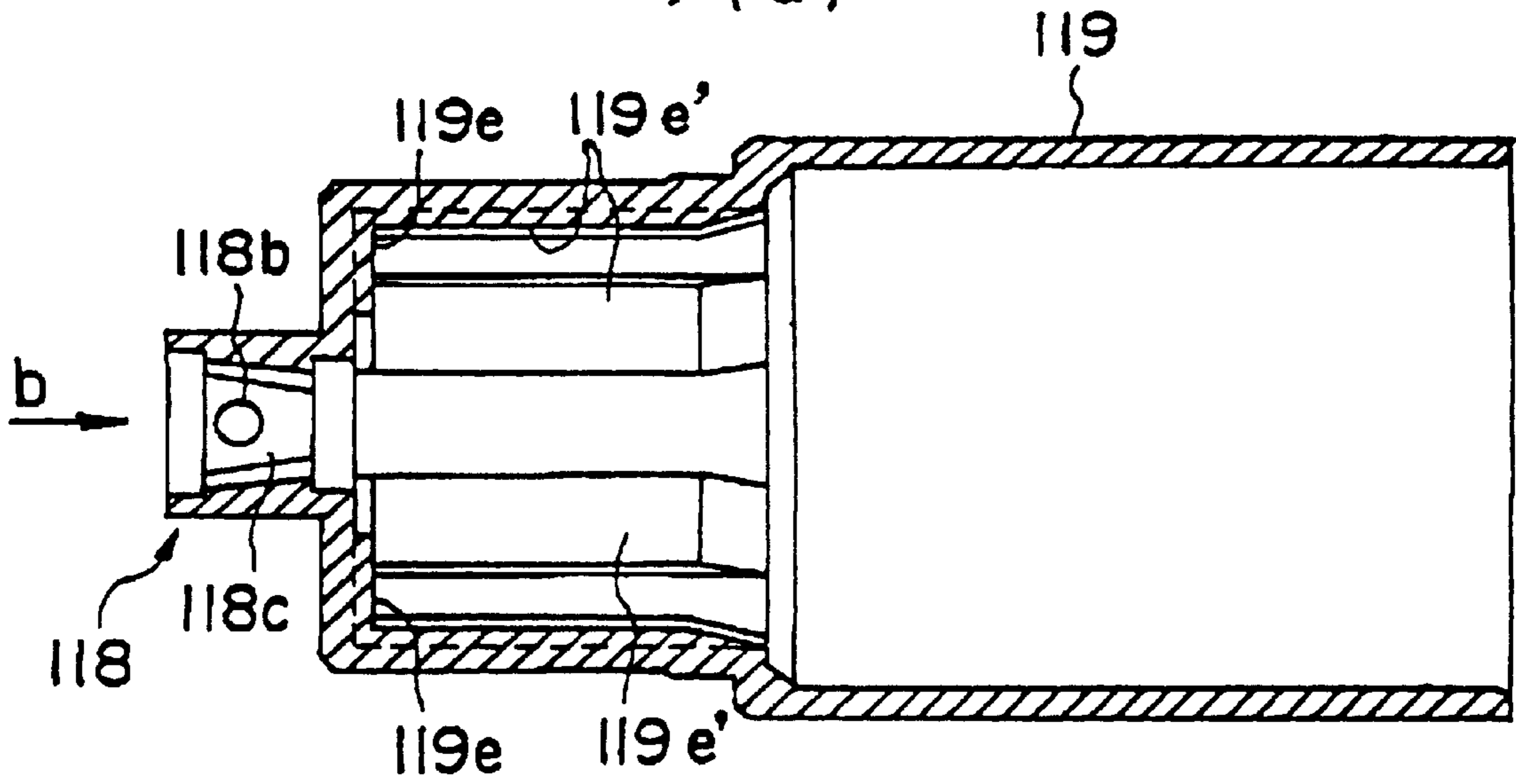
FIG. 9 (a)
