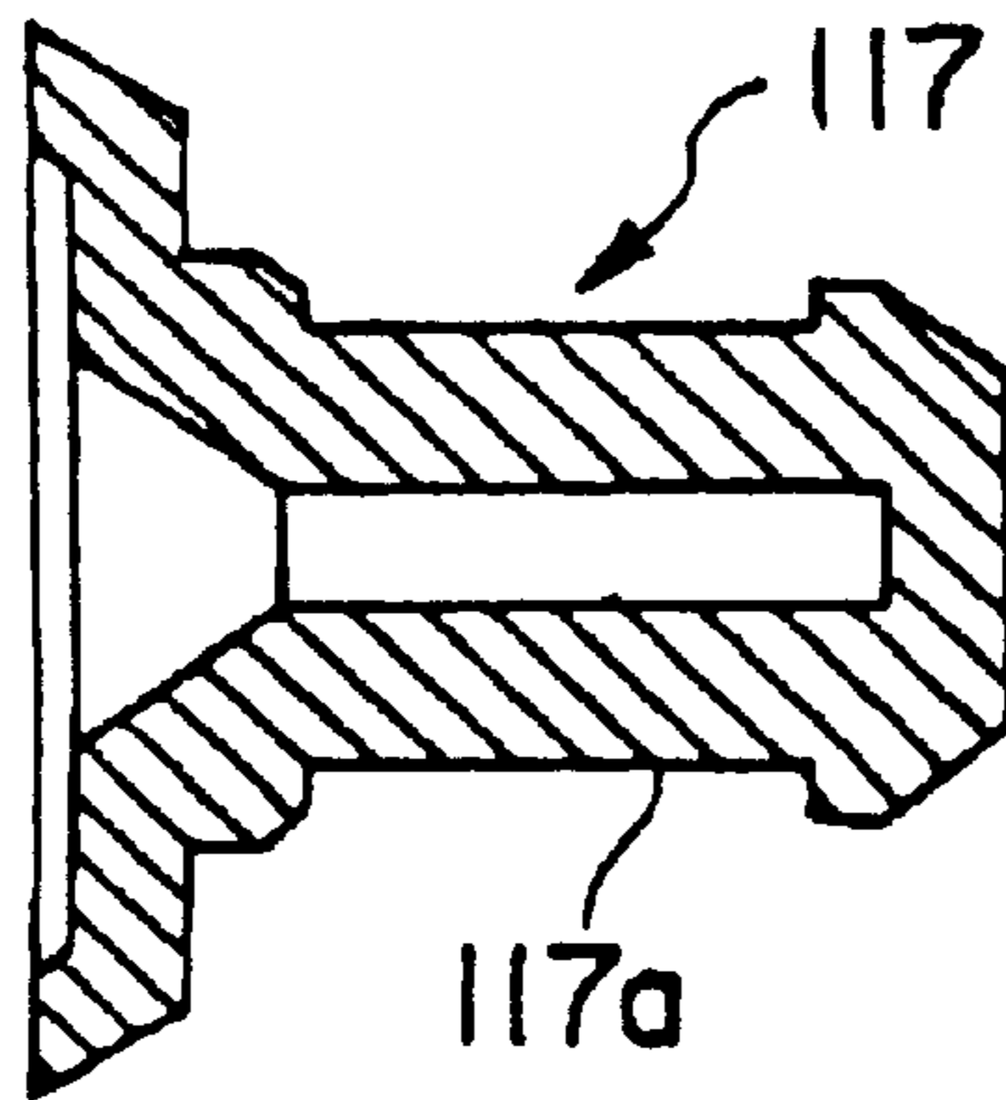
FIG. 10 (c)
