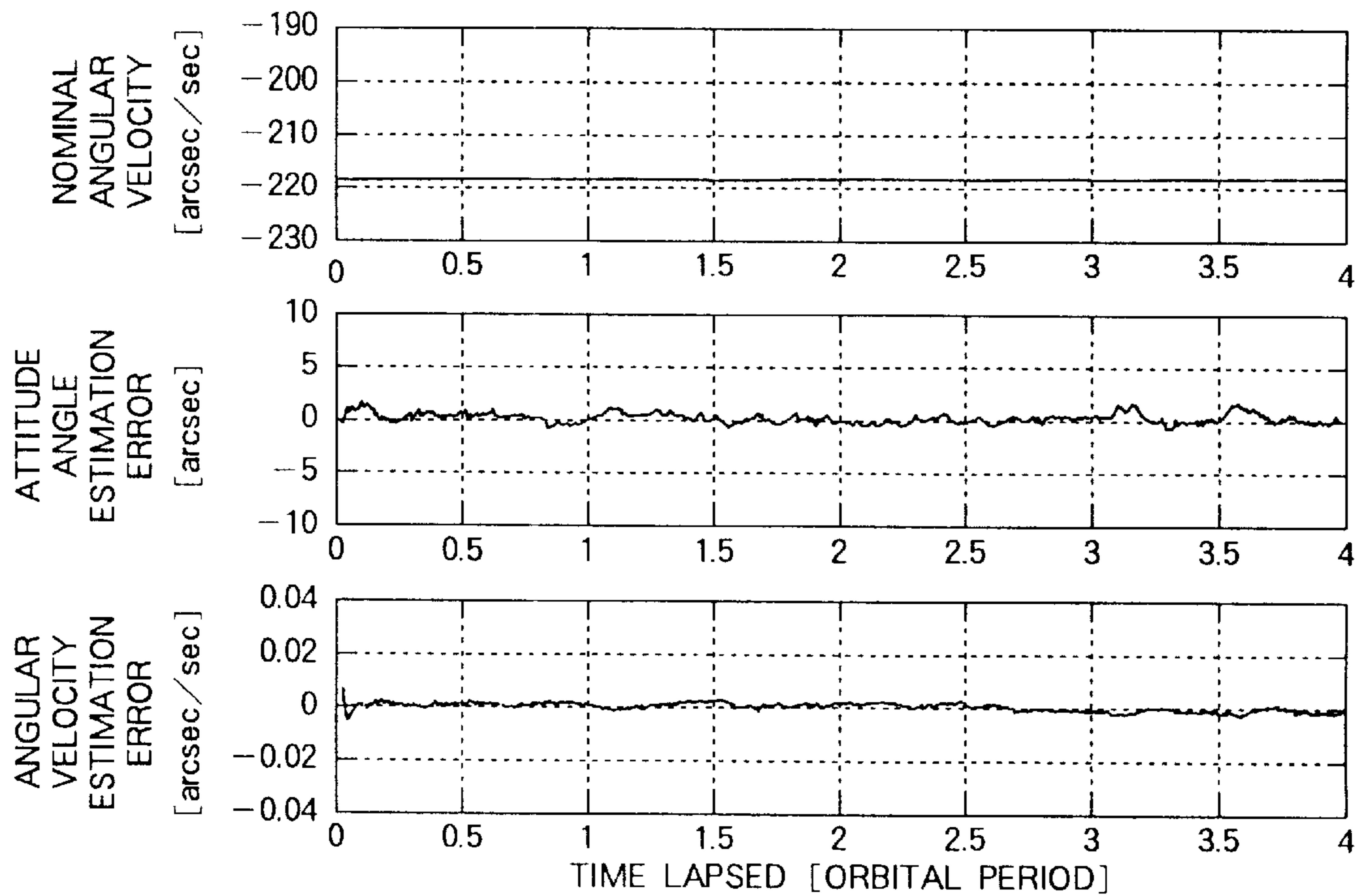
(a) CASE OF CONSTANT NOMINAL ANGULAR VELOCITY
