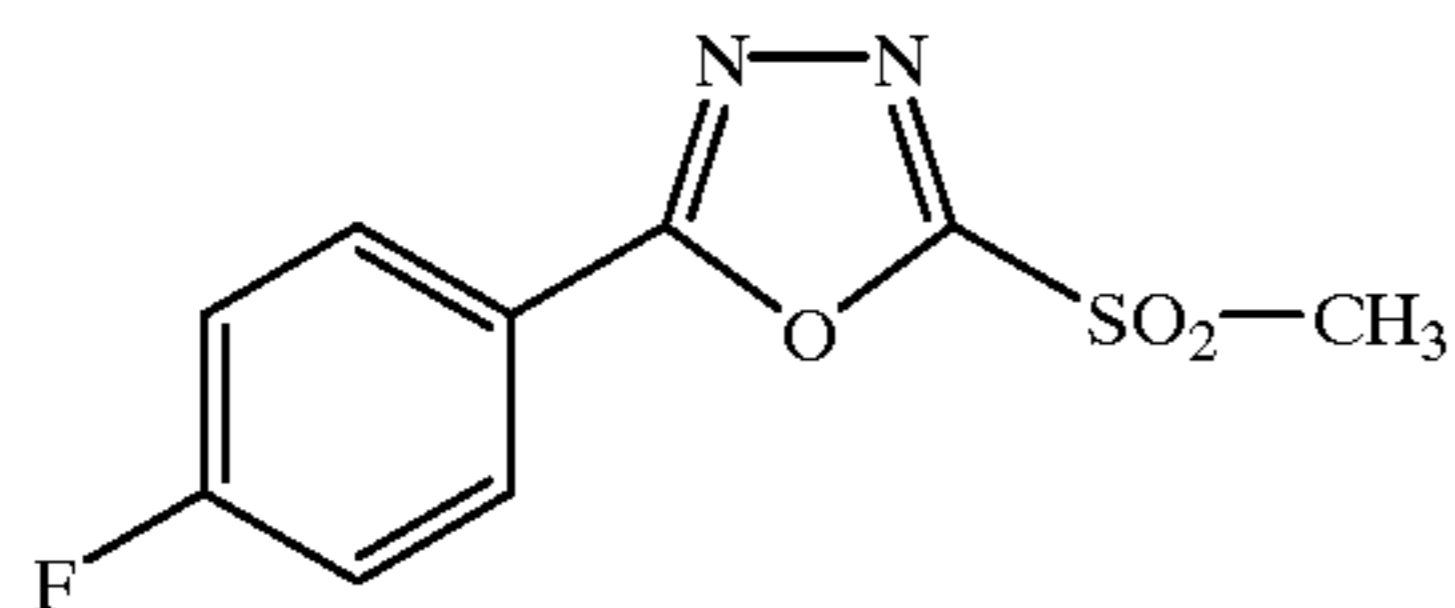
2-(4-Fluorophenyl)-5-methylsulphonyl-1,3,4-oxadiazole
