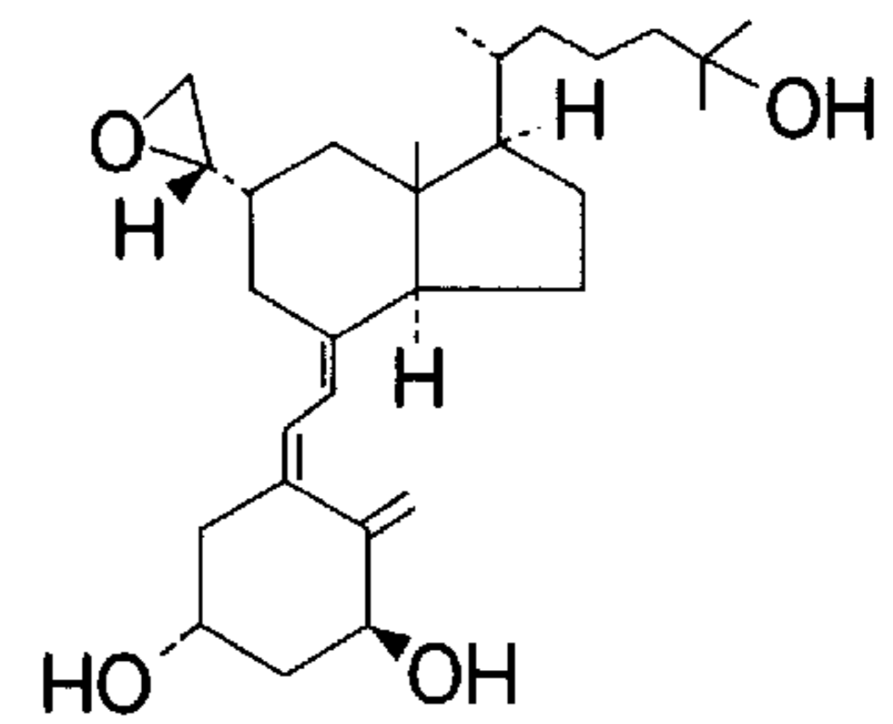
11 \alpha -[(11'(S)-oxacyclopropyl)]- 1 \alpha ,25-(OH) 2 -D 3
