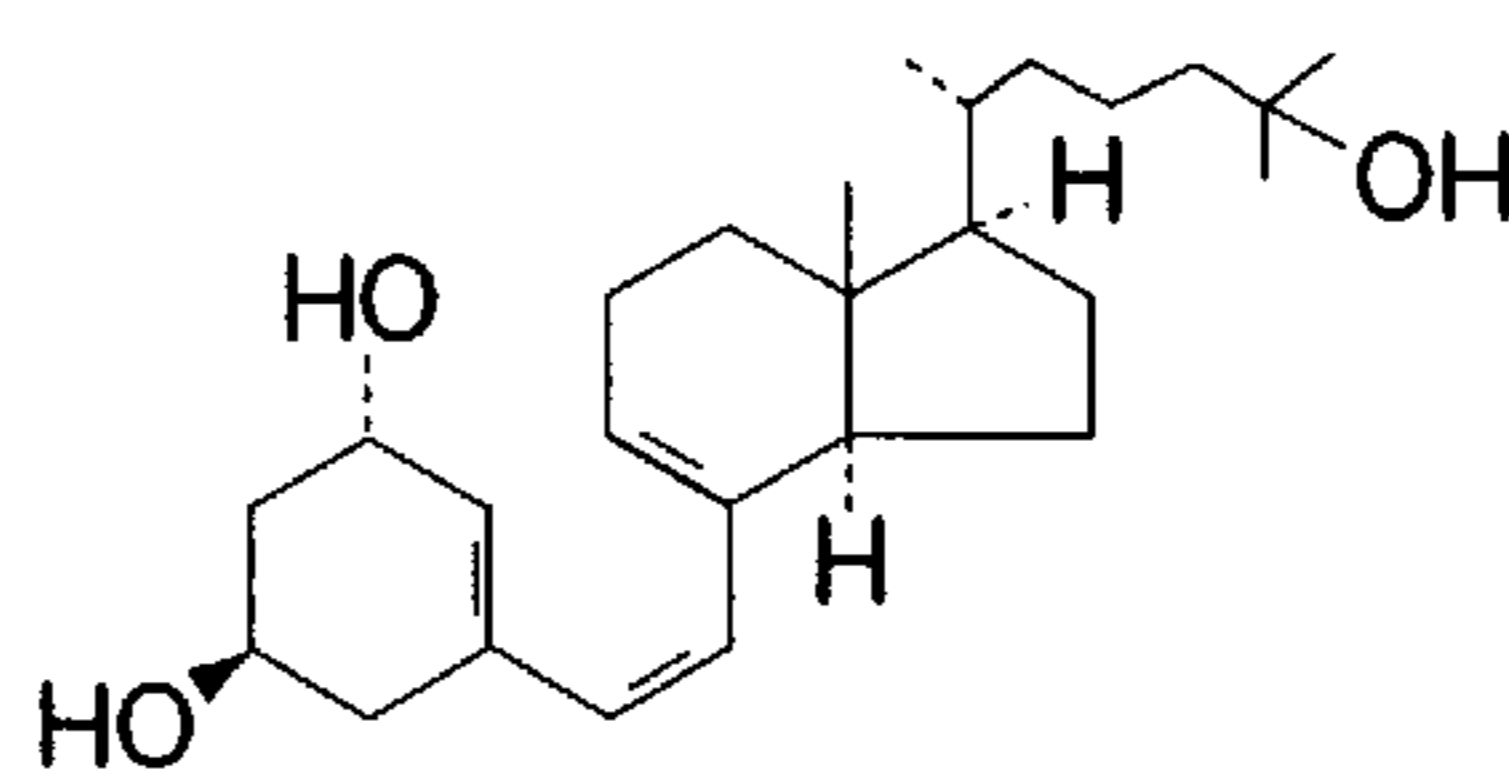
1 \alpha ,25-(OH) 2 - 19-nor-pre-D 3
