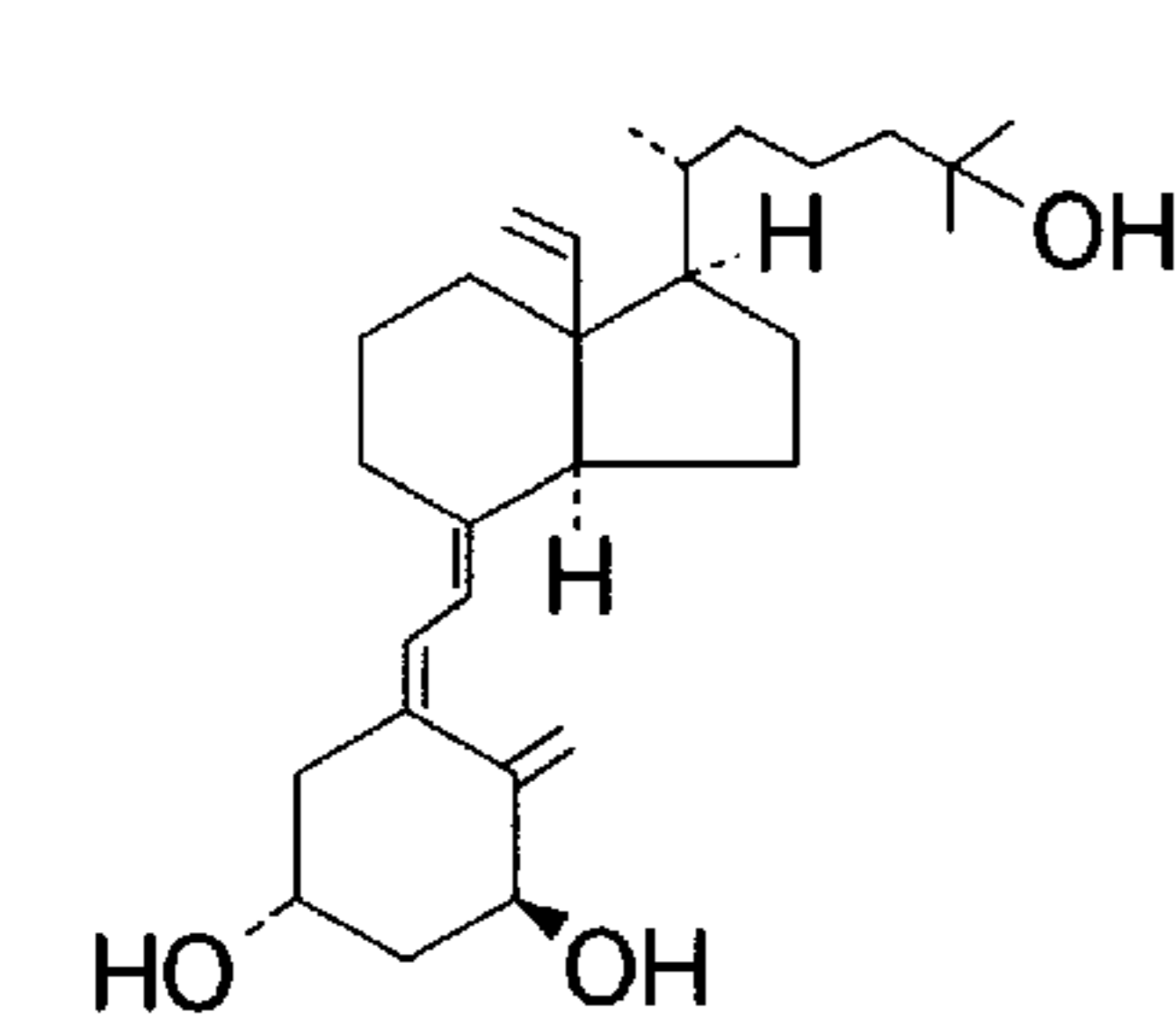
1 \alpha ,25-(OH) 2 - 13-vinyl-18-nor-D 3
