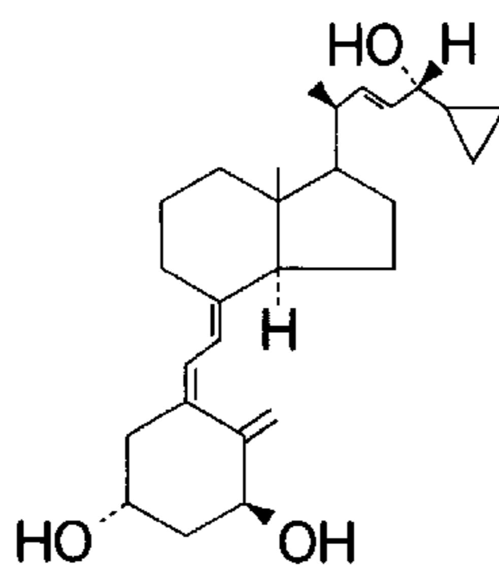
20-epi-22-ene- 26,27-dehydro- 1 \alpha ,24S-(OH) 2 -D 3
