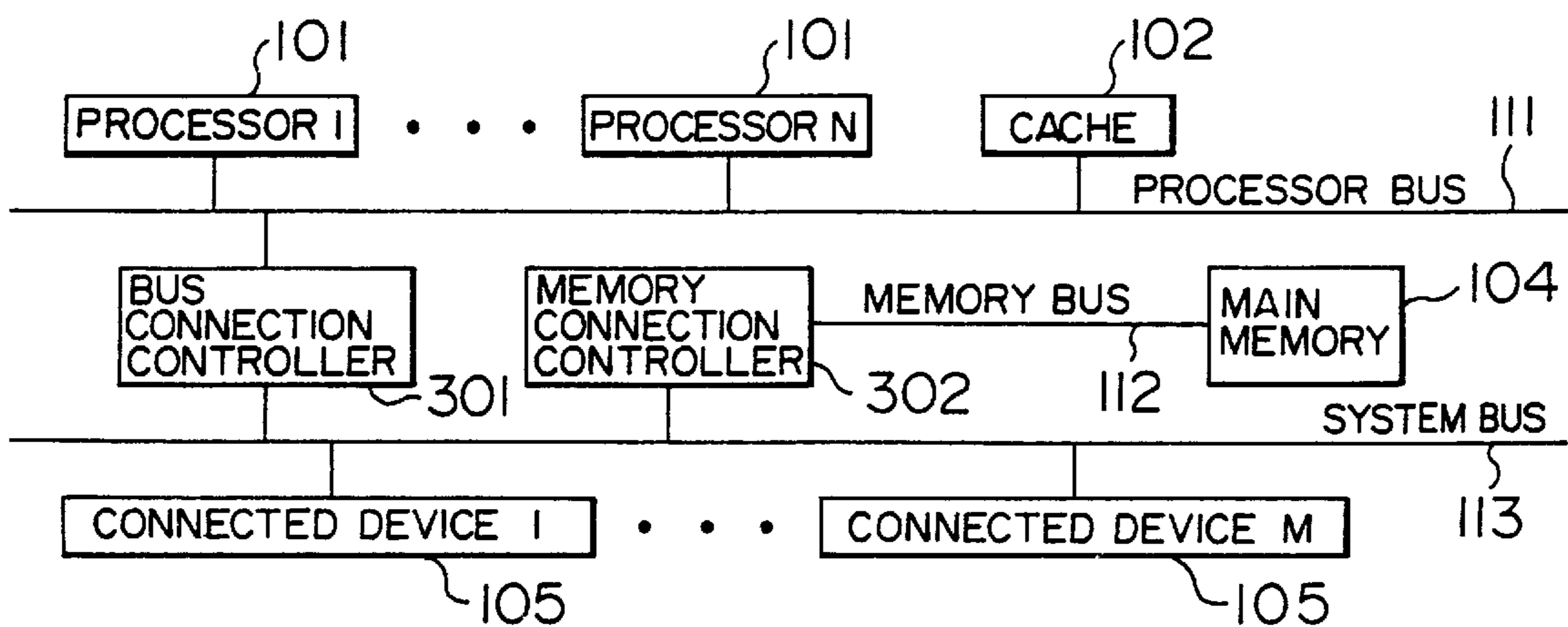
FIG. 3 PRIOR ART
