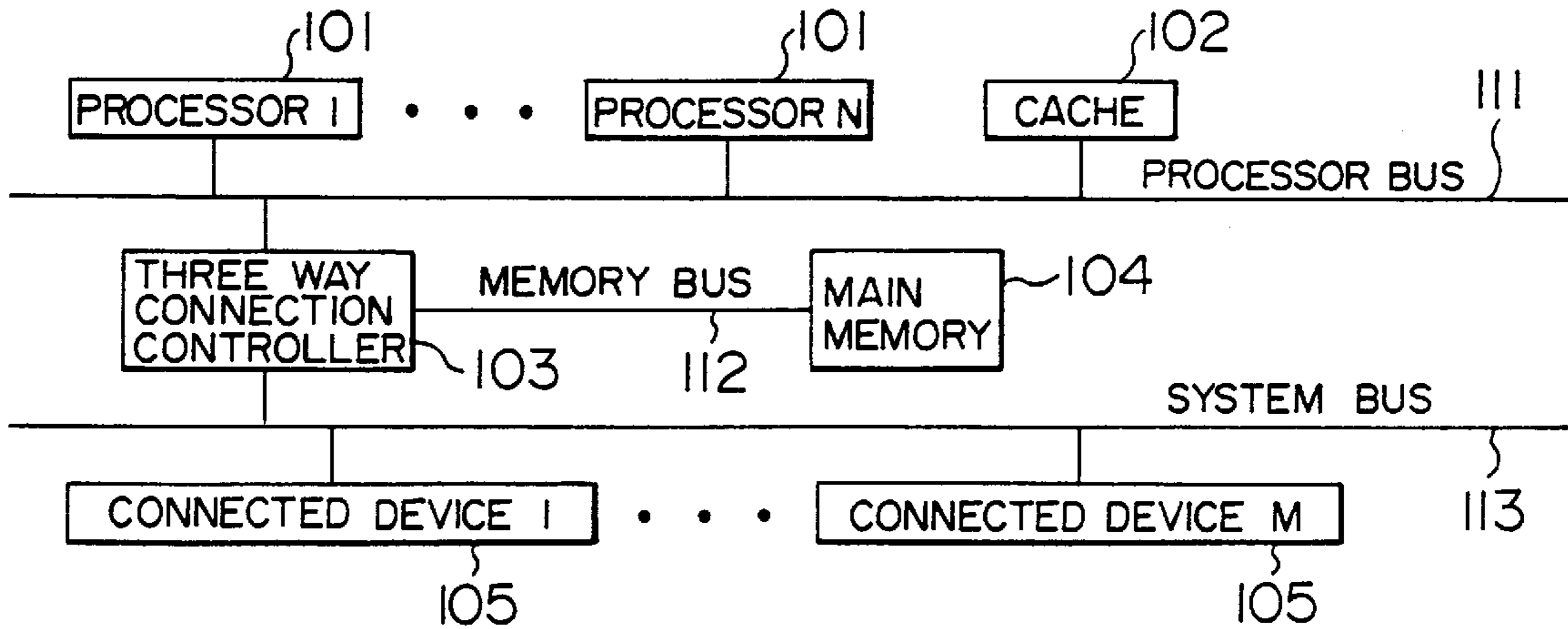
FIG. 2 PRIOR ART
