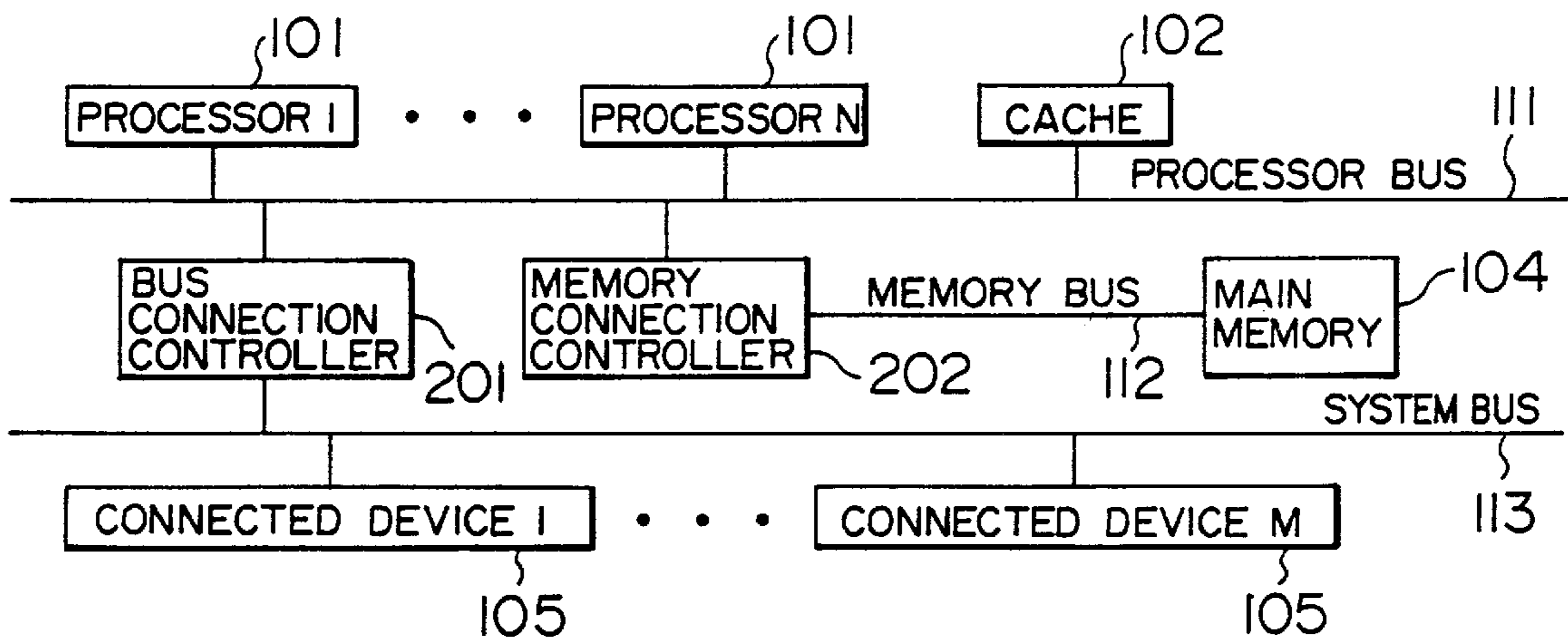
FIG. 3 PRIOR ART
