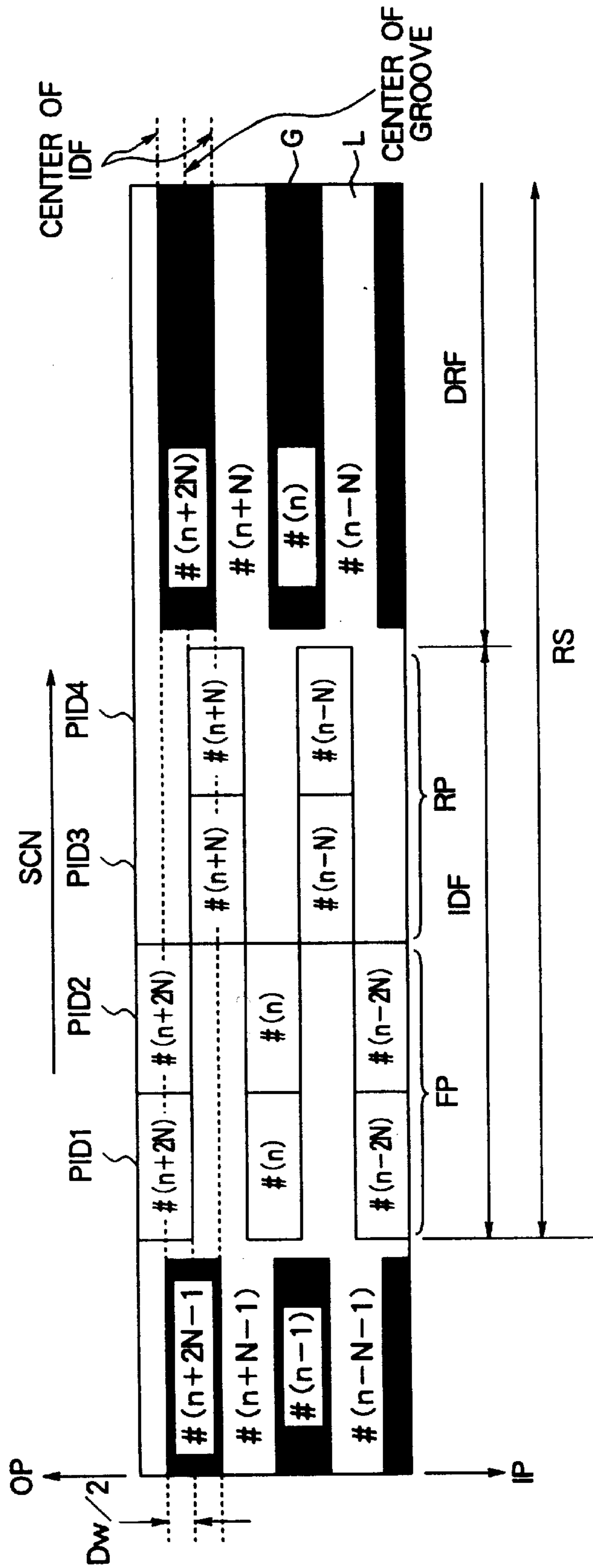
FIG. 13 PRIOR ART
