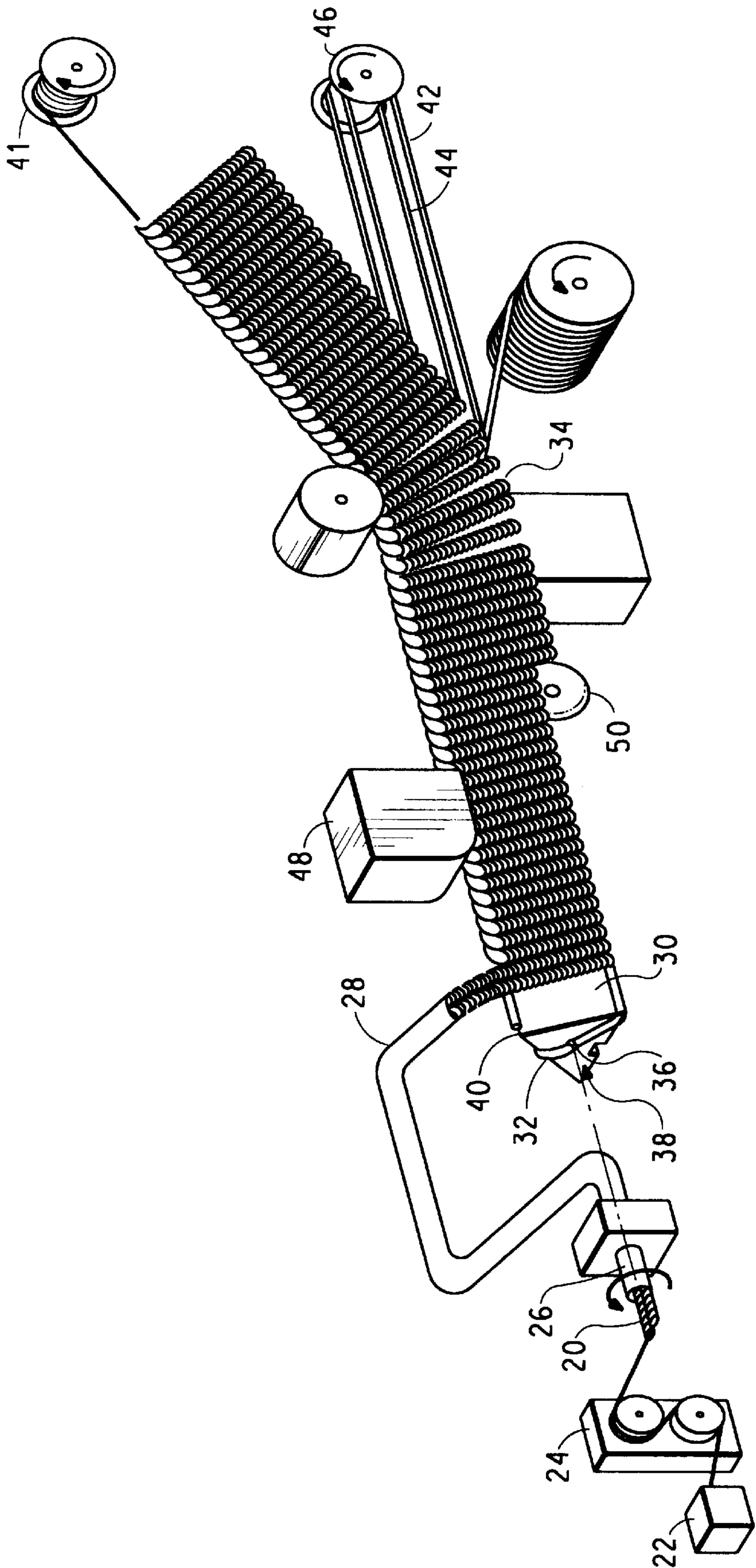
FIG. 1 (PRIOR ART)
