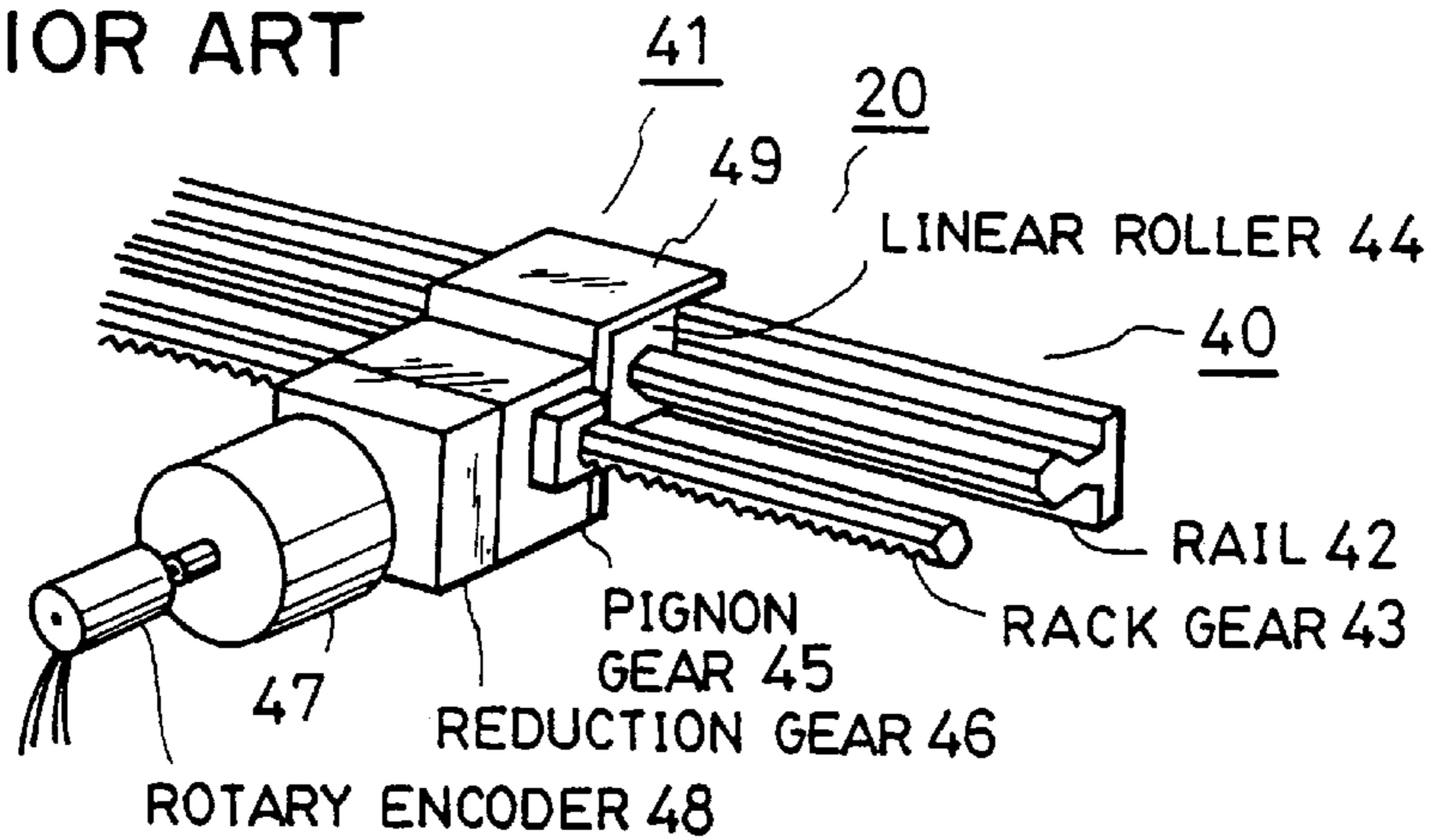
FIG. 20 PRIOR ART
