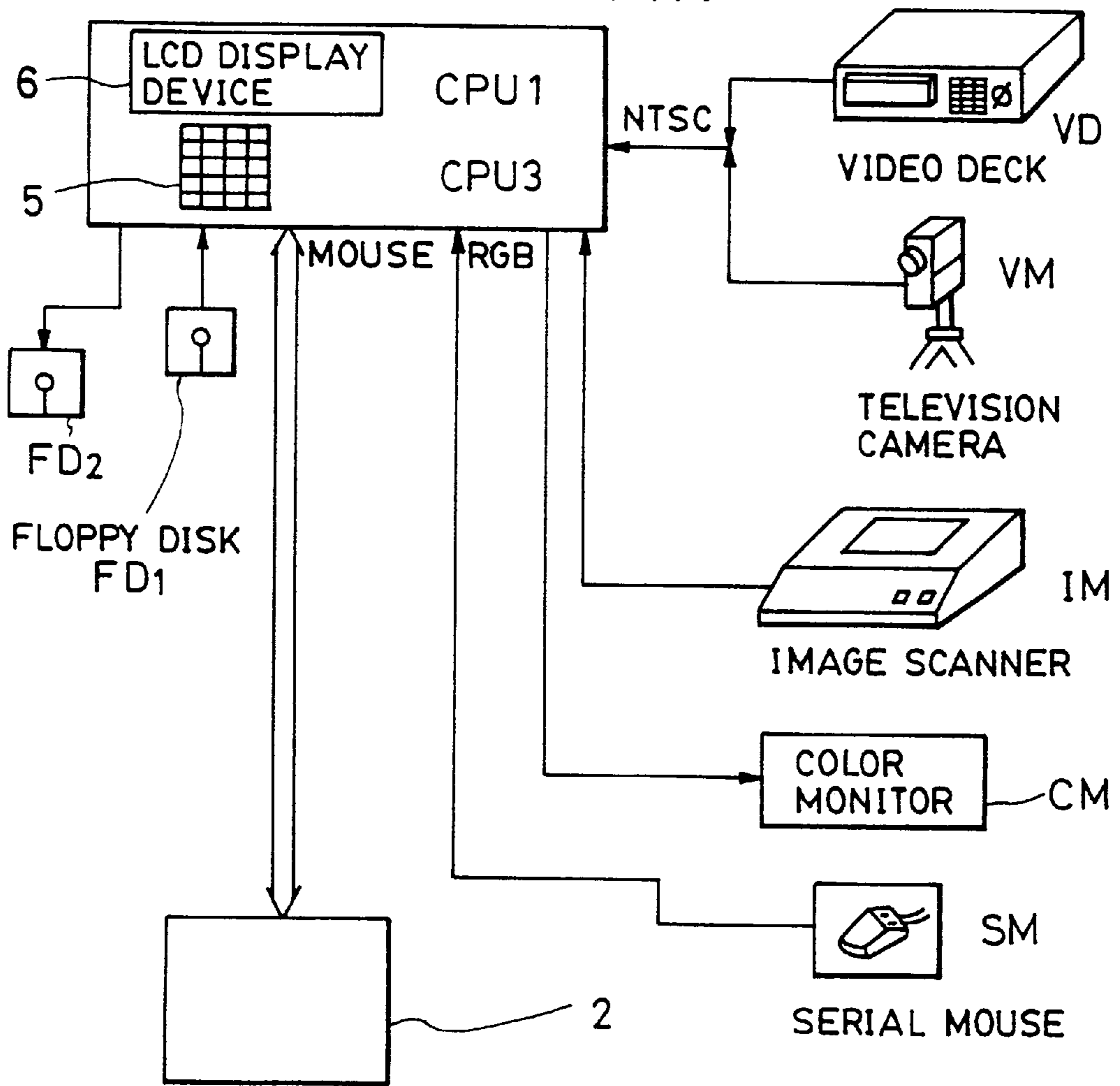
FIG. 14 PRIOR ART
