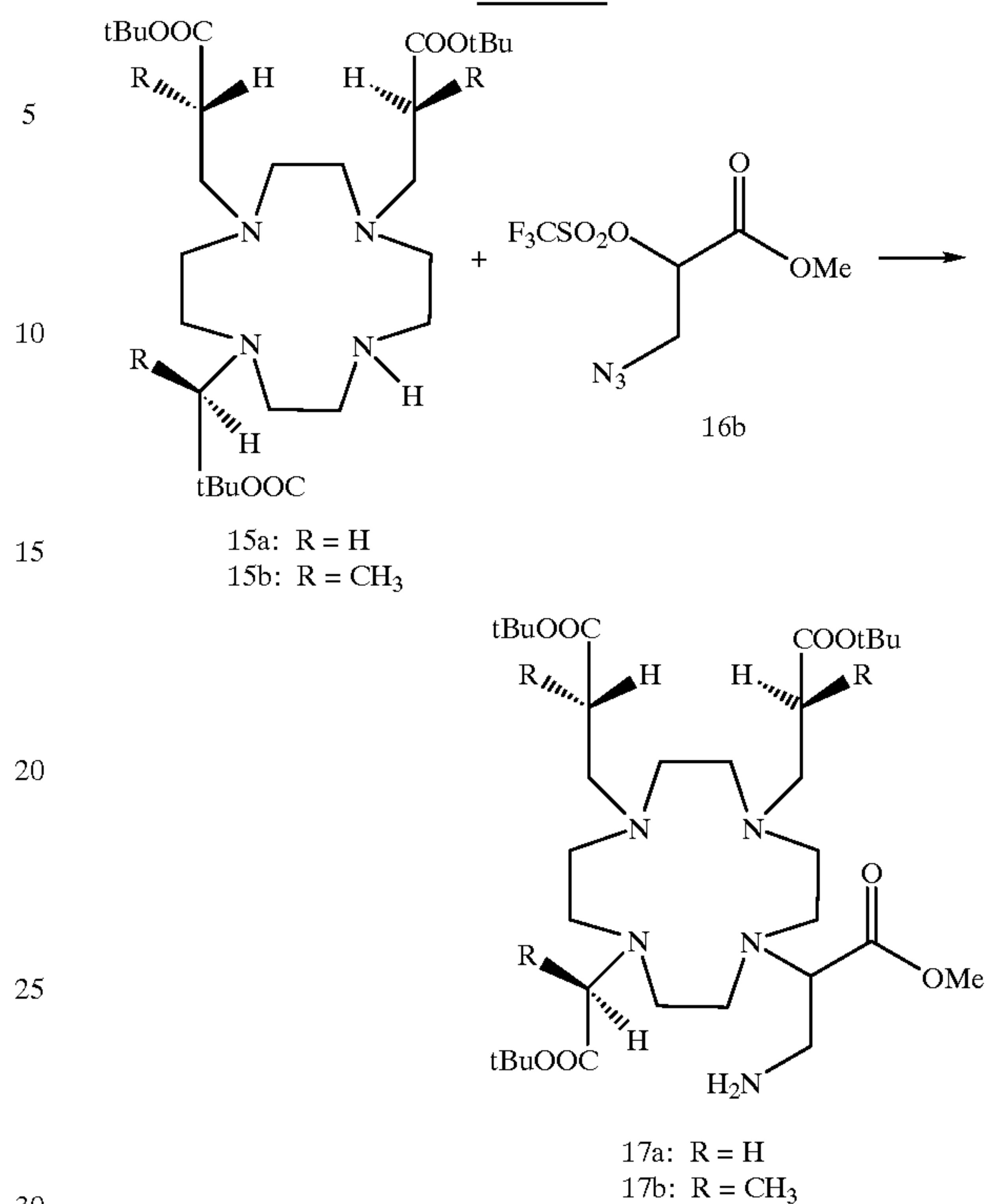
Scheme 4
