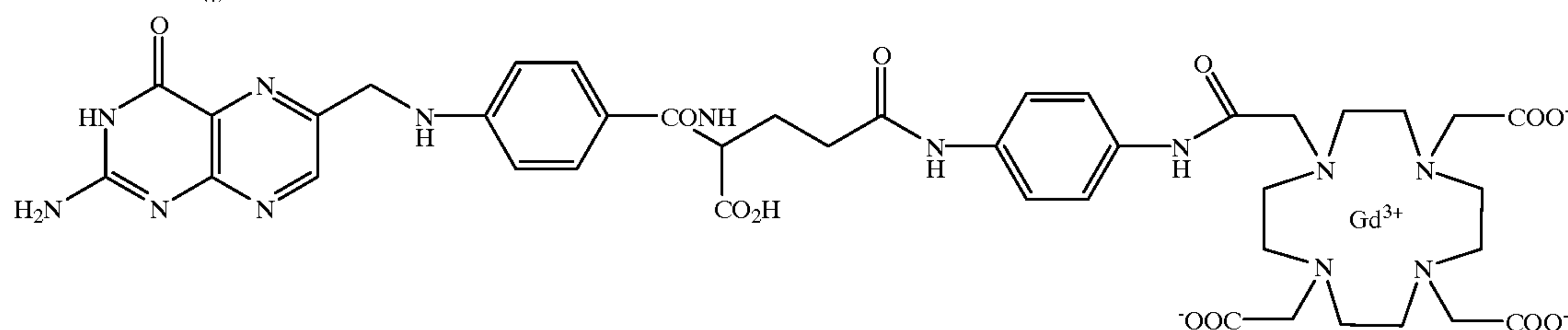
Gd-DO3A-APA-( \gamma )-folate
