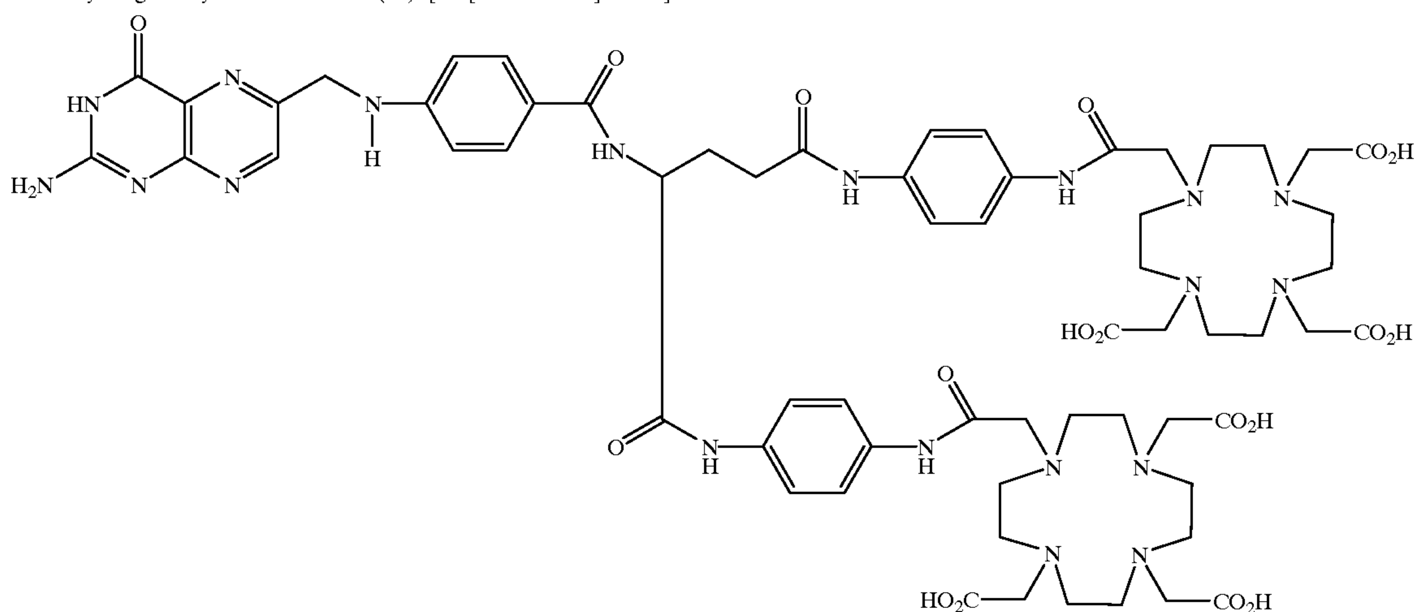
N-Pteroyl-L-glutamyl-bis APADO3A (14) [Bis[DO3A-APA]-folate]
