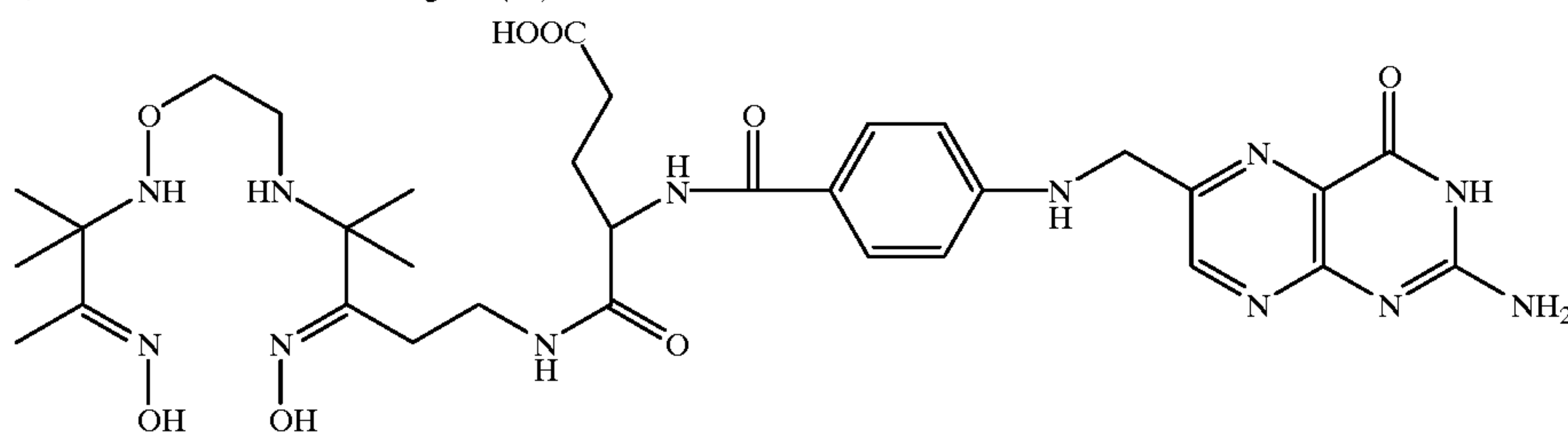
12-N-(N-Pteroyl- \alpha -L-glutamyl)-3,3,9,9-tetramethyl-5-oxa-4,8-diaza-2,10-dodecanedione dioxime ligand (62)
