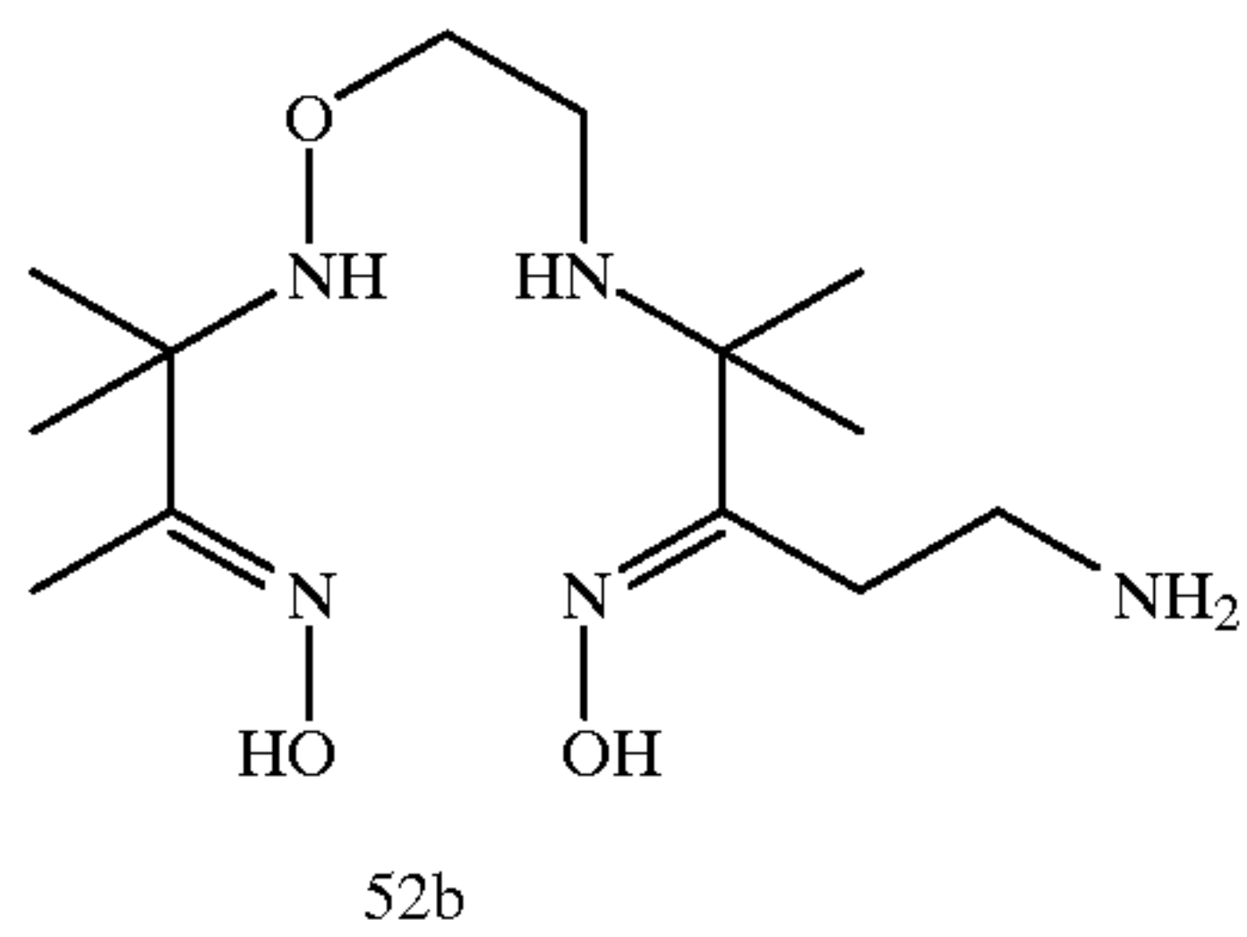
Scheme 18
