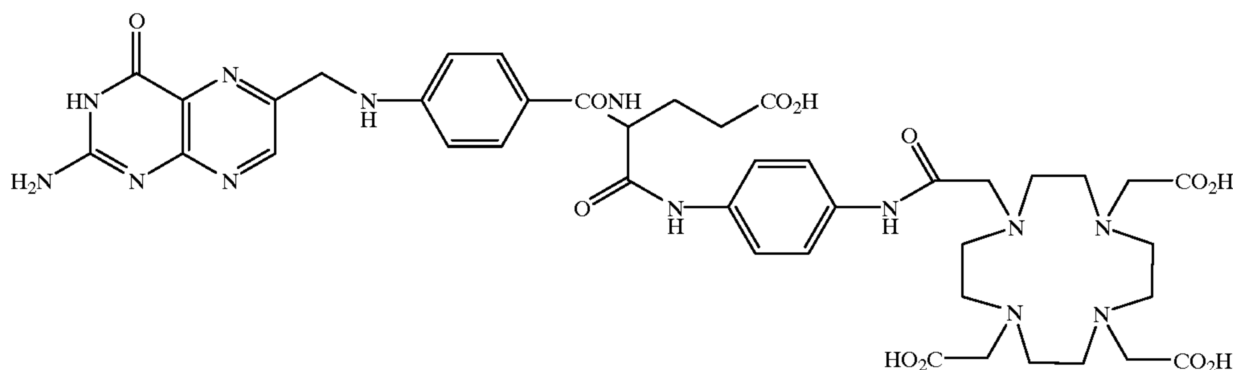
N-Pteroyl-α-L-glutamyl-APADO3A (10) [DO3A-APA-(γ)-folate
