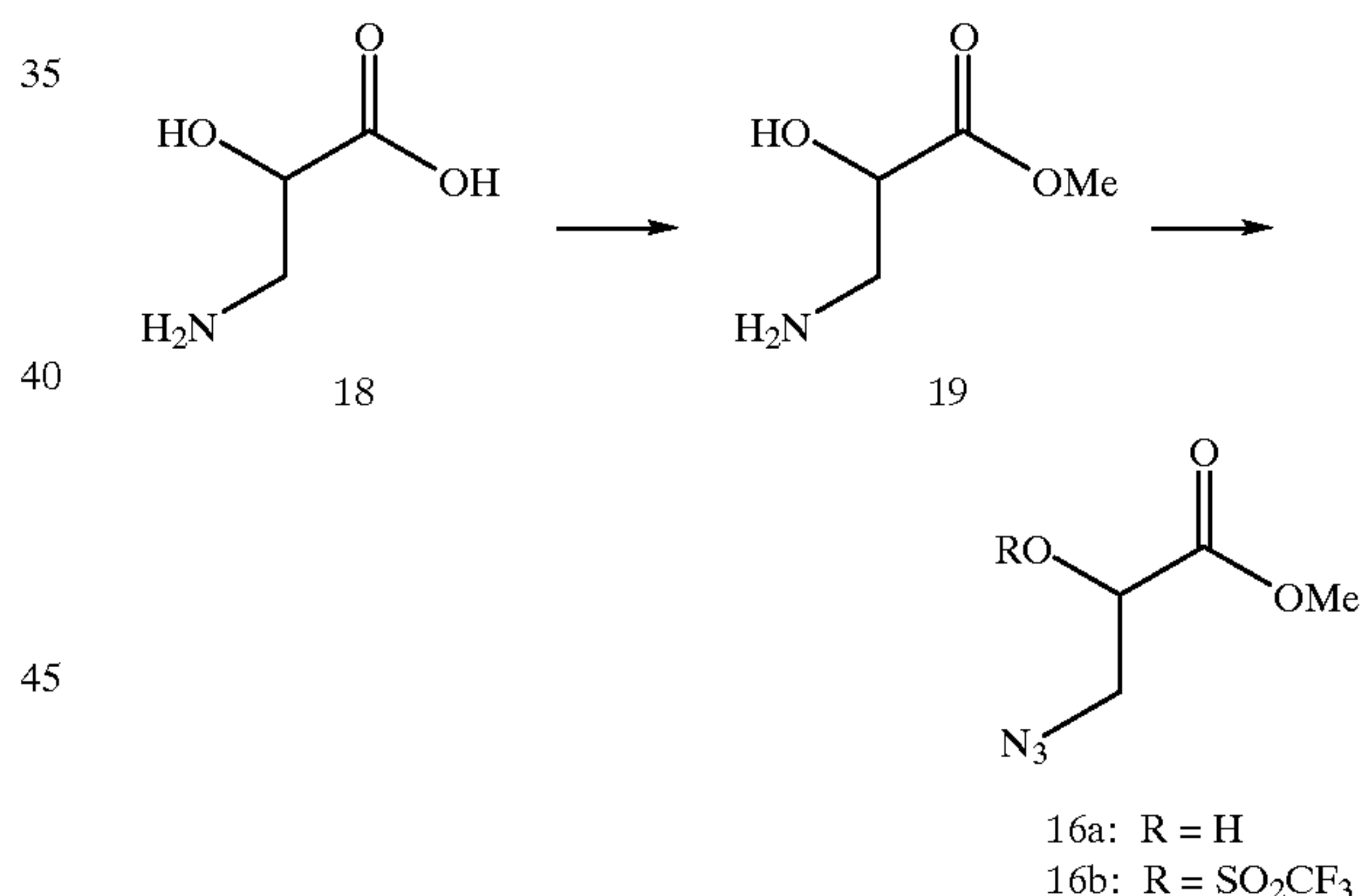
Scheme 5
