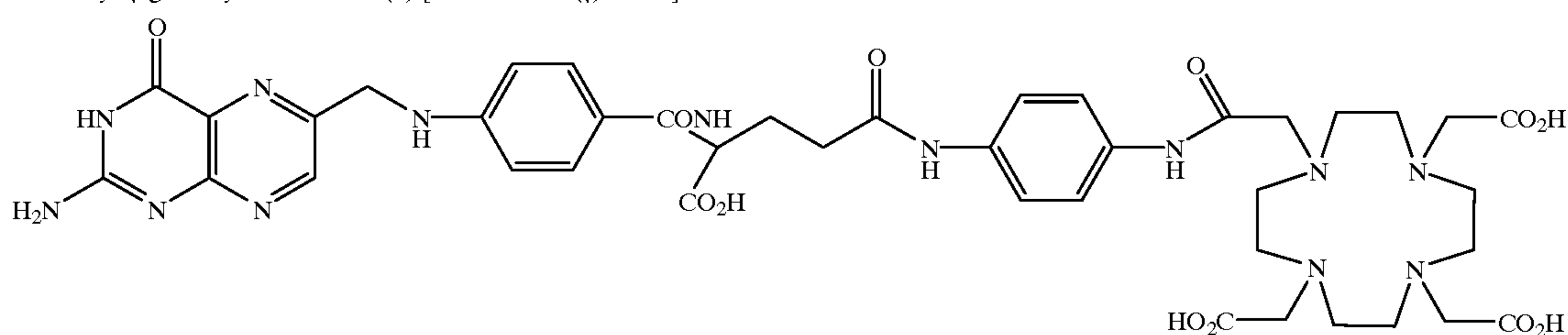
N-Pteroyl- \gamma -glutamyl-APADO3A (6) [DO3A-APA-( \gamma )-folate]
