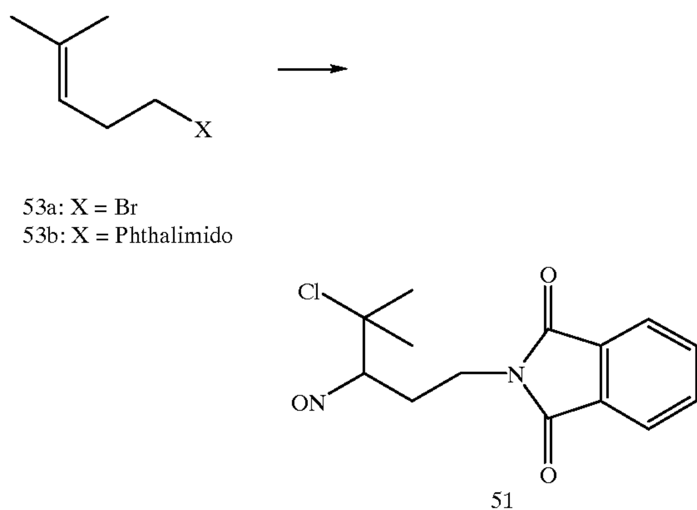
Scheme 15
