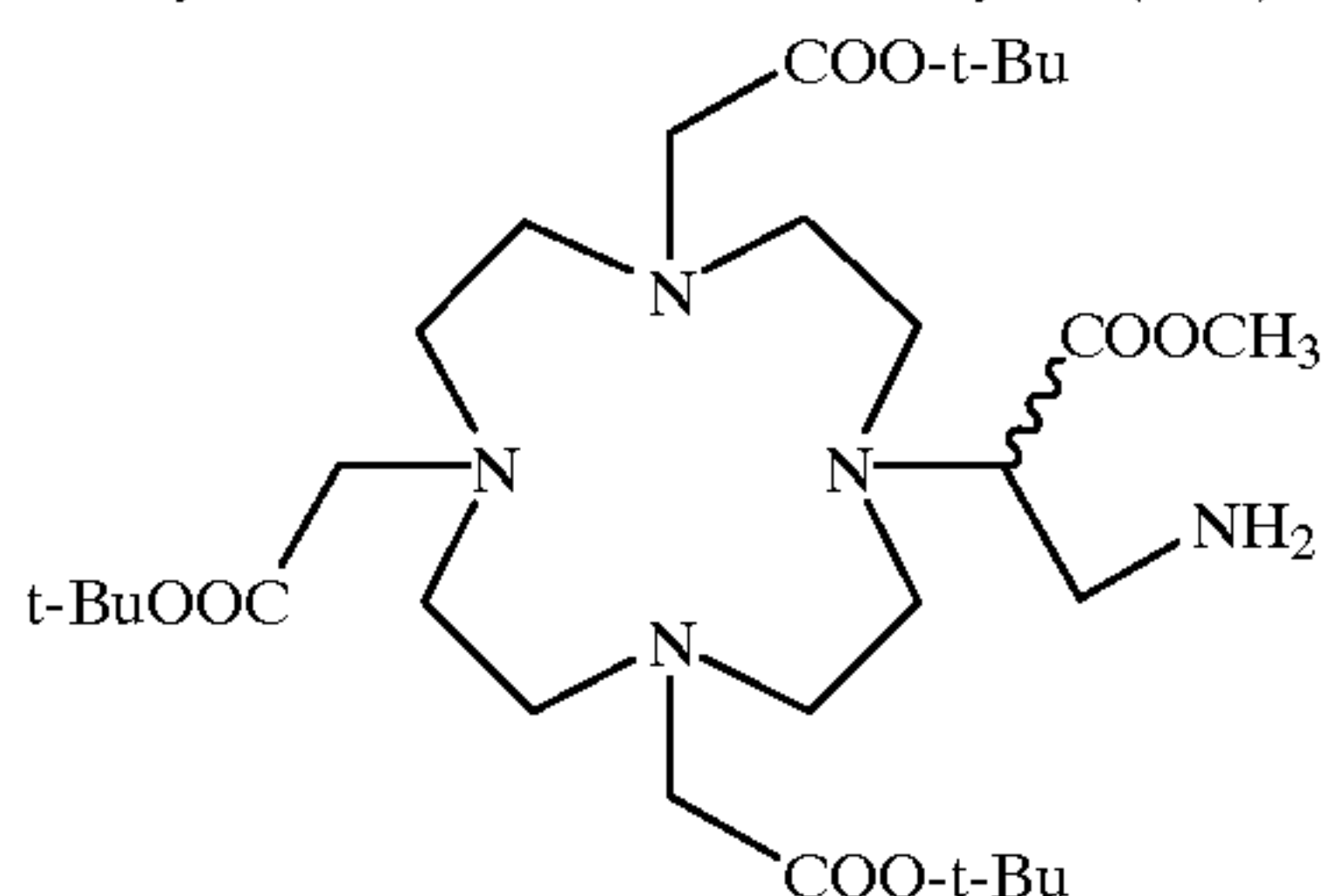
Tris-t-butyl N-12-(3-amino-2-methoxycarbonyl-1-ethyl)-1,4,7,10-tetracyclododecane-1,4,7-tricarboxylate (17A)
