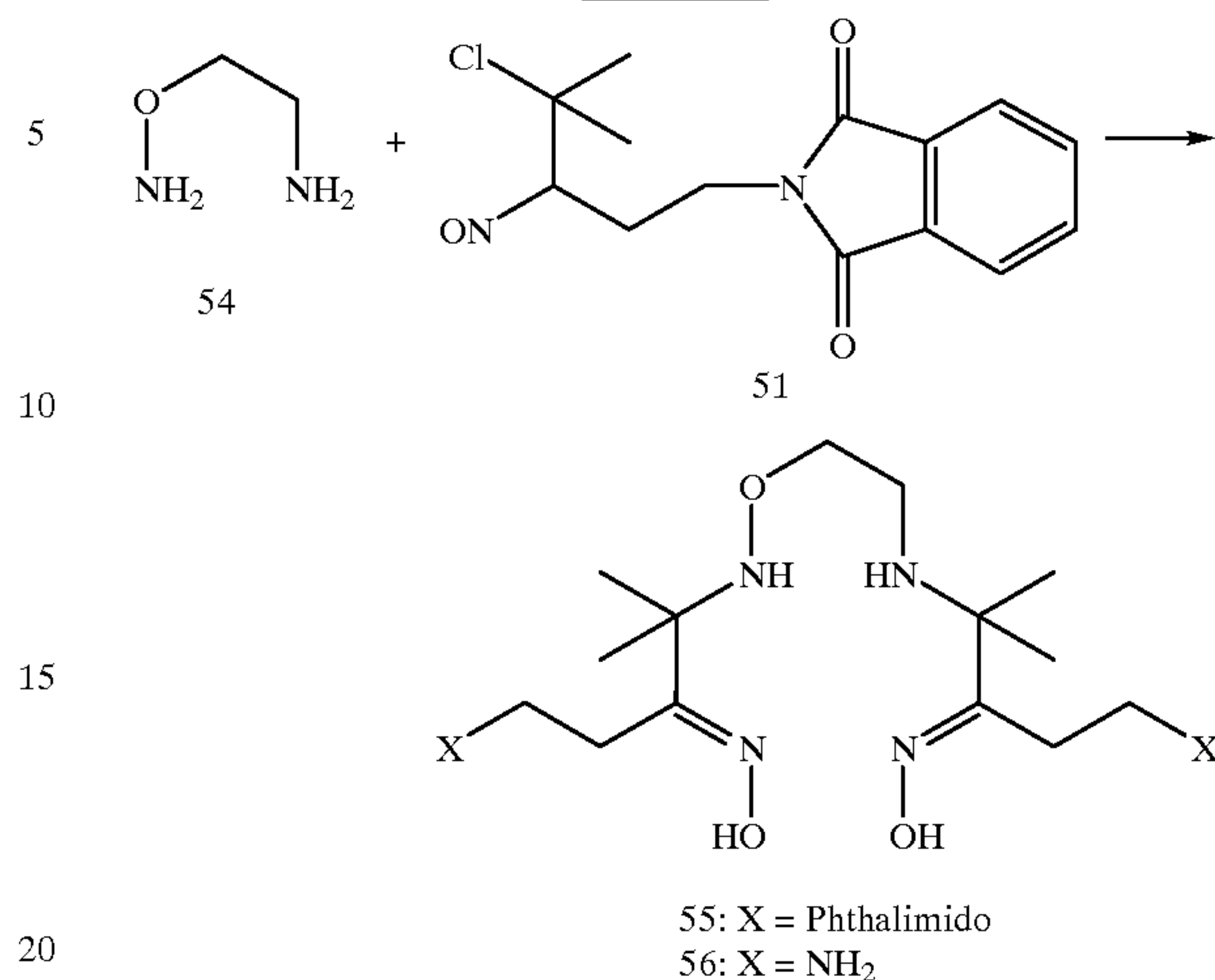
Scheme 16
