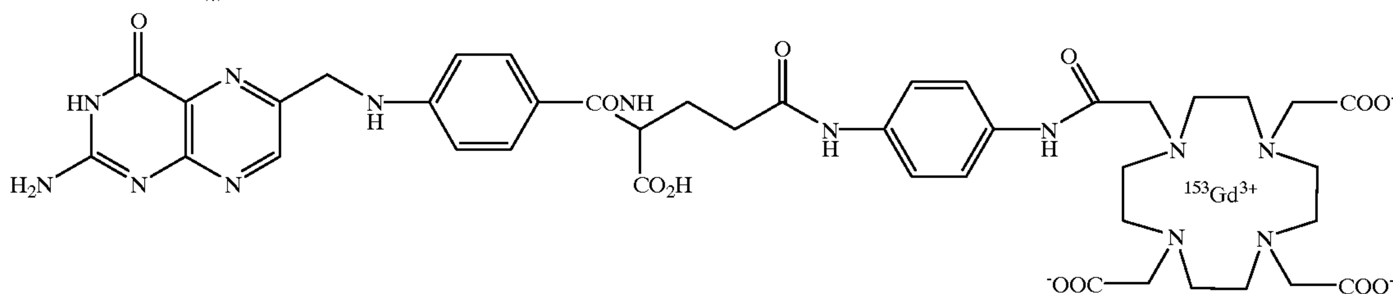
153 Gd-DO3A-APA-(γ)-folate
