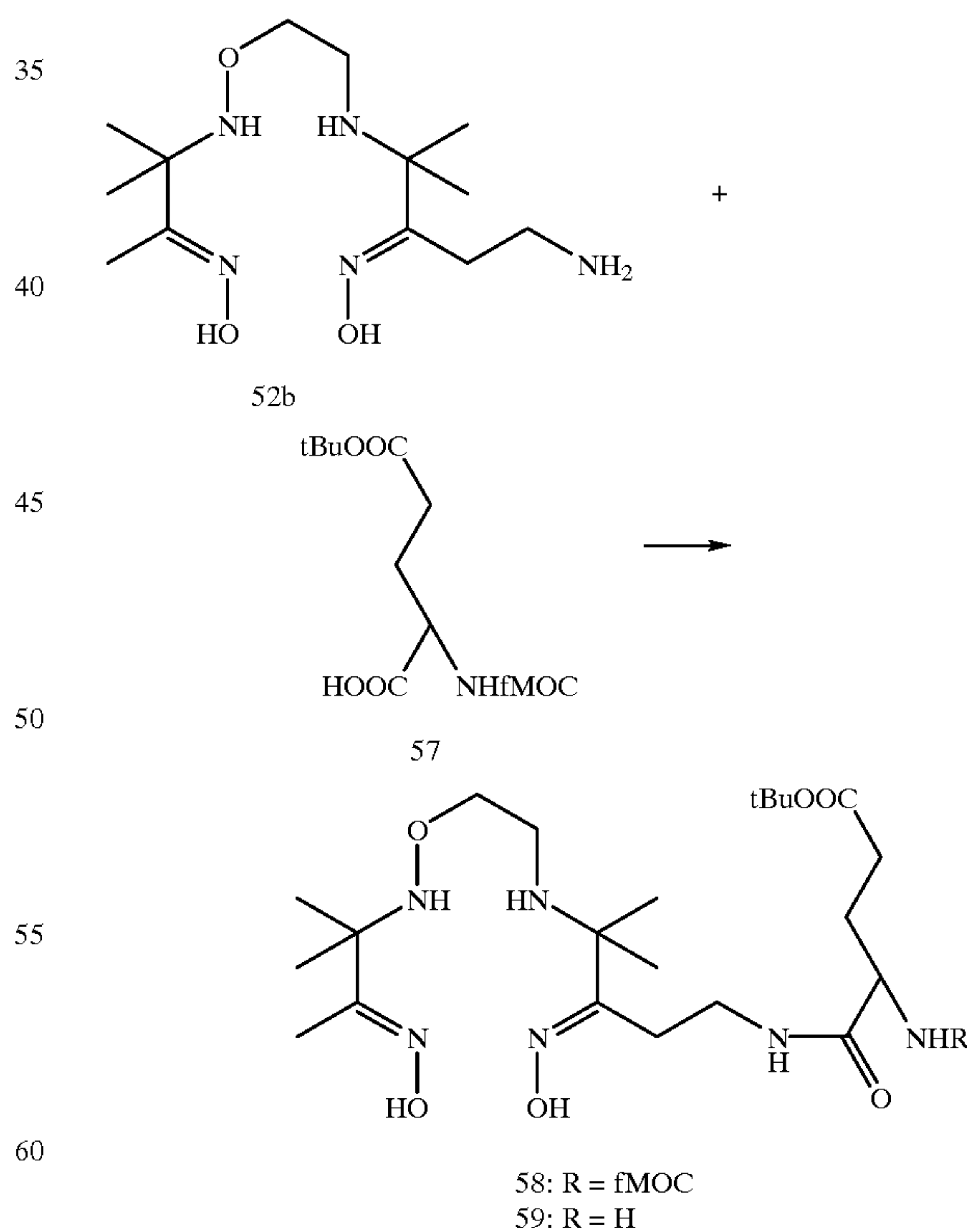
Scheme 17
