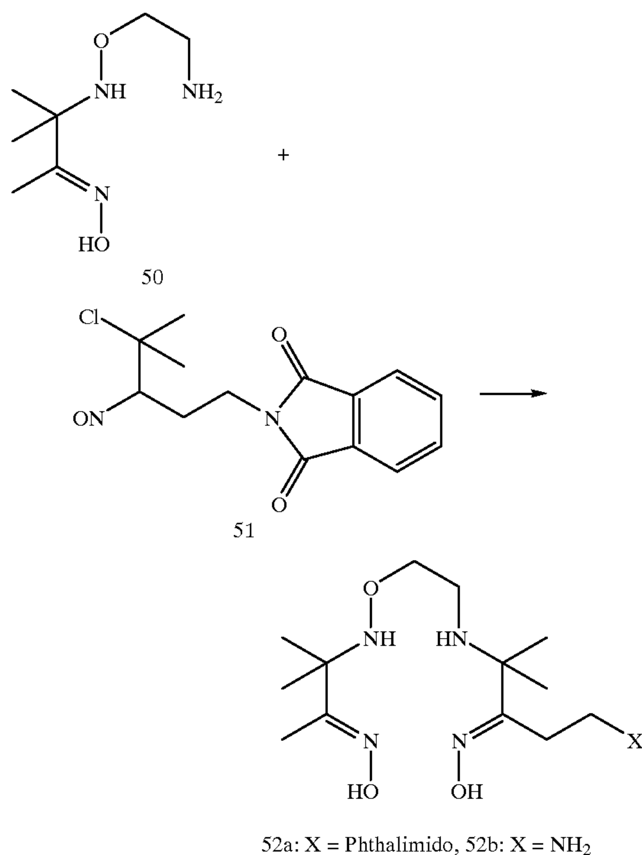
Scheme 14
