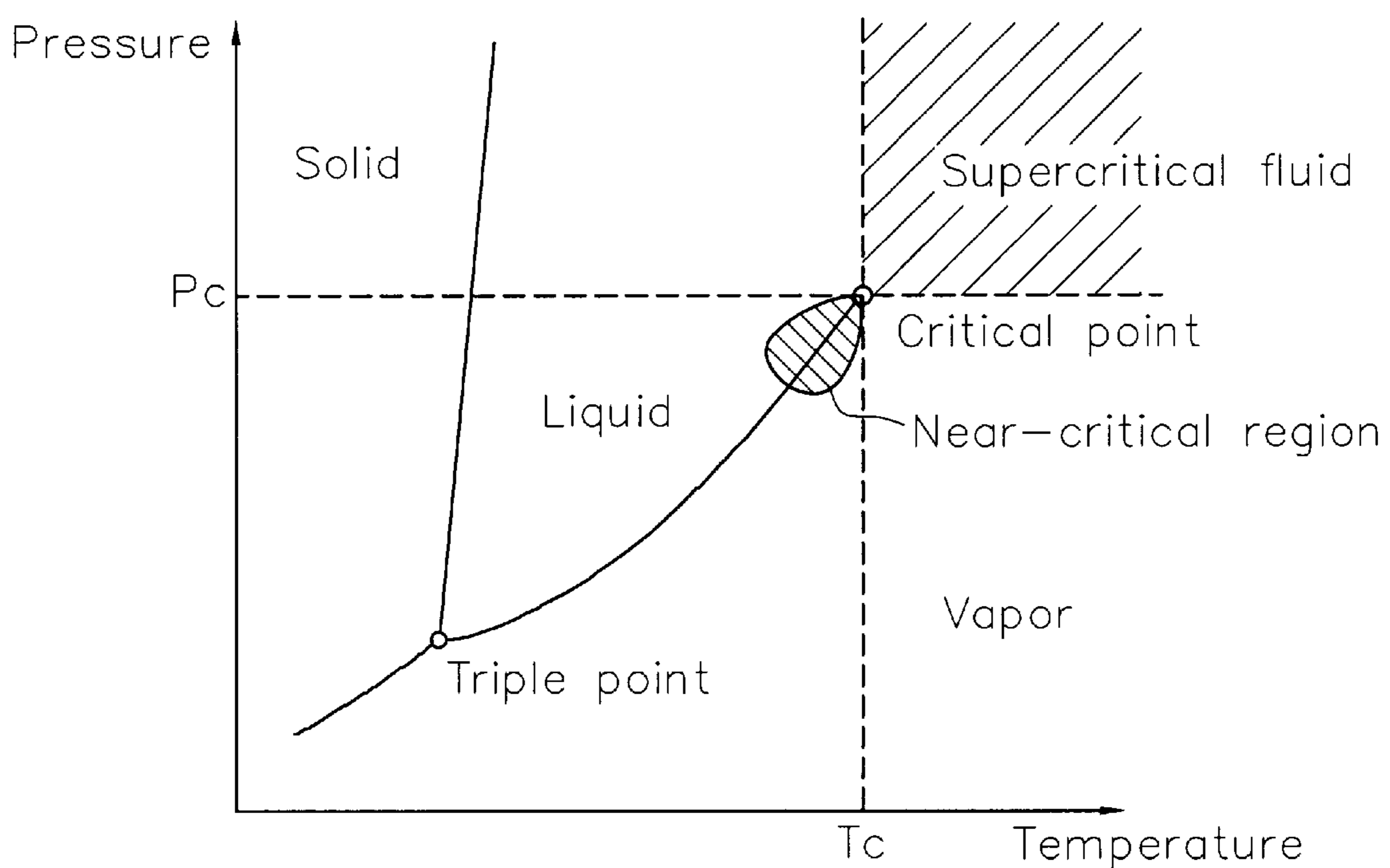
State diagram for a pure component showing supercritical fluid & near-critical fluid regions.
