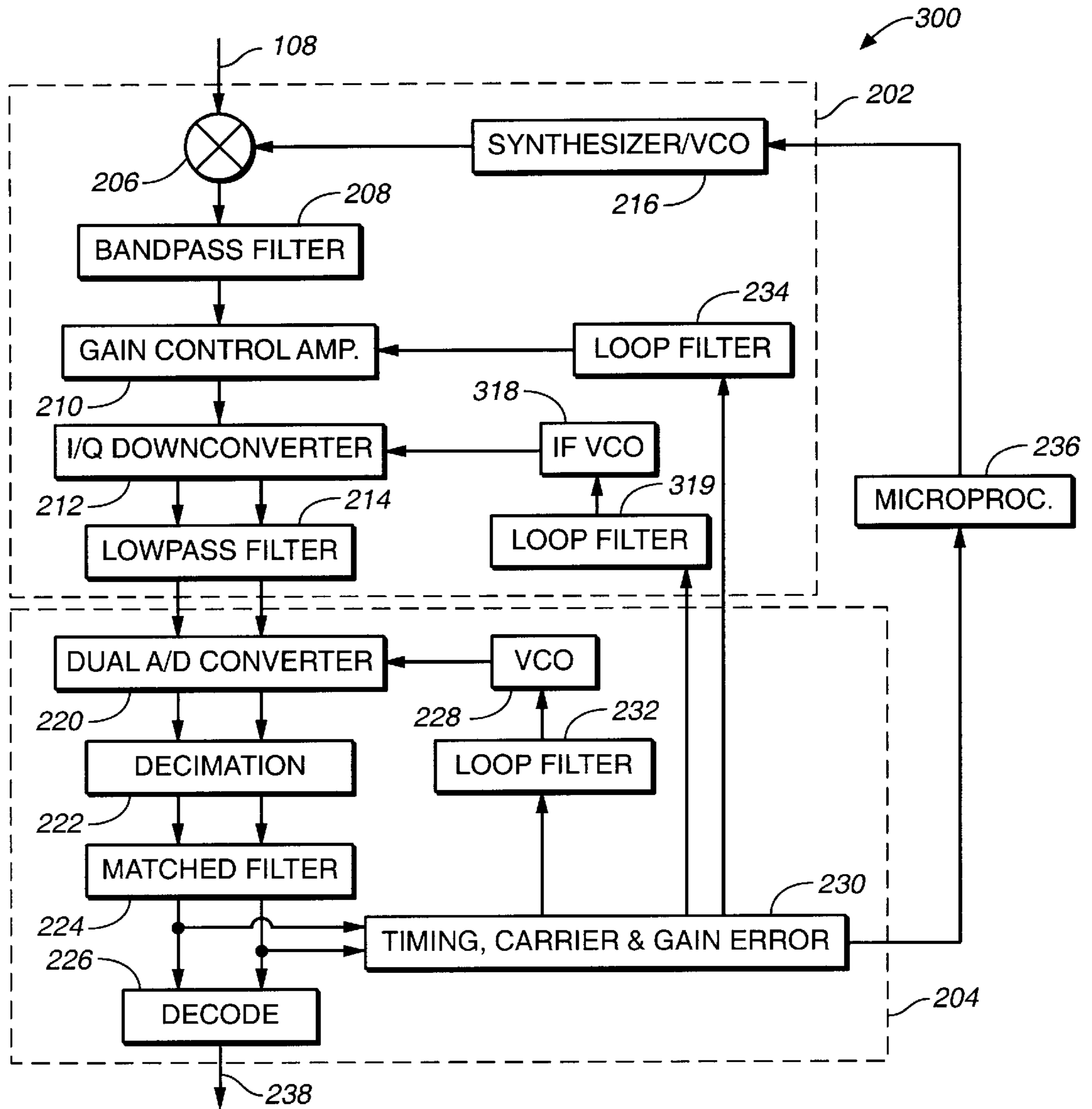
FIG. 3 (PRIOR ART)
