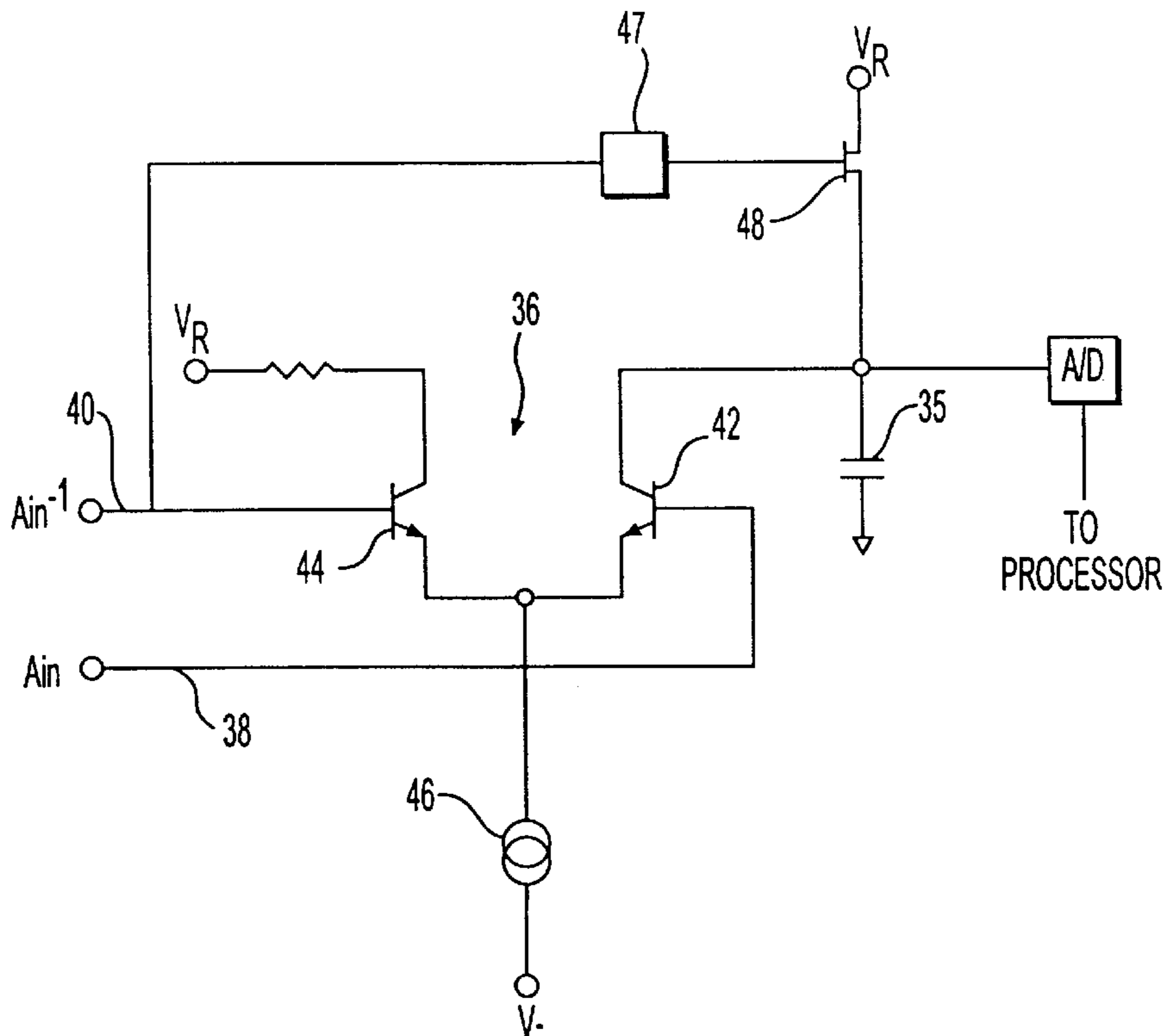
FIG. 3 PRIOR ART
