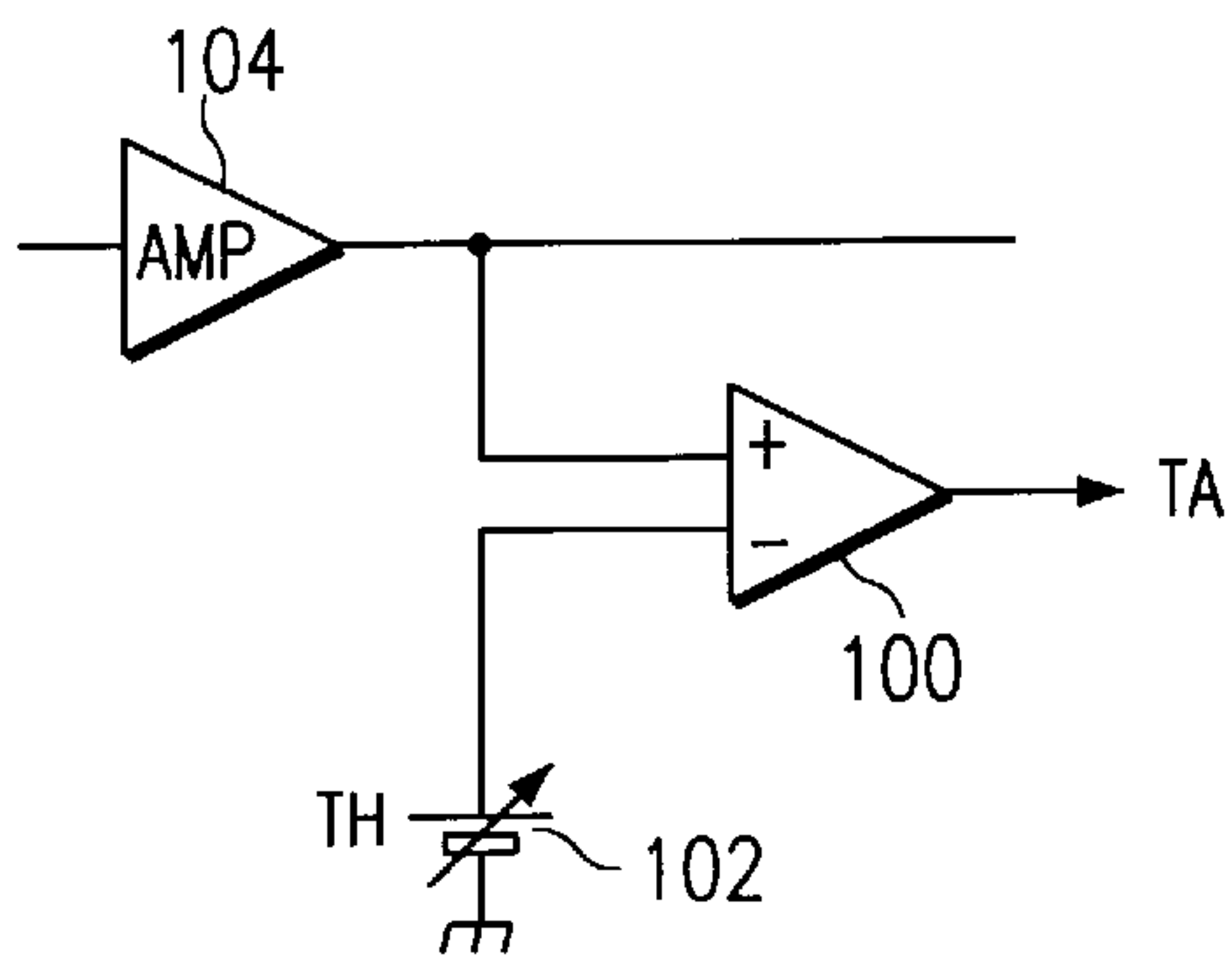
FIG. 4 (PRIOR ART)
