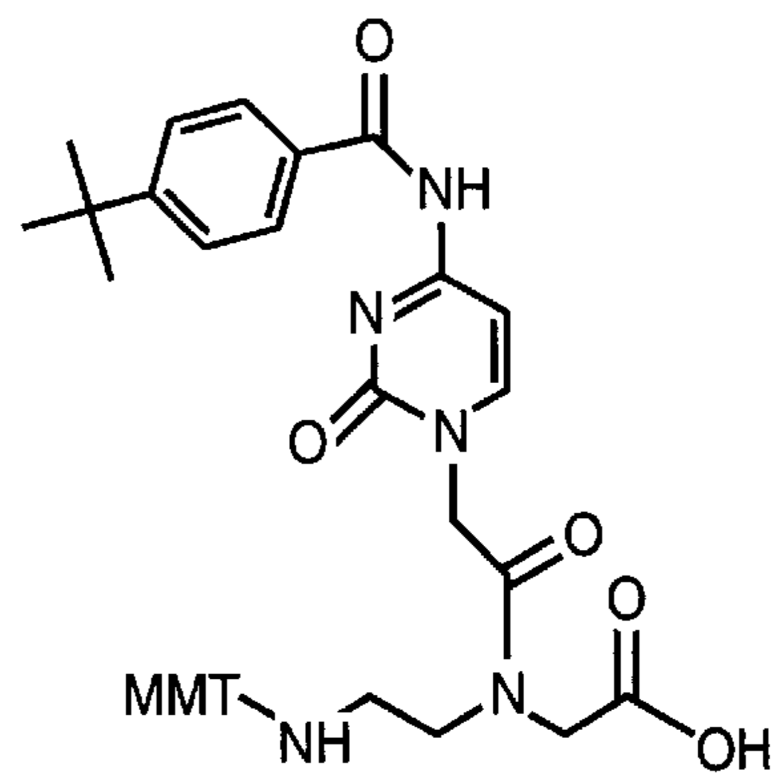
MMT-PNA-C
