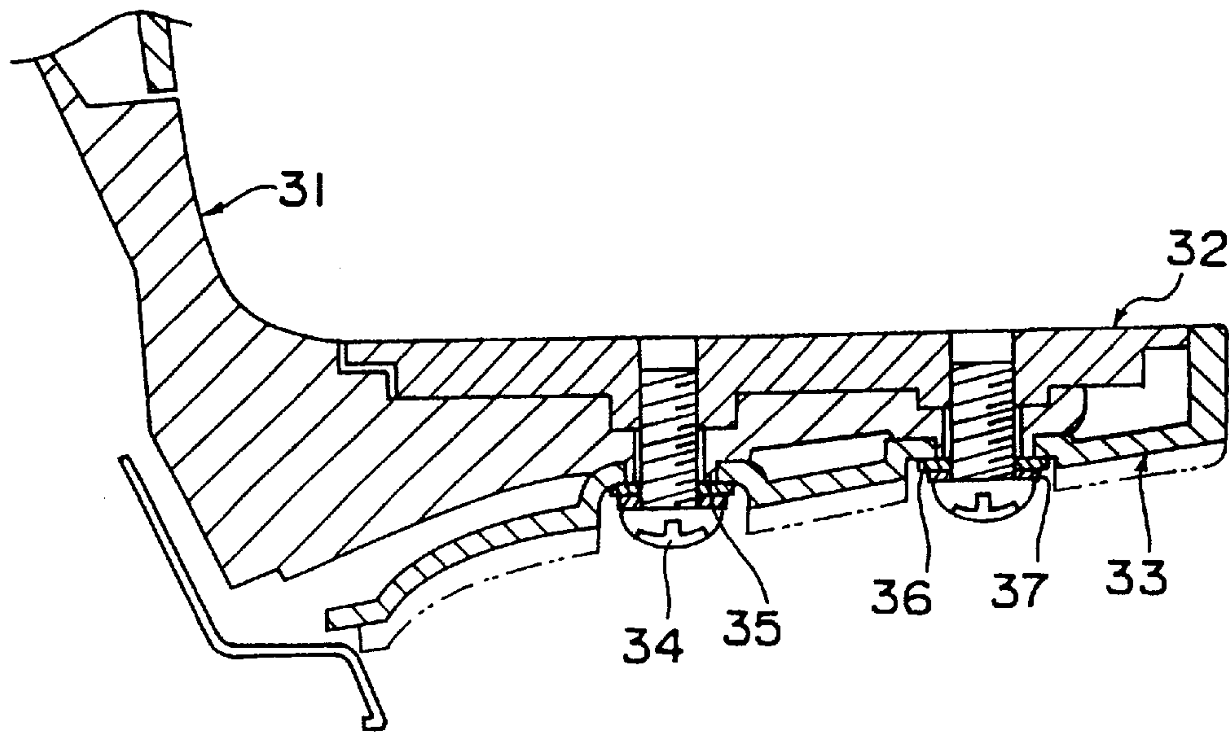
Fig. 6 PRIOR ART
