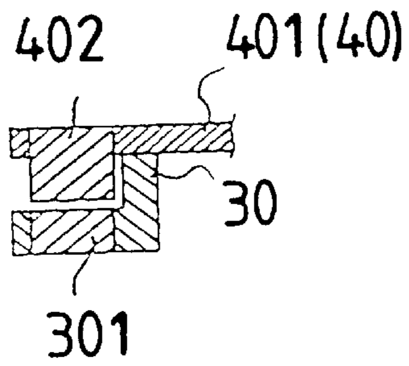
FIG. 6 (PRIOR ART)
