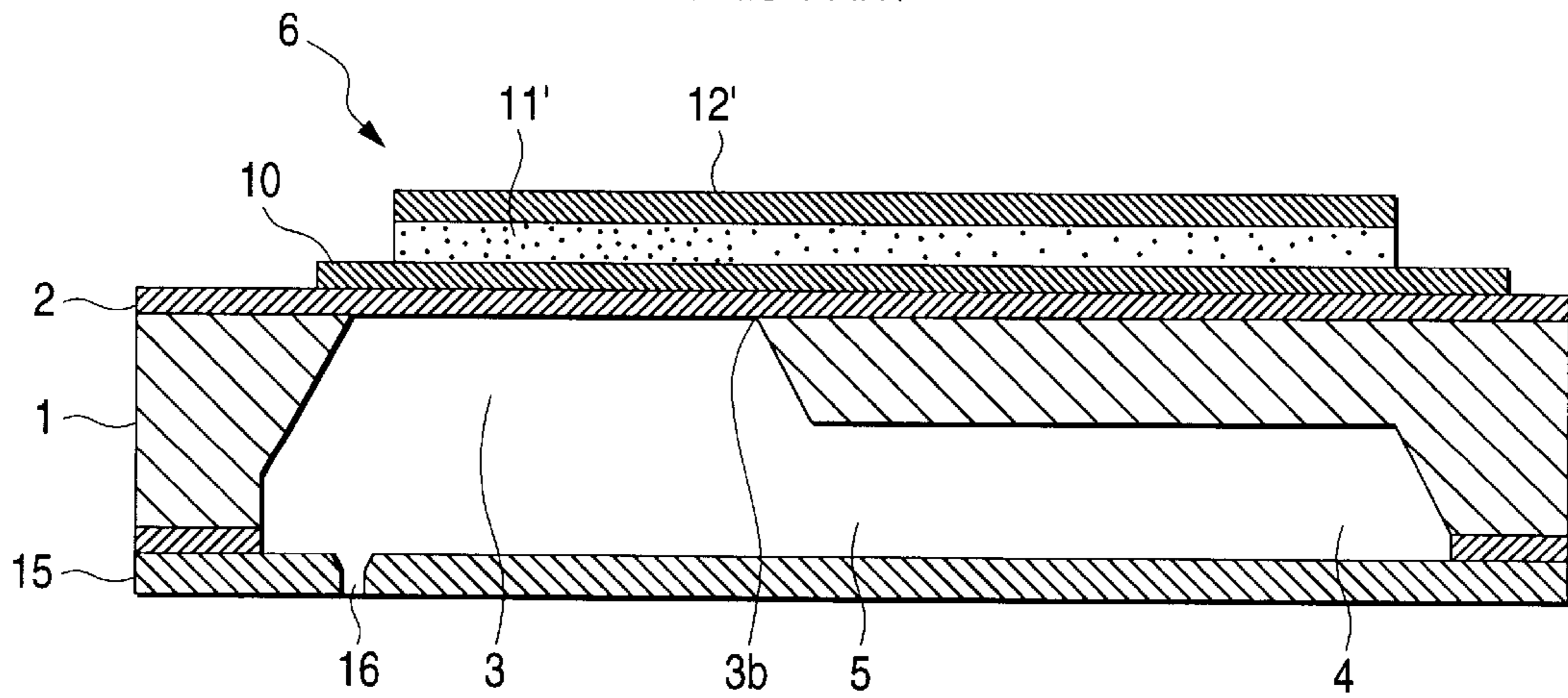
FIG. 8 PRIOR ART
