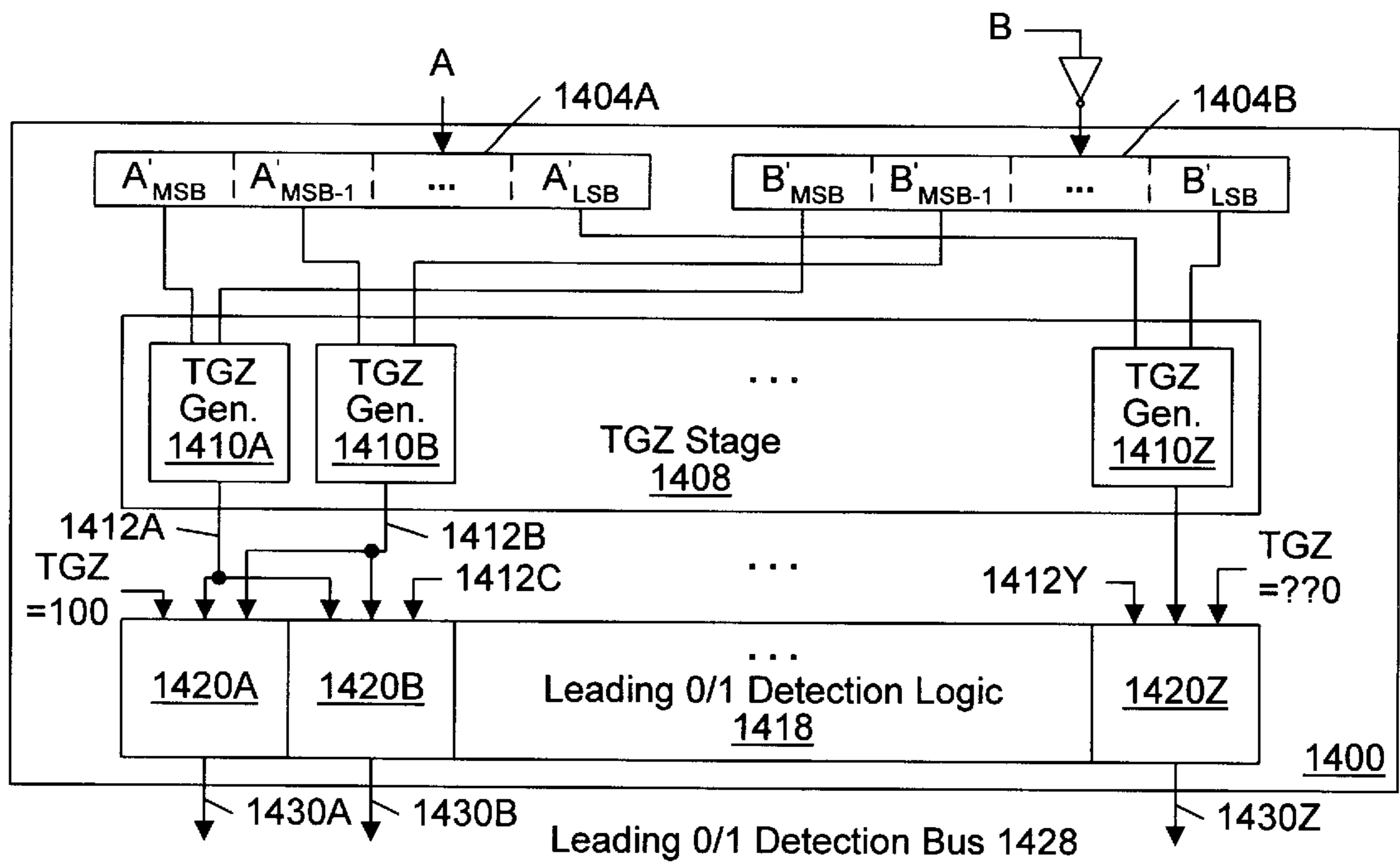
Fig. 20 (Prior Art)
