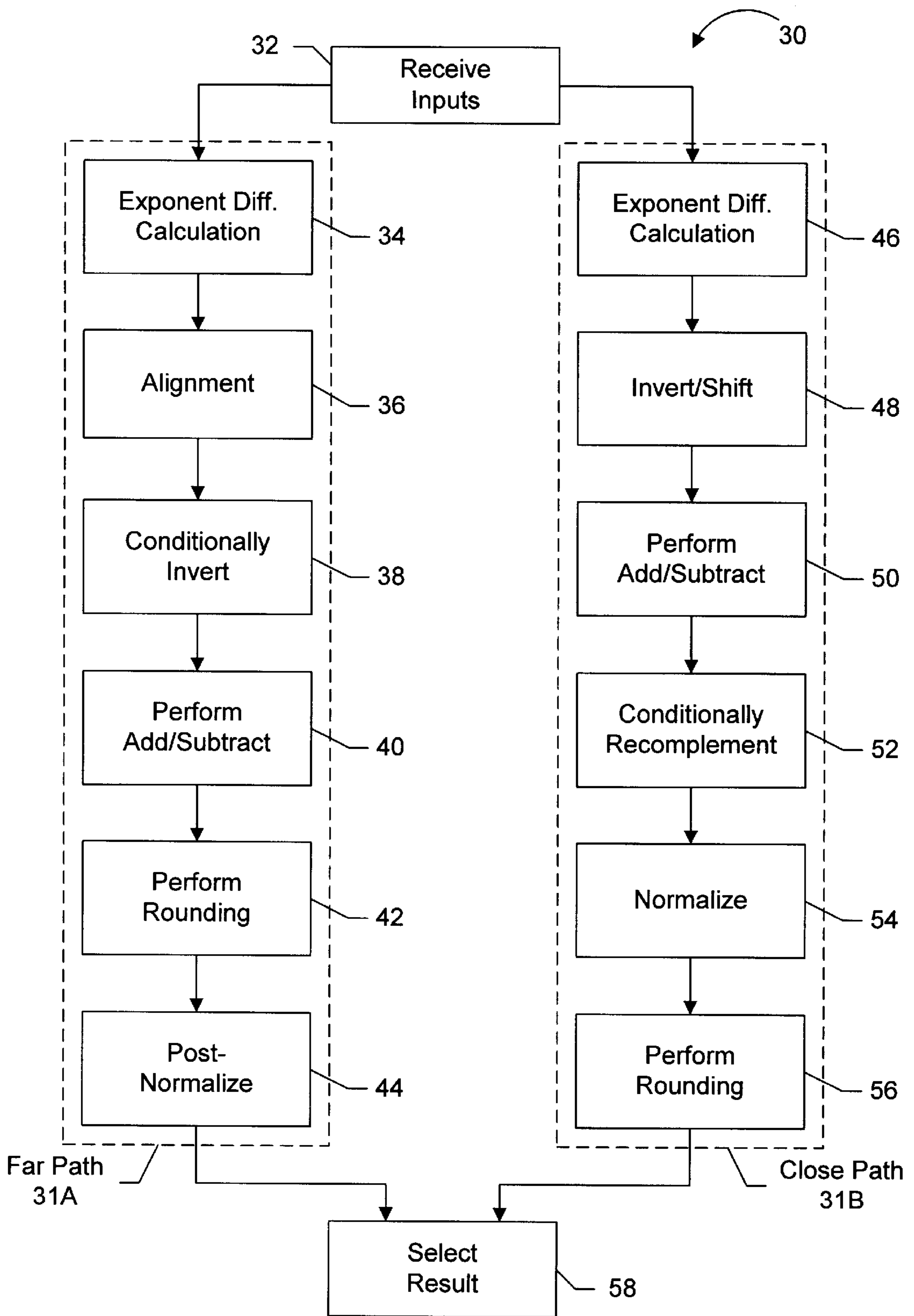
Fig. 3 (Prior Art)
