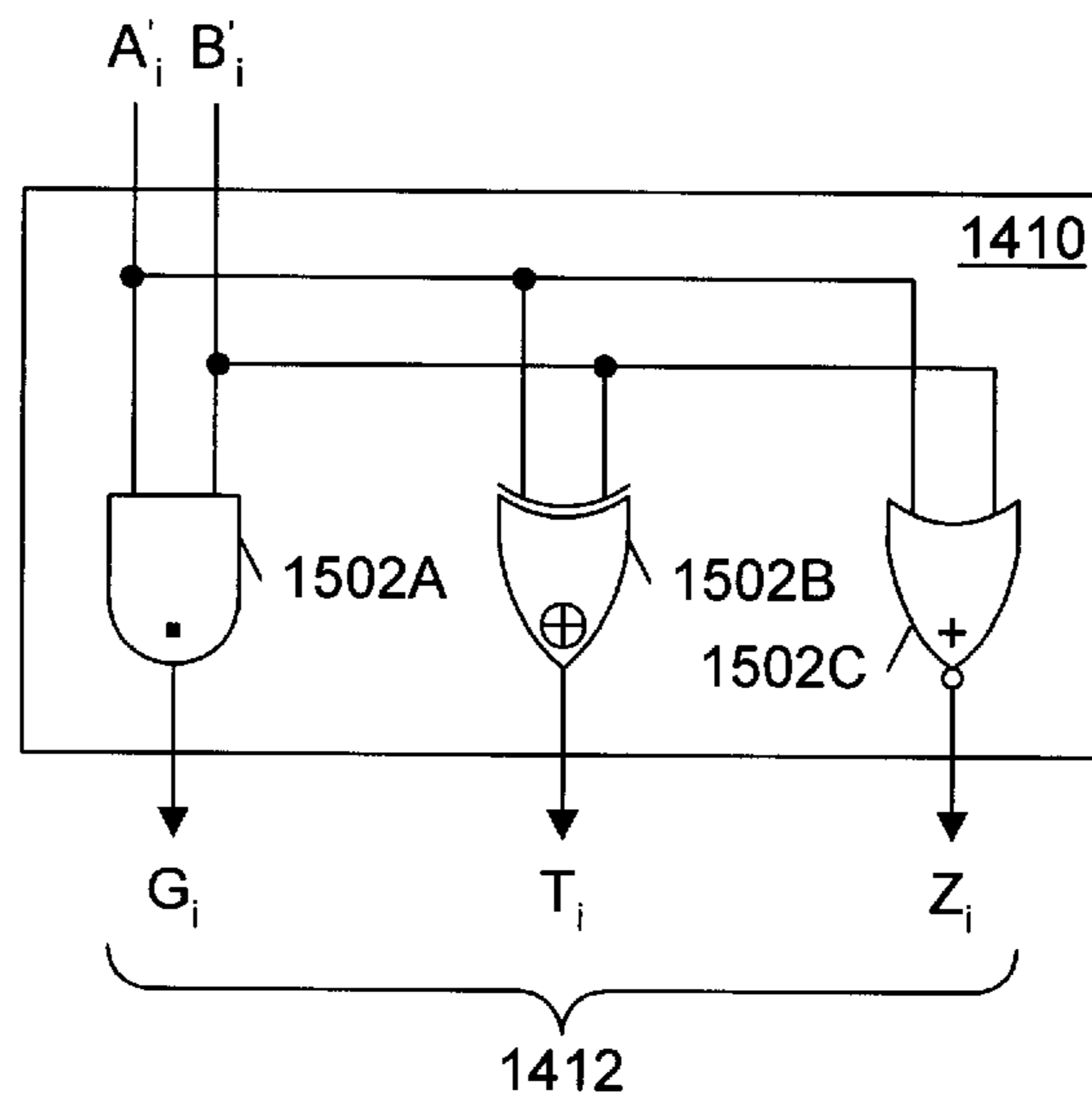
Fig. 21 (Prior Art)
