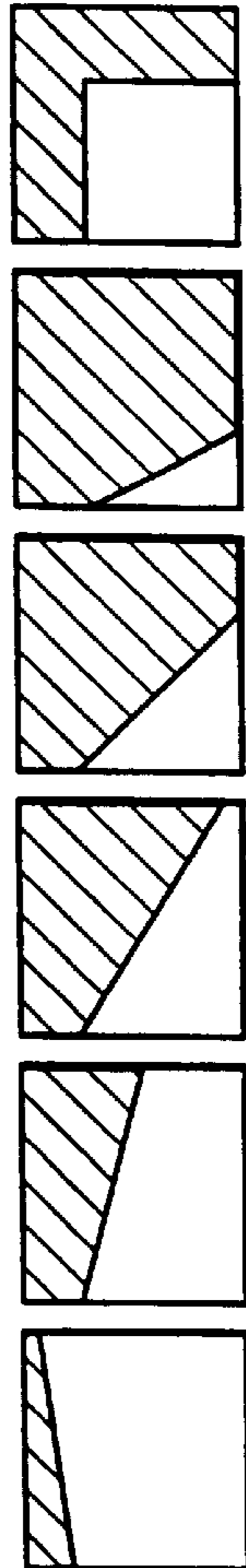
RL M=2
