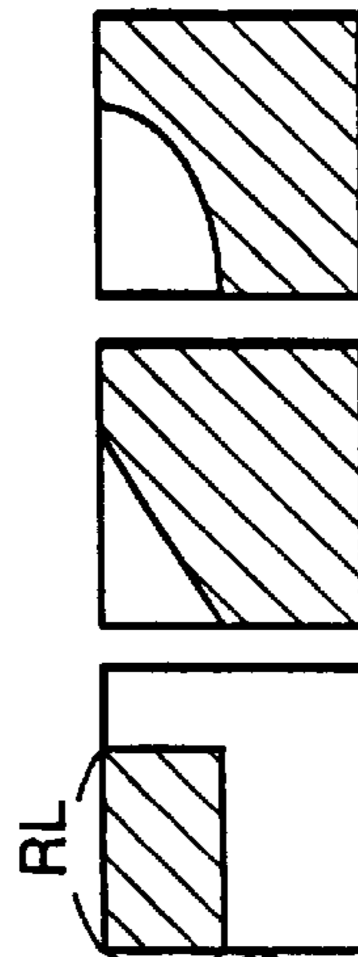
RL M=3
