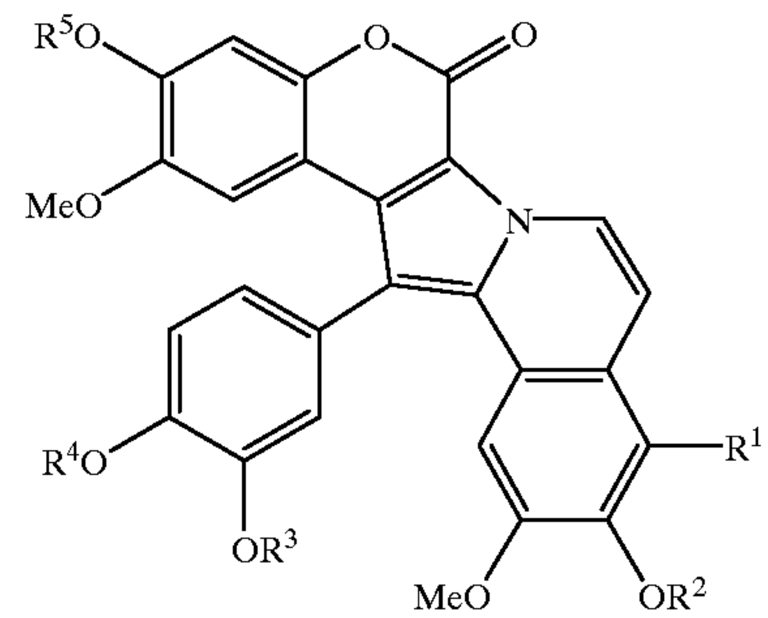
GROUP-II: Unsaturated Lamellarins
