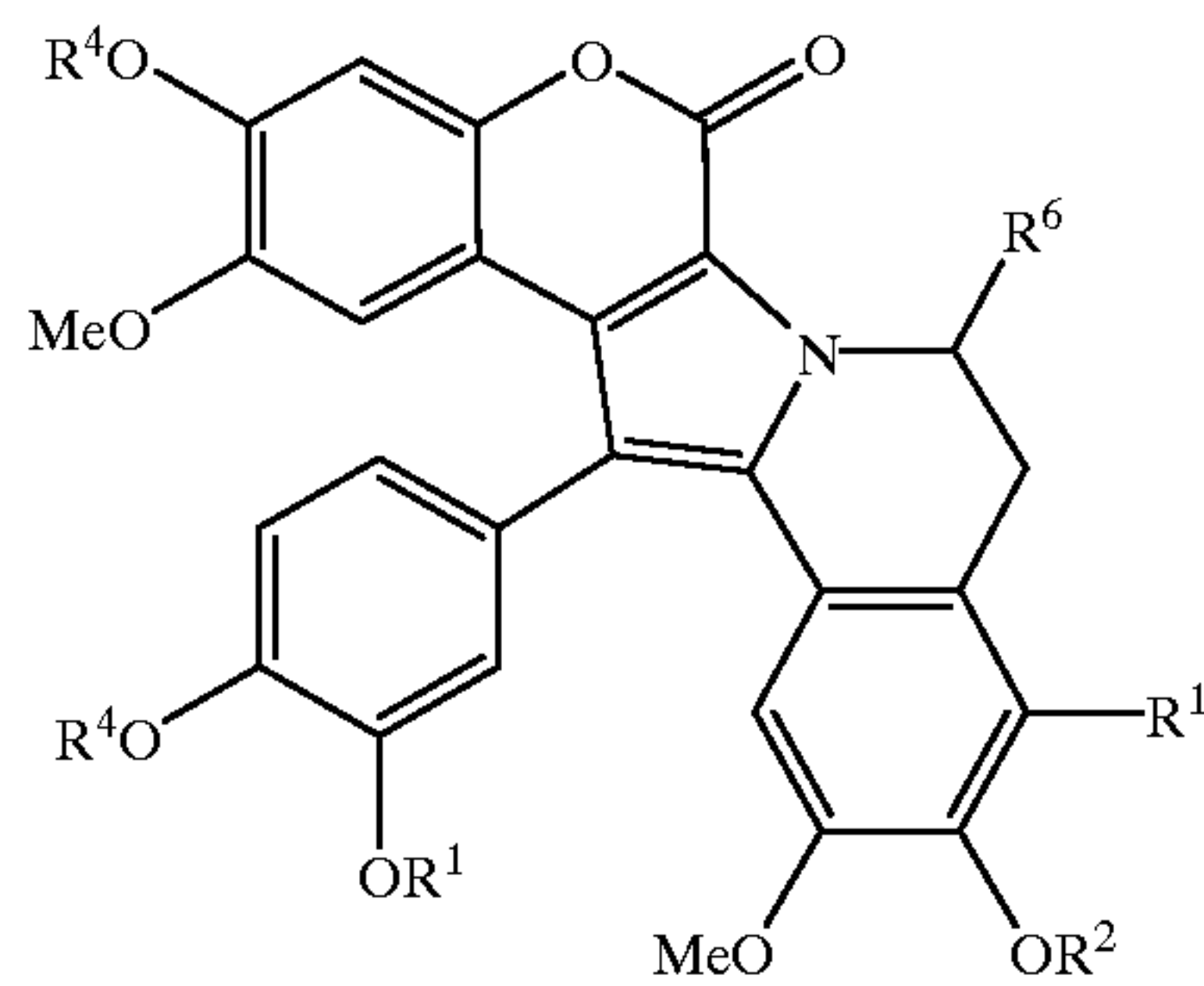
GROUP-I: Saturated Lamellarins
