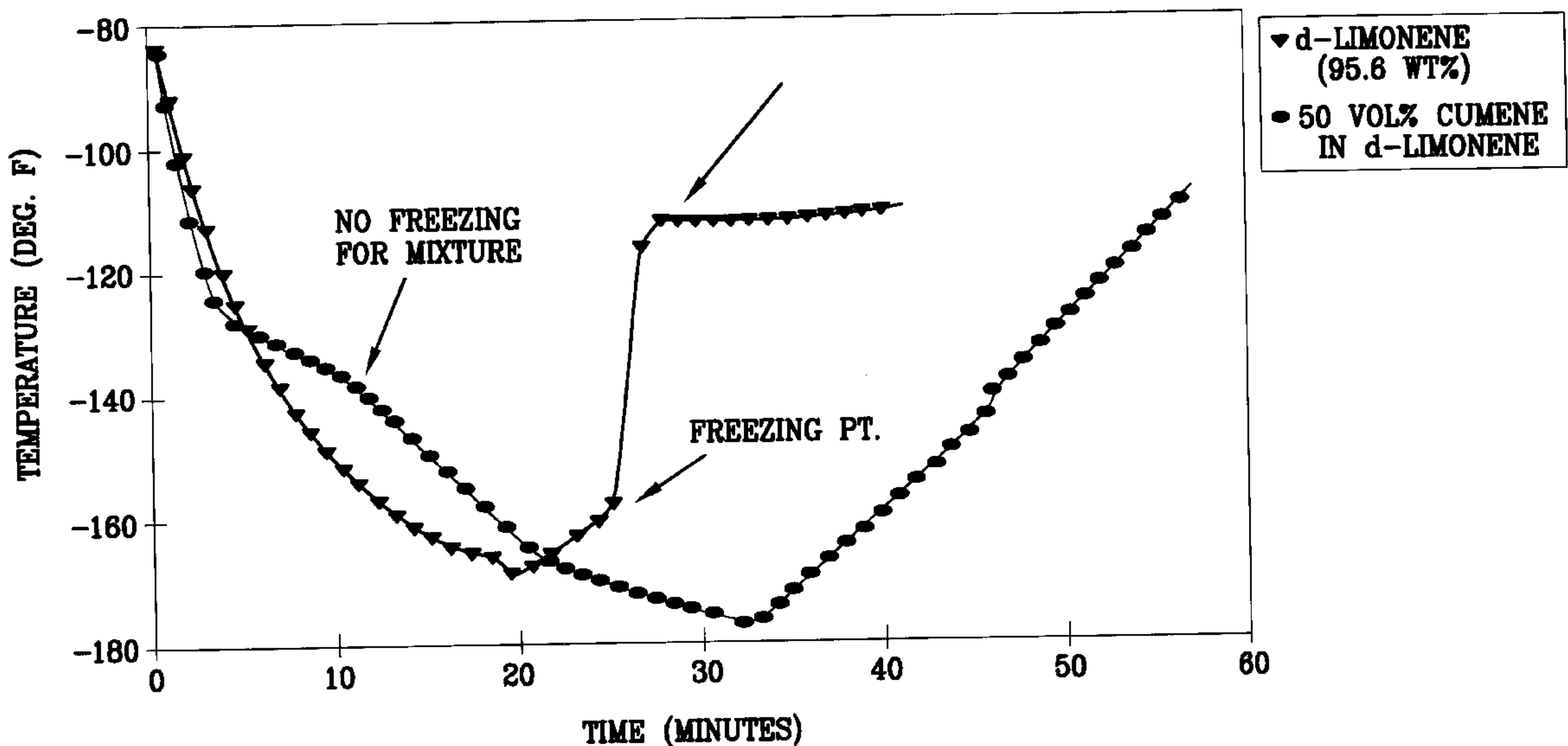
TEMP. vs. TIME FOR 95.6 WT% d-LIMONENE AND FOR 50 VOL% CUMENE IN d-LIMONENE
