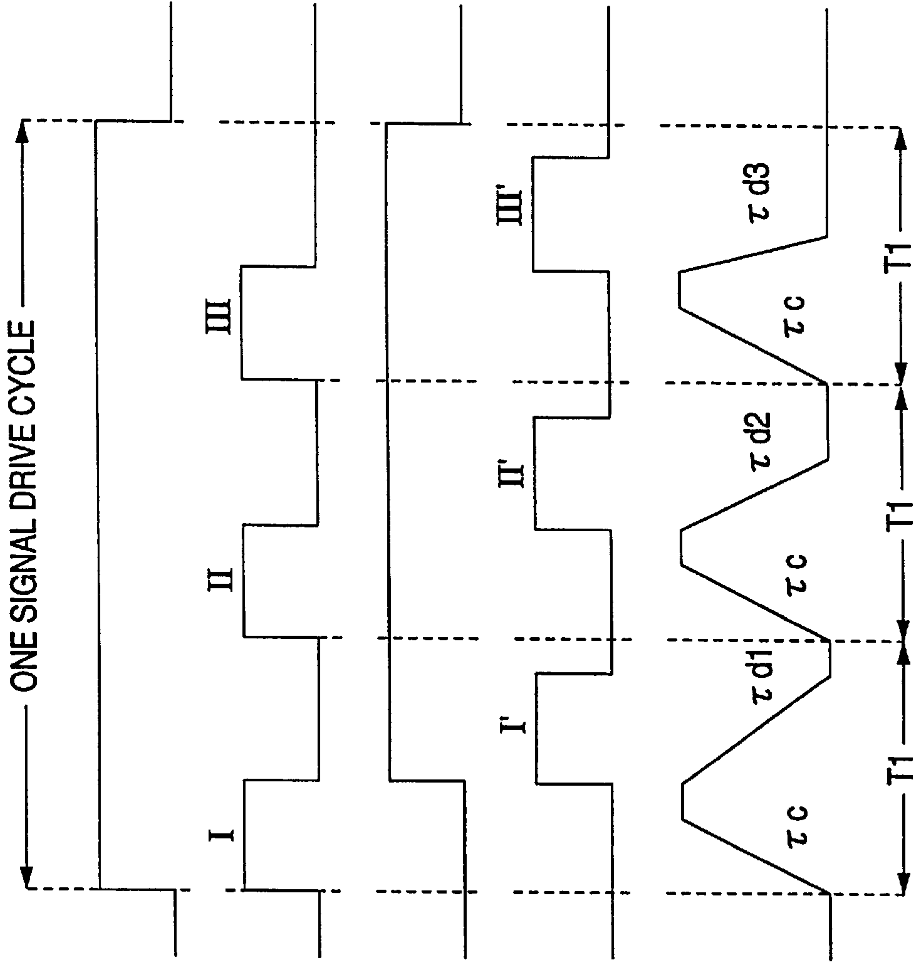
FIG. 3(a) AUXILIARY PRINT SIGNAL
