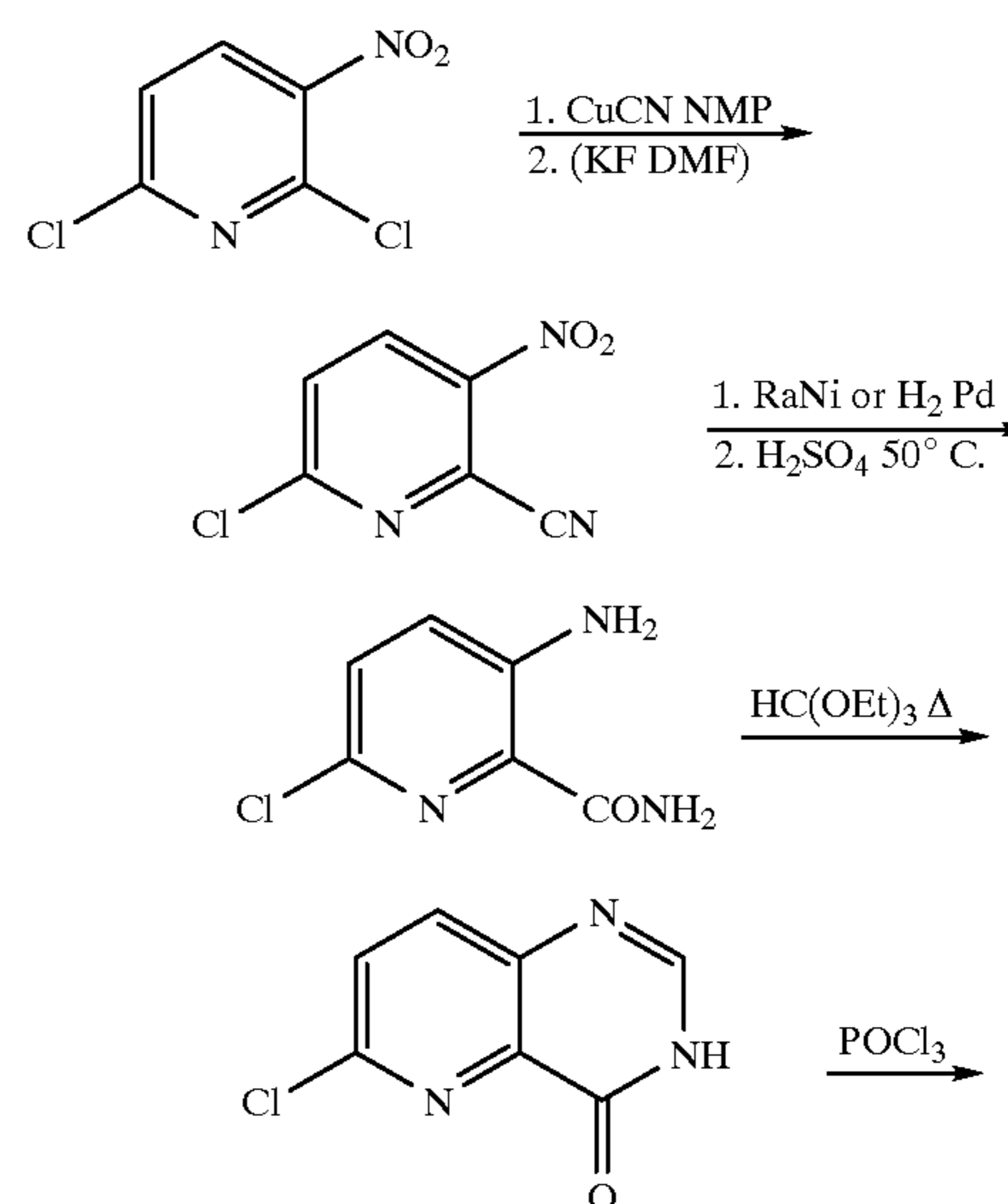
Scheme 1. Synthesis of Preferred Groups 1-5: R 4 = H
