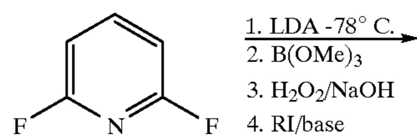
Scheme 3. Synthesis of Preferred Groups 6 and 8-10: \text{R}^4 = \text{RO}
