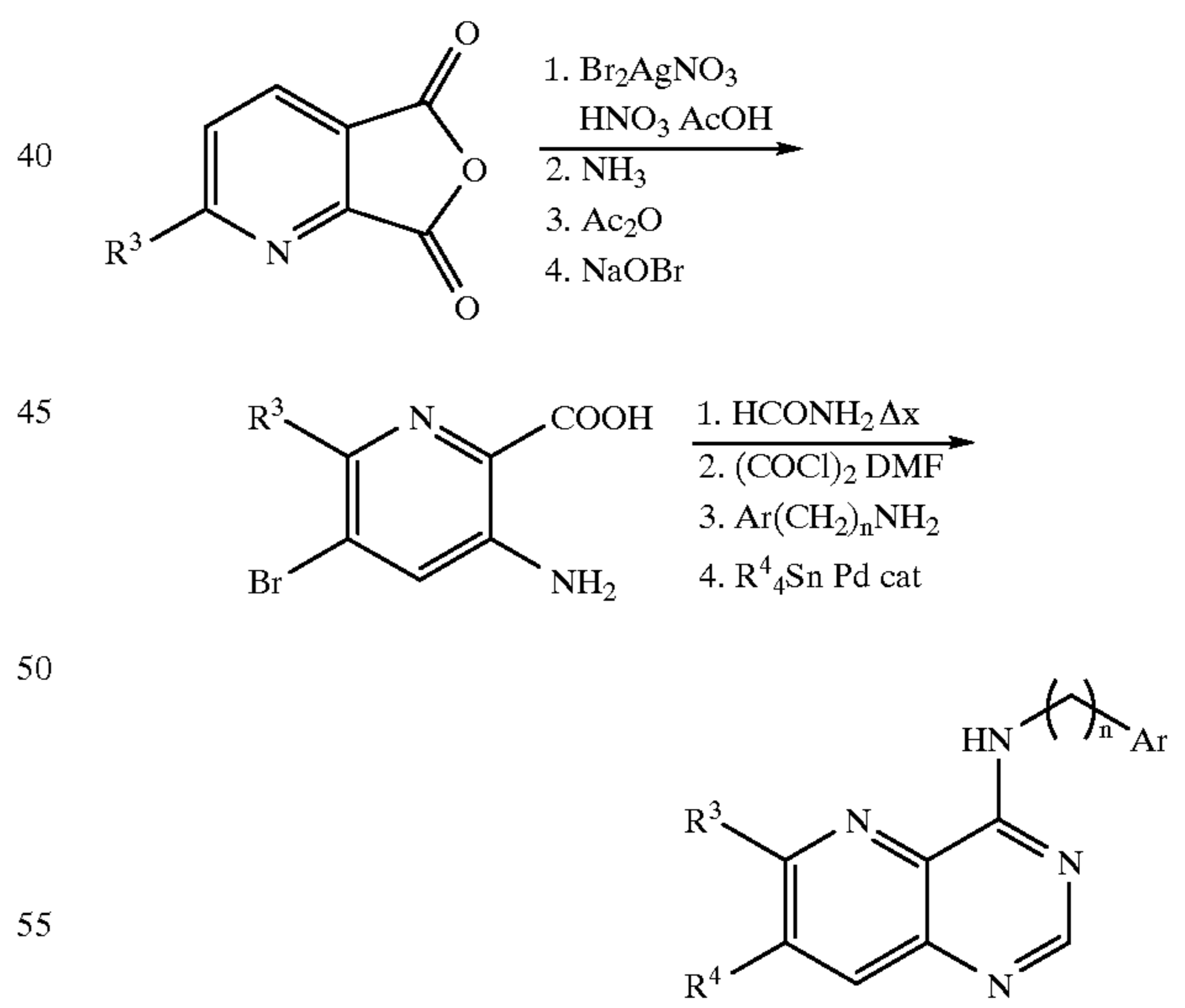
Scheme 4. Synthesis of Preferred Group 7.
