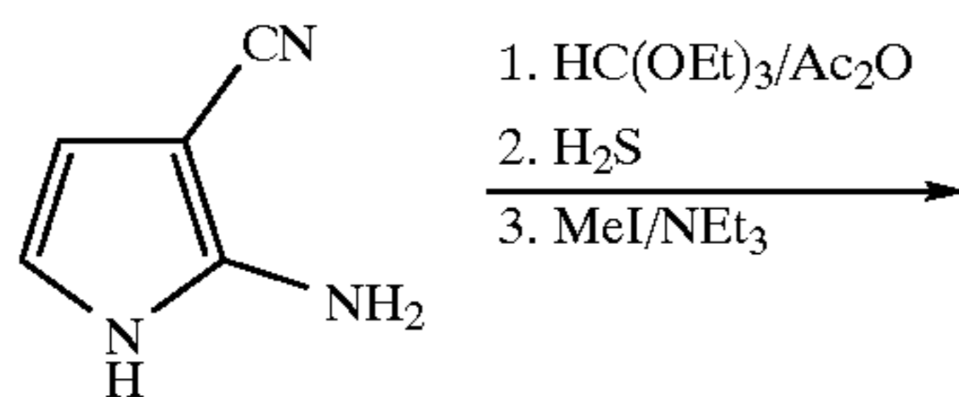
Scheme 21 Synthesis of Preferred Group 43: [2,3-d] ring fusion.
