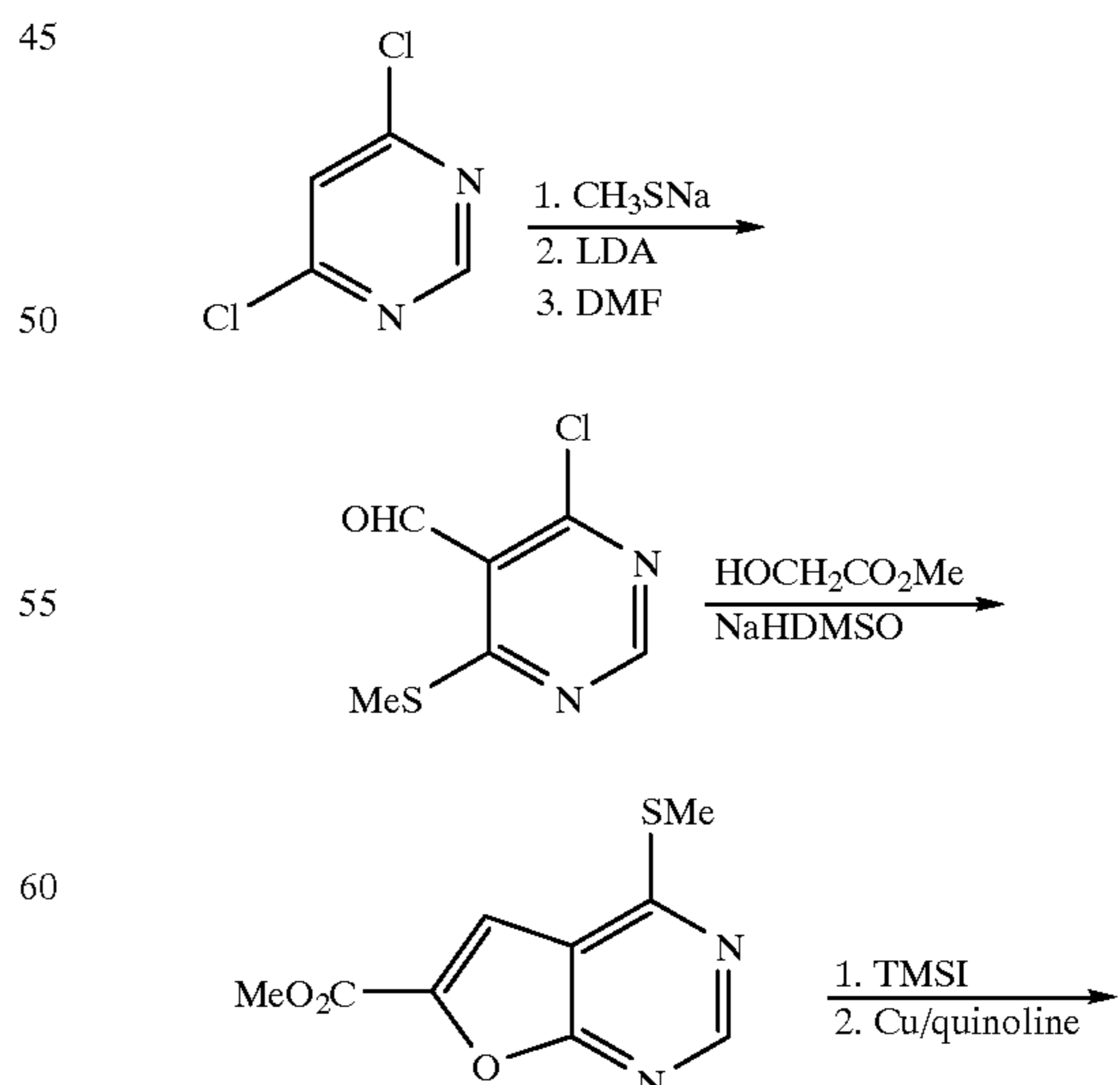
Scheme 20 Synthesis of Preferred Group 42: [2,3-d] ring fusion
