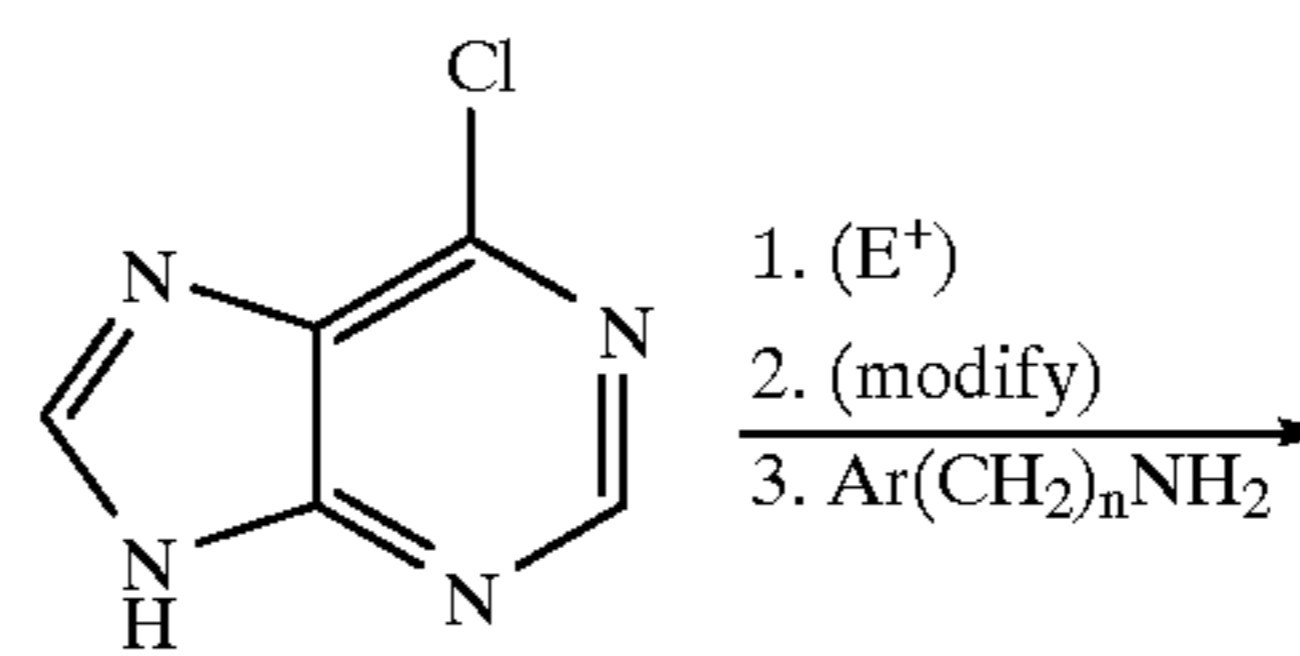
Scheme 27. Synthesis of Preferred Group 46.
