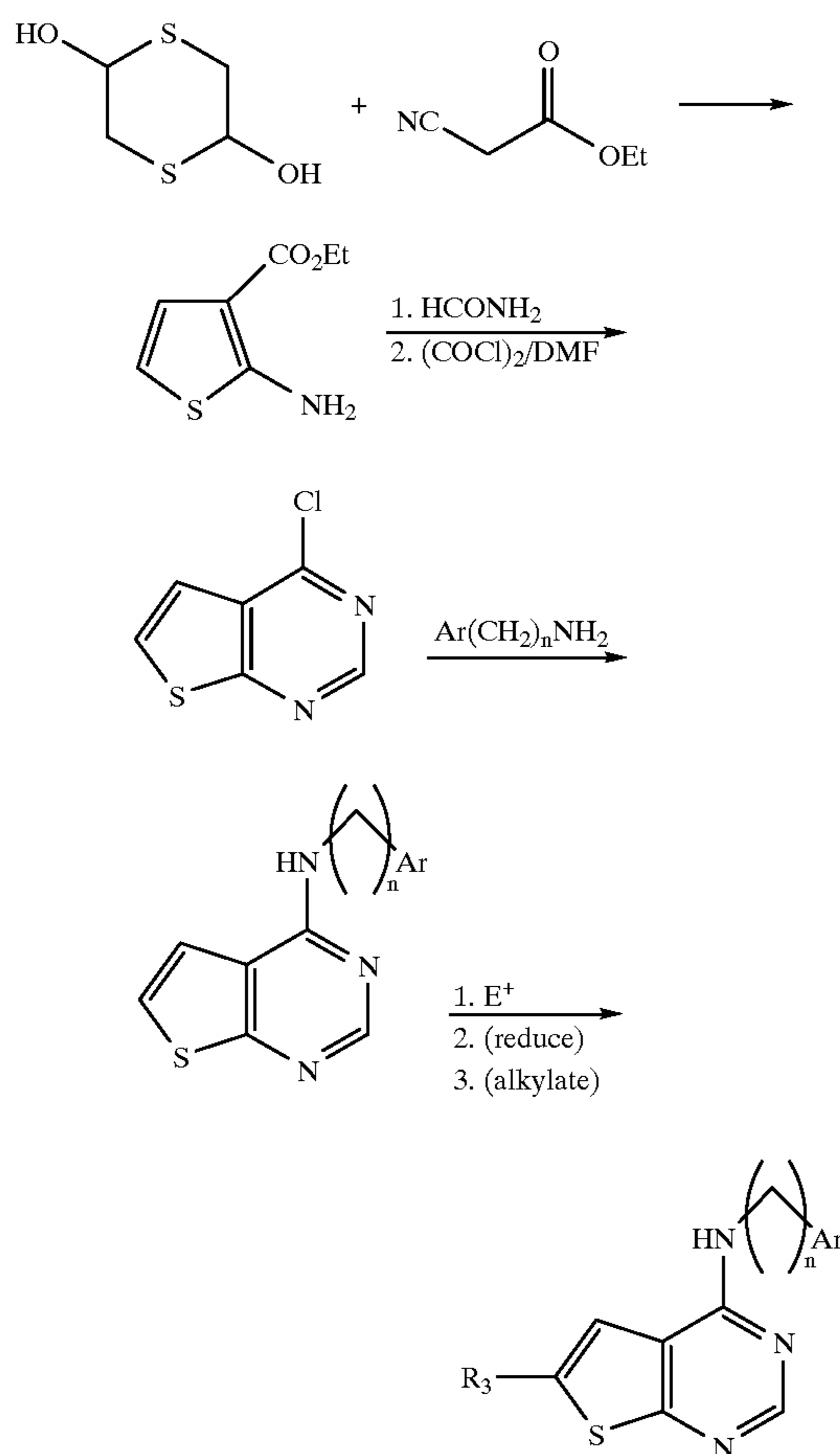
Scheme 18 Synthesis of Preferred Group 41: [2,3-d] ring fusion
