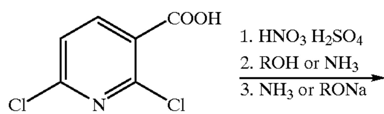
Scheme 13 Synthesis of Preferred Groups 29 & 30; R 4 = OR
