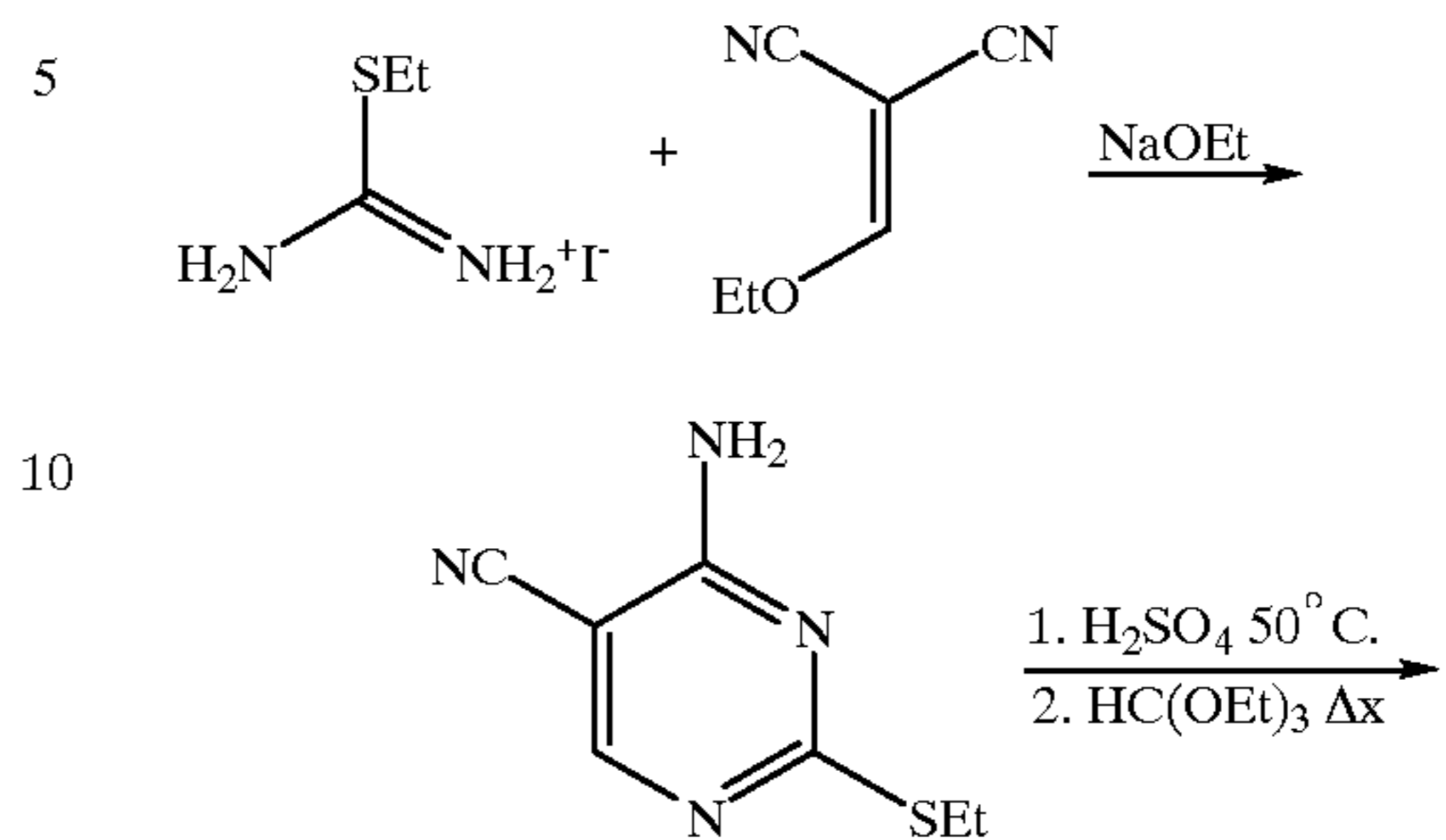
Scheme 15 Synthesis of Preferred Groups 33-36
