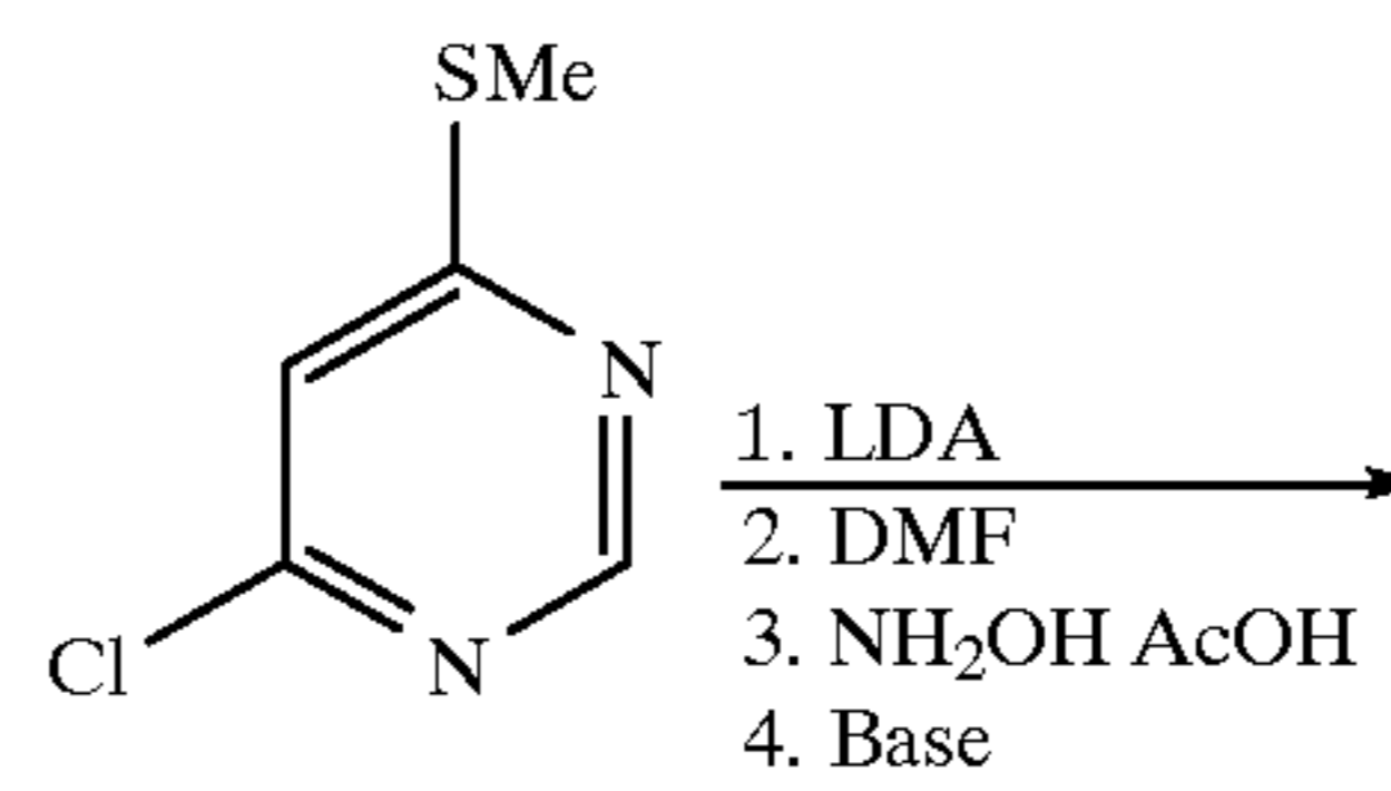
Scheme 28. Synthesis of Preferred Group 47: [5,4-d] ring fusion.
