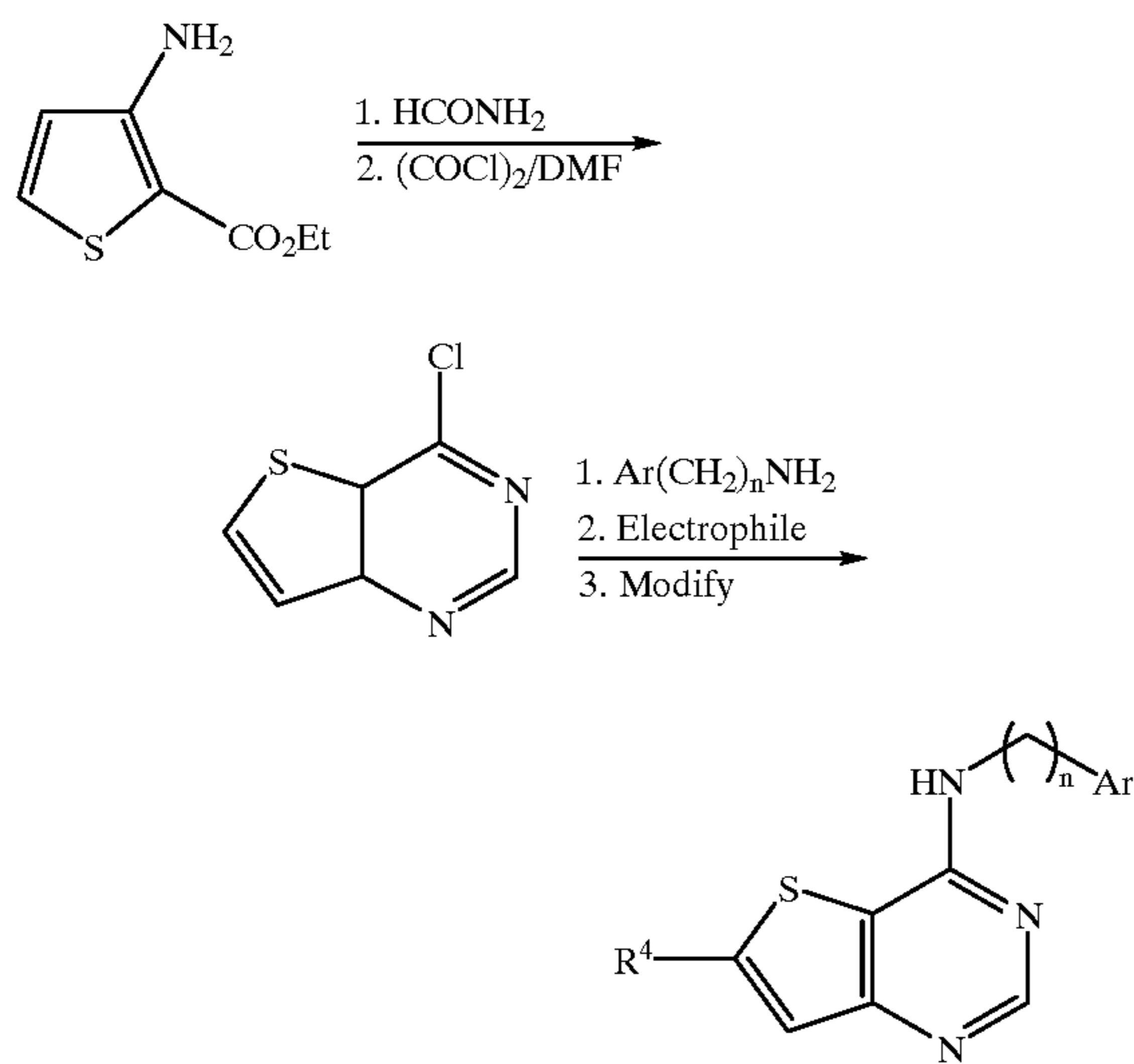
Scheme 17 Synthesis of Preferred Group 41: [3,2-d] ring fusion
