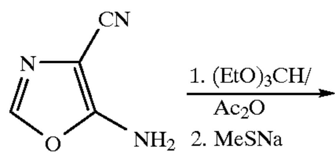
Scheme 25. Synthesis of Preferred Group 45: [5,4-d] ring fusion.
