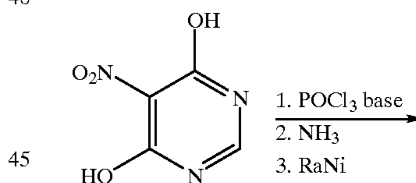
Scheme 16 Synthesis of Preferred Groups 37-40
