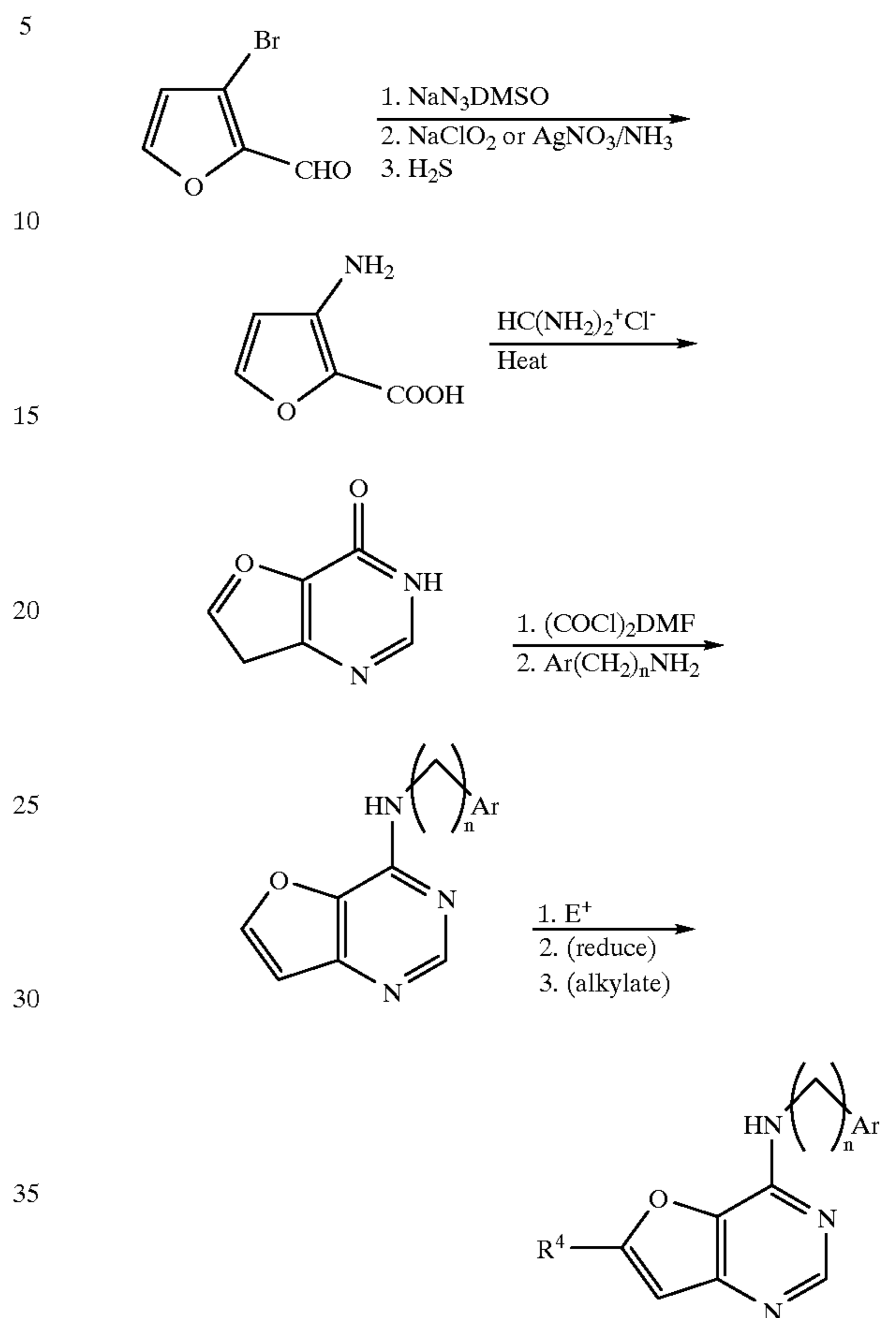
Scheme 19 Synthesis of Preferred Group 42: [3,2-d] ring fusion
