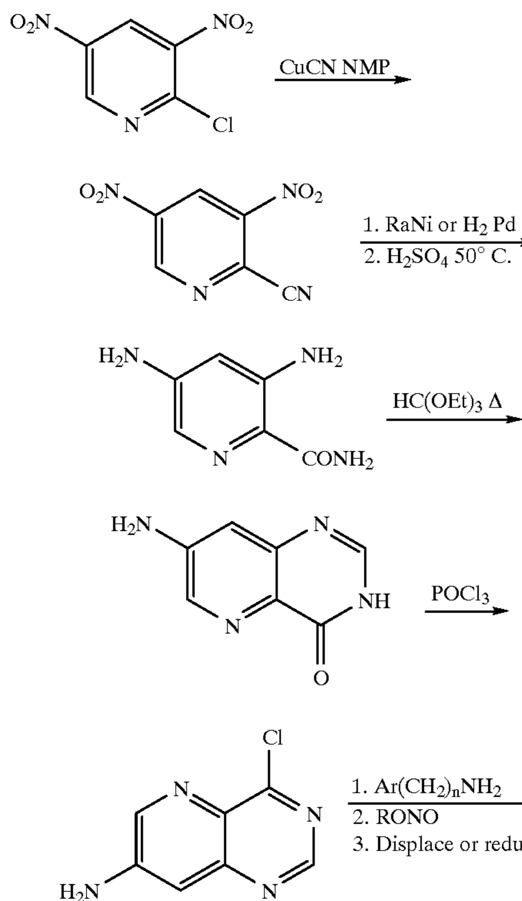
Scheme 2. Synthesis of Preferred Groups 1-5: \text{R}^3 = \text{H}
