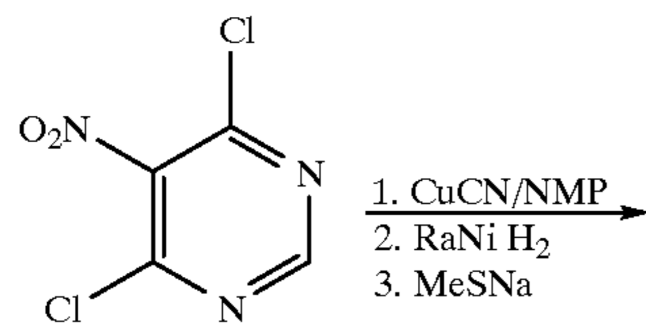
Scheme 31. Synthesis of Preferred Group 48: [4,5-d] ring fusion.
