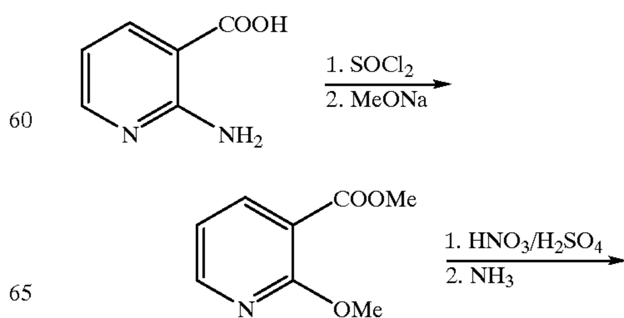
Scheme 9 Synthesis of Preferred Groups 22-26; R 4 = H
