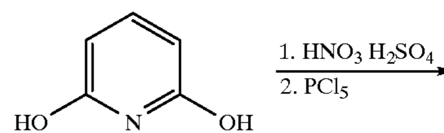
Scheme 5. Synthesis of Preferred Groups 8 & 9: \text{R}^3 = \text{OR} .
