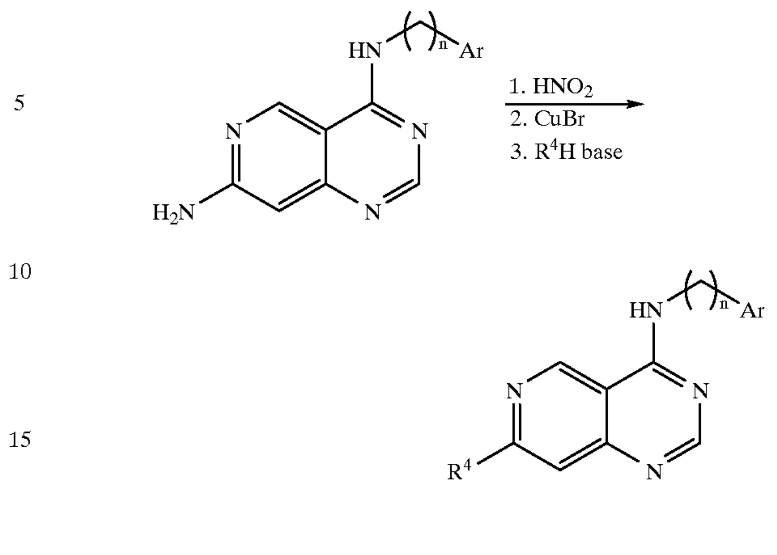
Scheme 8 Synthesis of Preferred Groups 17-21
