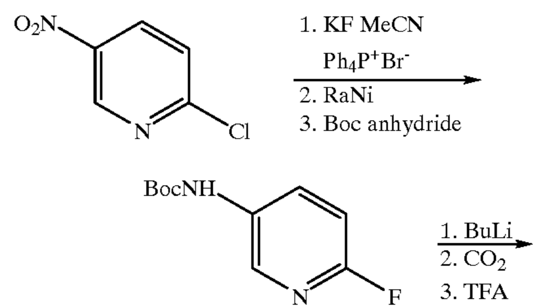
Scheme 8 Synthesis of Preferred Groups 17-21
