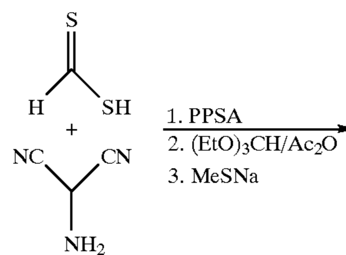
Scheme 23 Synthesis of Preferred Group 44: [5,4-d] ring fusion.
