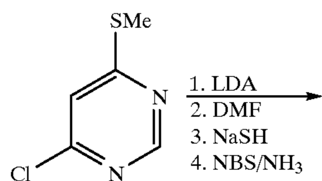
Scheme 30. Synthesis of Preferred Group 48: [5,4-d] ring fusion.
