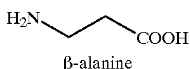
\beta -alanine
