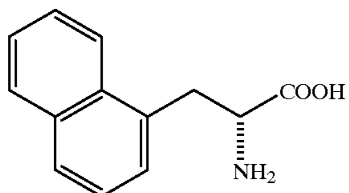
D-1-Nal
