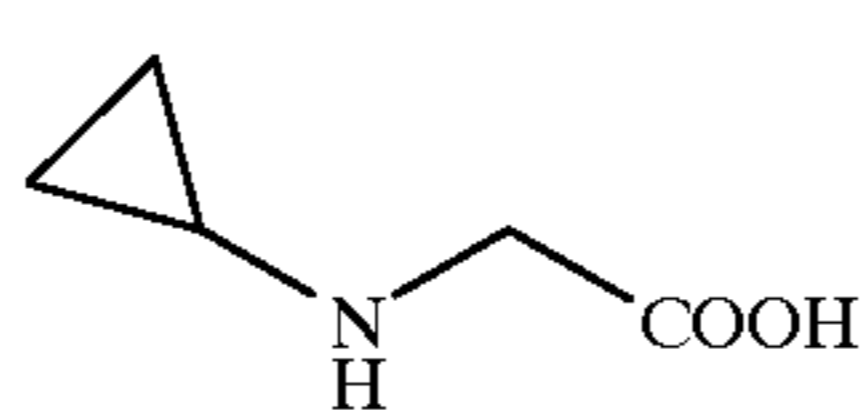
N-Cyclopropyl glycine
