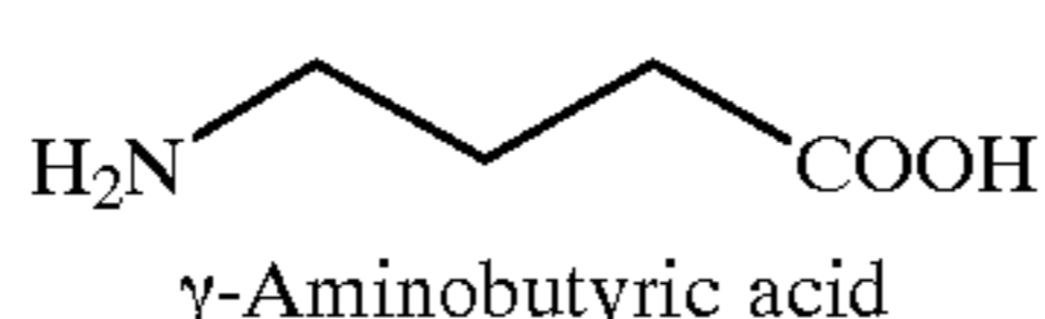
\gamma -Aminobutyric acid
