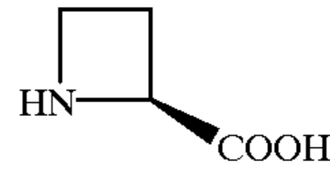
L-Azetidine carboxylic acid
