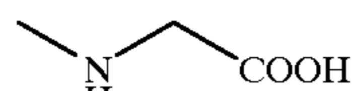
Sarcosine
