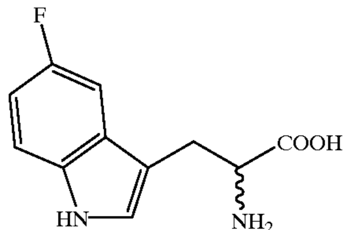
DL-5-F-Trp
