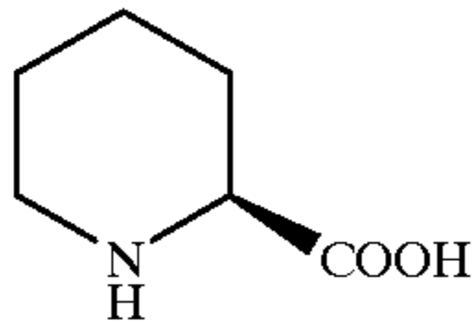
L-Pipecolic acid
