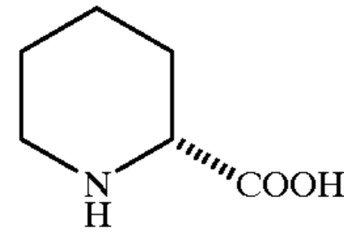
D-Pipecolic acid
