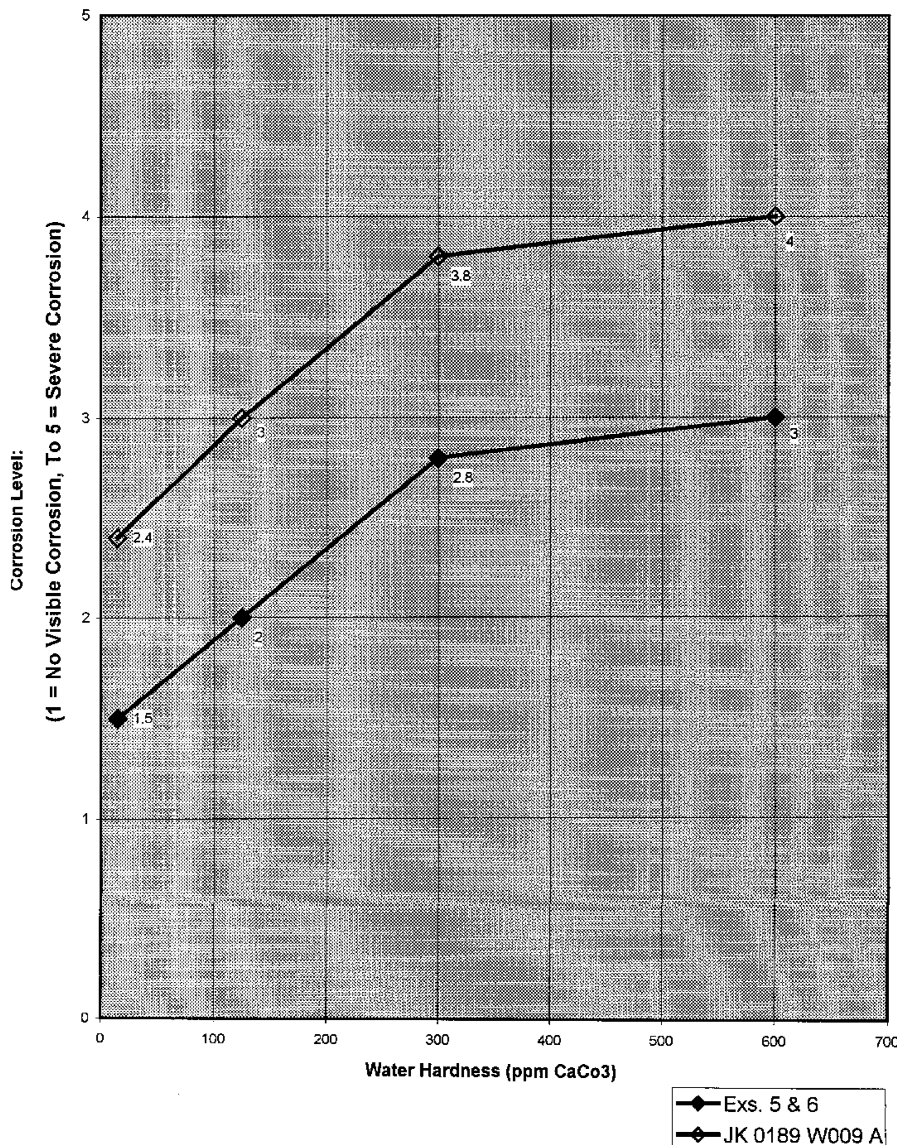
Corrosion Of (.1%) Detergent Concentrations Of Formula examples #5 and 6 and formula JK 0189 W009 A (Control) on Glass In Various ppm Of Water Hardness.
