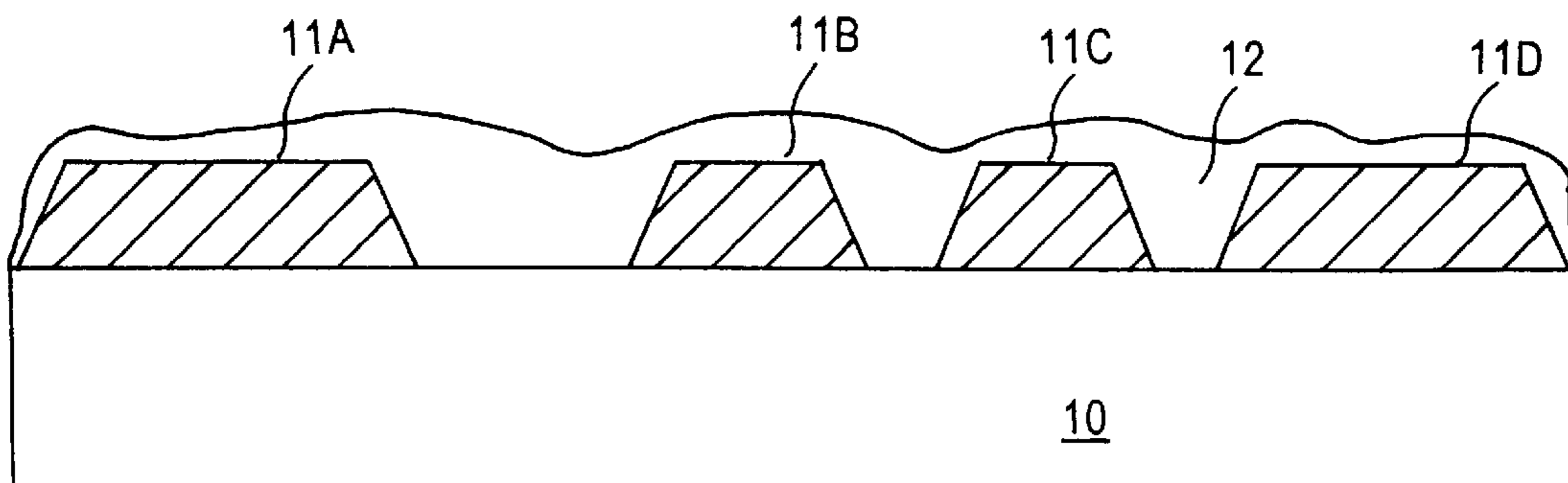
FIG. 2 (PRIOR ART)
