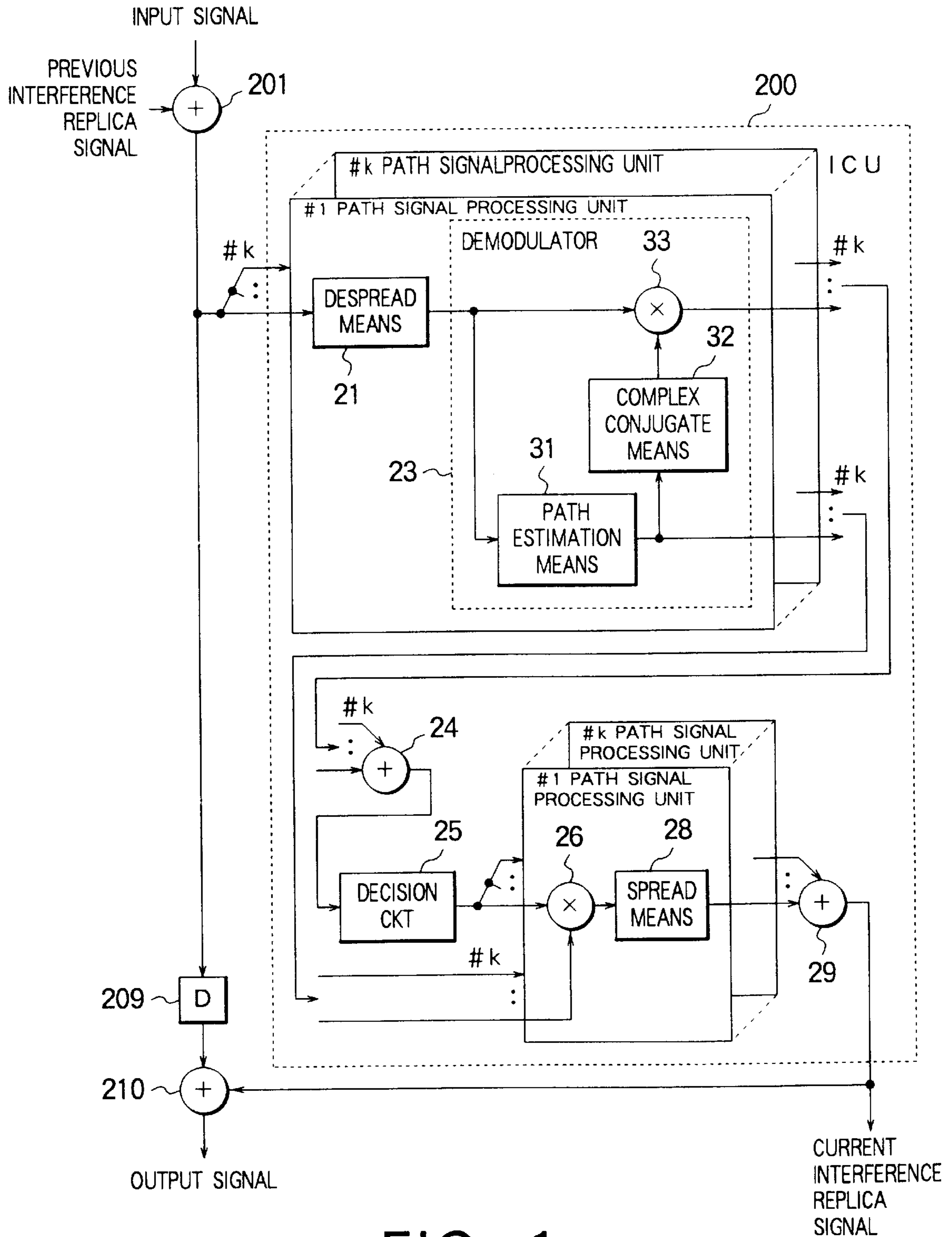
FIG. 1 PRIOR ART
