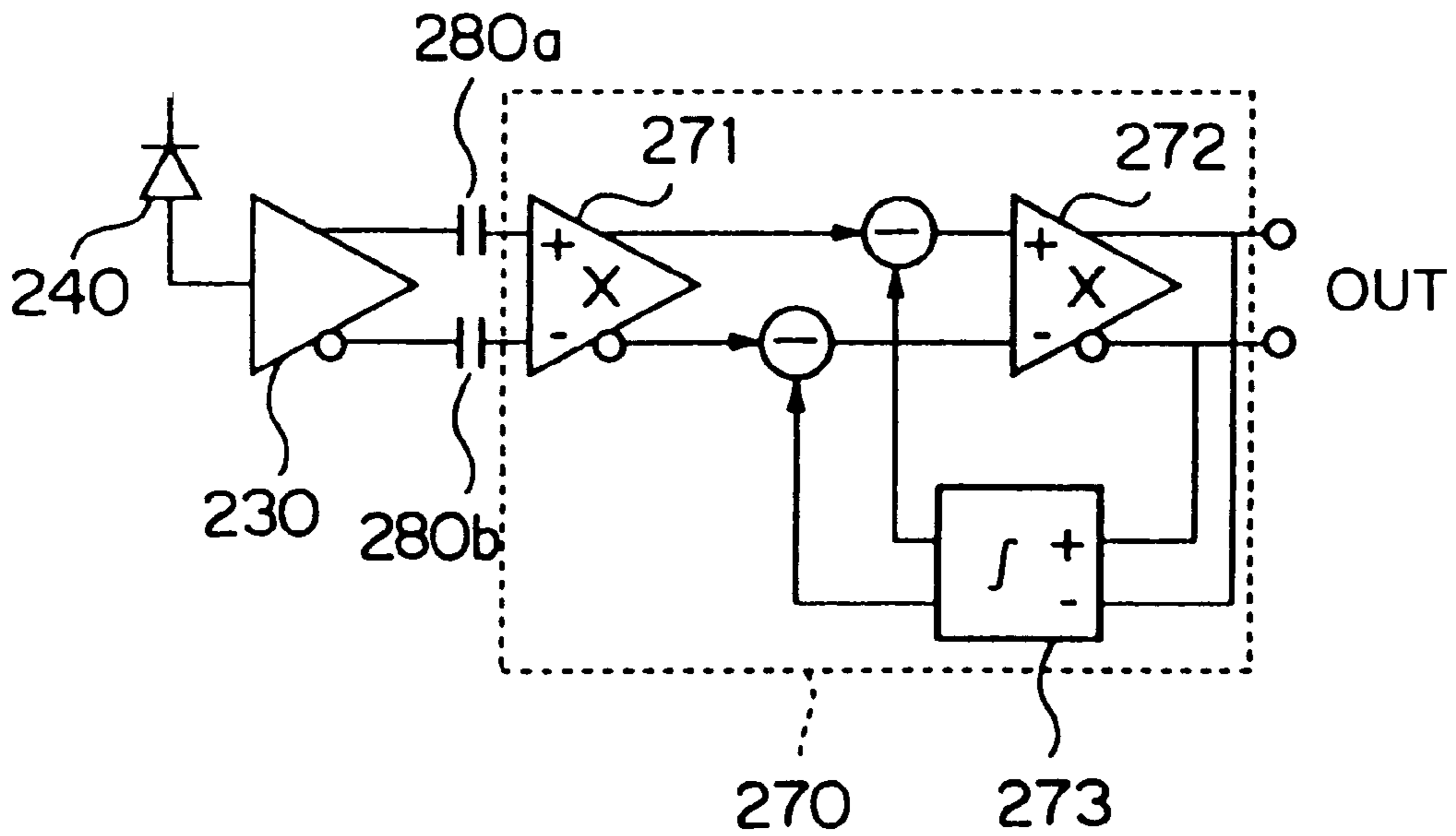
FIG. 2 PRIOR ART
