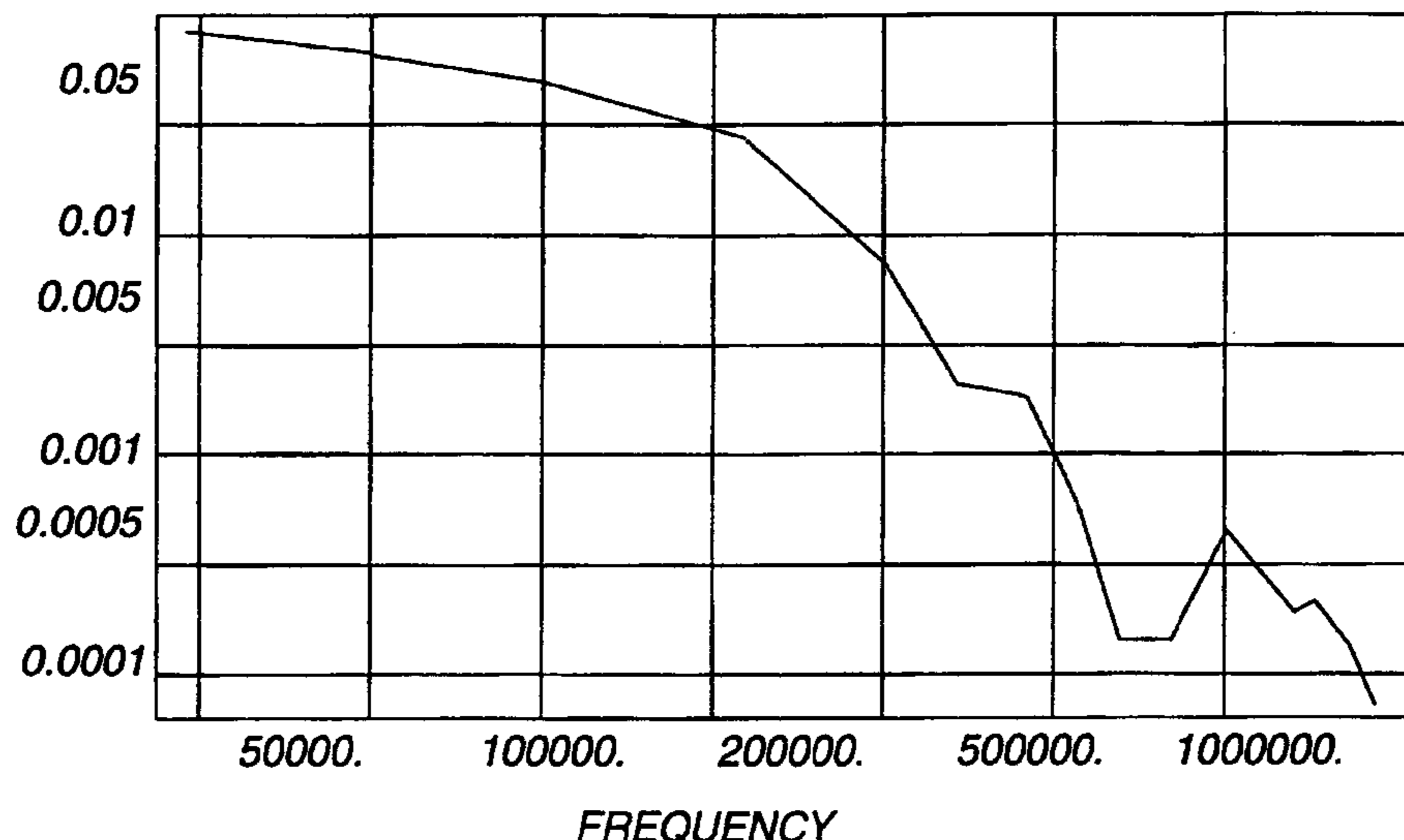
AMPLITUDE VERSUS FREQUENCY OF INTER-BUILDING UTP LOOP
