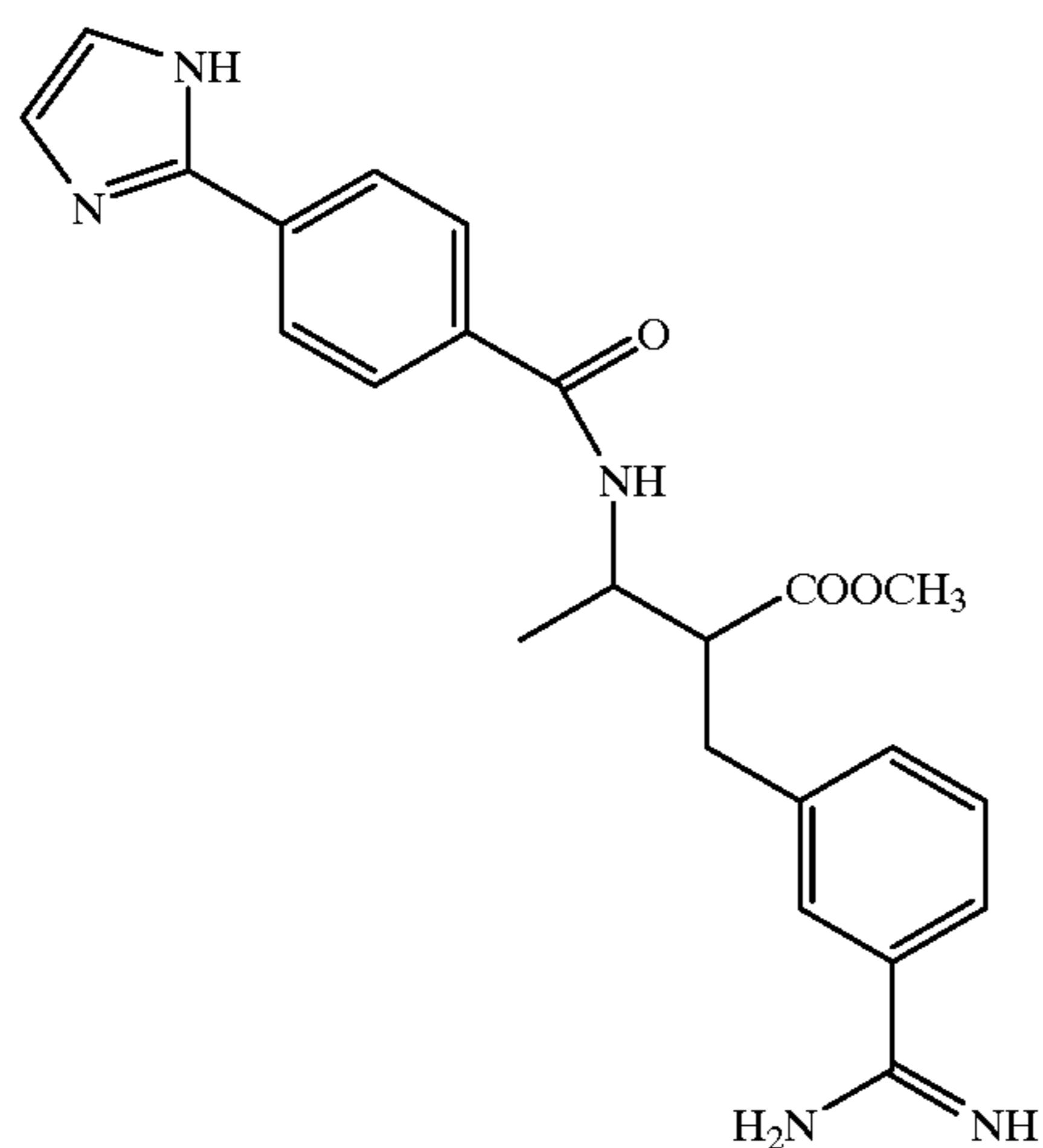
Compound 281
