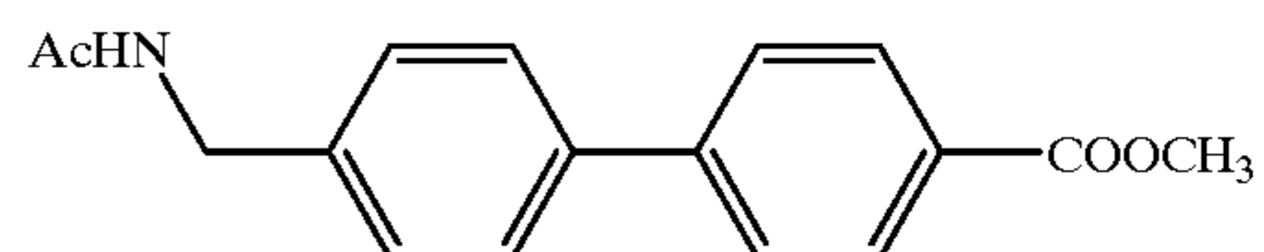
Compound 87
