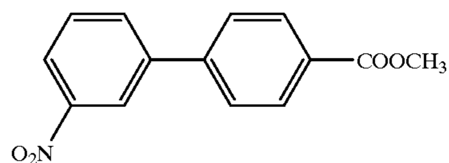
Compound 88
