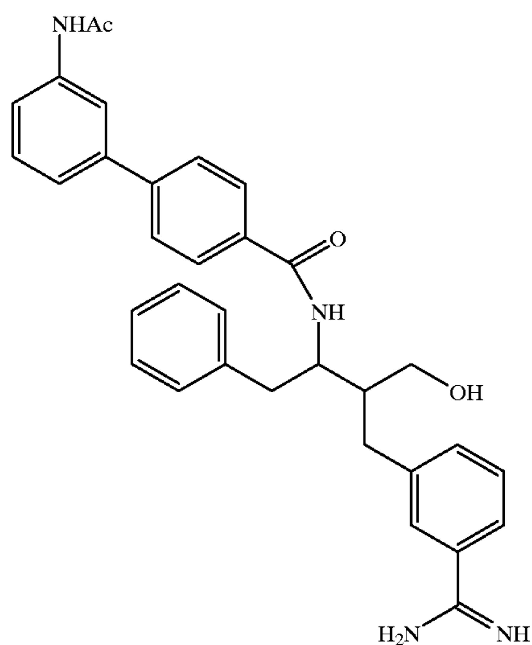
Compound 182
