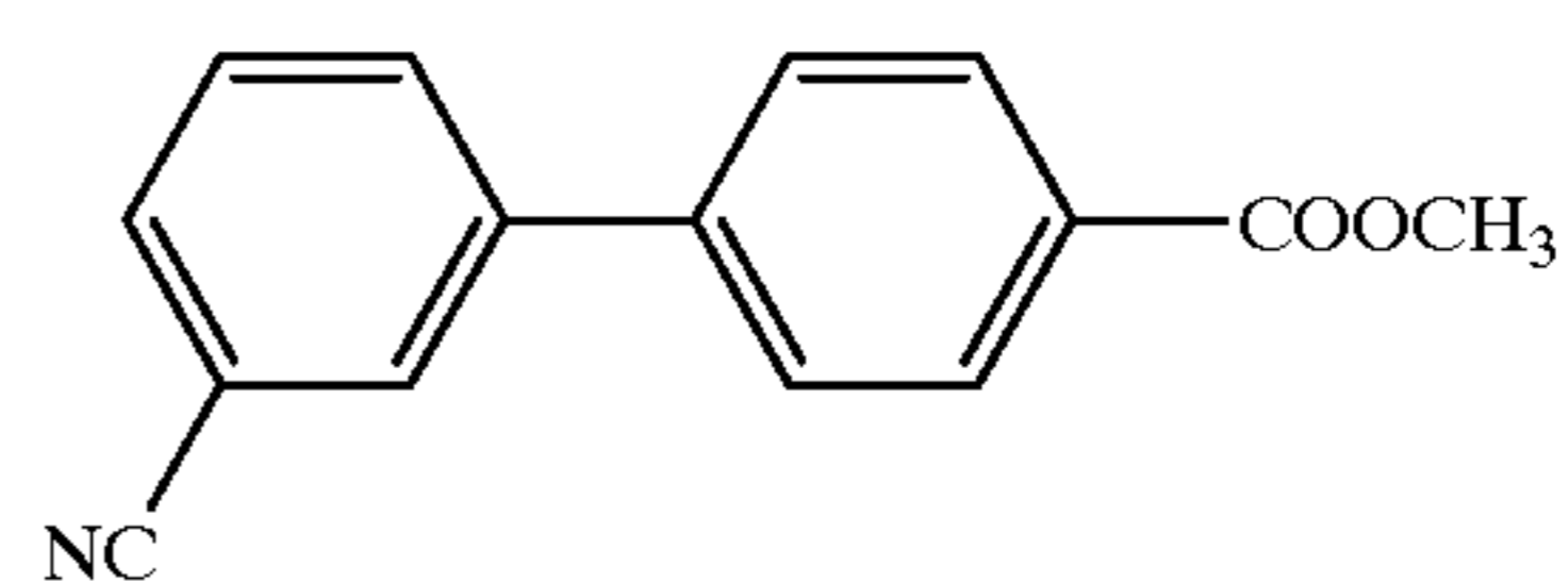
Compound 80
