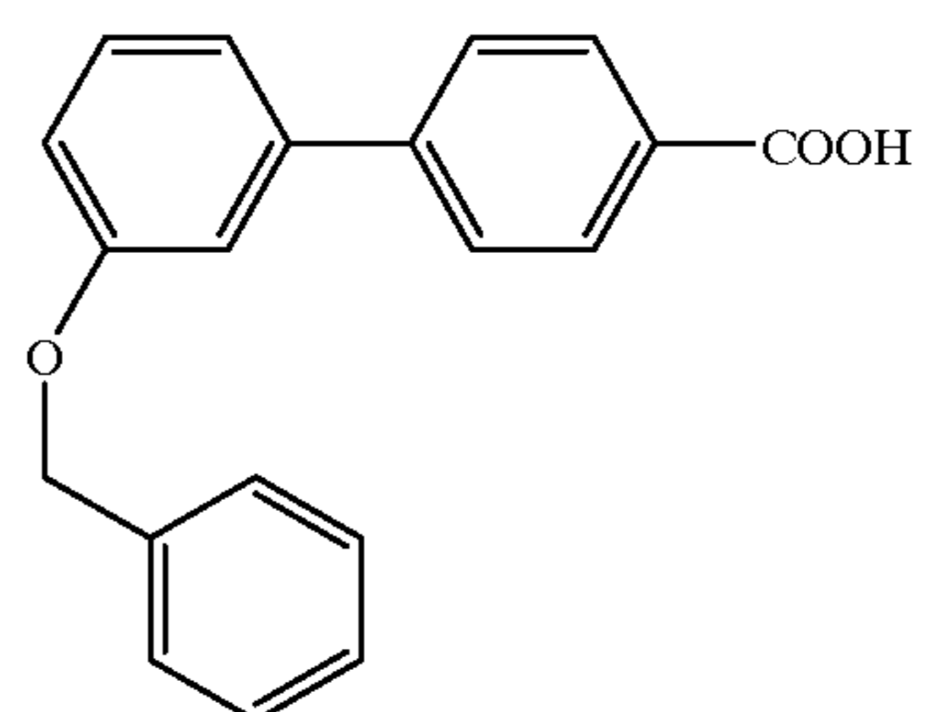
Compound 105
