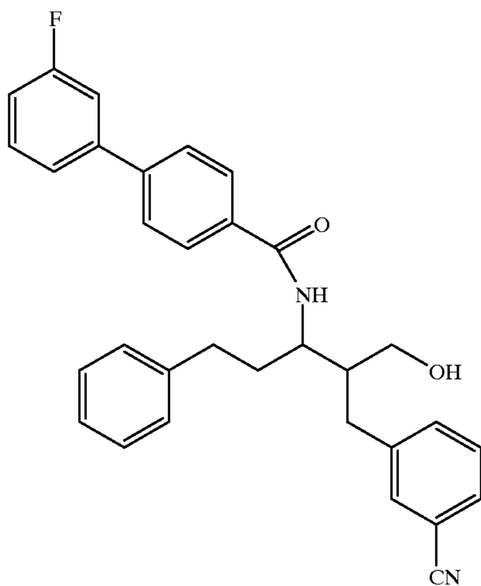
Compound 131
