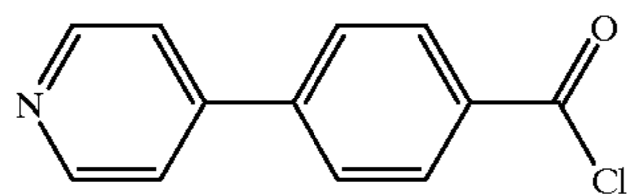
Compound 227
