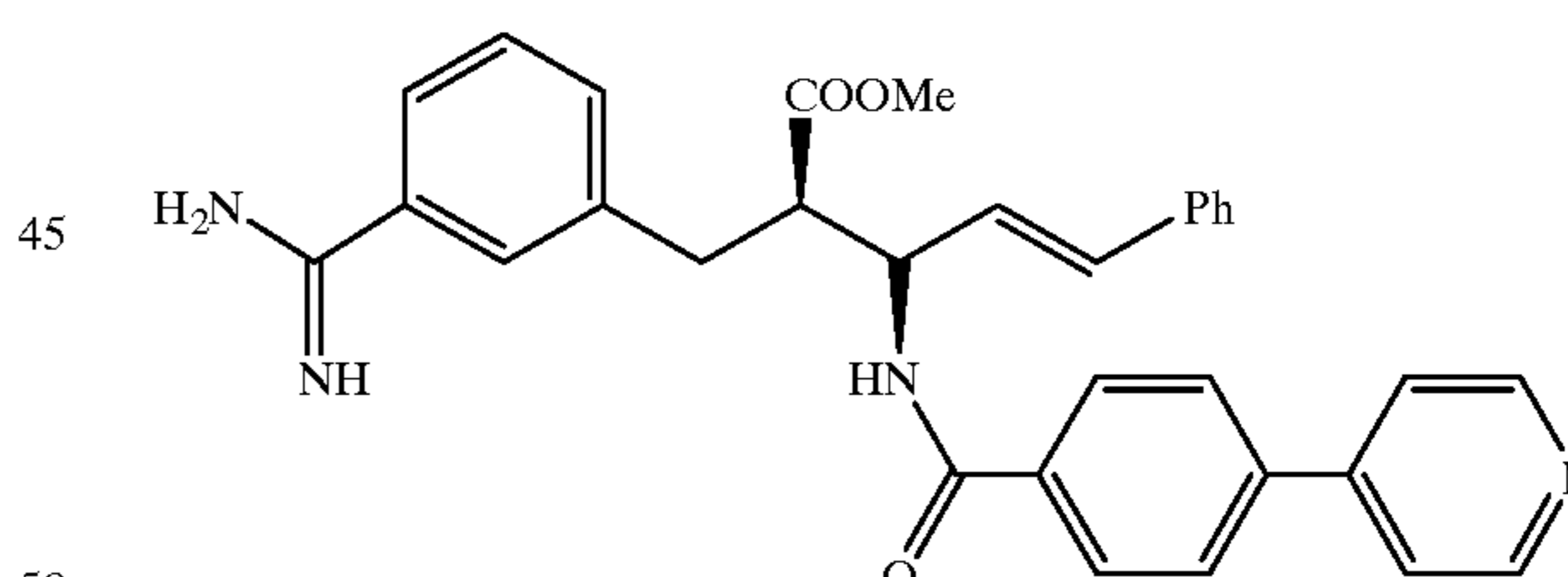
Compound 18
