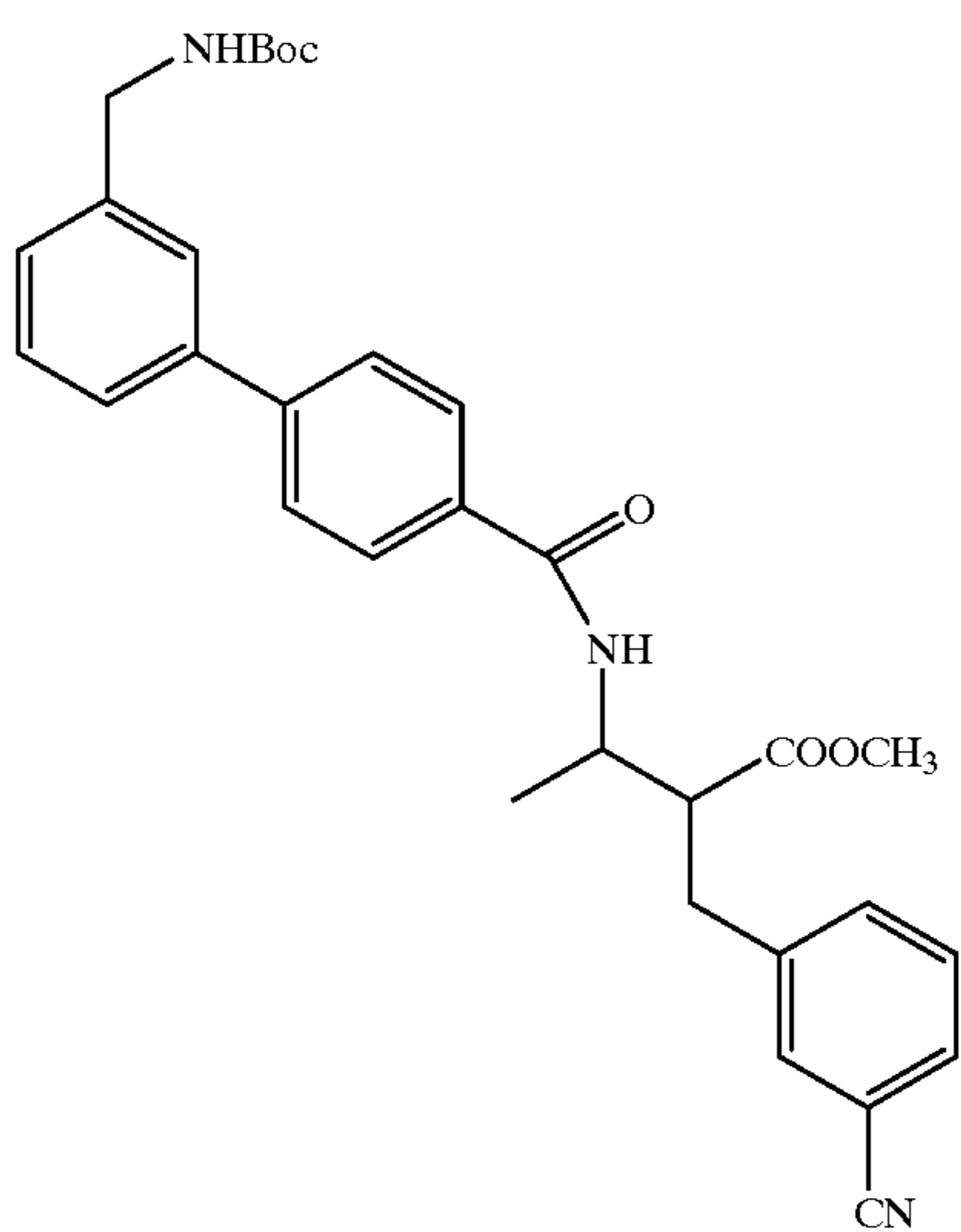
Compound 123
