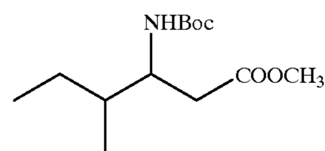
Compound 60
