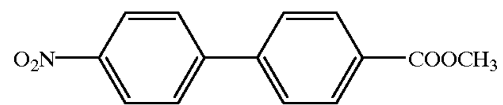
Compound 89
