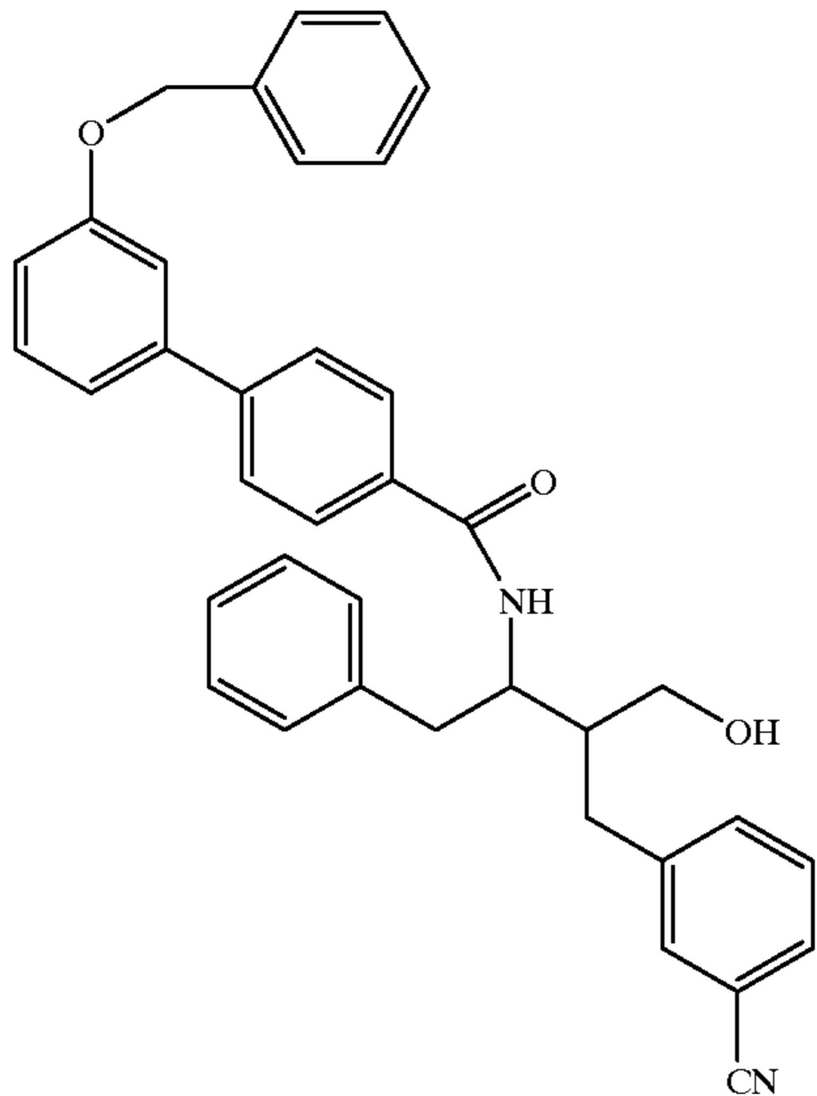
Compound 142
