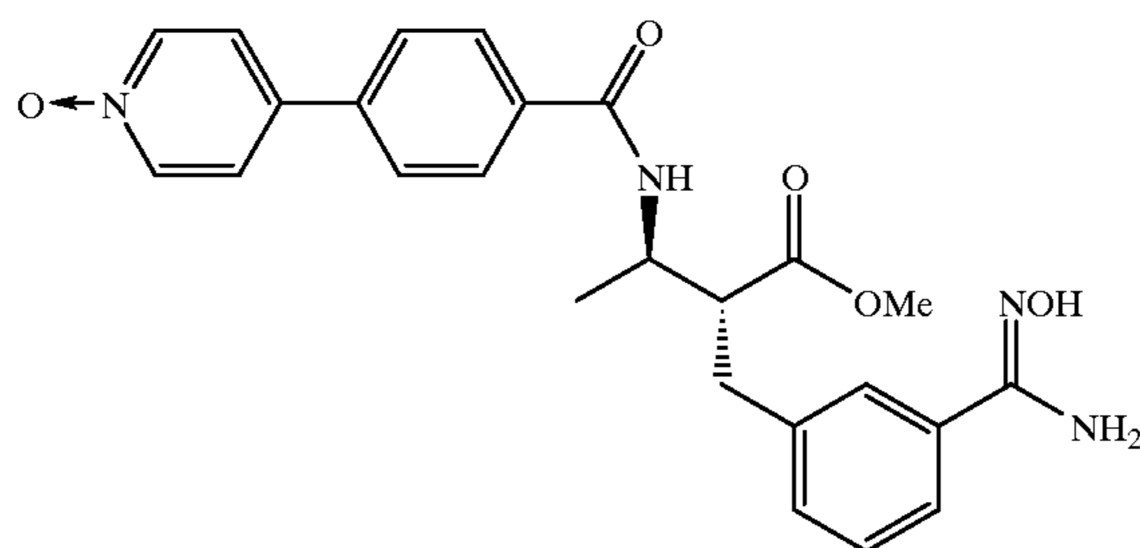
Compound 217
