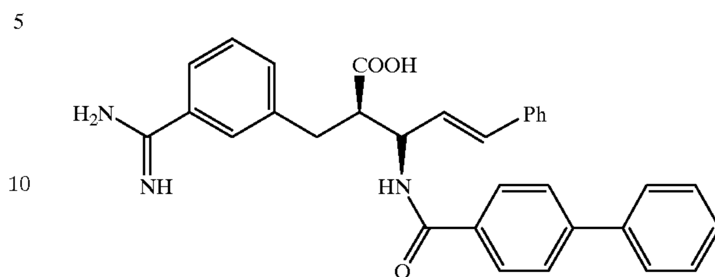
Compound 47
