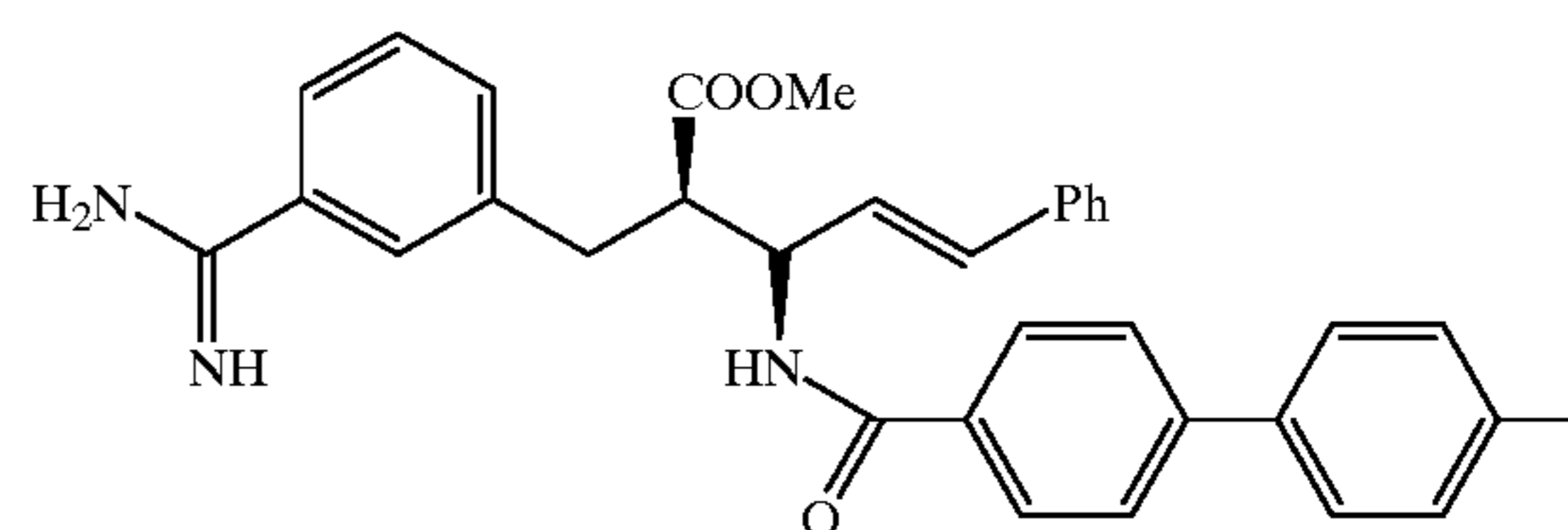
Compound 29
