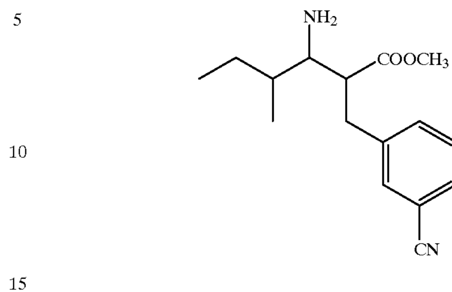
Compound 72
