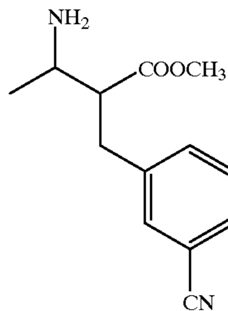
Compound 69
