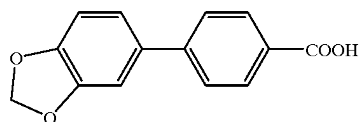
Compound 97
