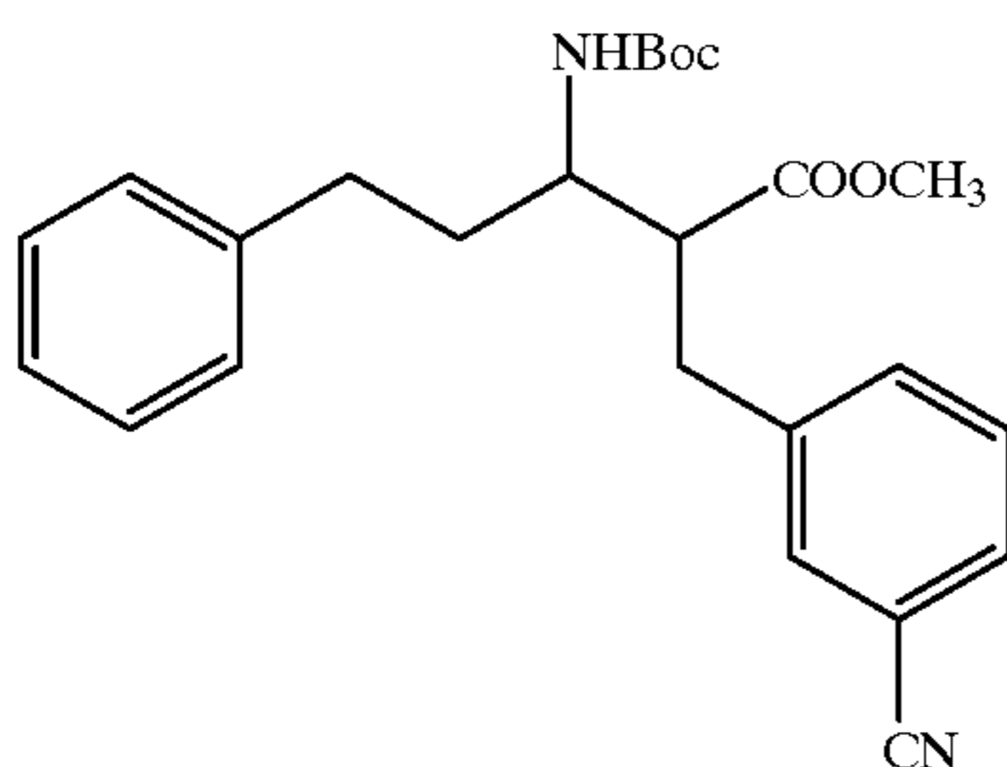
Compound 64
