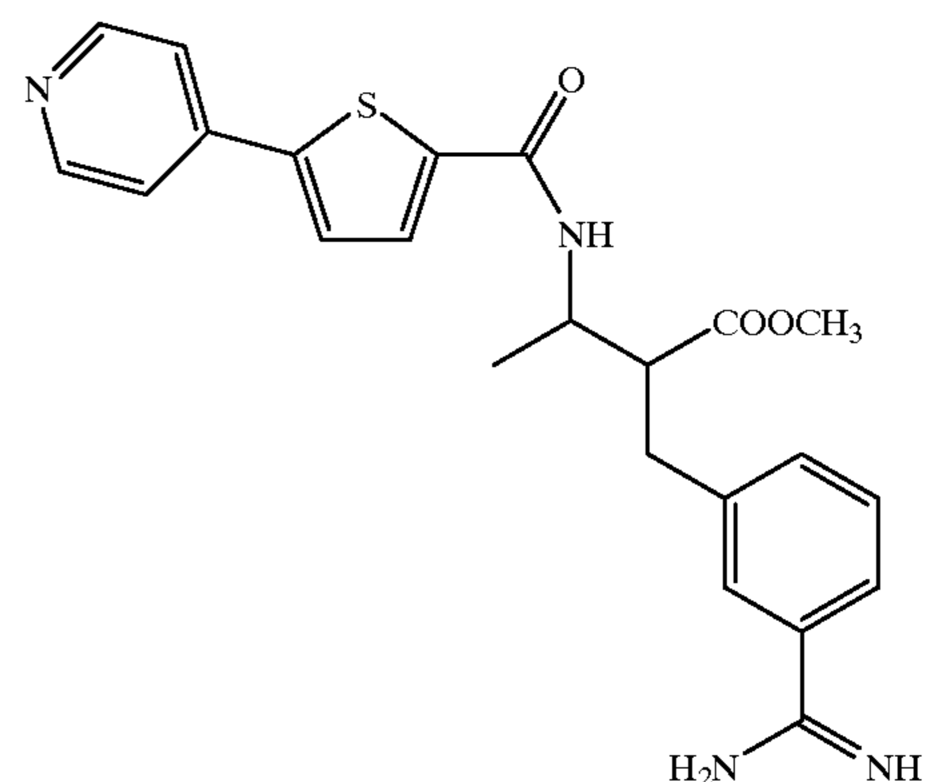
Compound 275
