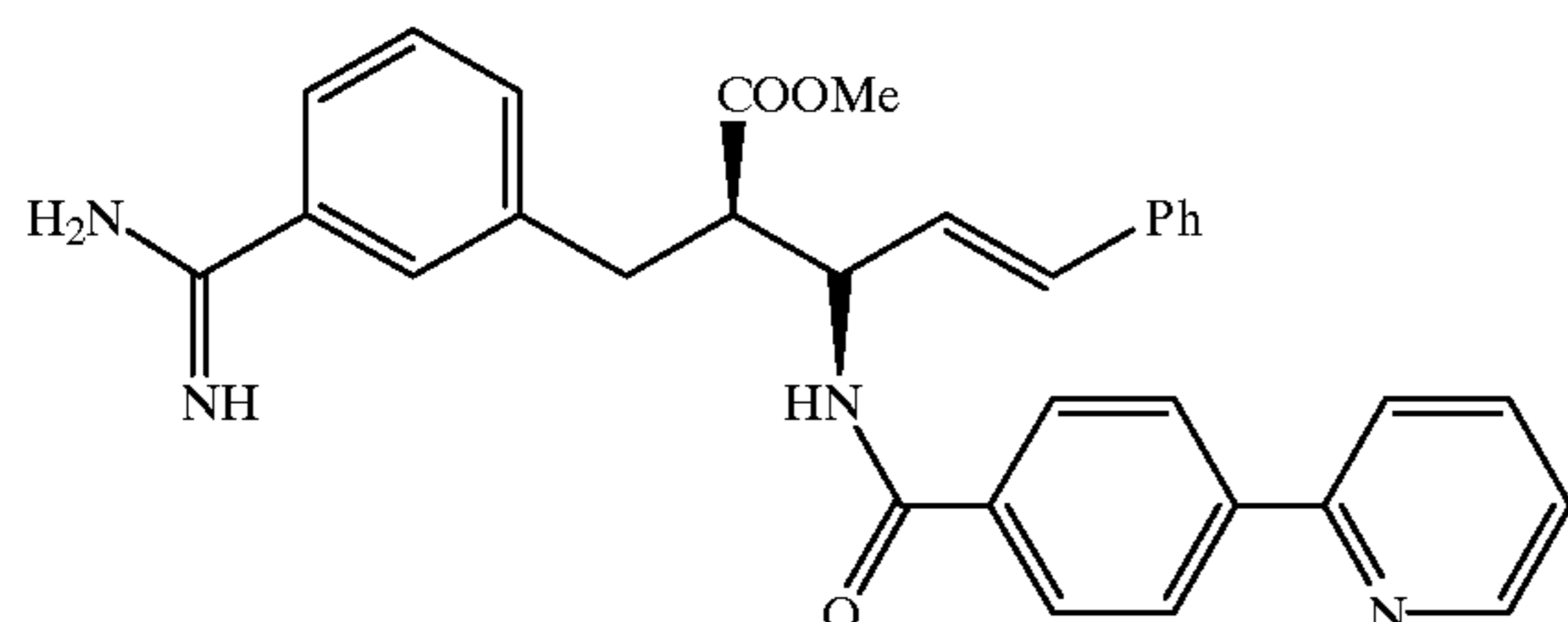
Compound 16
