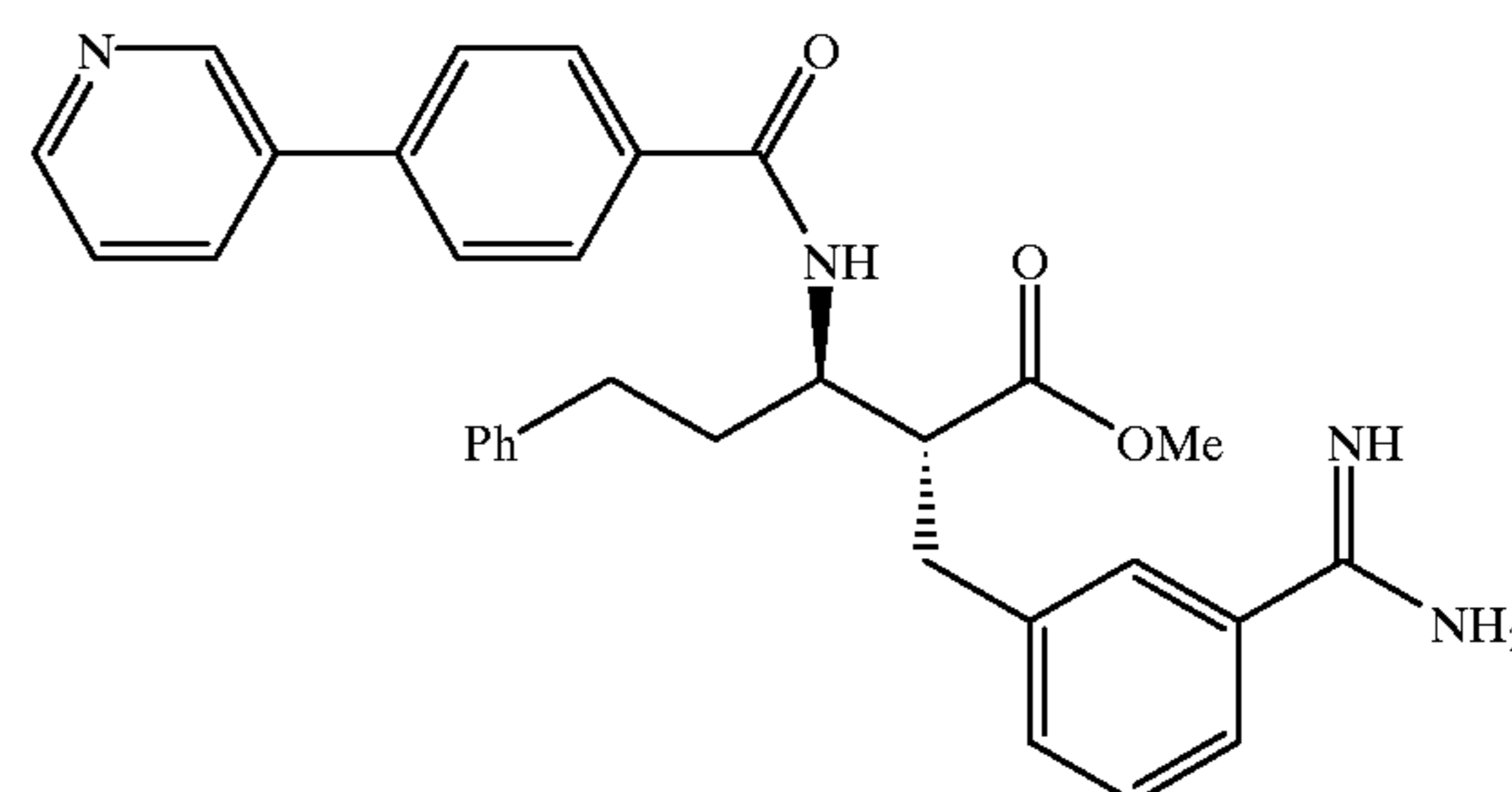
Compound 231
