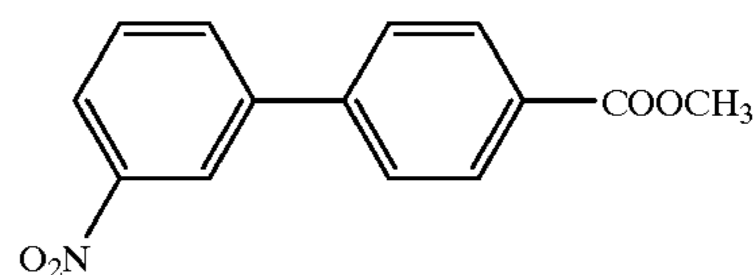
Compound 88
