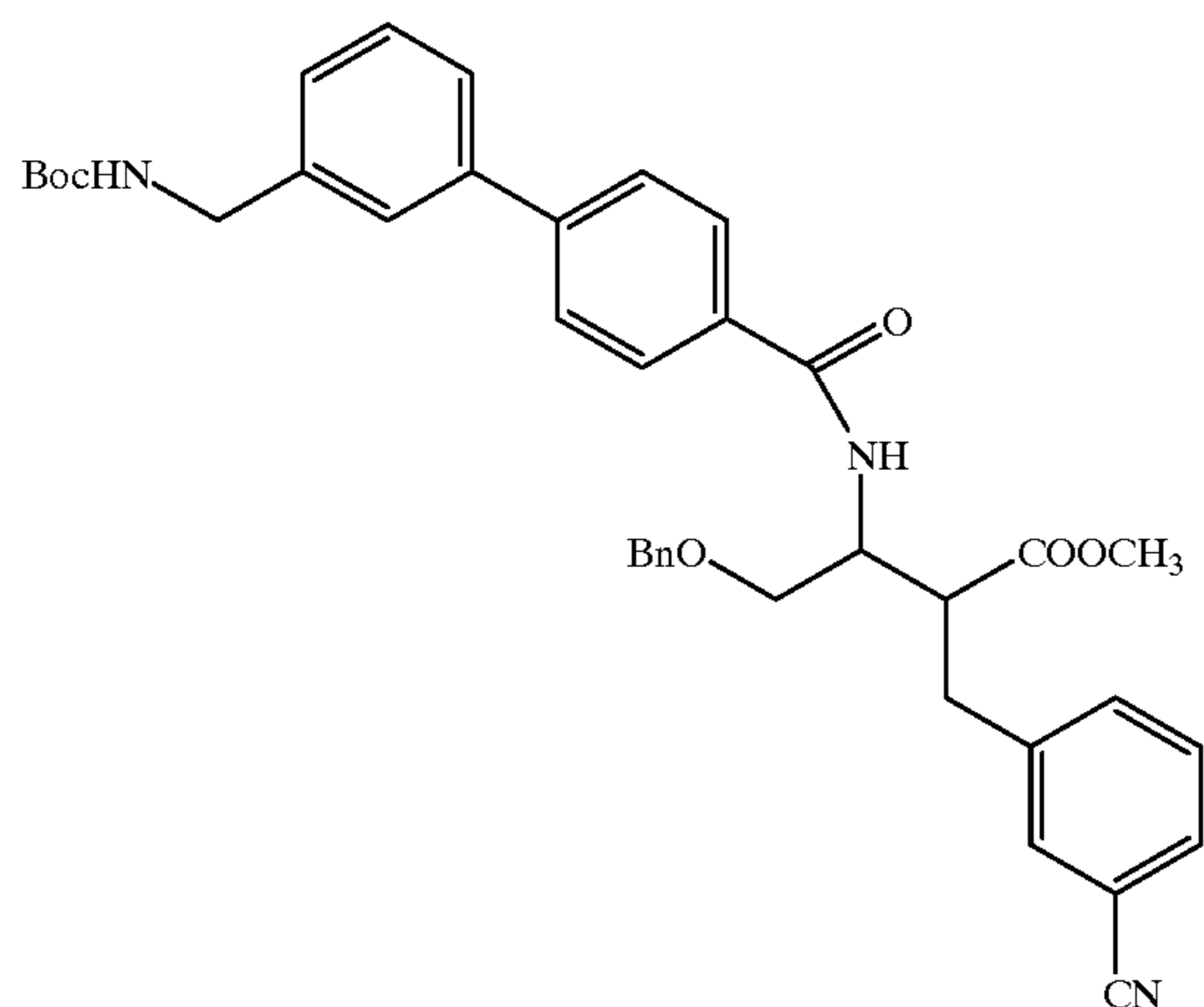
Compound 265
