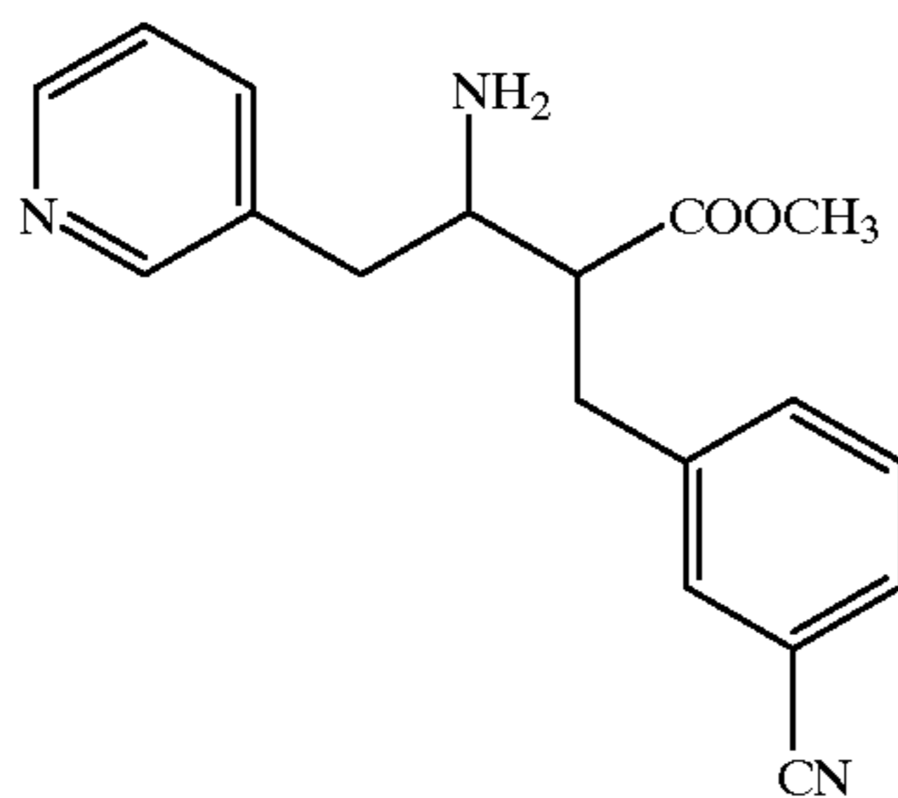
Compound 71
