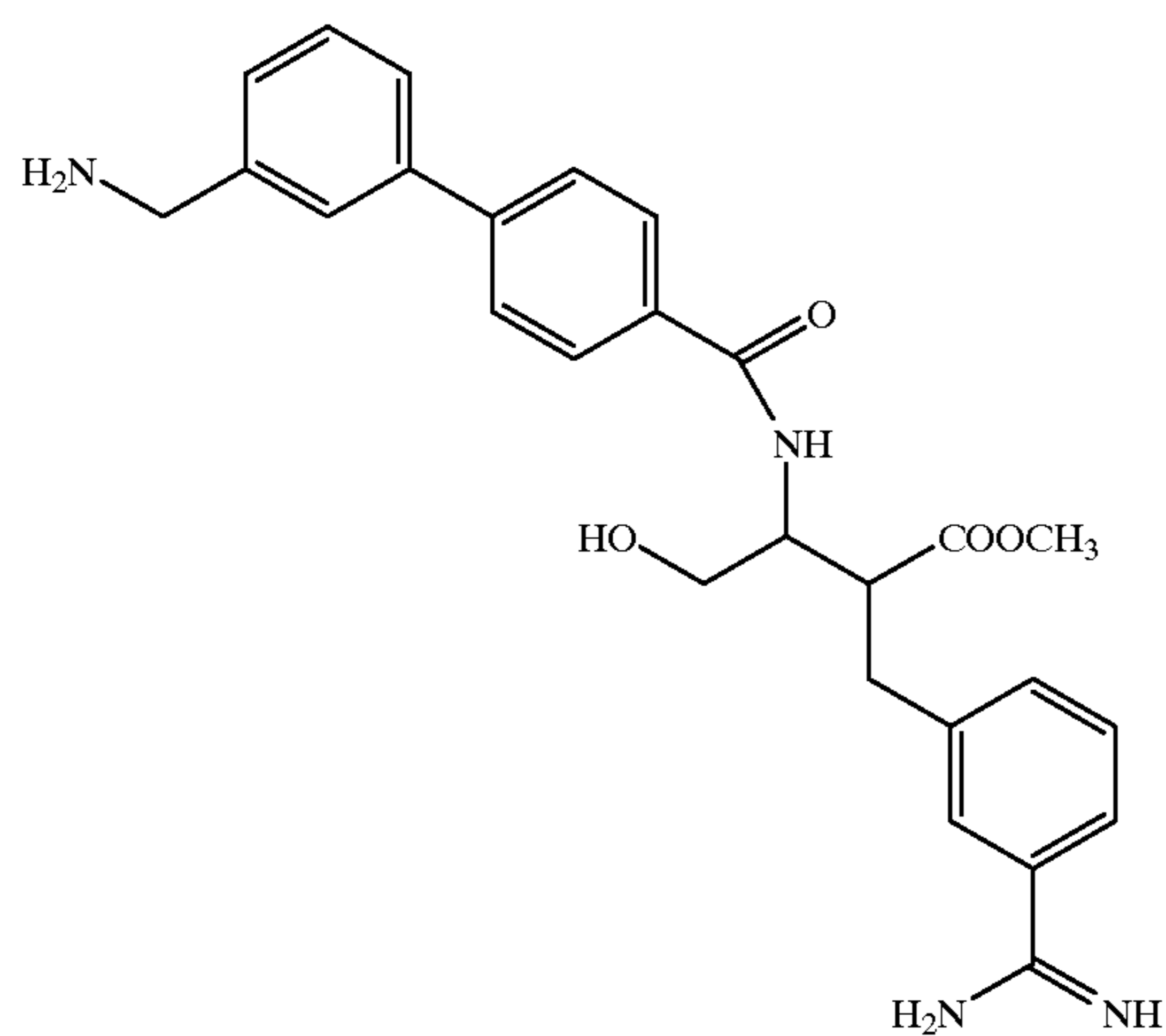
Compound 297
