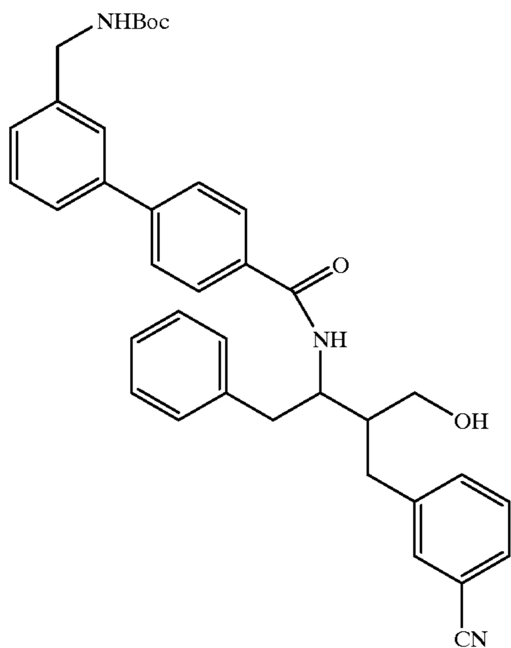
Compound 135
