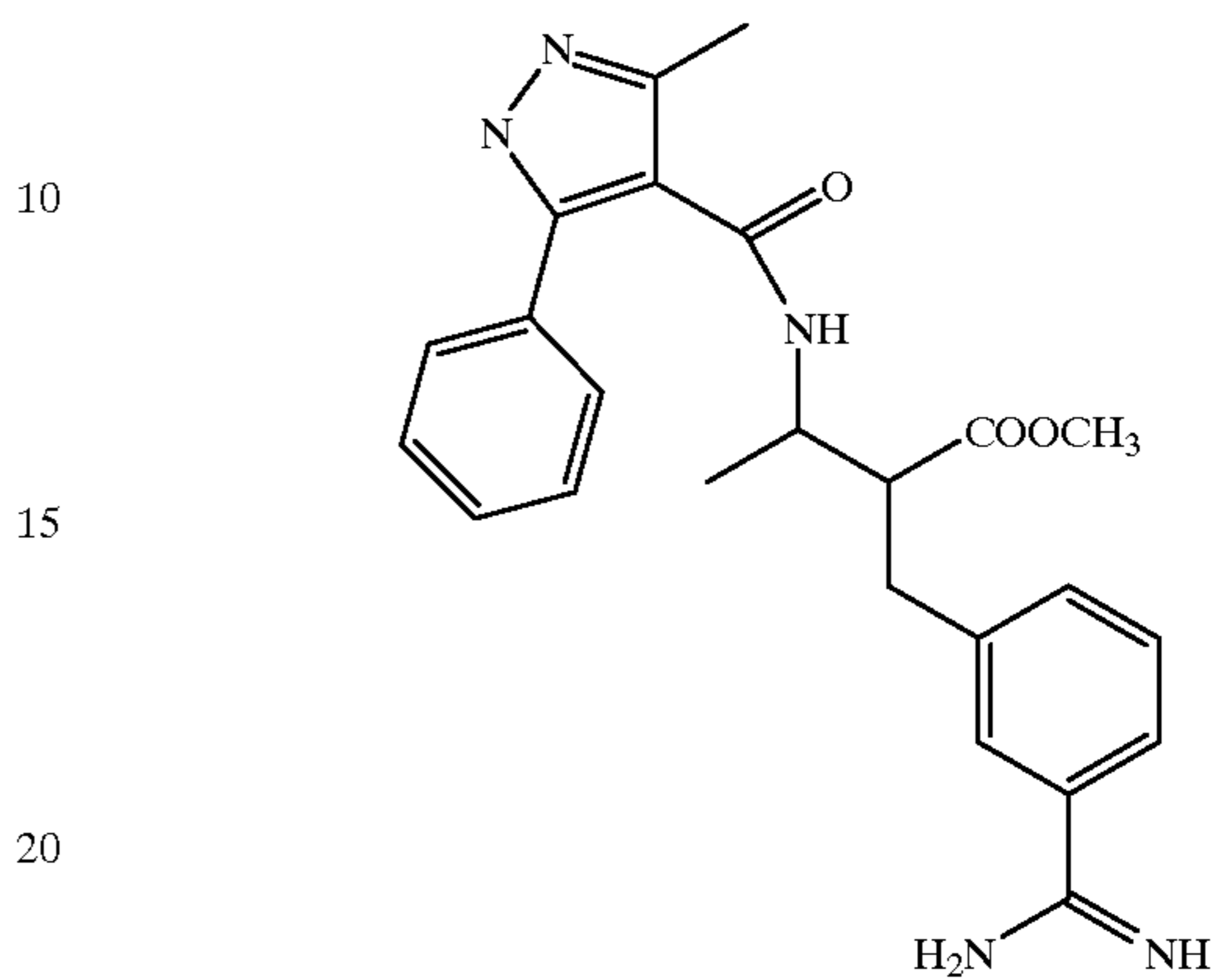
Compound 290
