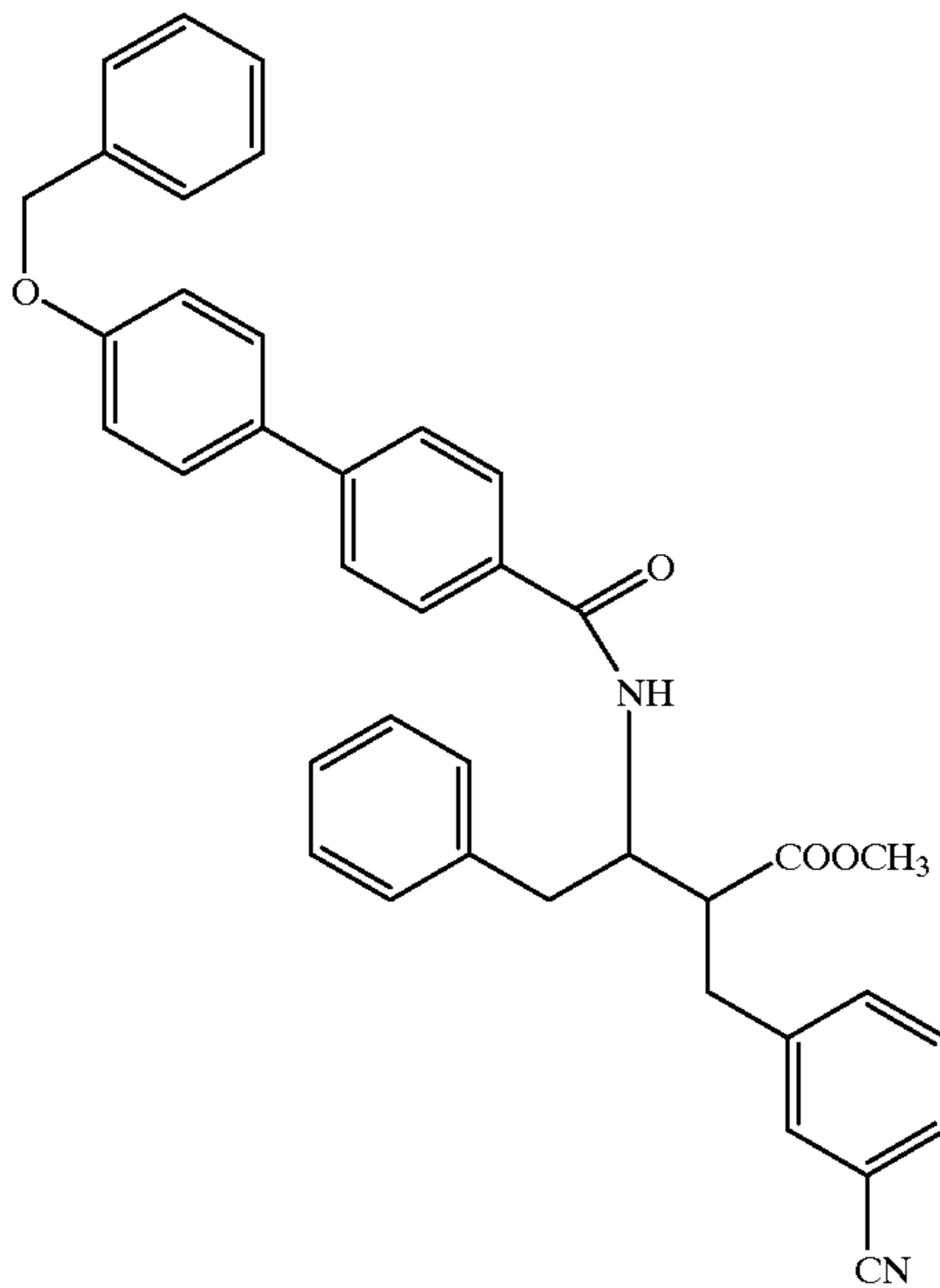
Compound 122
