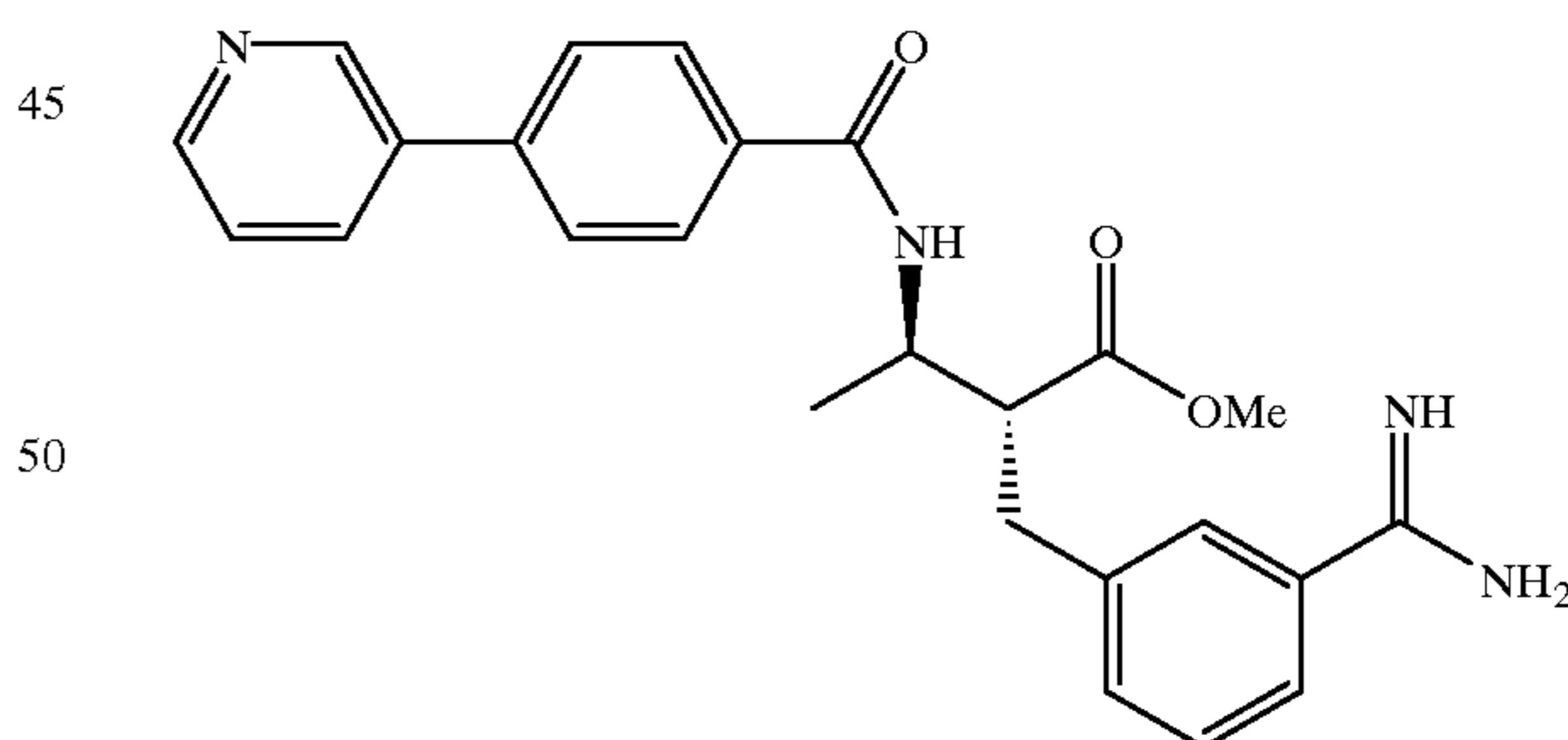
Compound 210
