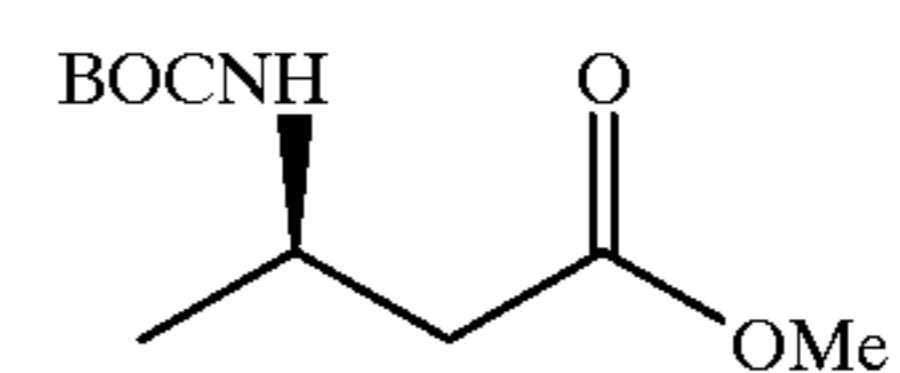
Compound 197
