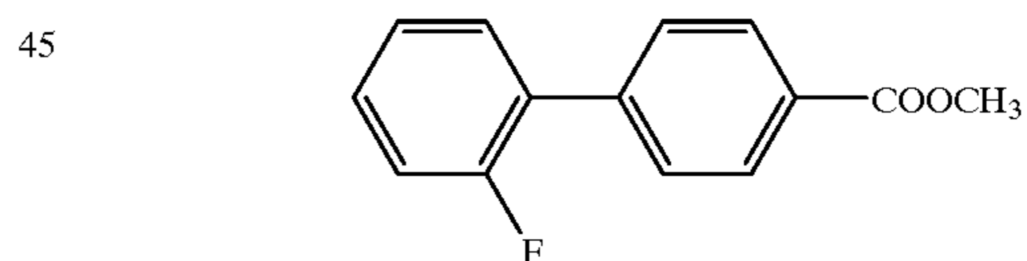
Compound 74
