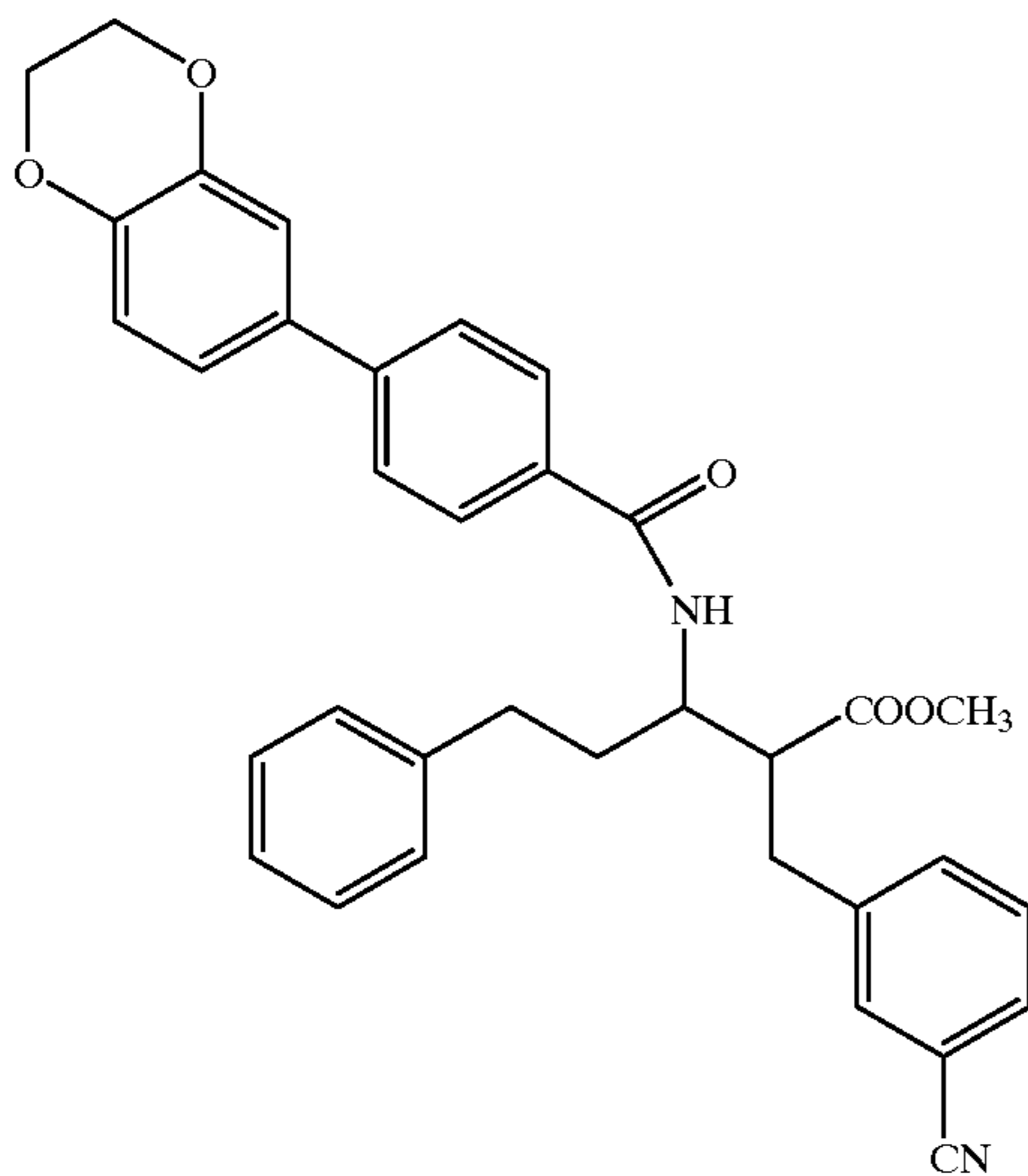
Compound 107
