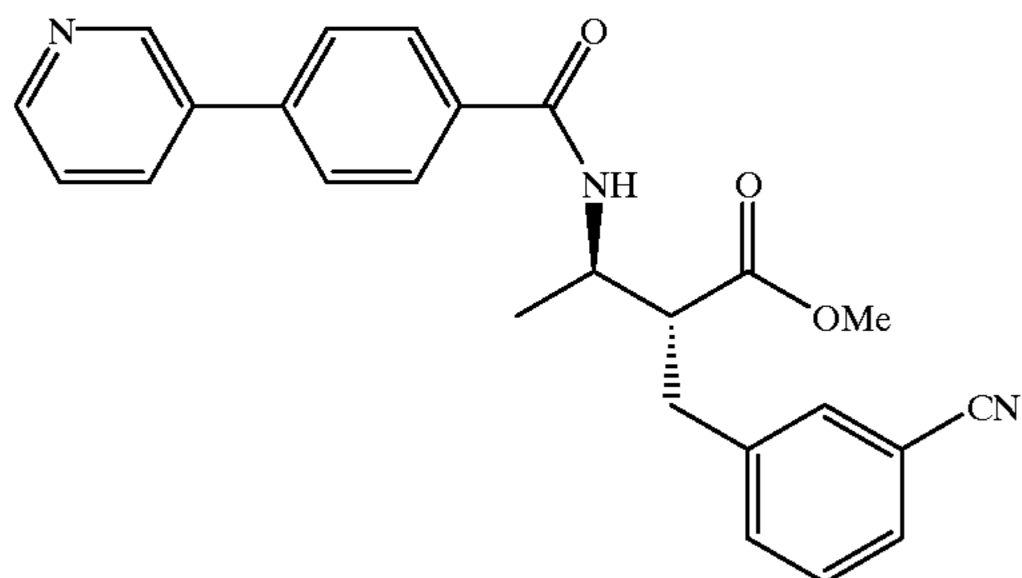
Compound 203
