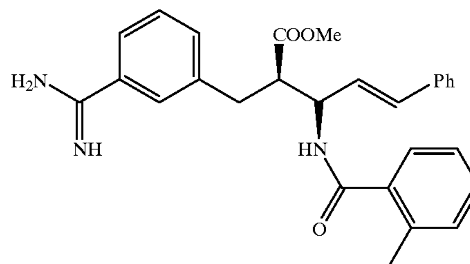
Compound 12
