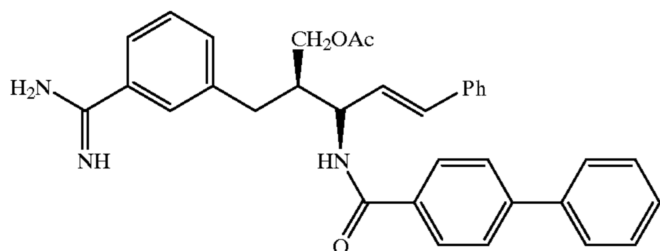
Compound 46
