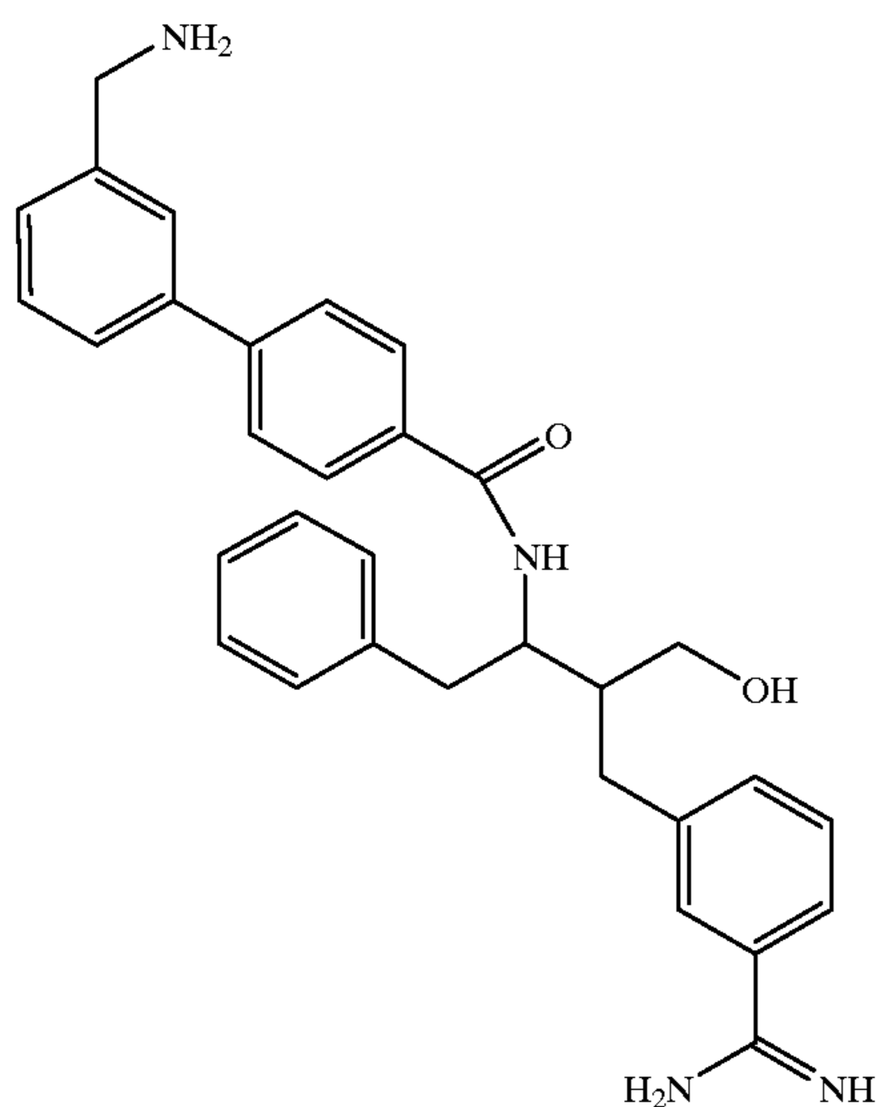
Compound 171
