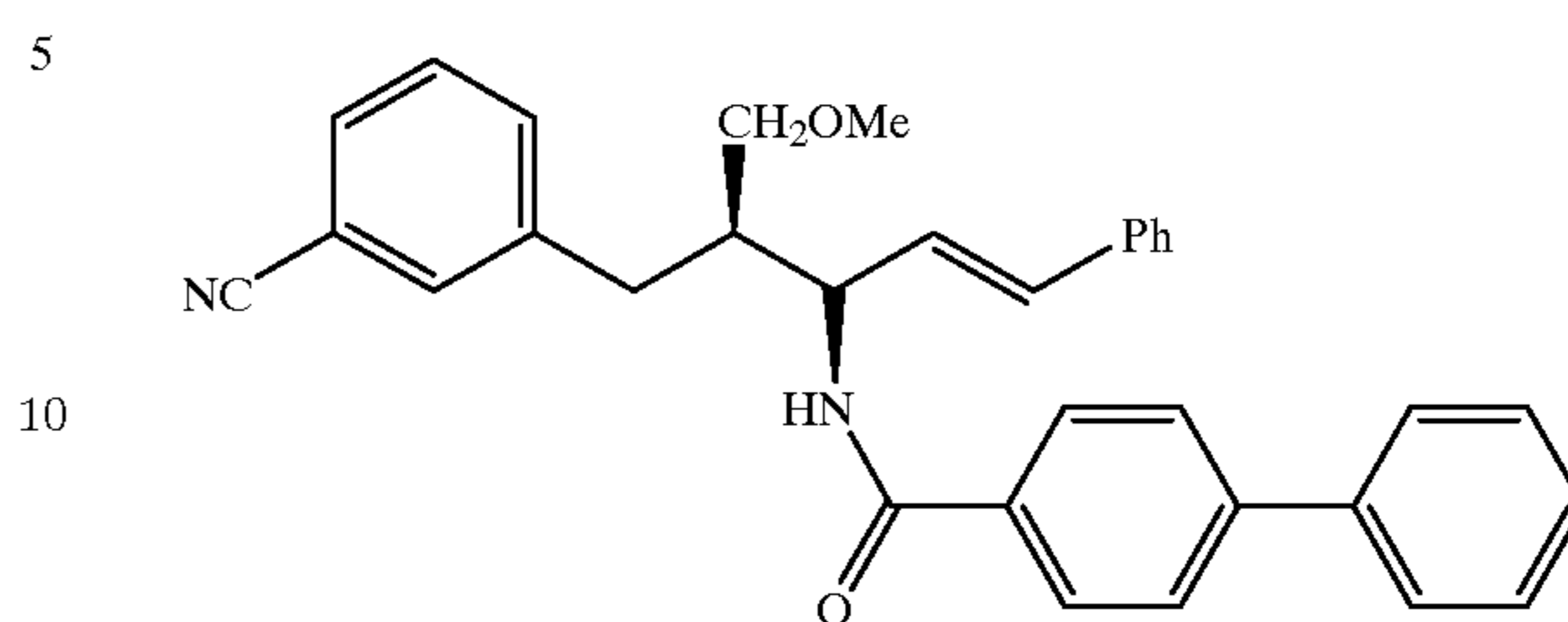
Compound 43
