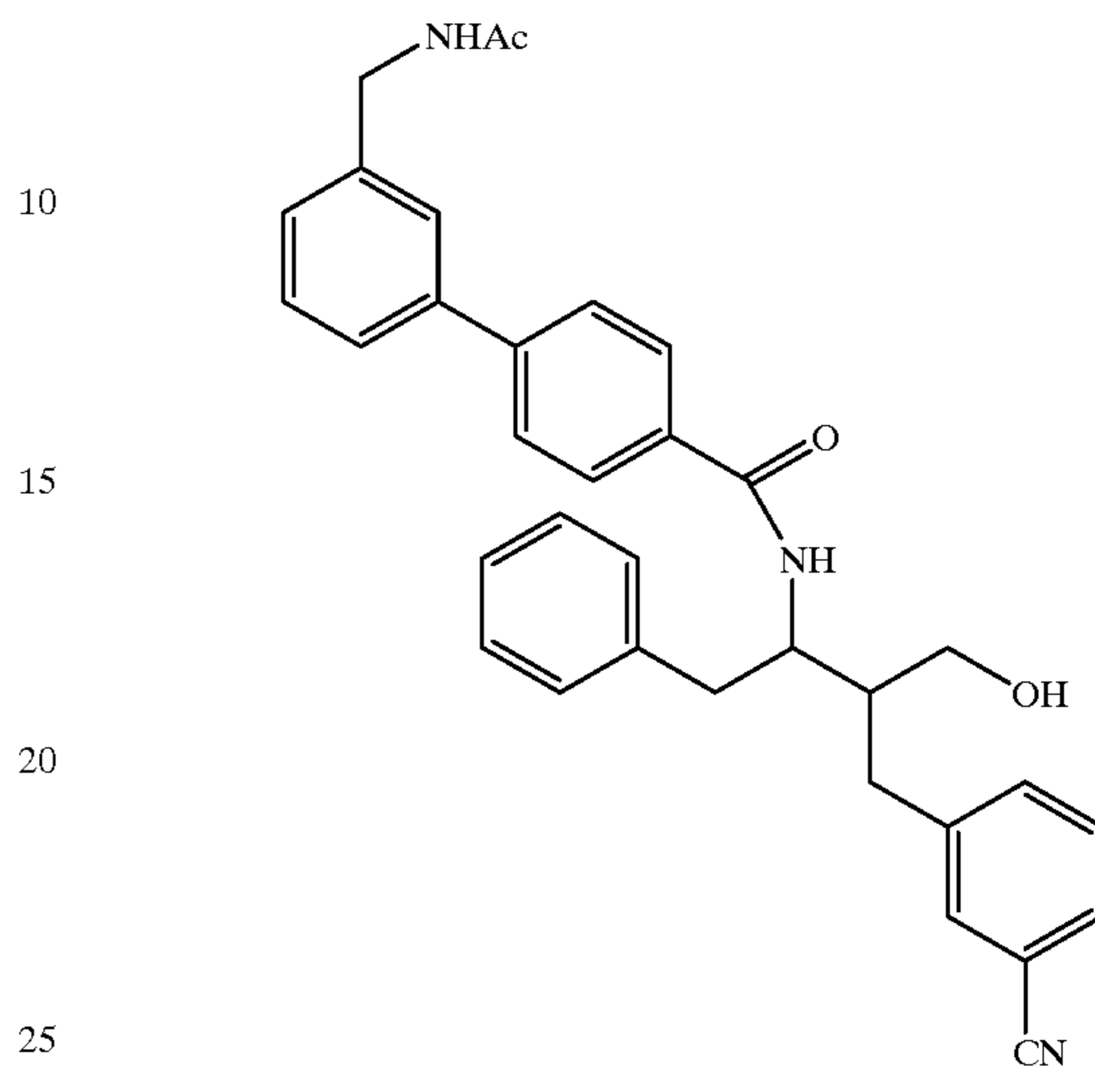
Compound 136
