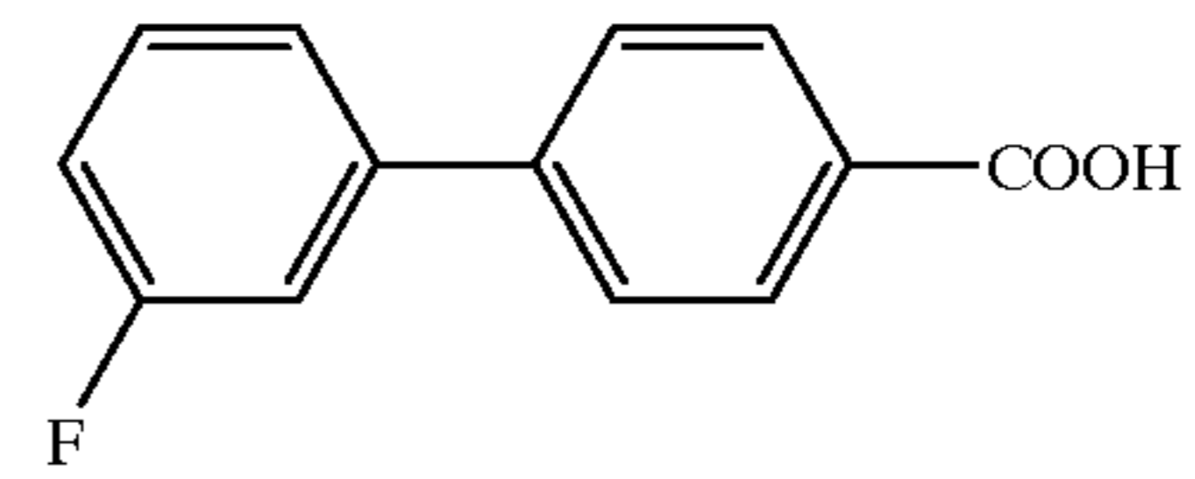
Compound 94
