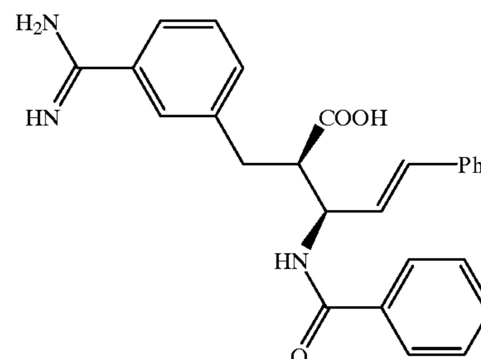
Compound 49
