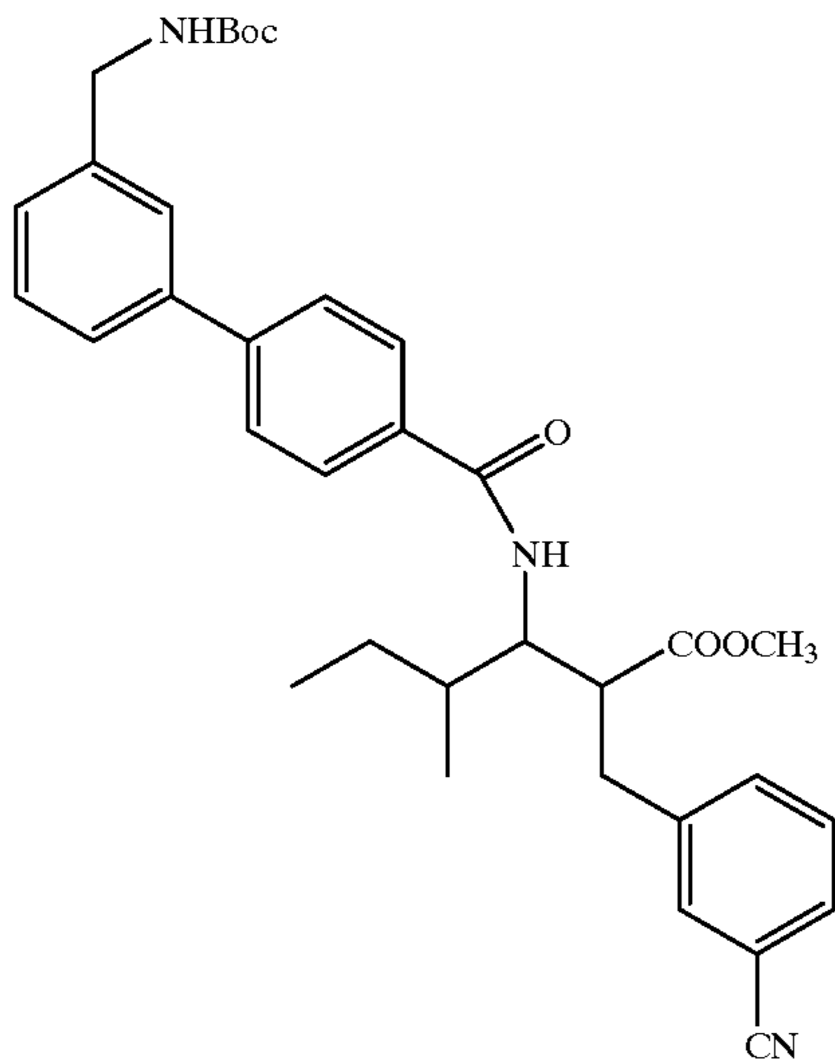
Compound 126
