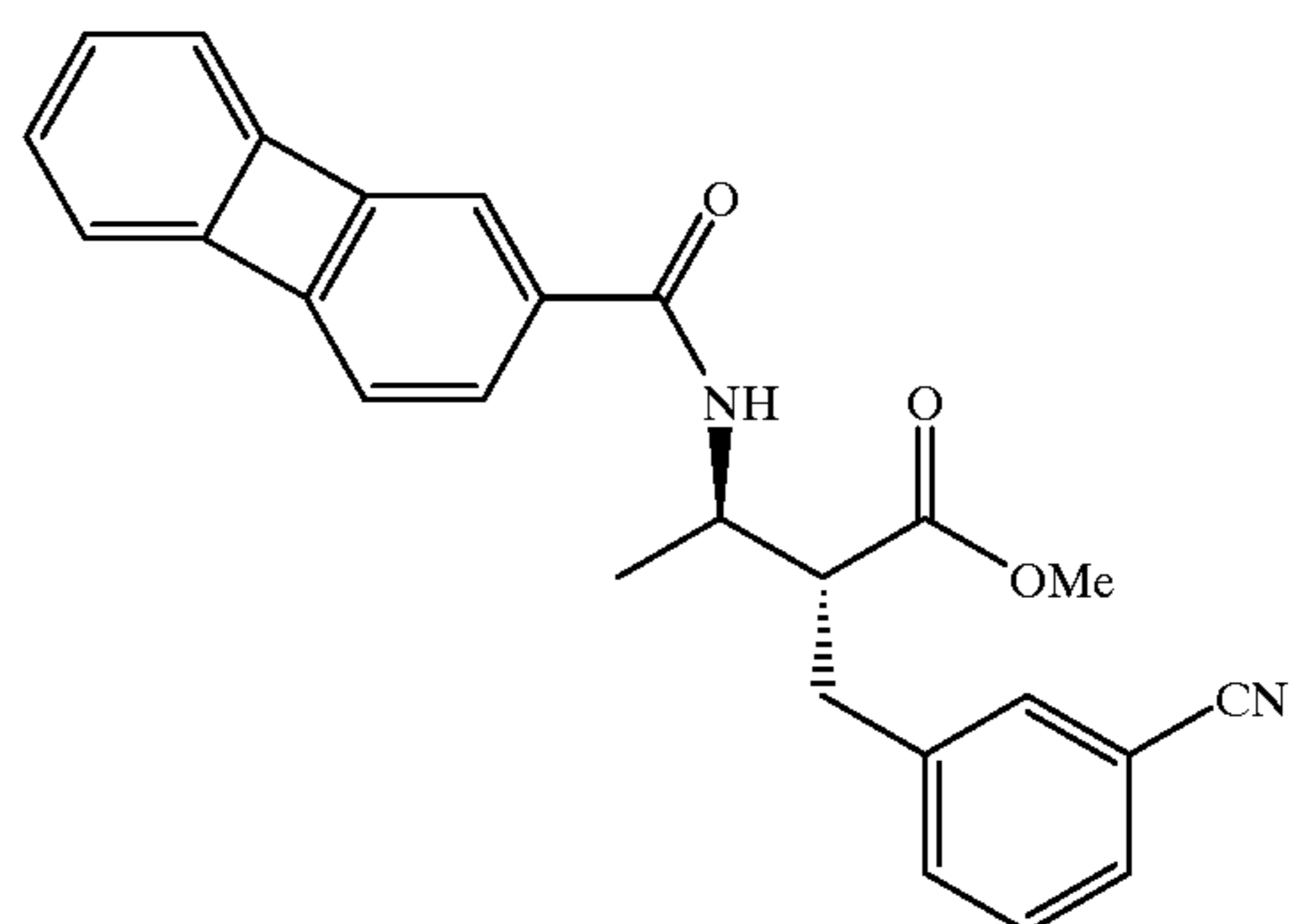
Compound 206
