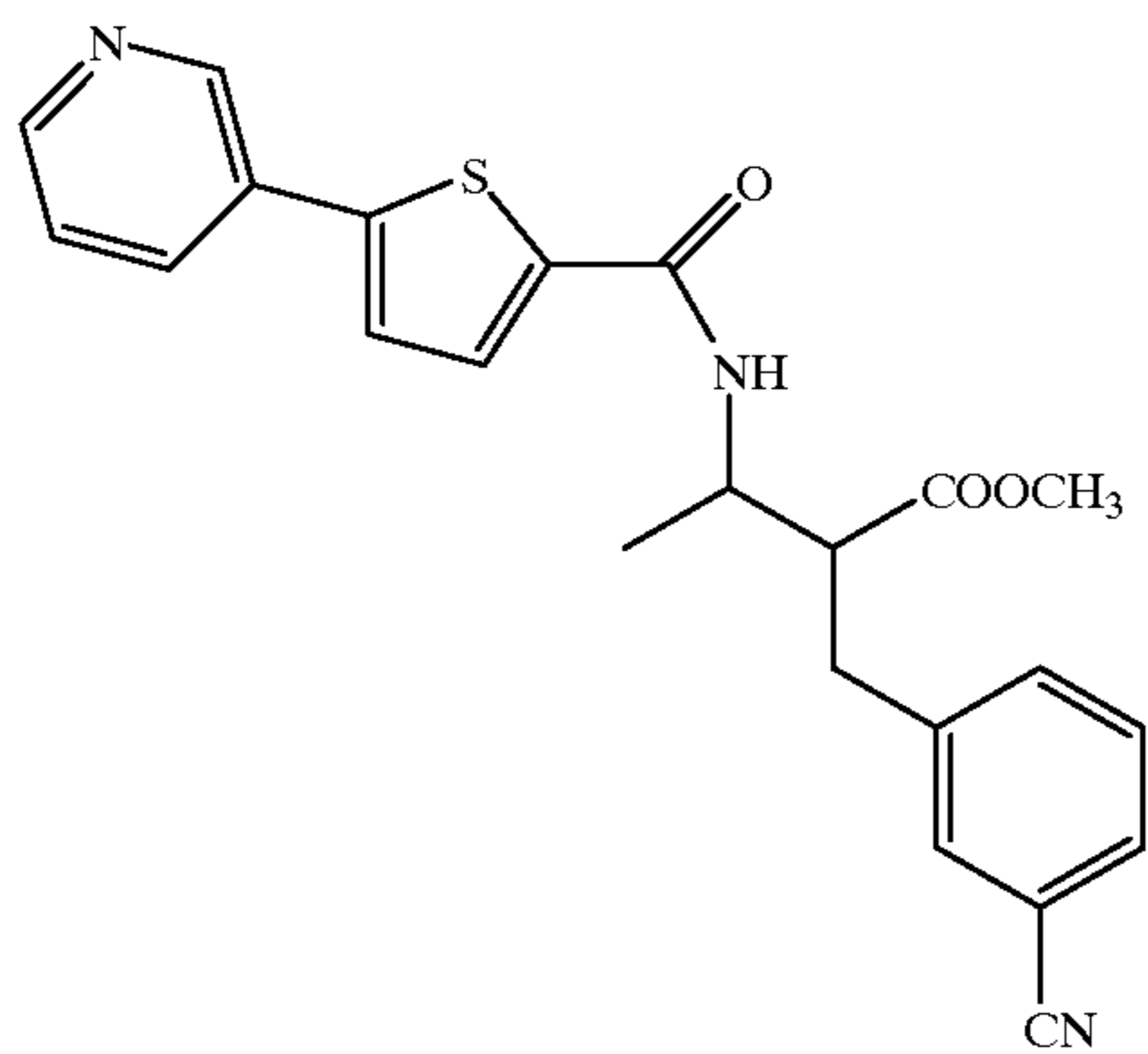
Compound 242
