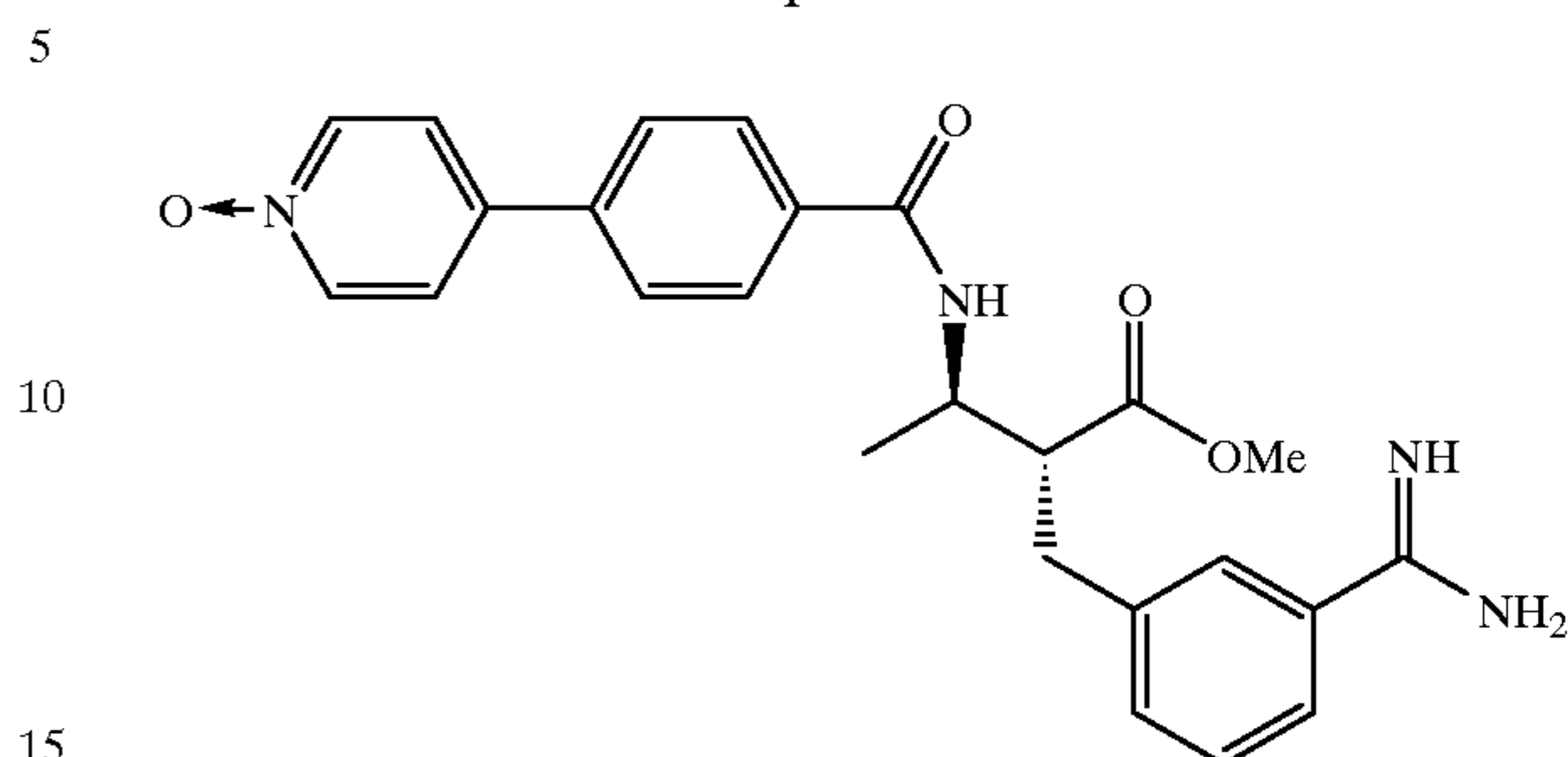
Compound 209
