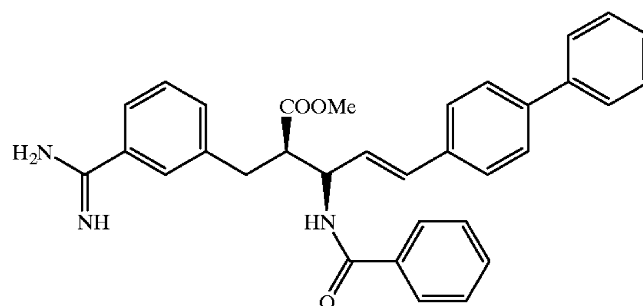
Compound 39
