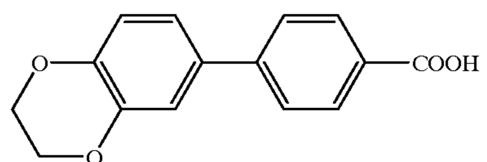
Compound 96
