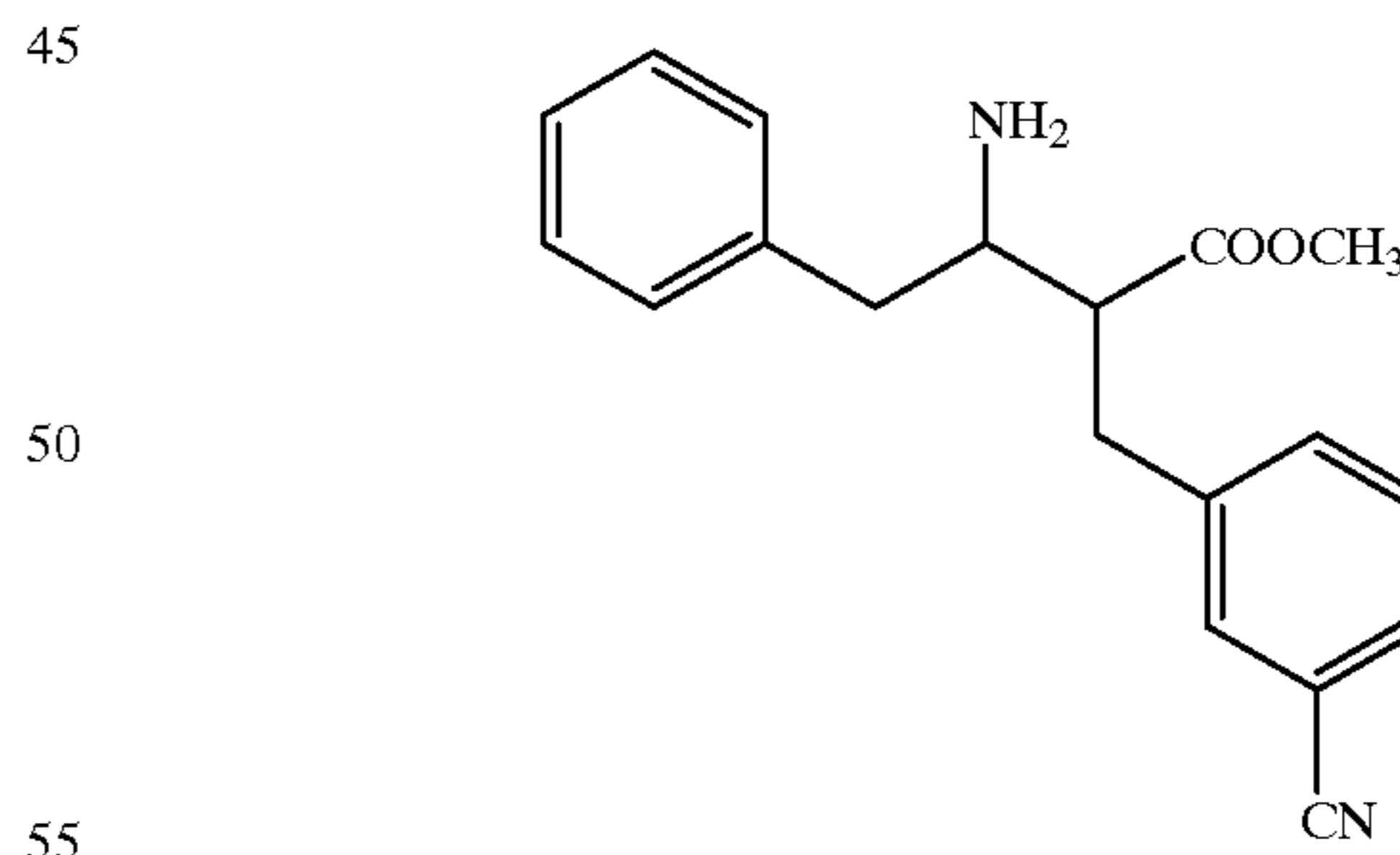
Compound 68
