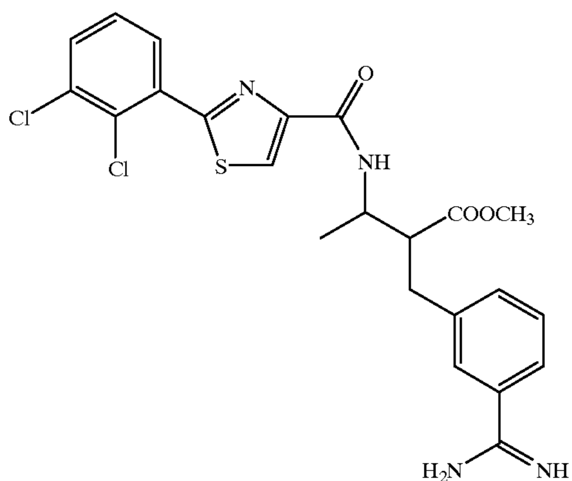
Compound 289
