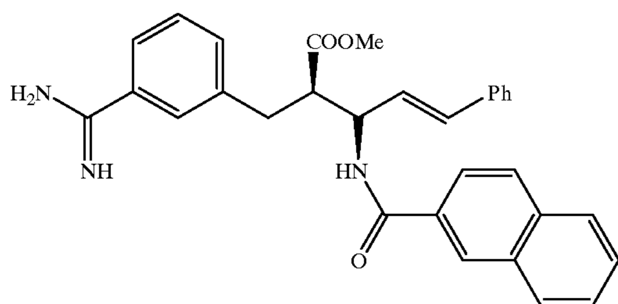
Compound 23
