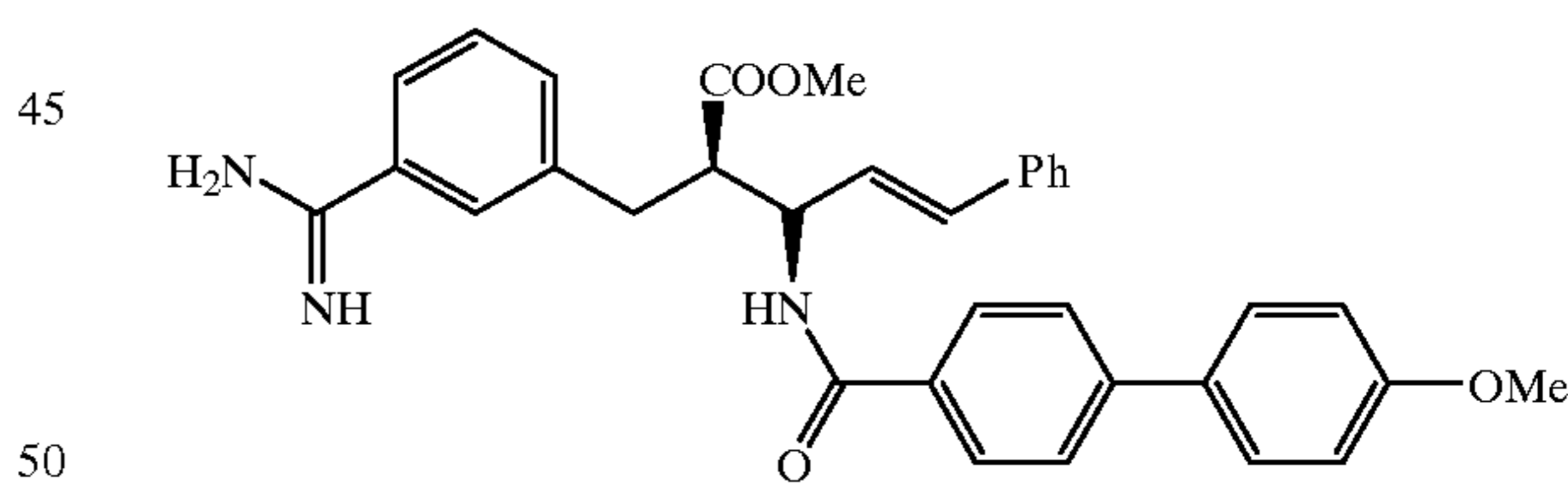
Compound 26
