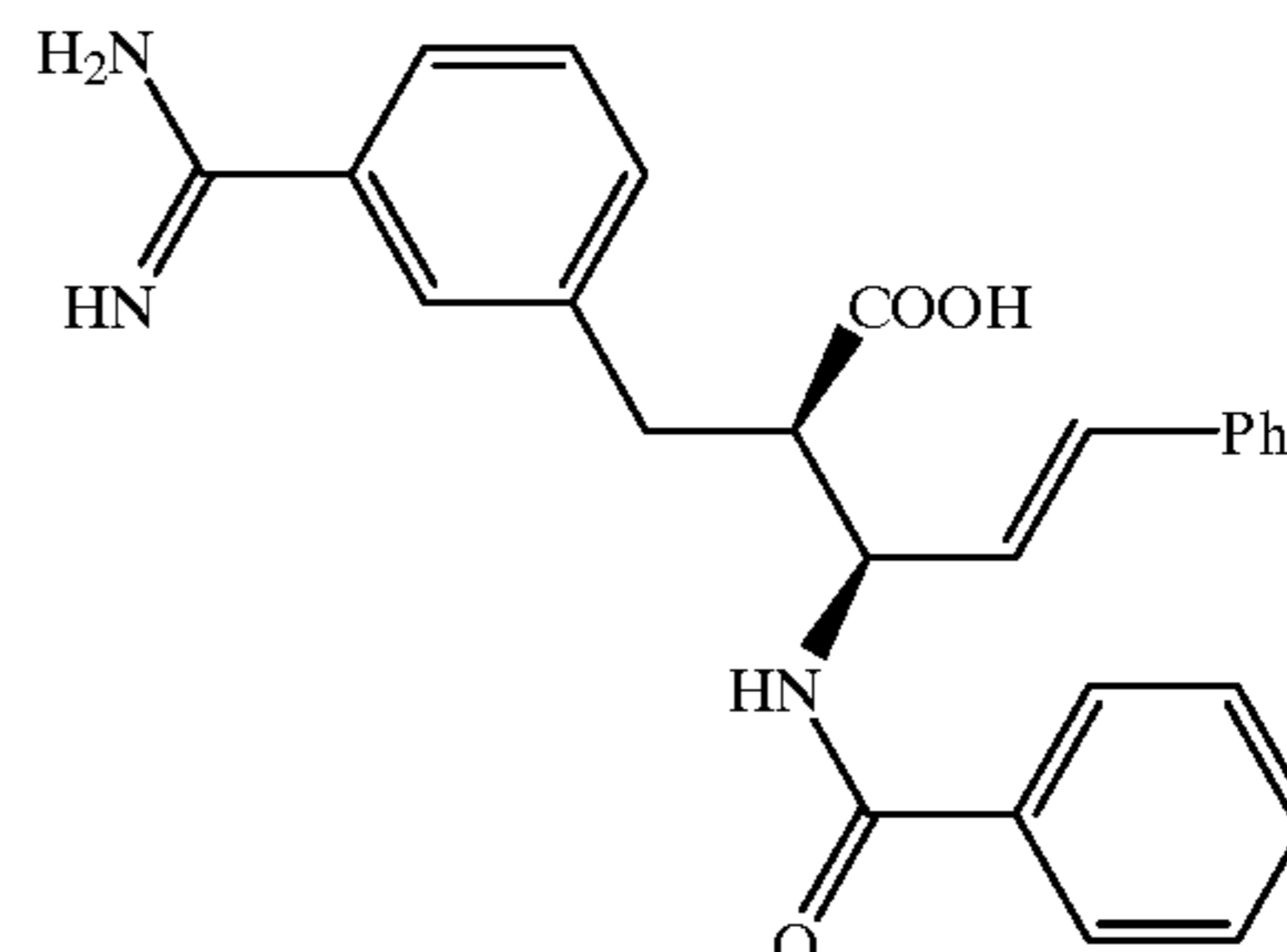
Compound 49
