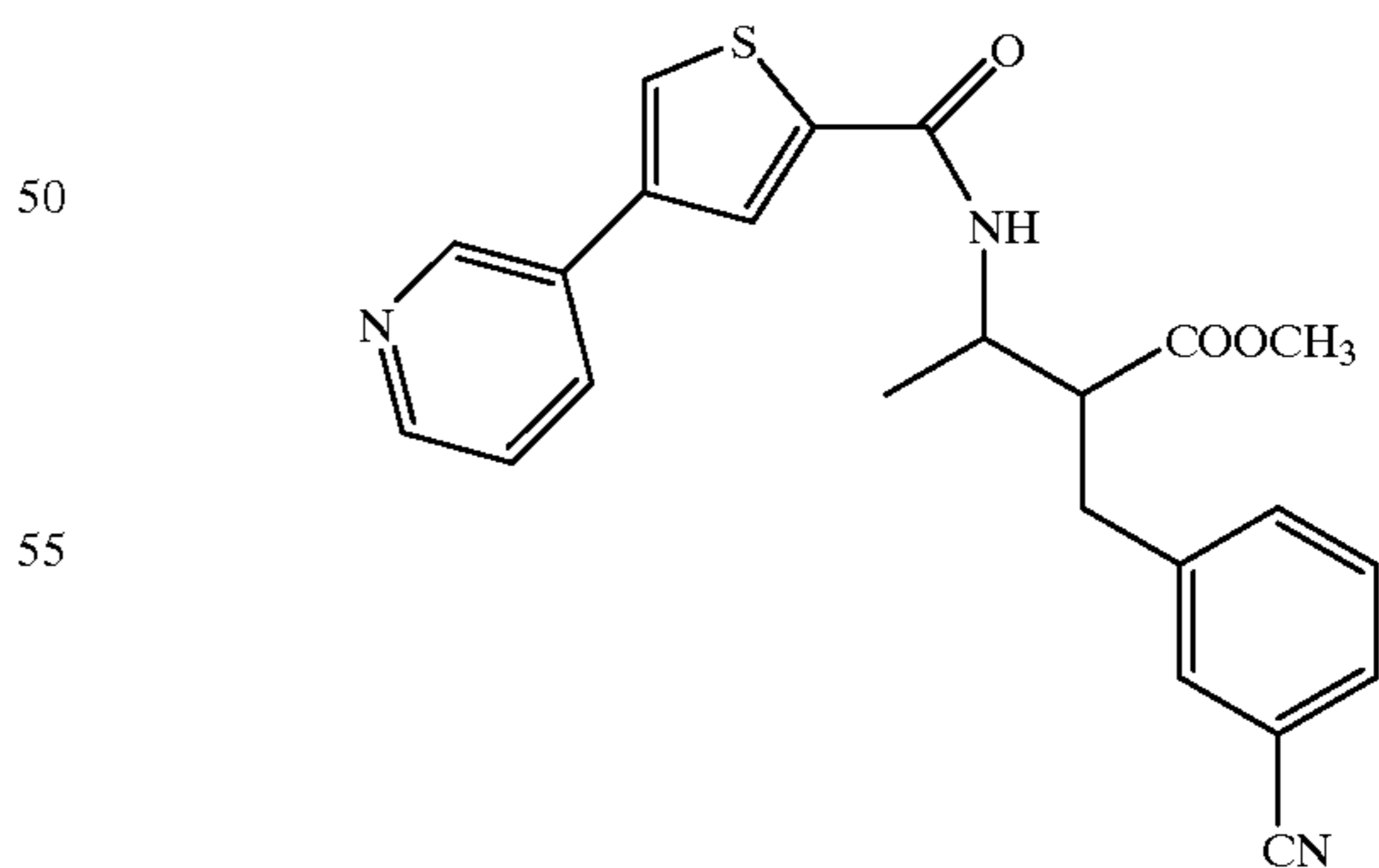
Compound 245
