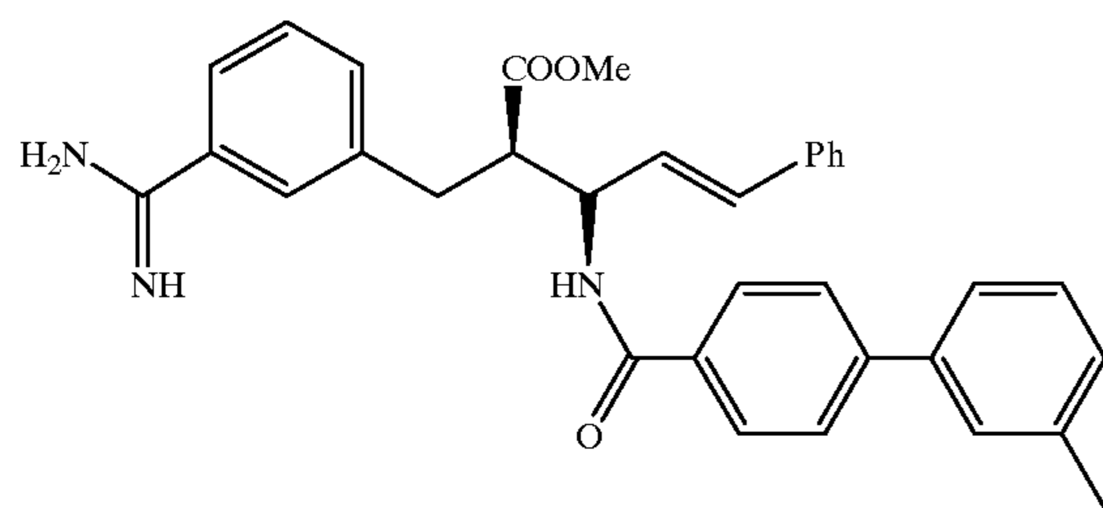
Compound 20
