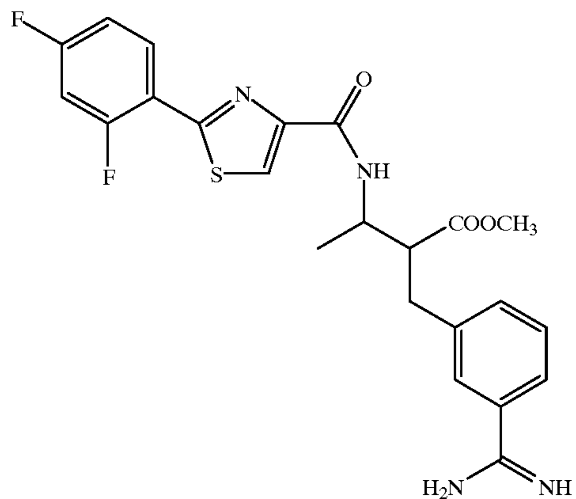
Compound 288
