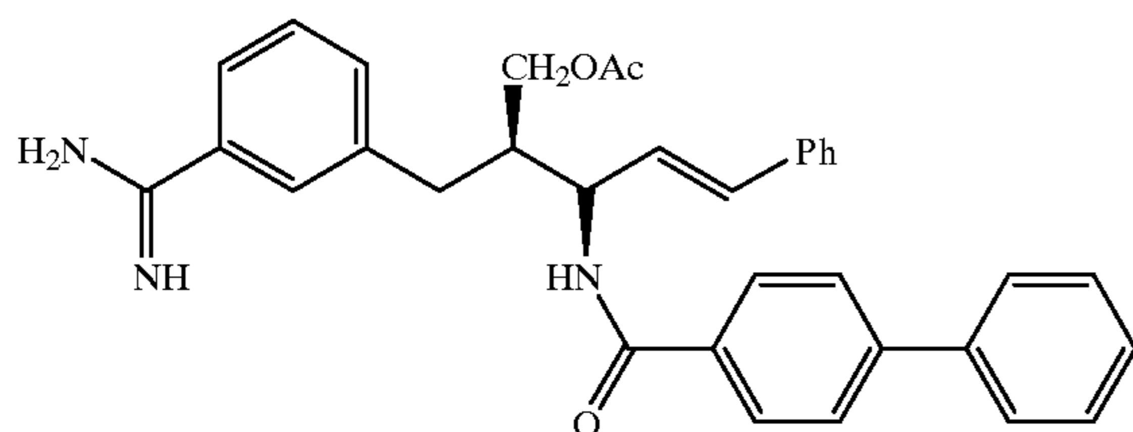
Compound 46
