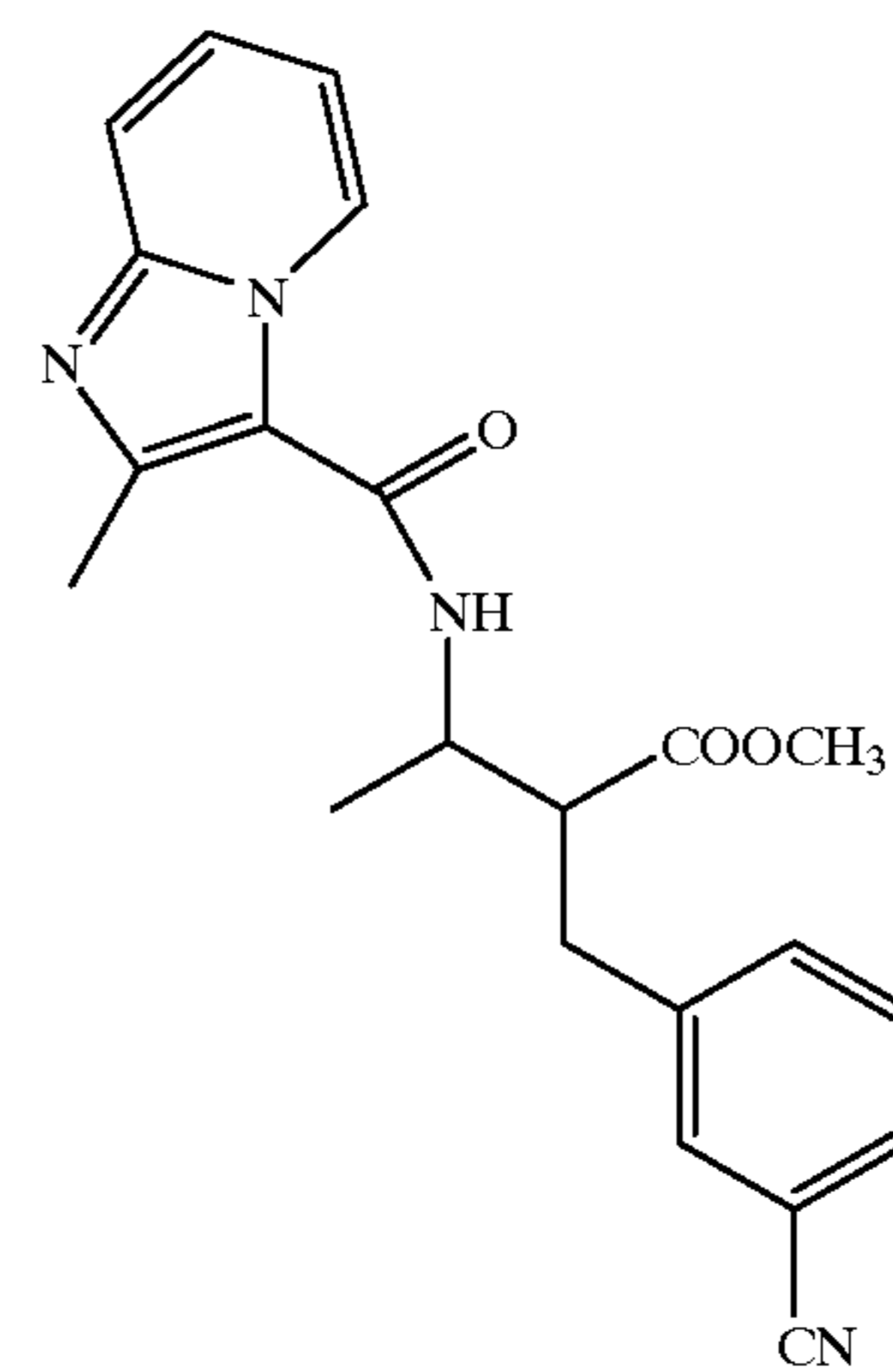
Compound 261
