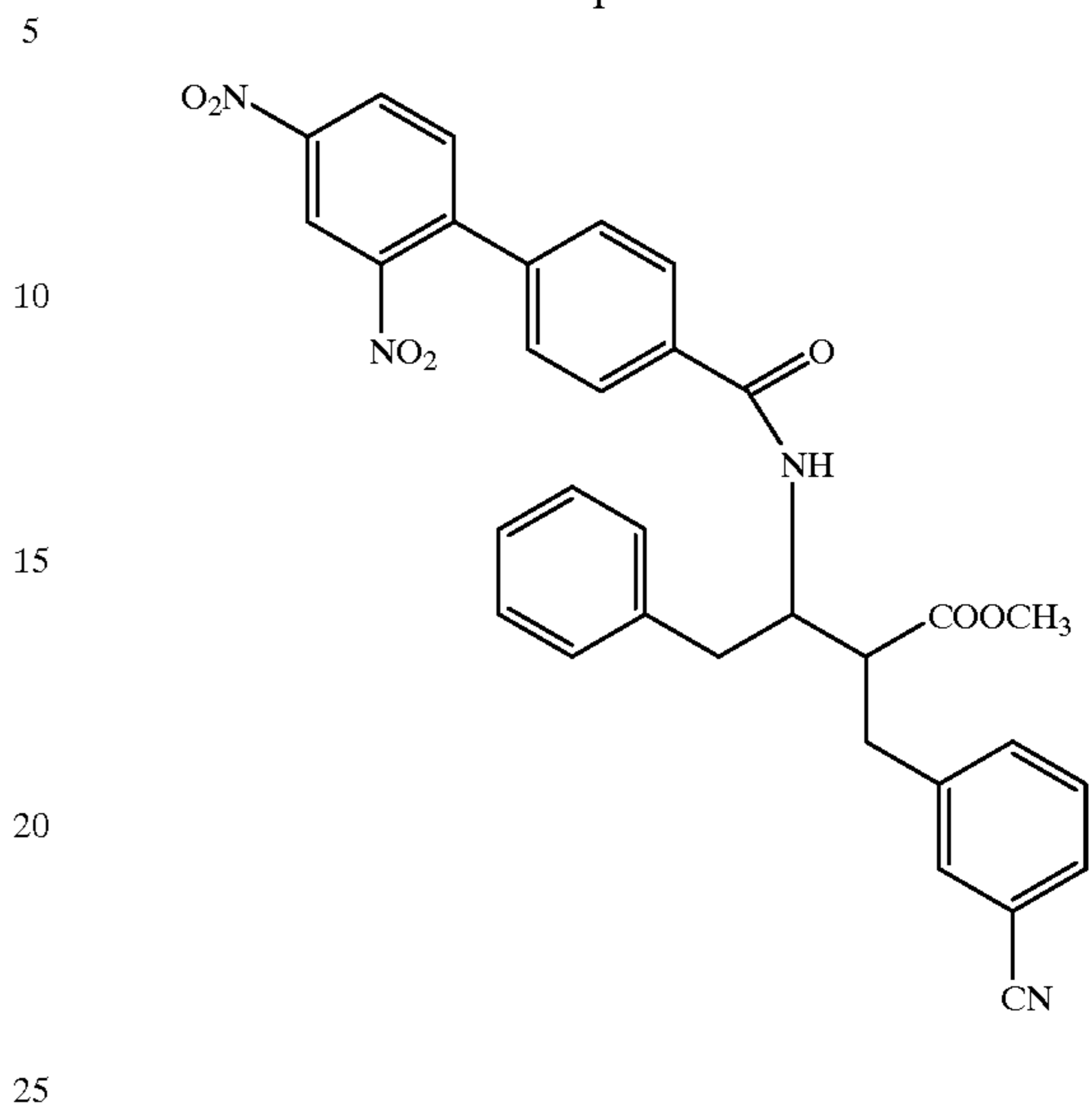
Compound 120
