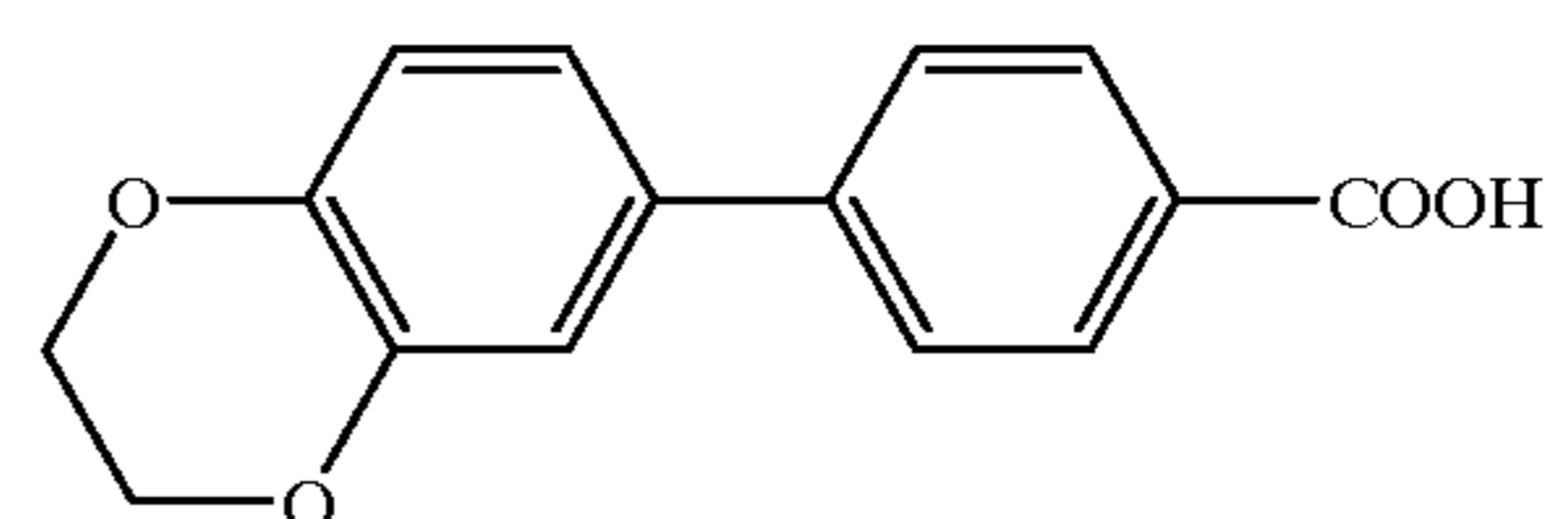
Compound 96
