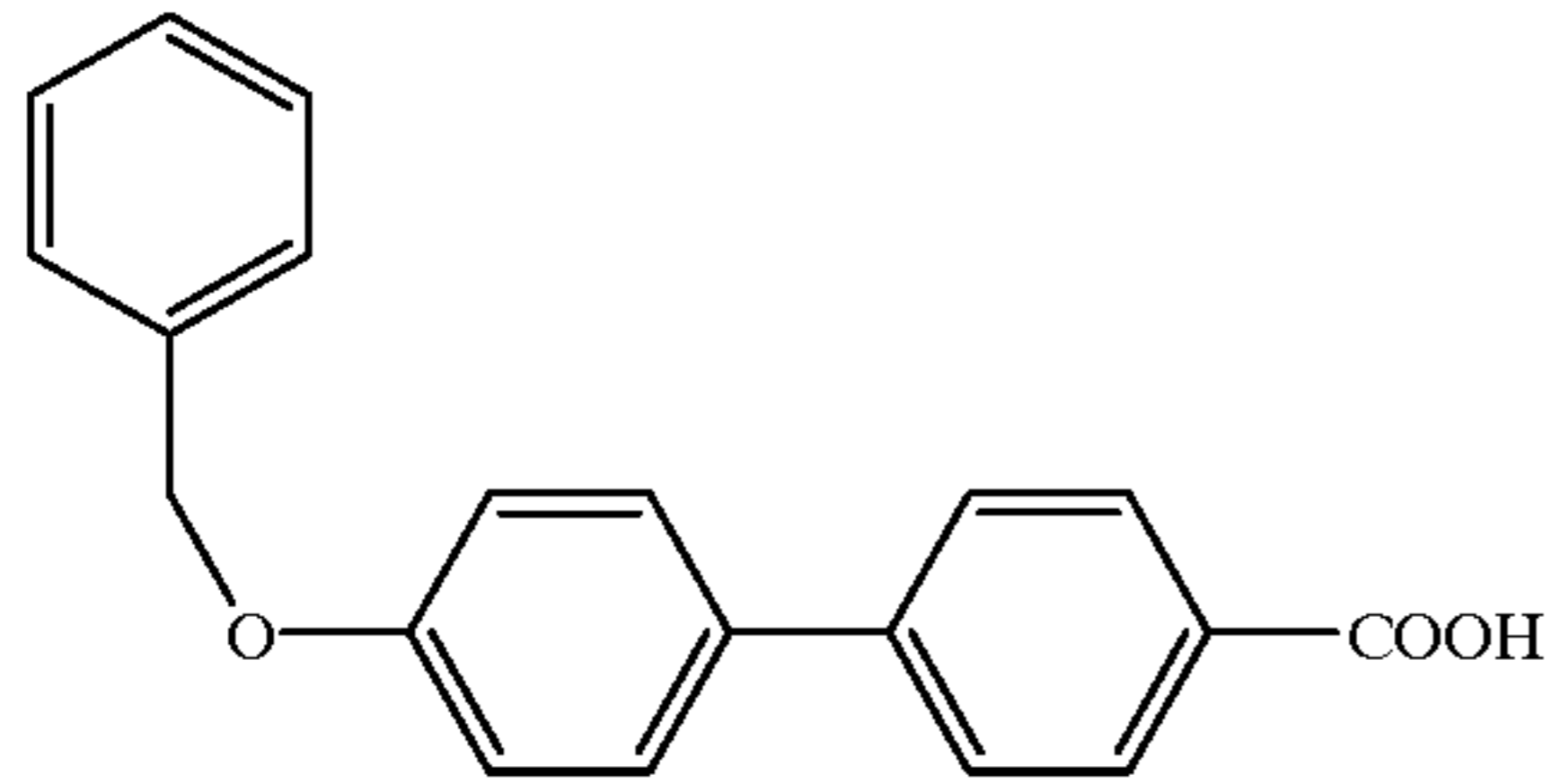
Compound 106
