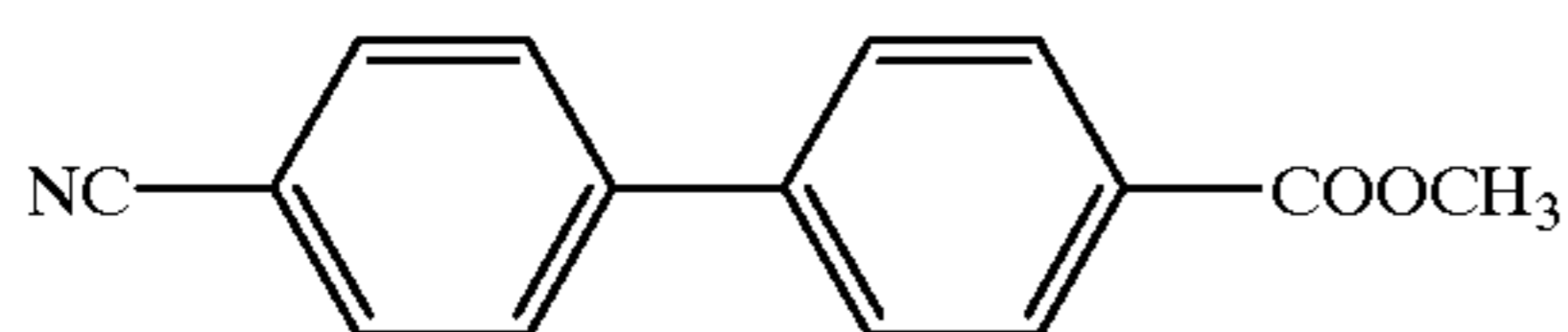
Compound 84
