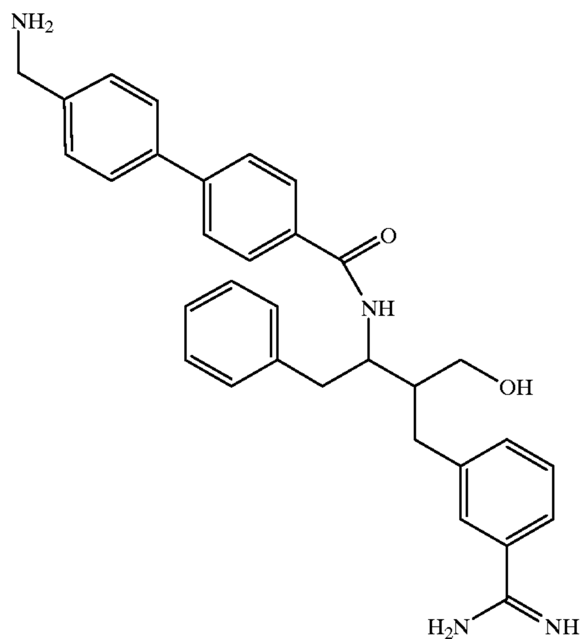
Compound 174
