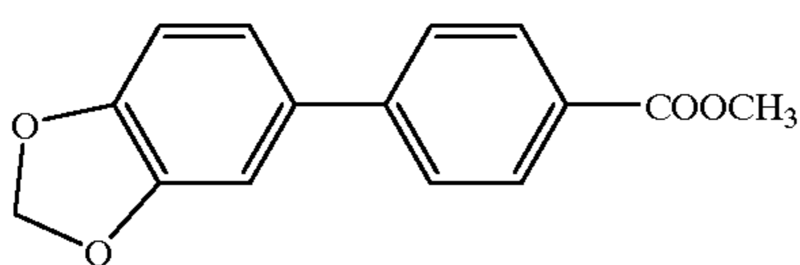
Compound 78
