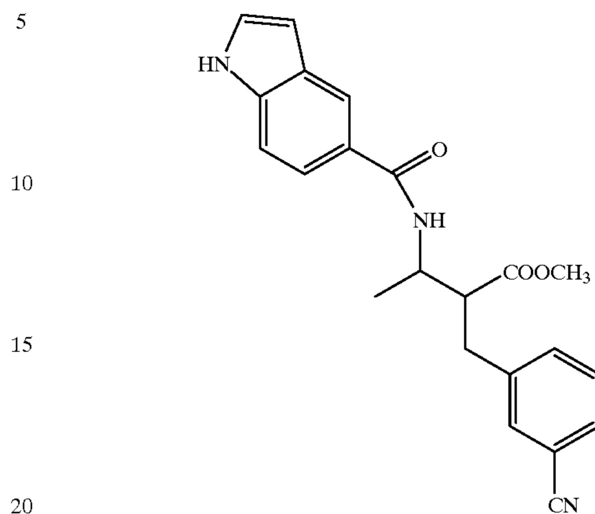
Compound 128
