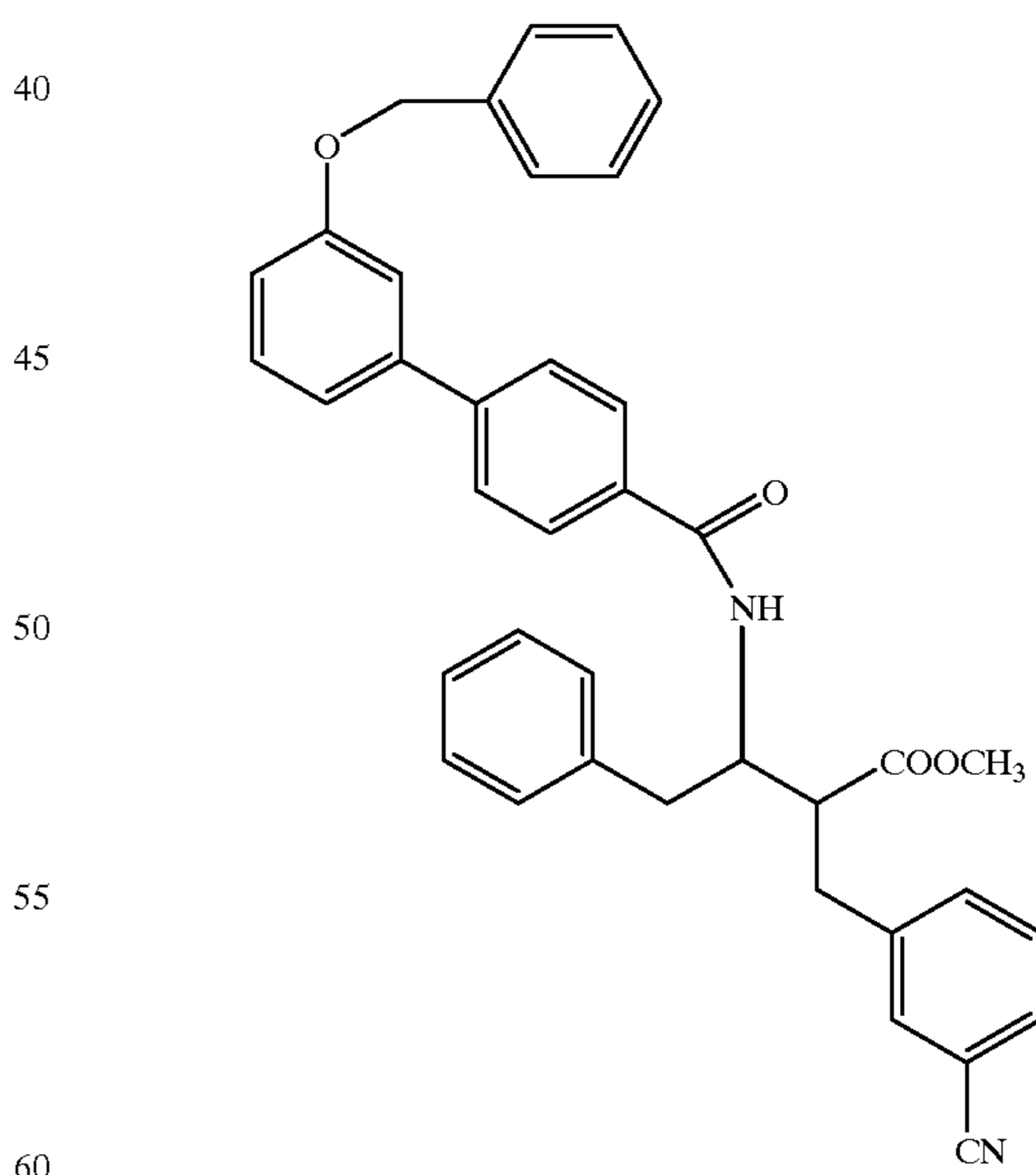
Compound 121
