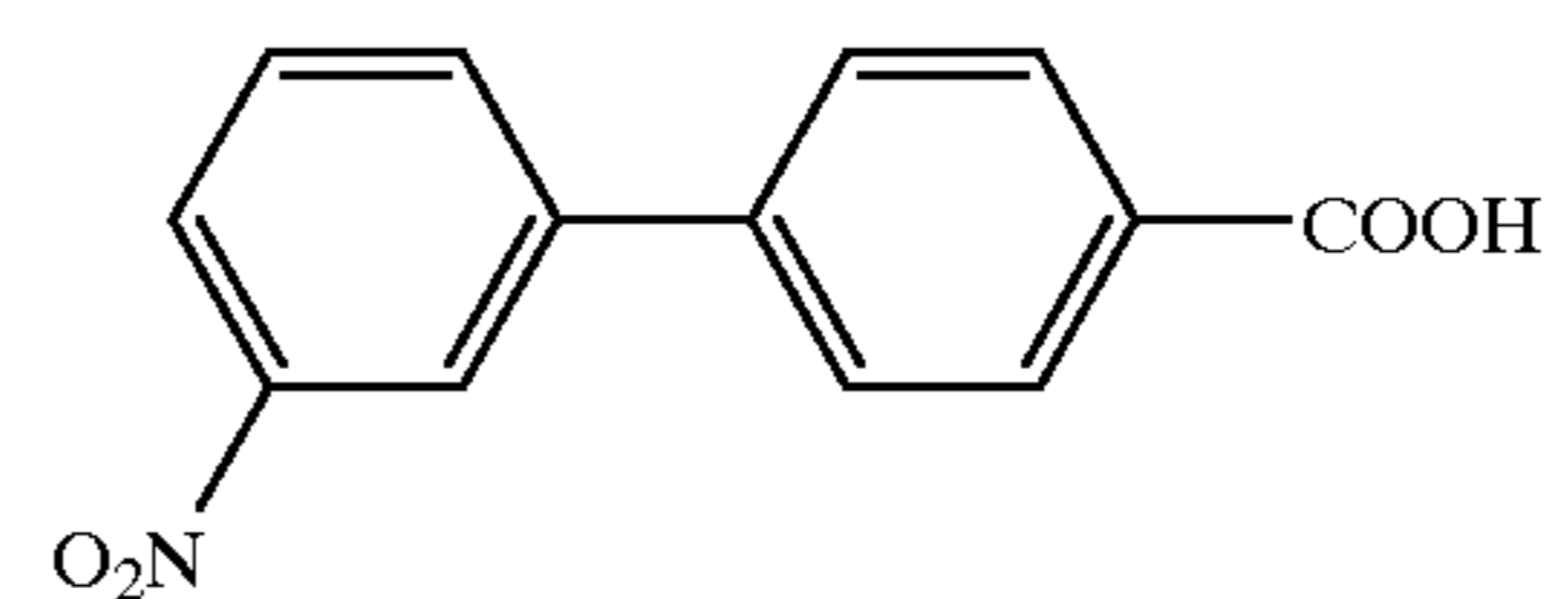
Compound 103
