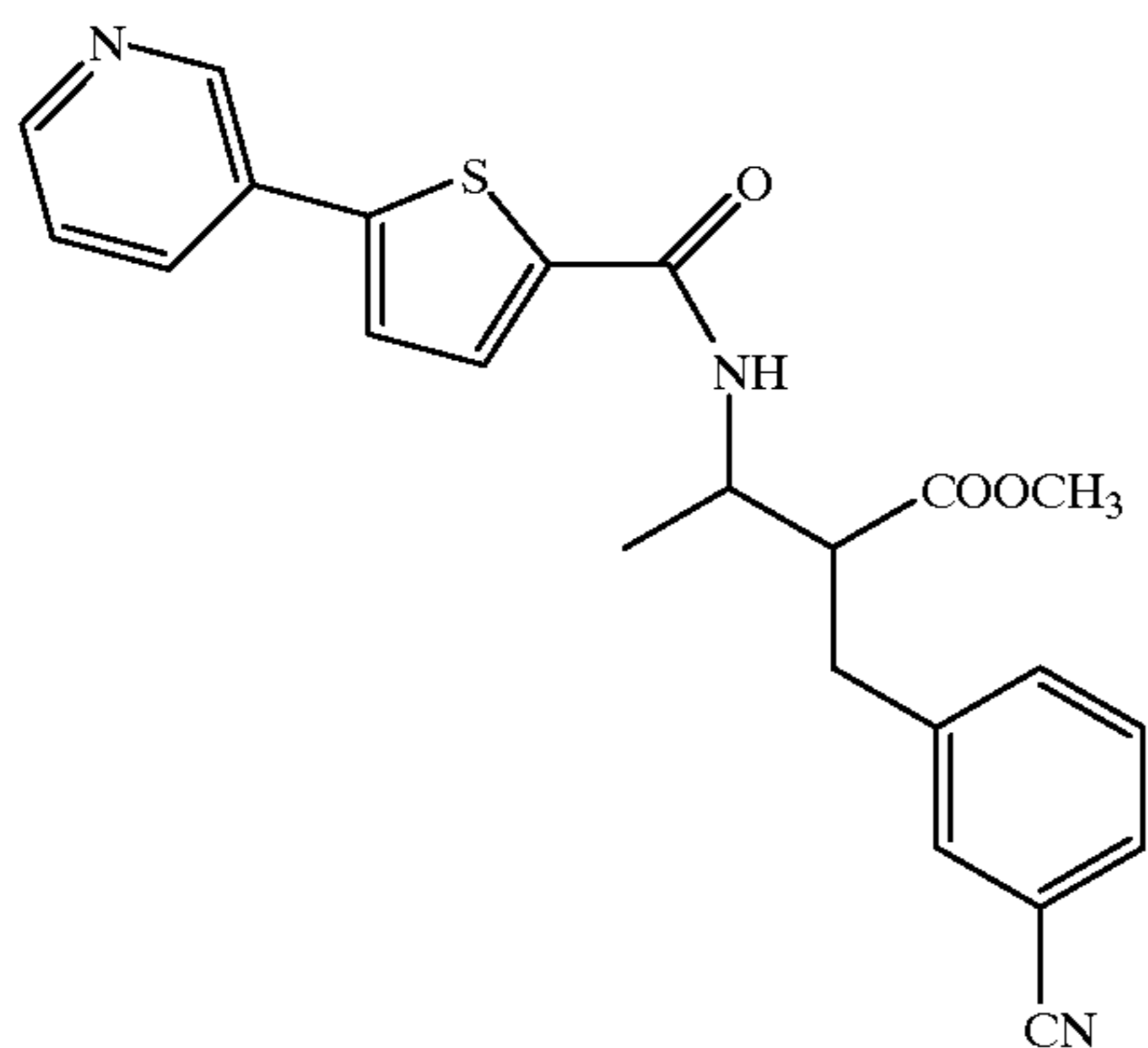
Compound 242
