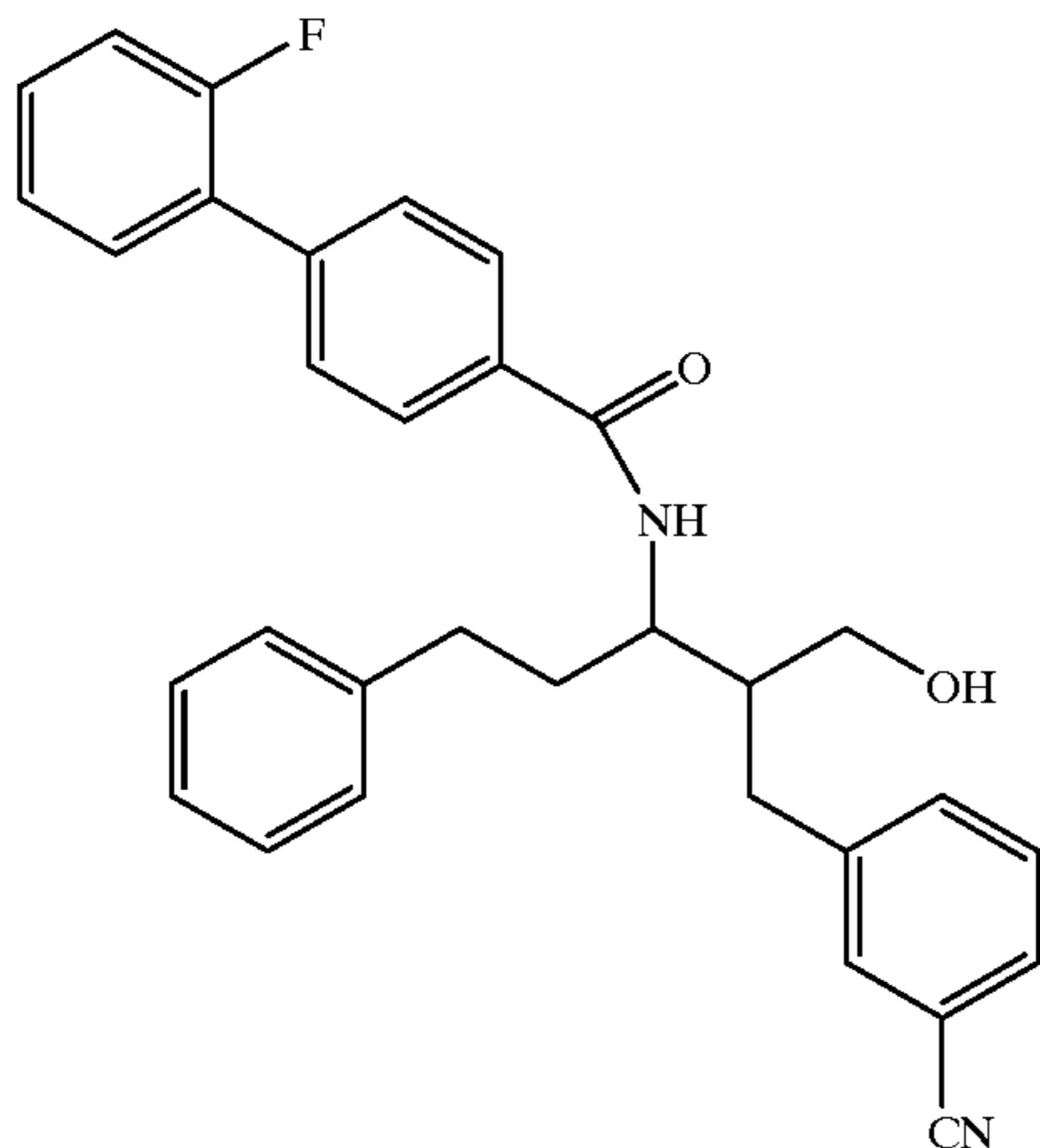
Compound 130
