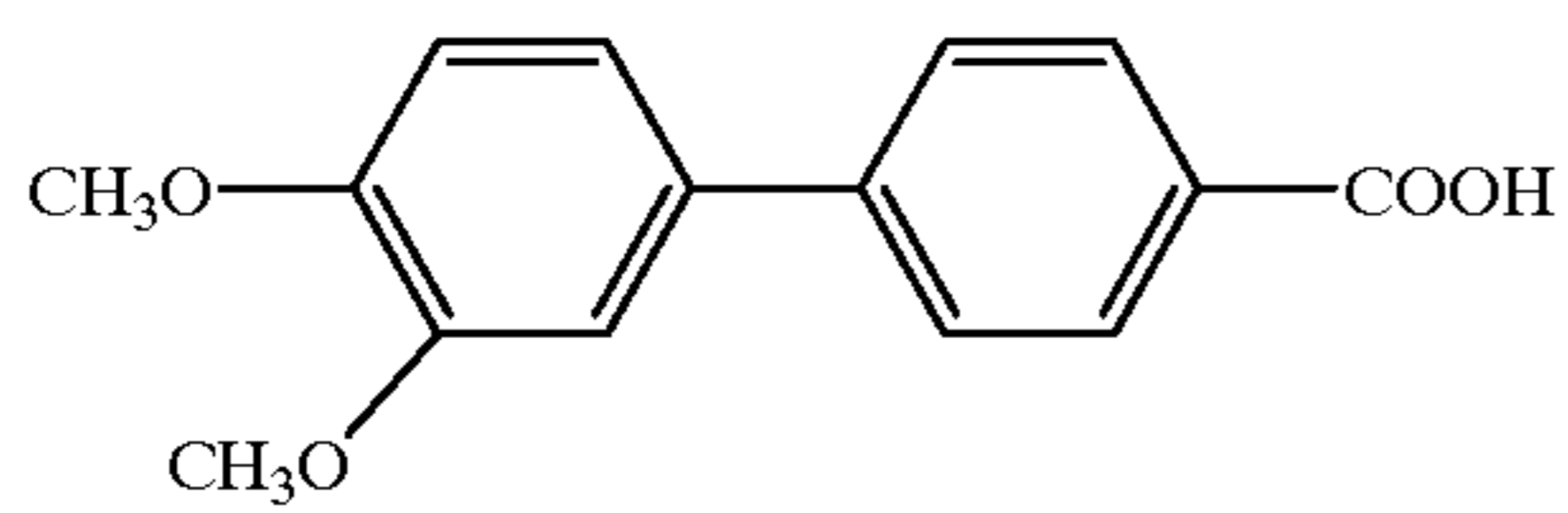
Compound 98
