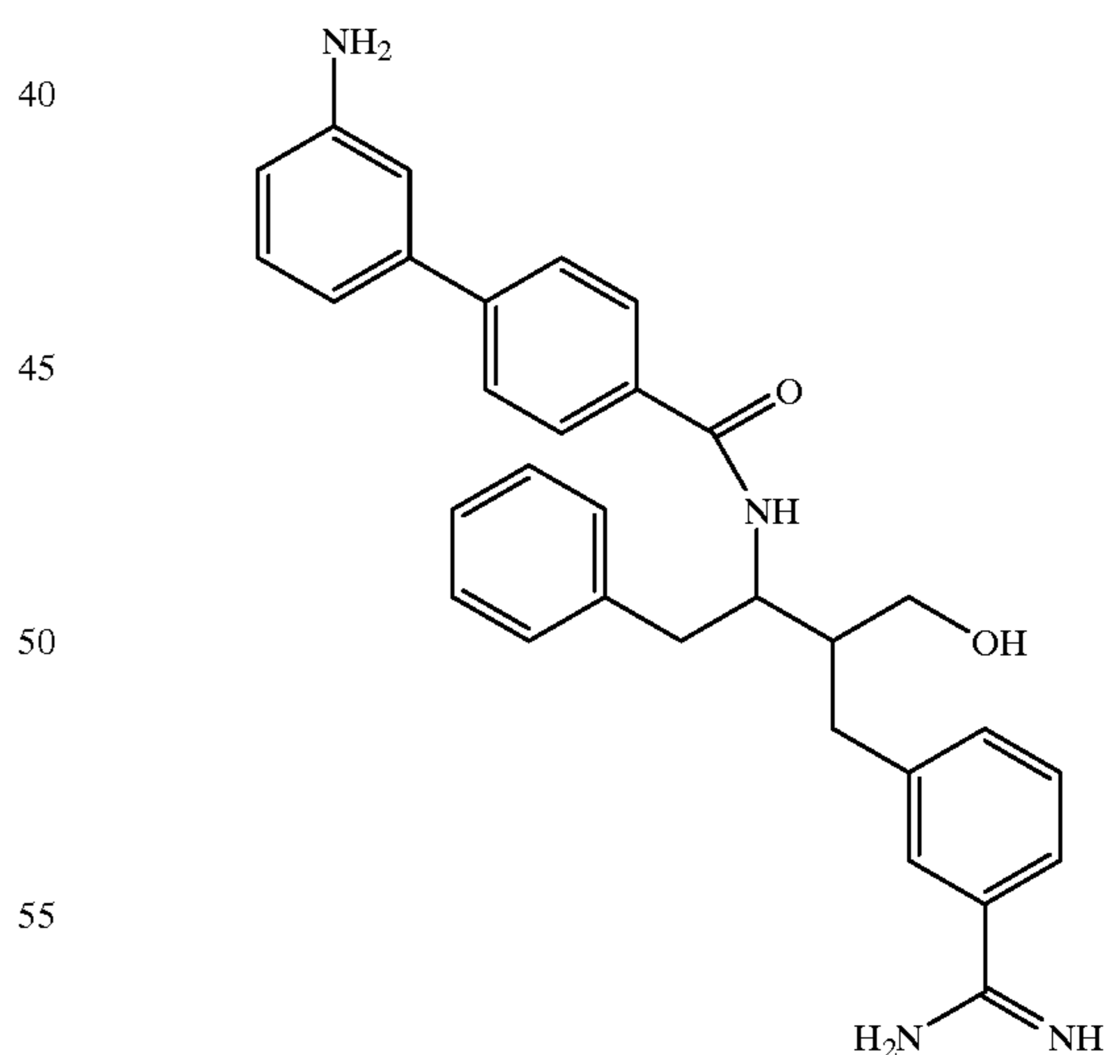
Compound 181
