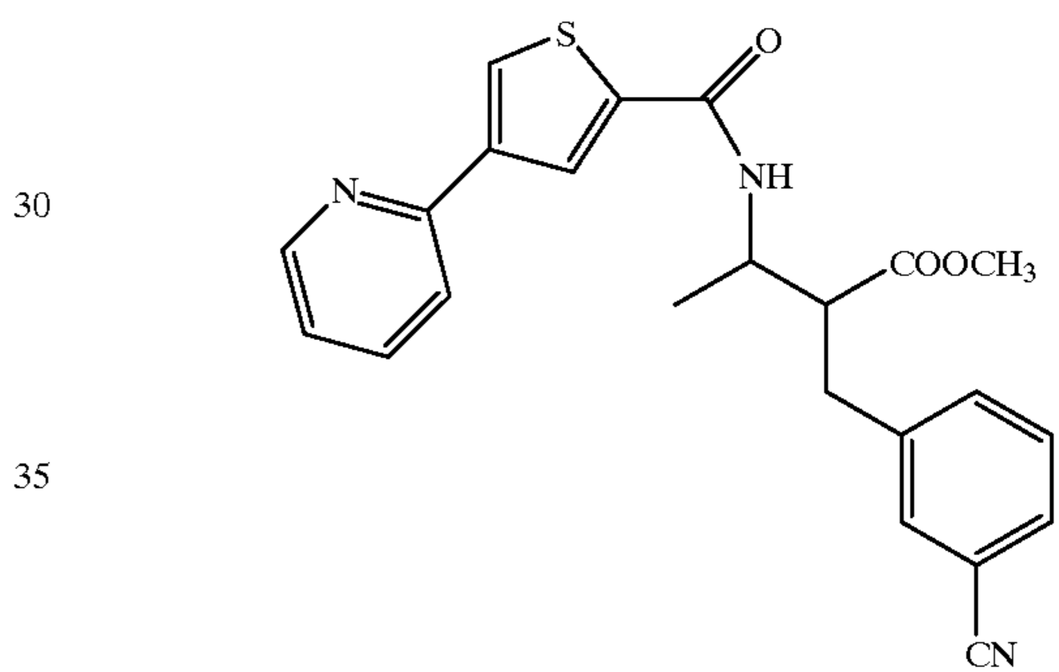
Compound 244
