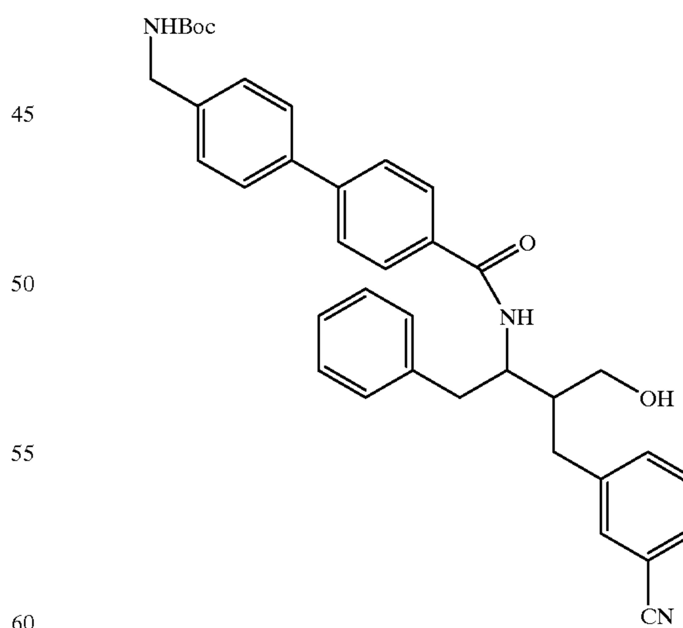
Compound 137
