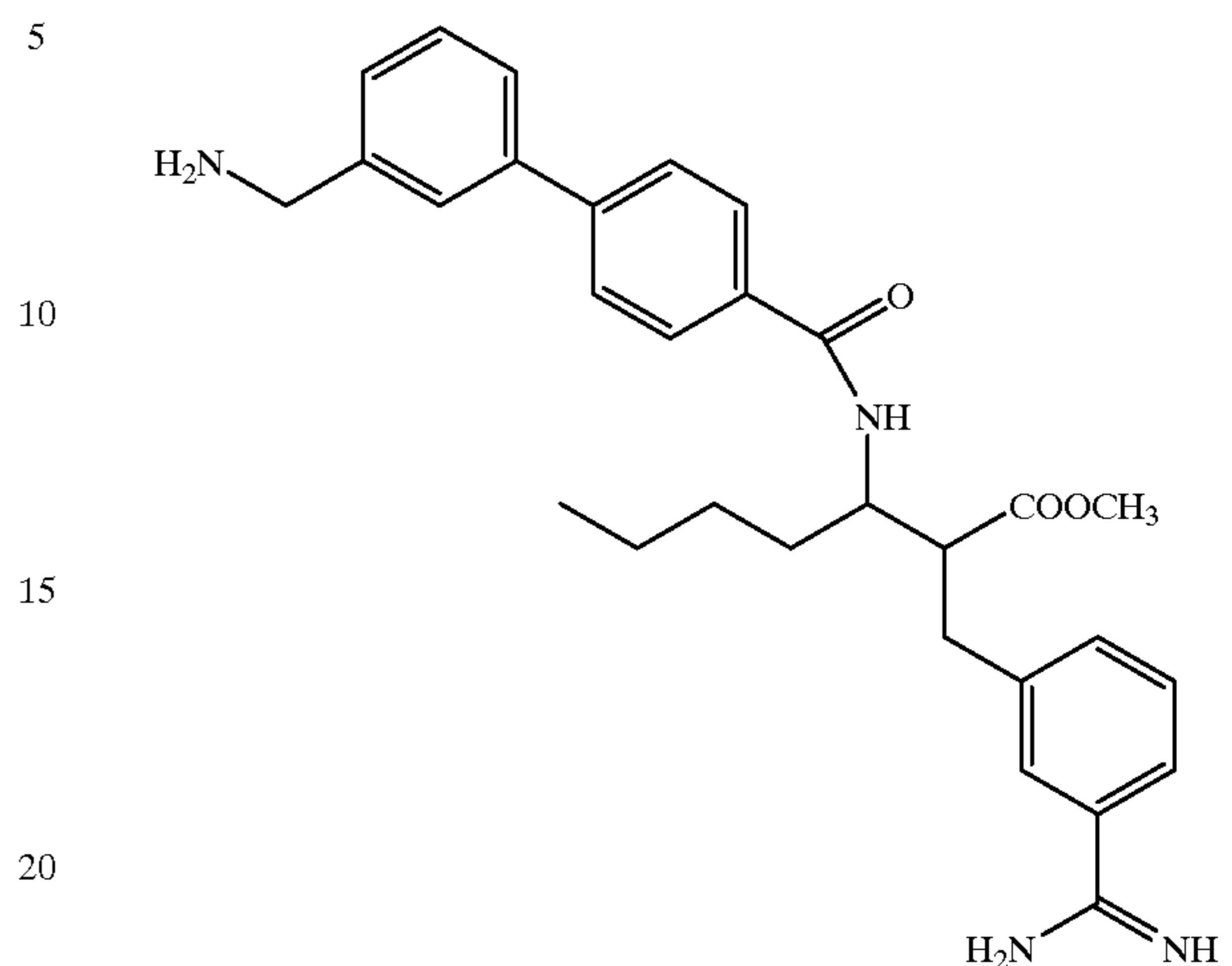
Compound 302
