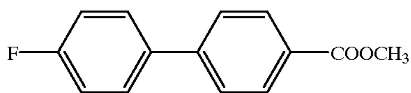
Compound 76
