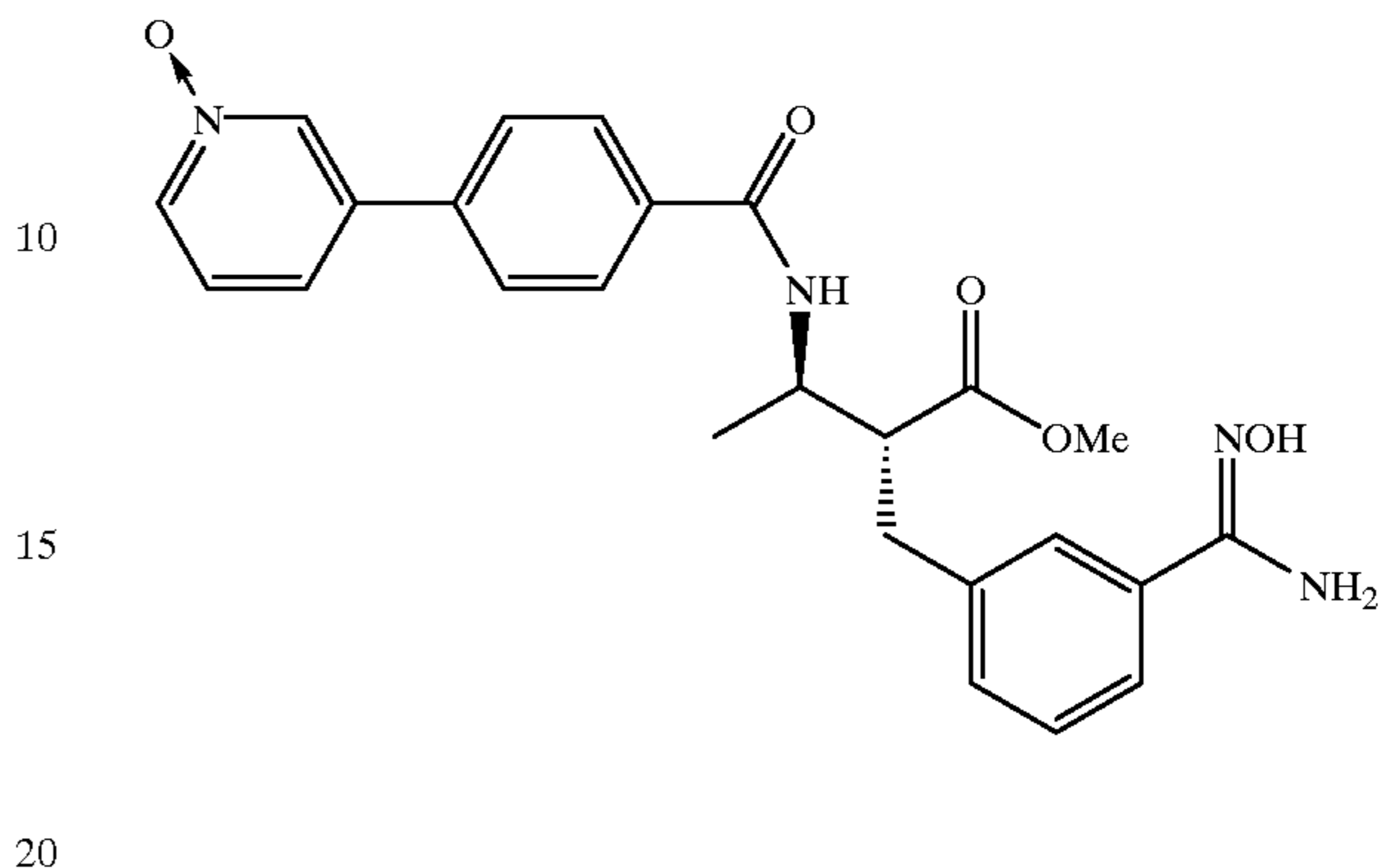
Compound 218
