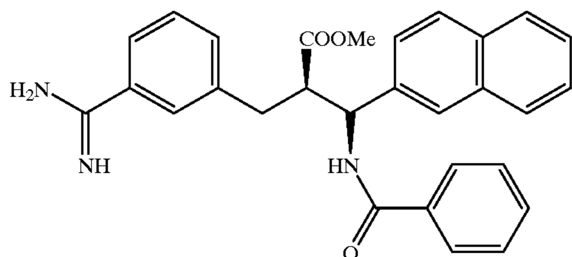
Compound 37
