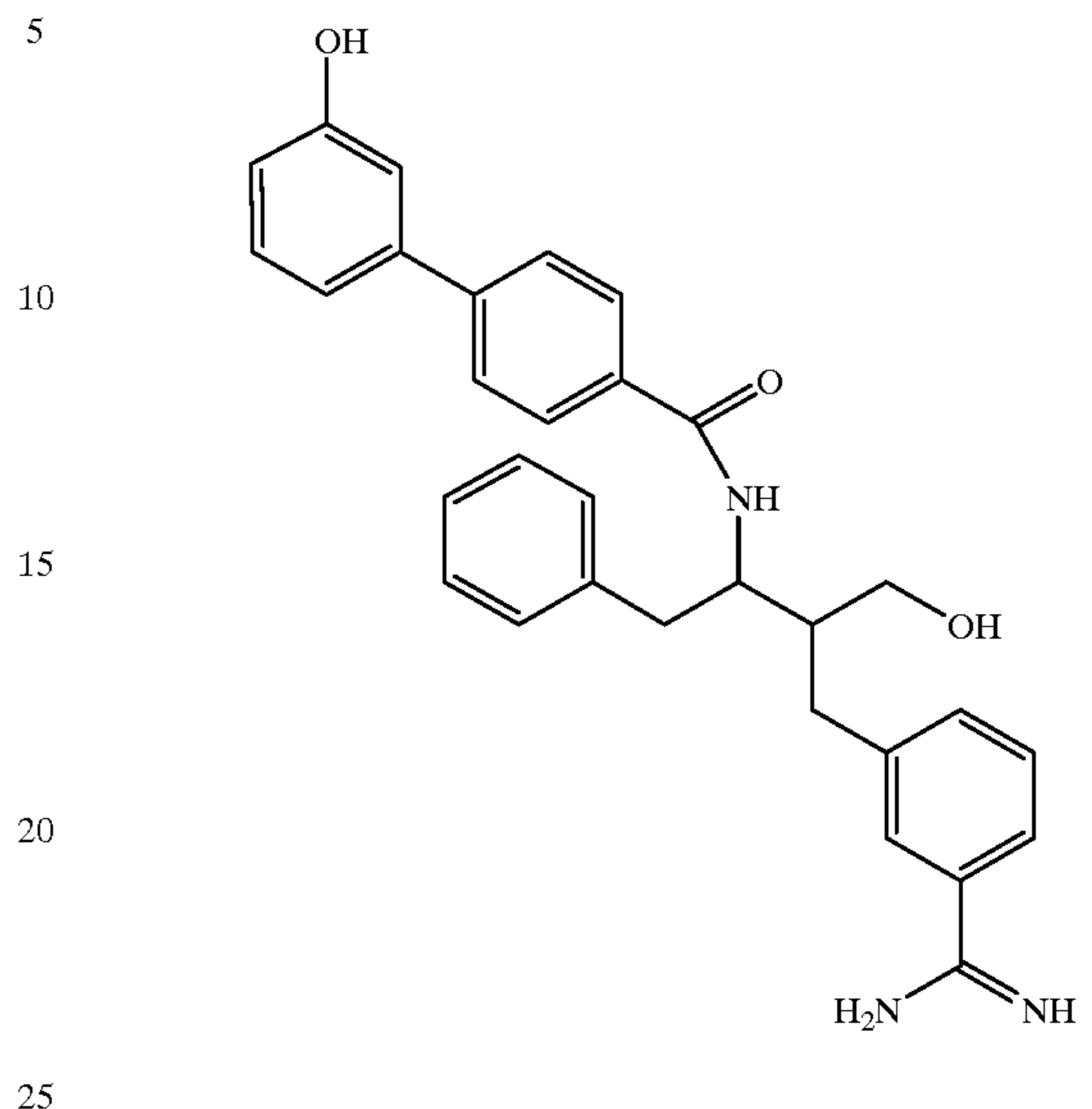
Compound 172
