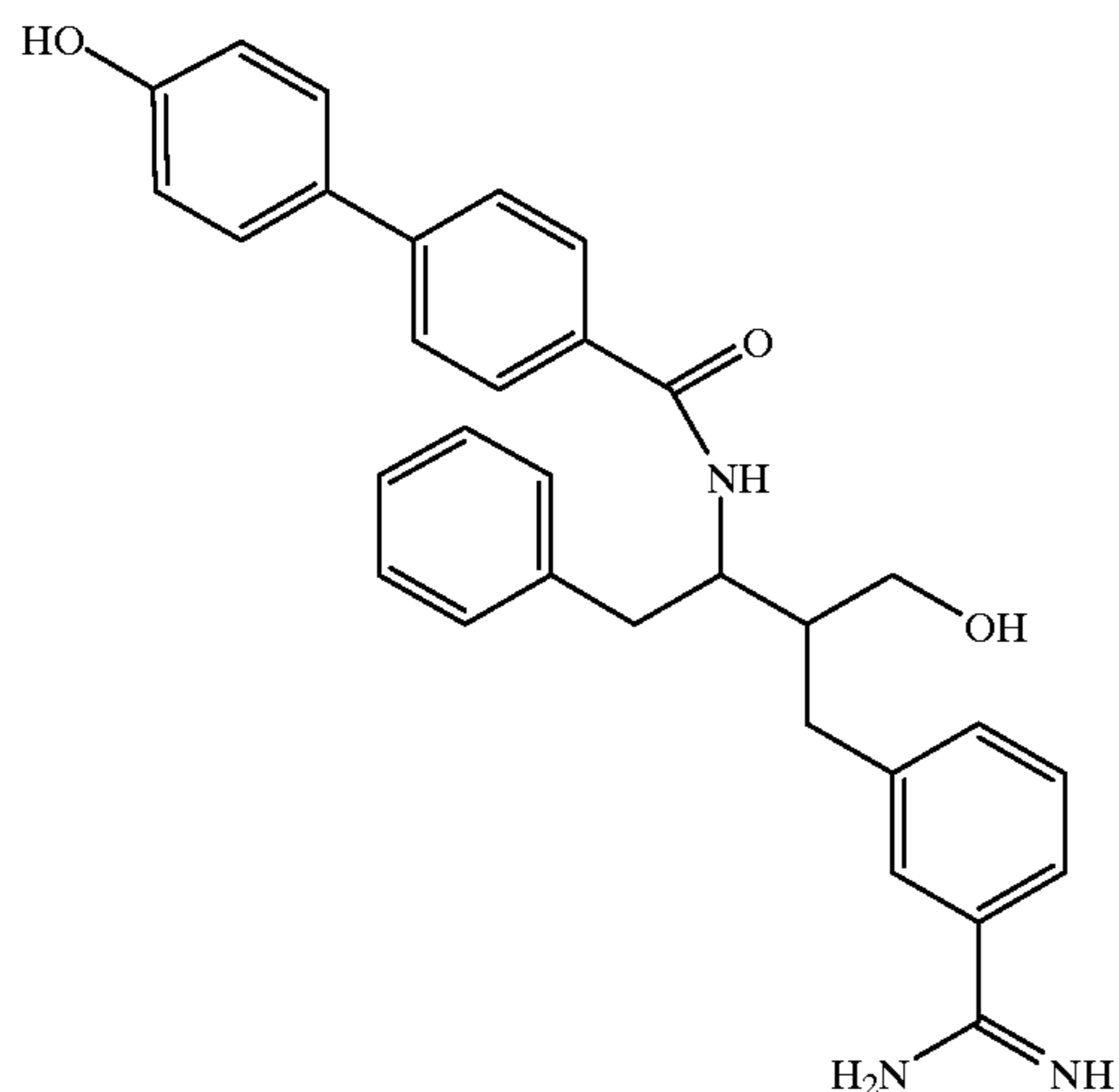
Compound 175
