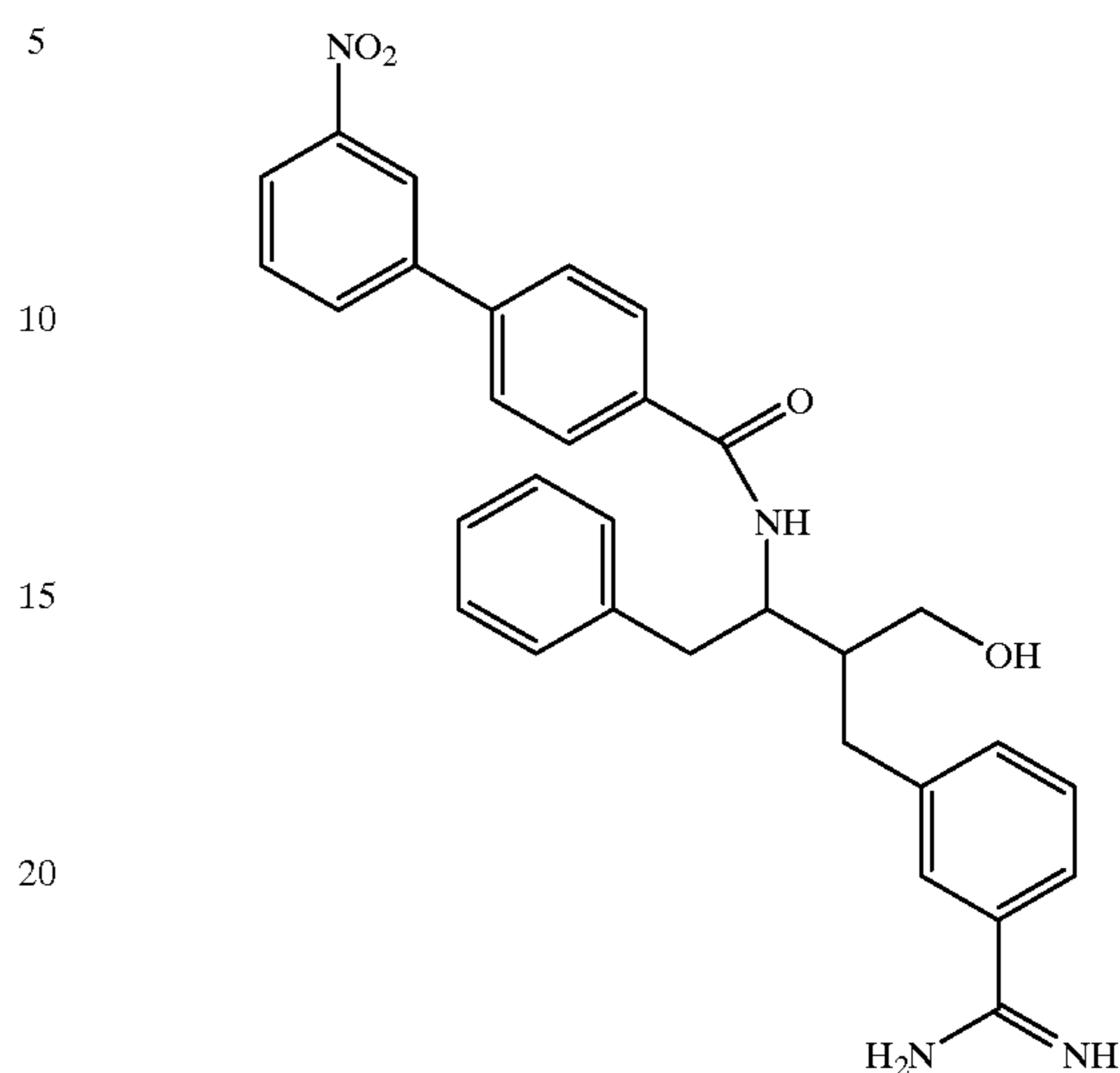
Compound 180
