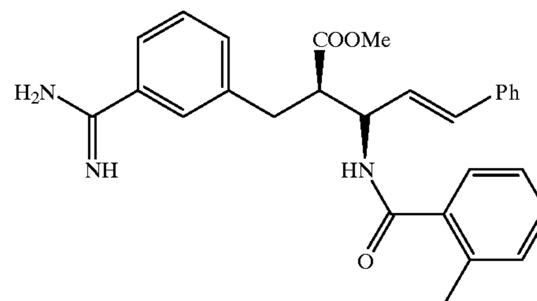
Compound 12
