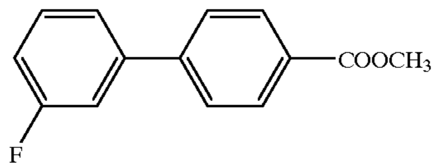
Compound 75
