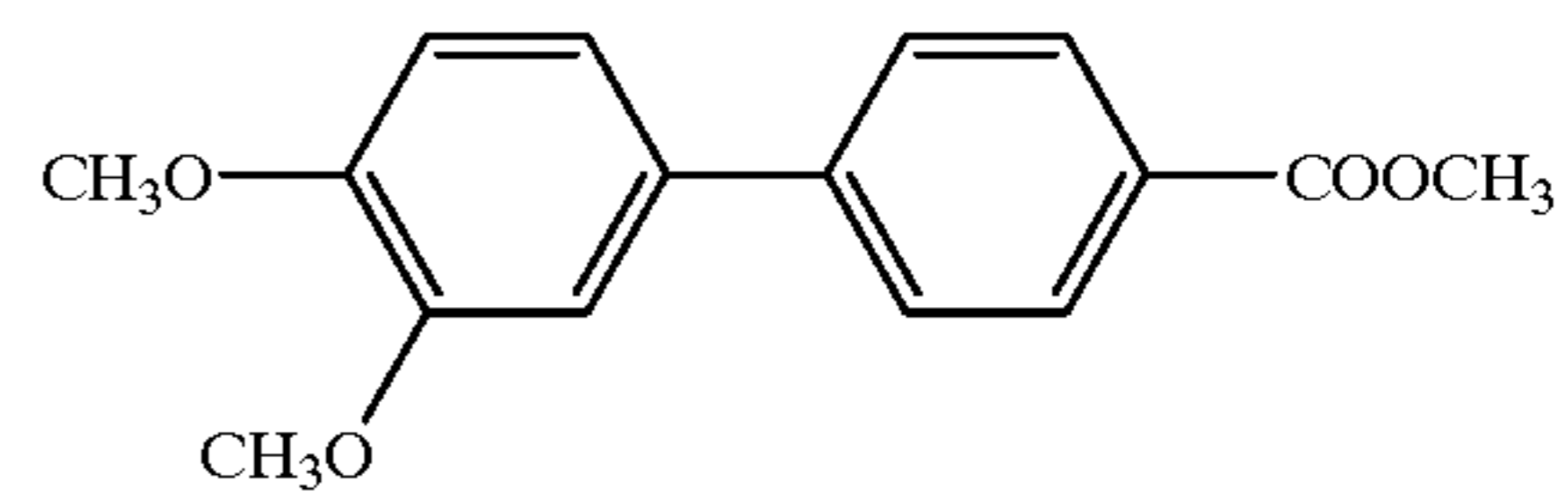
Compound 79
