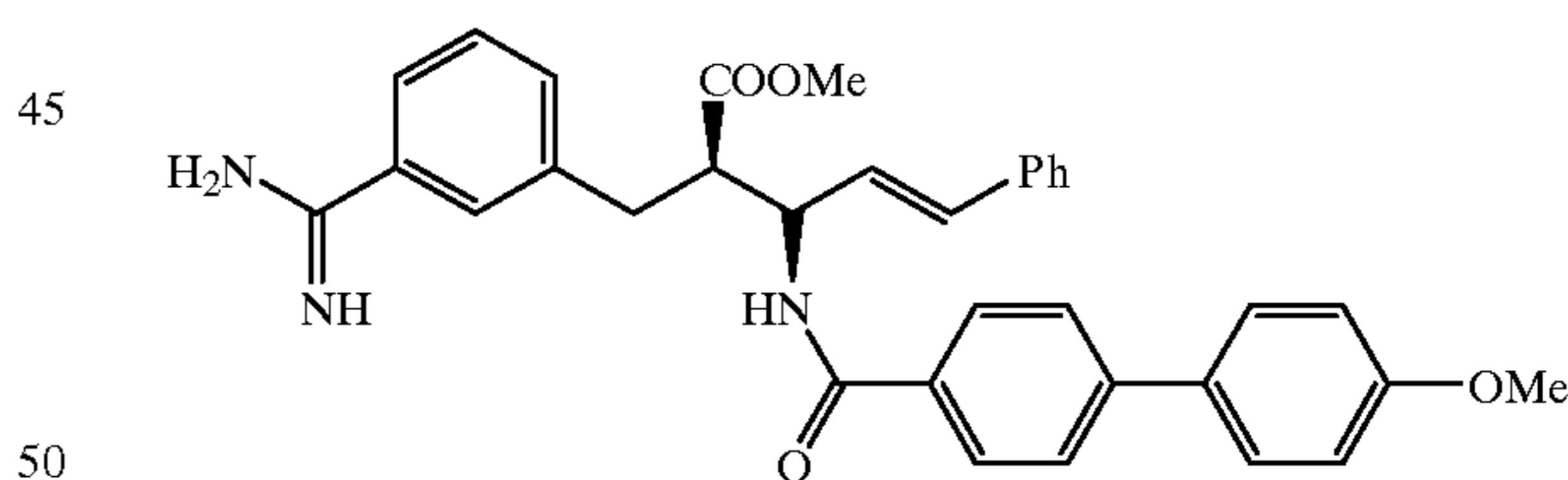
Compound 26
