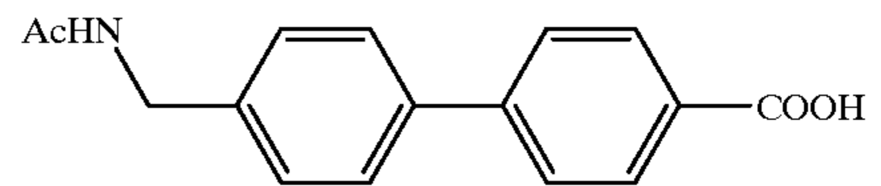
Compound 102
