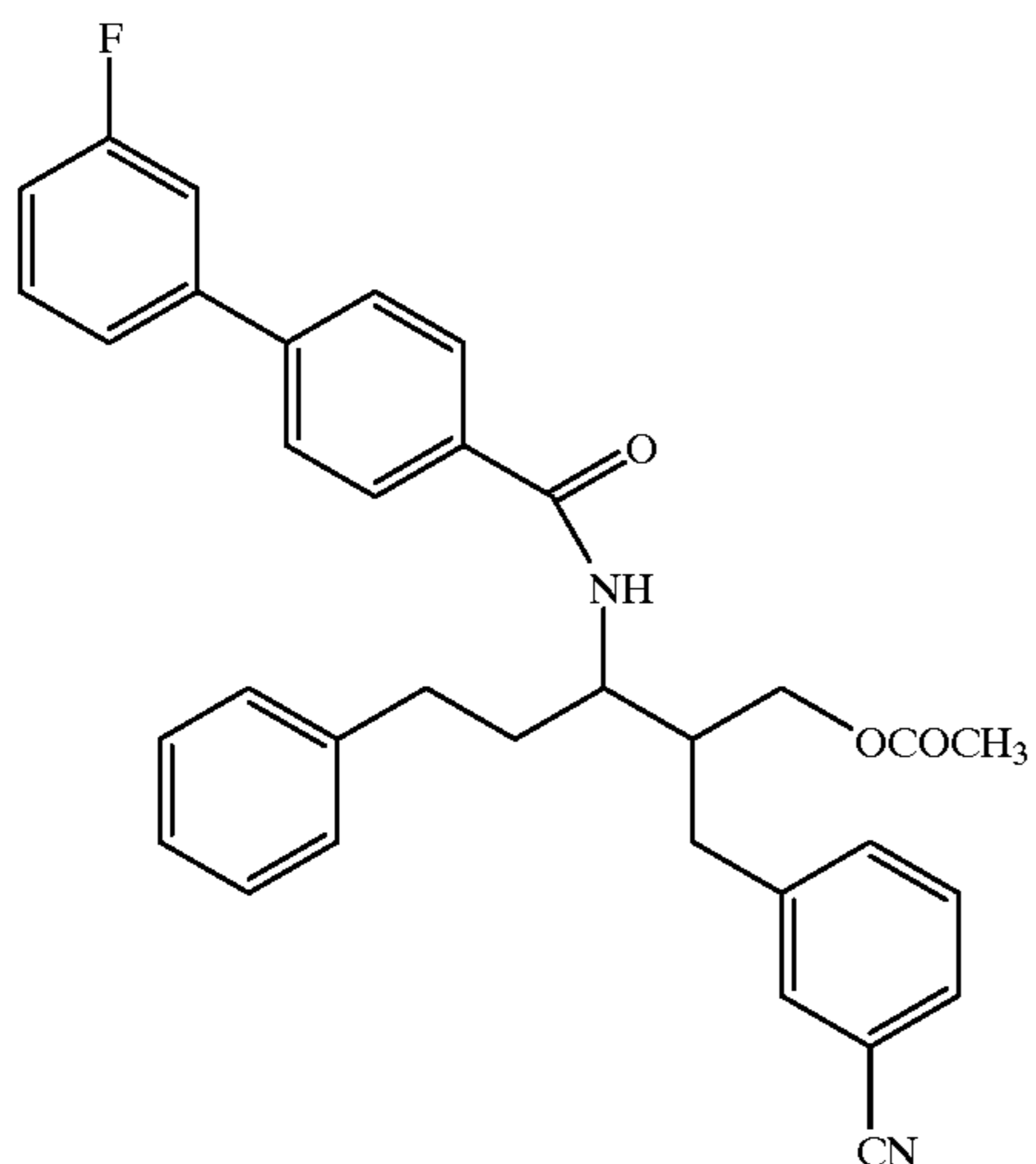
Compound 150
