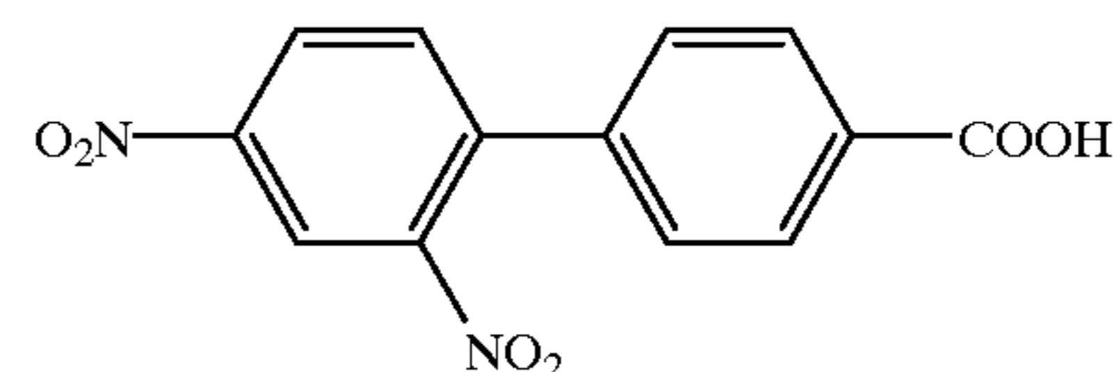
Compound 90
