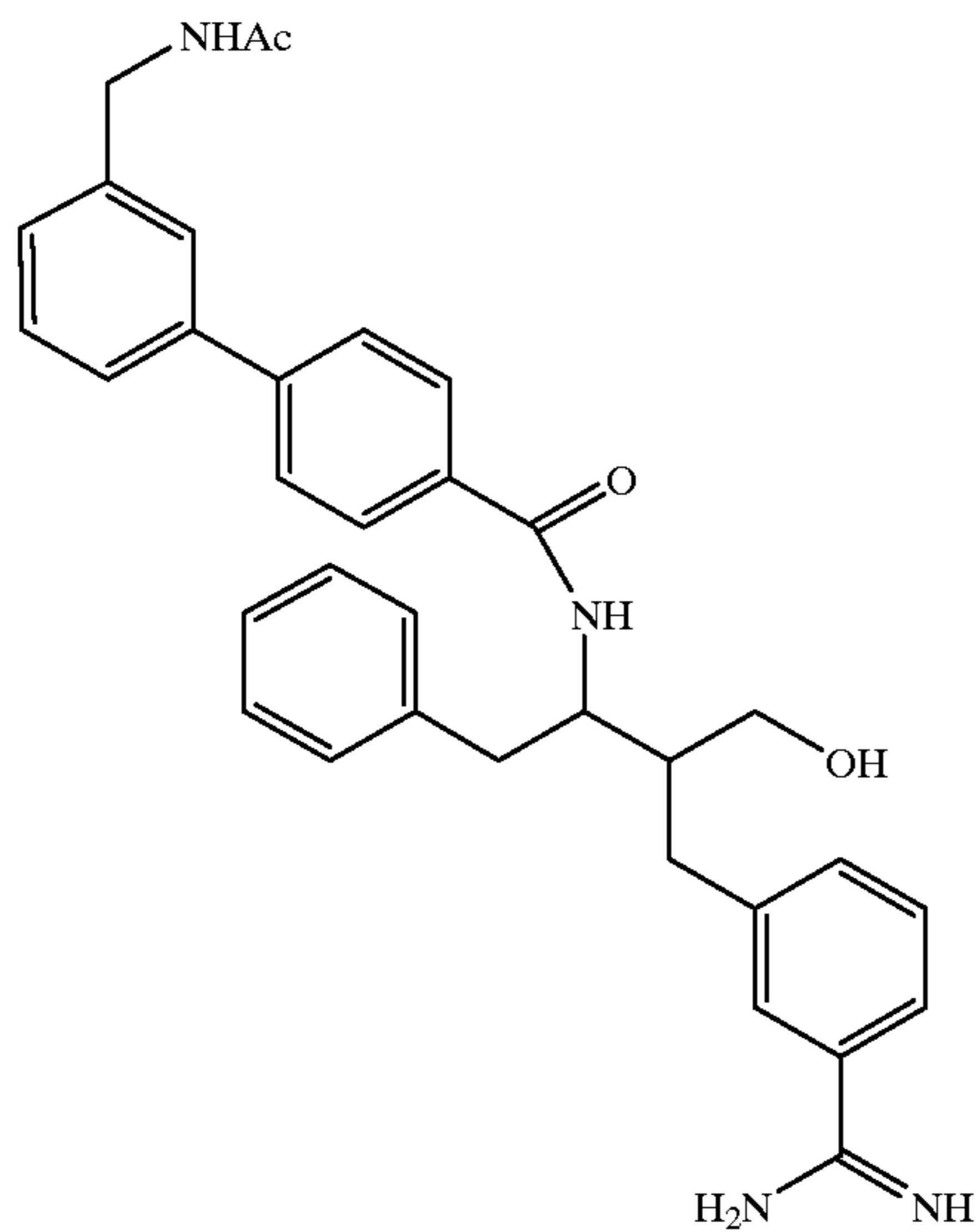
Compound 170
