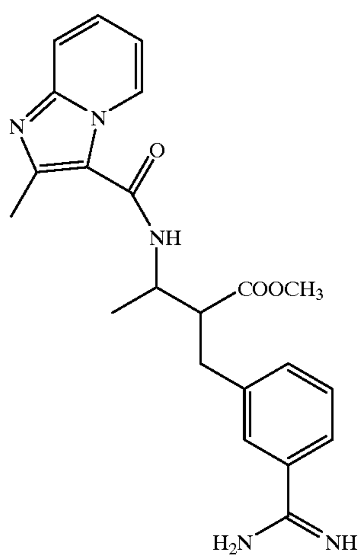
Compound 293
