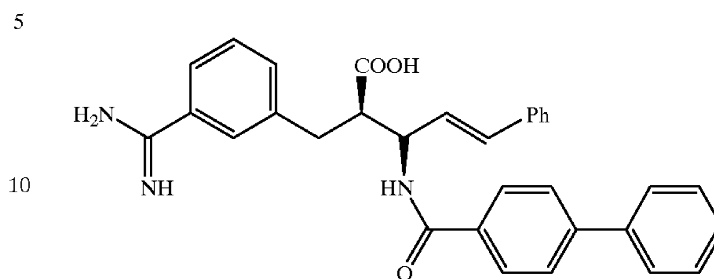
Compound 47
