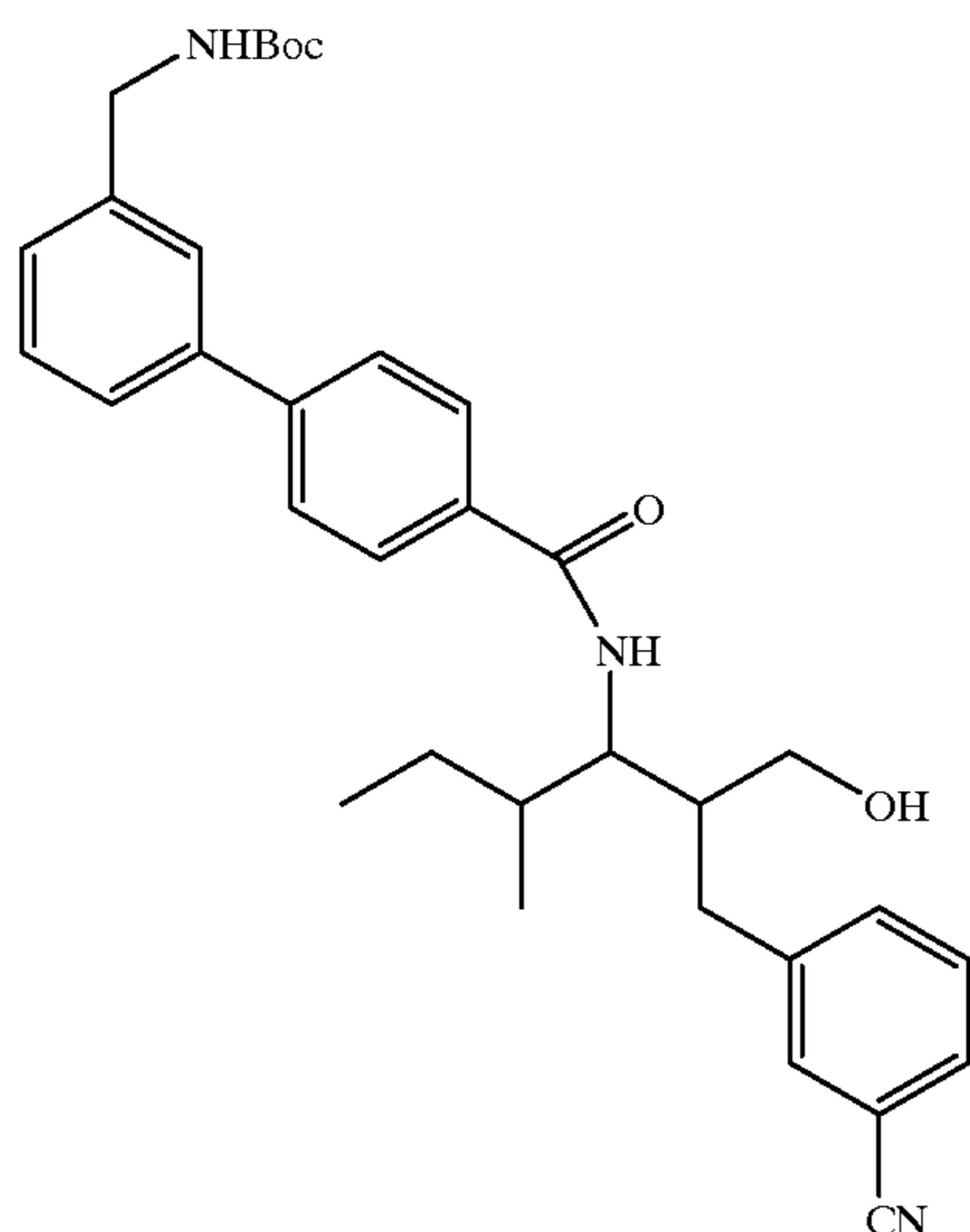
Compound 147
