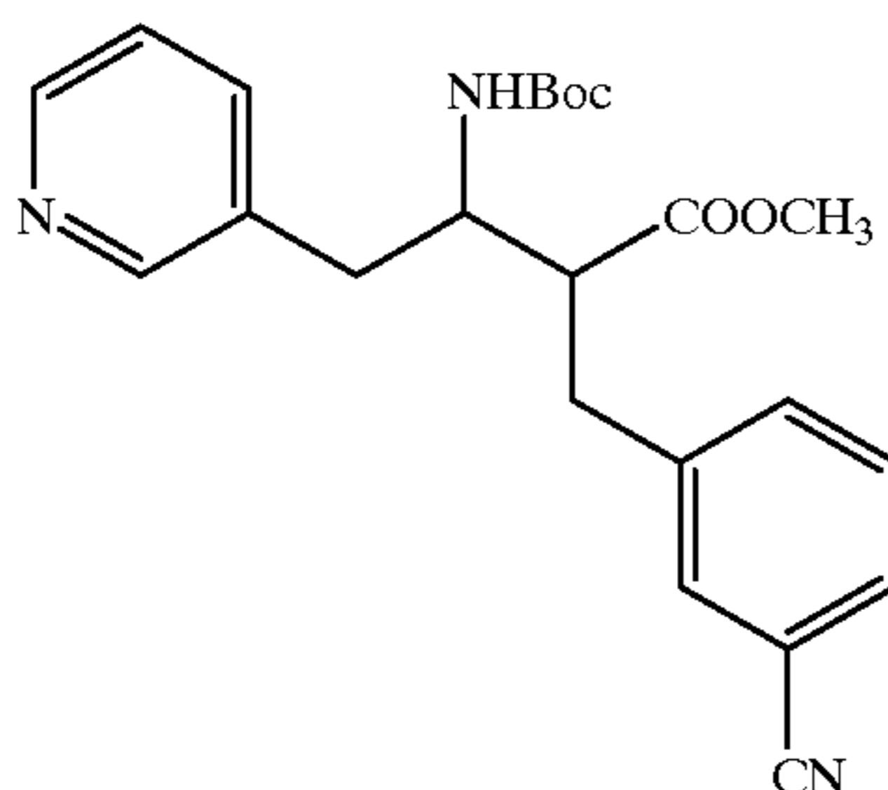
Compound 65
