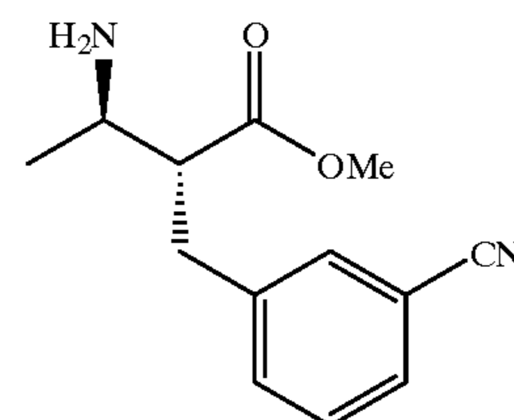
Compound 199
