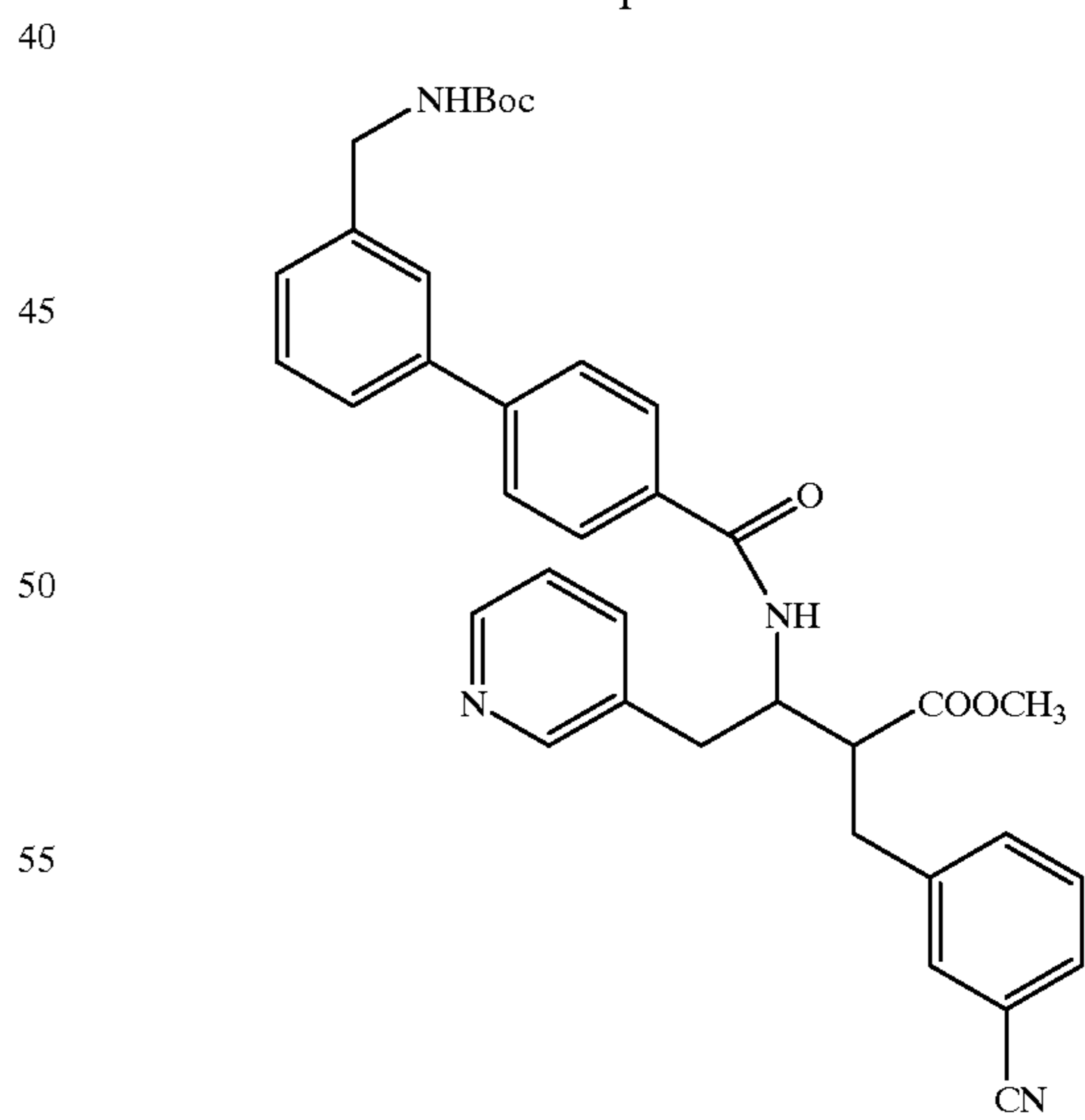
Compound 125
