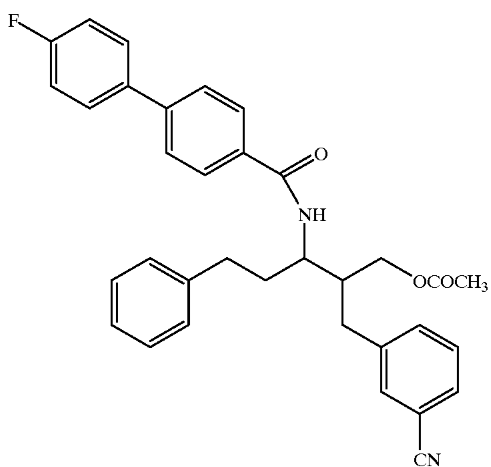
Compound 151
