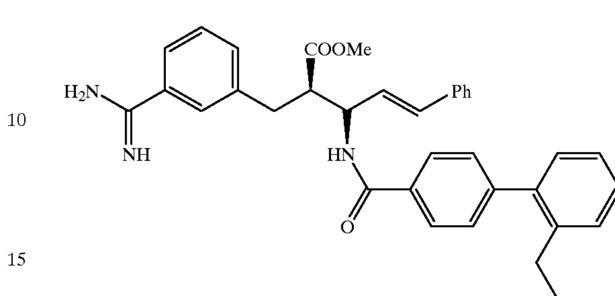
Compound 25
