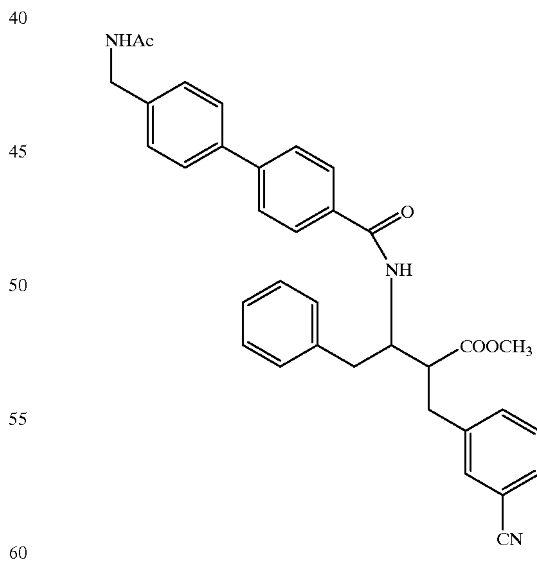
Compound 117
