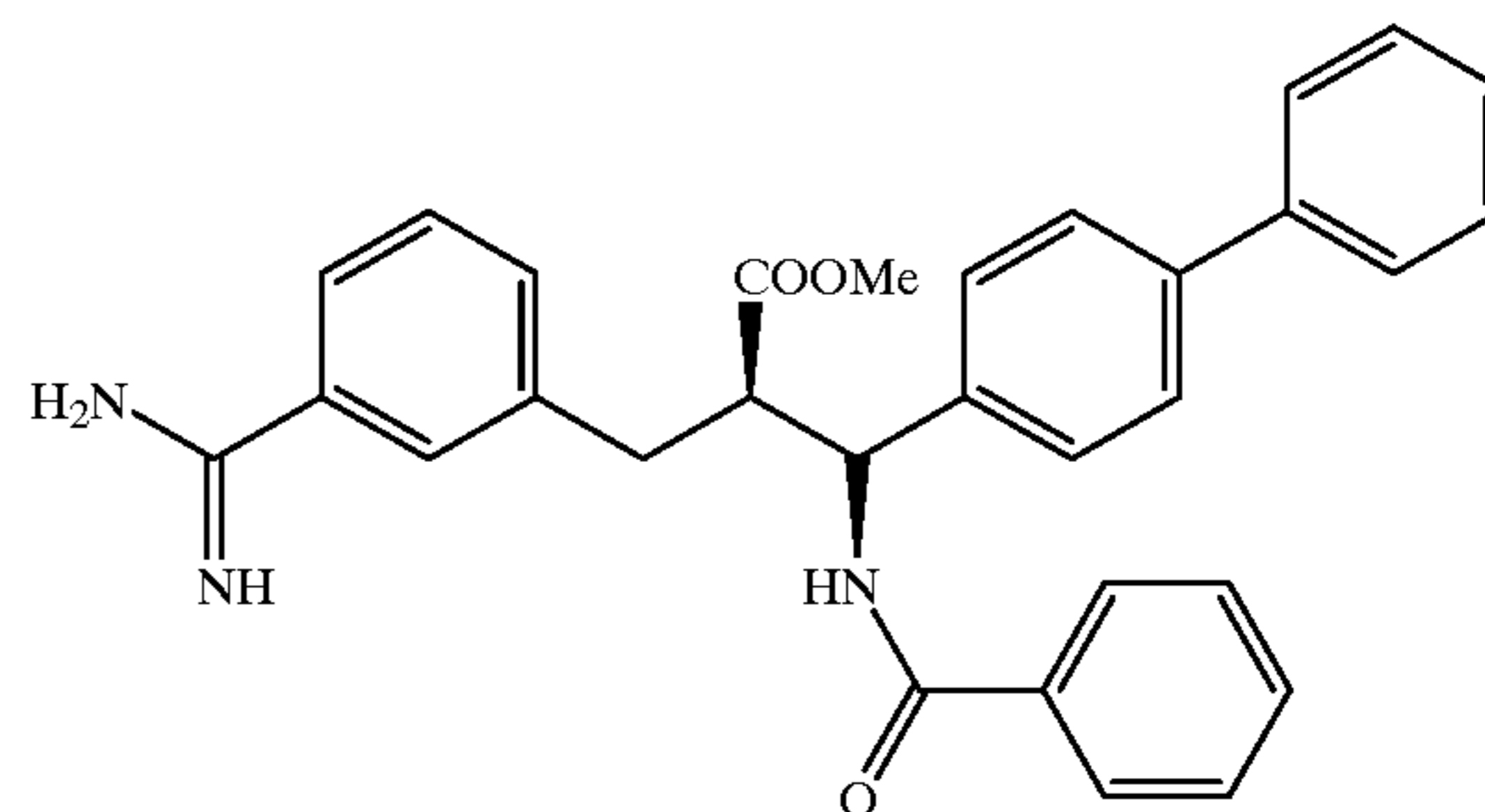
Compound 40
