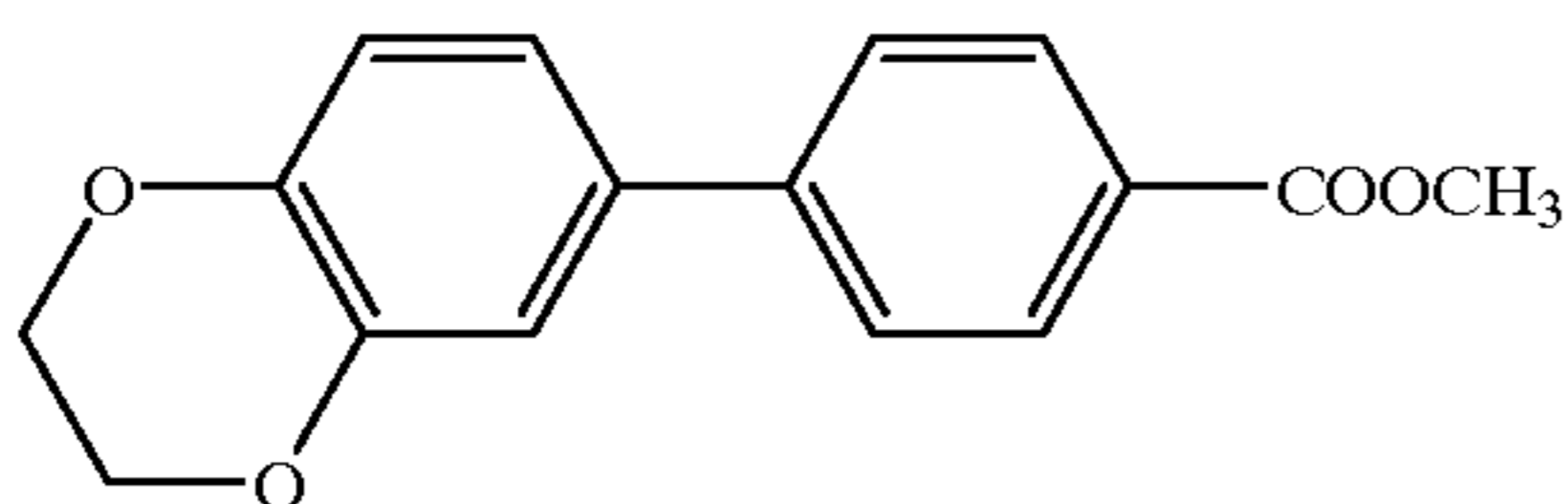
Compound 77
