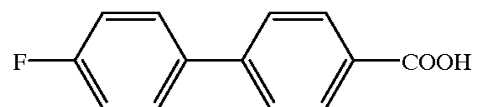
Compound 95
