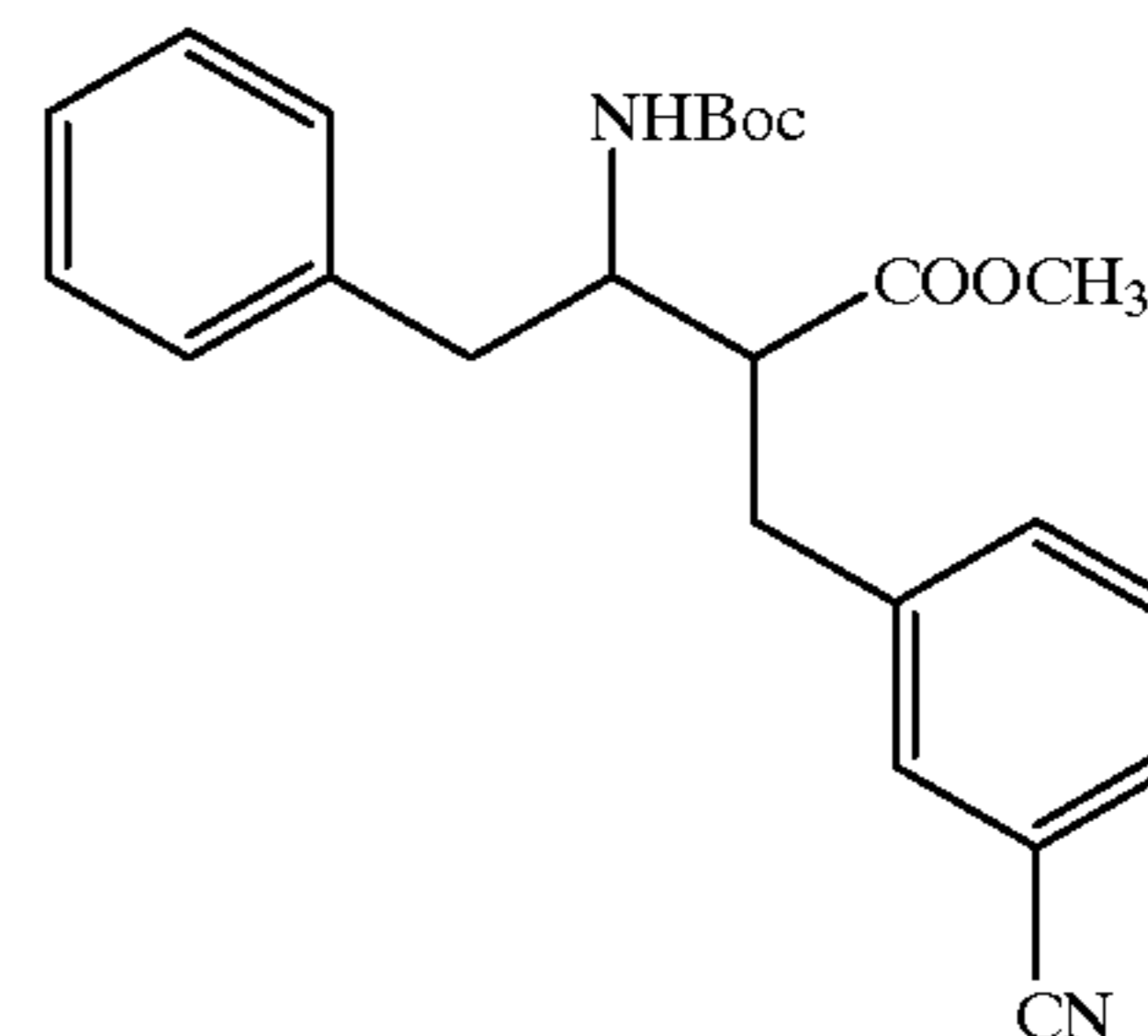
Compound 62
