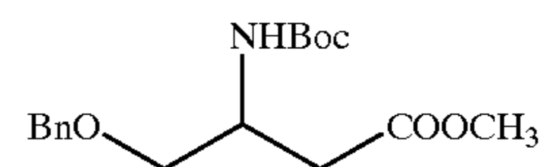
Compound 262
