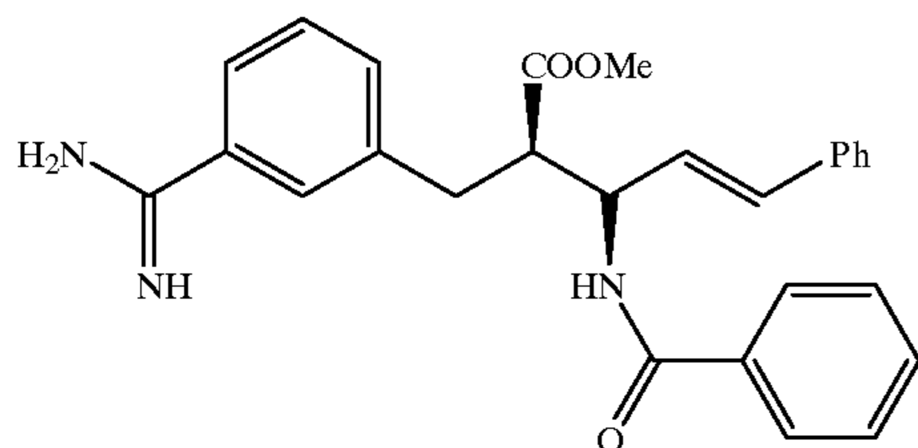
Compound 11
