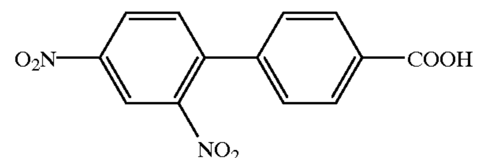
Compound 90
