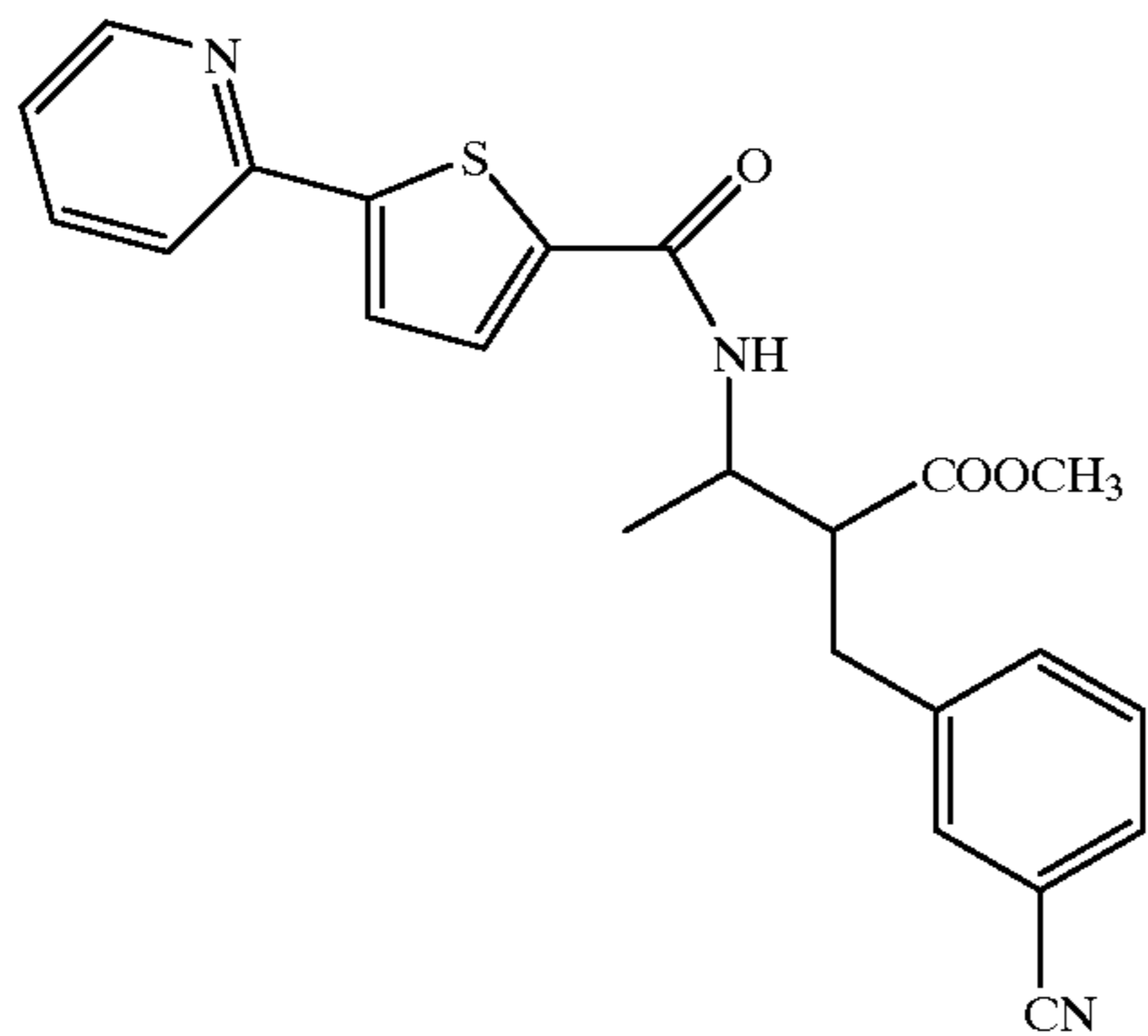
Compound 241
