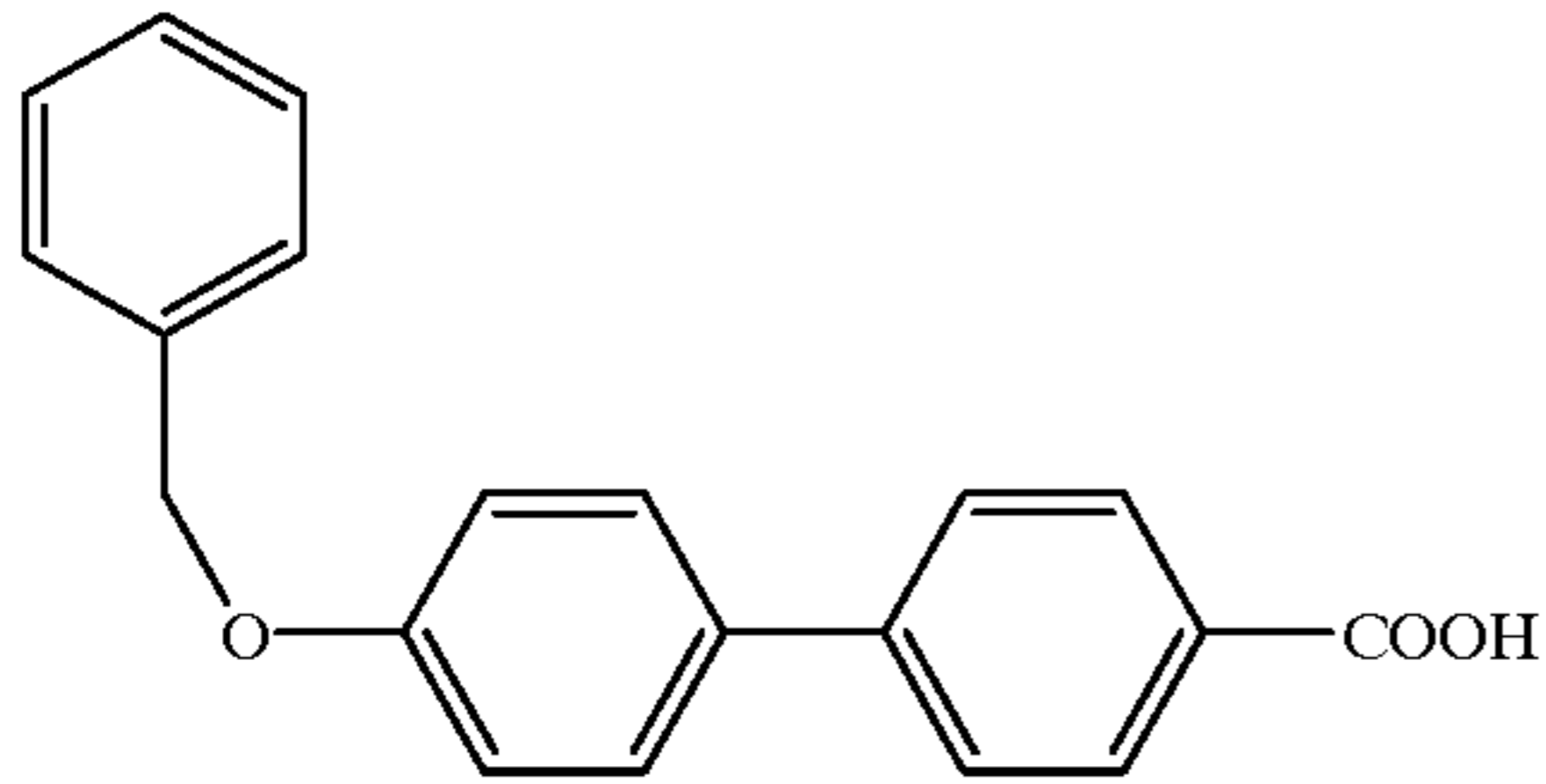
Compound 106
