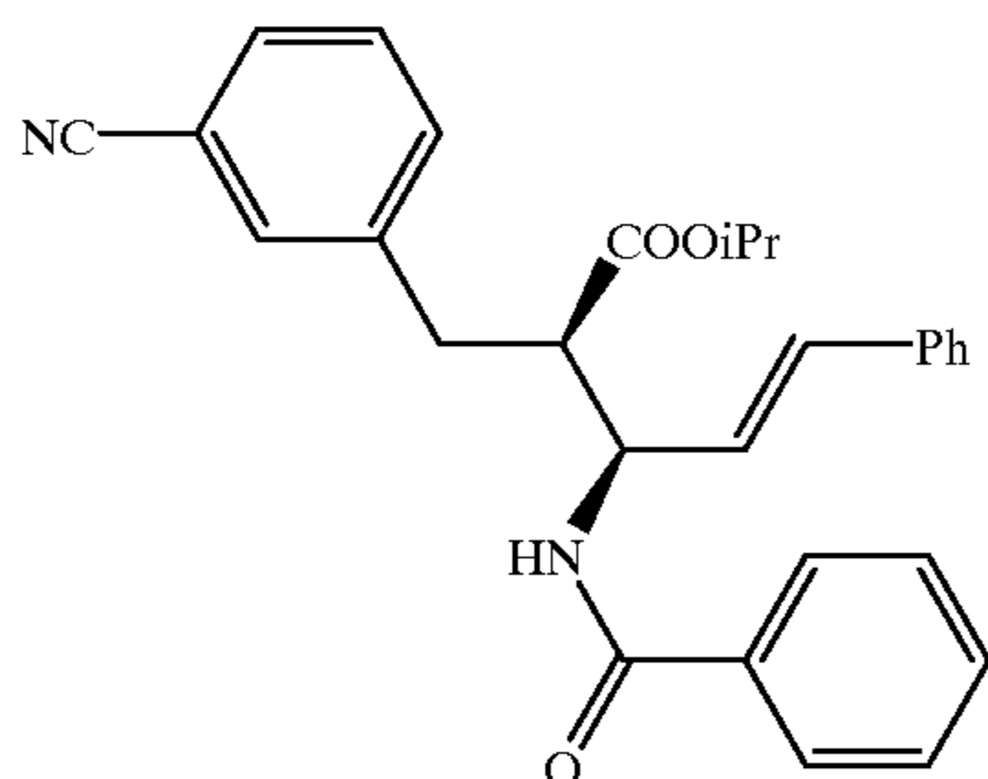
Compound 45
