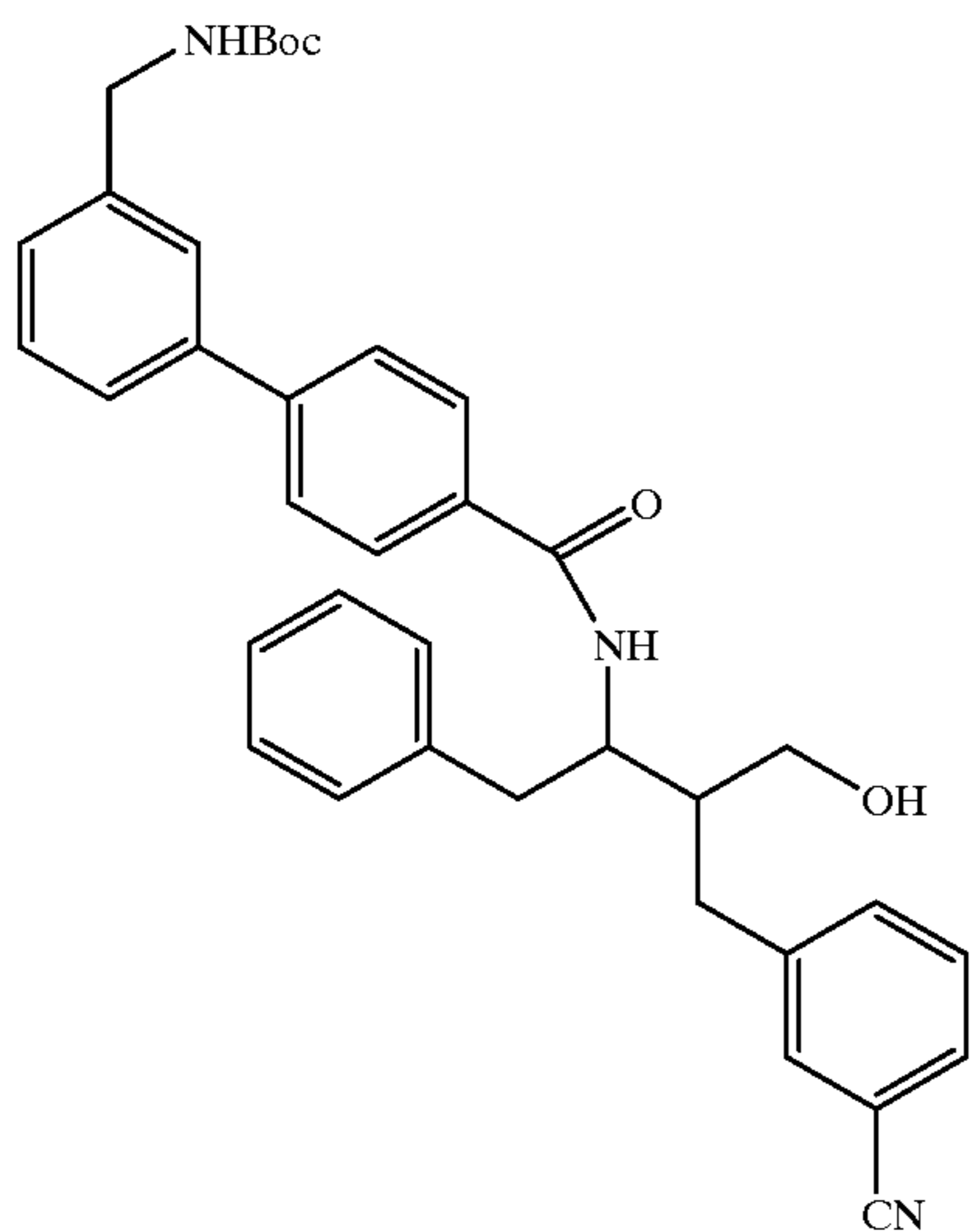
Compound 135
