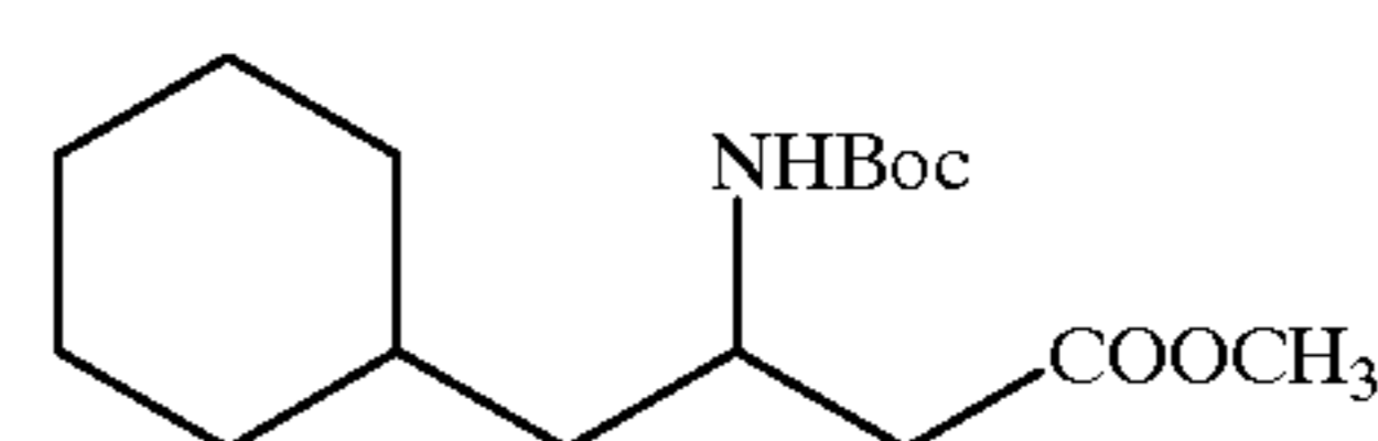
Compound 61
