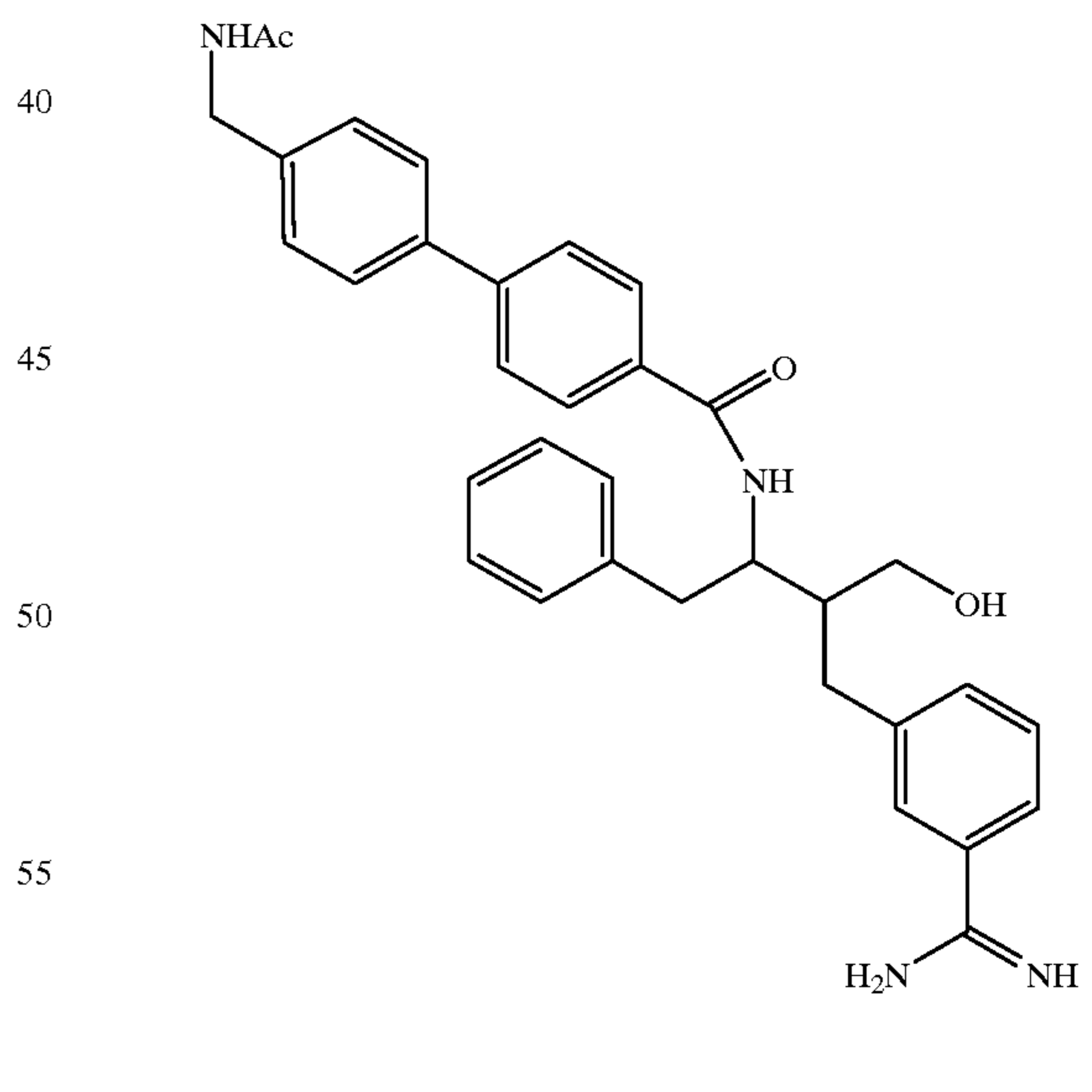
Compound 173
