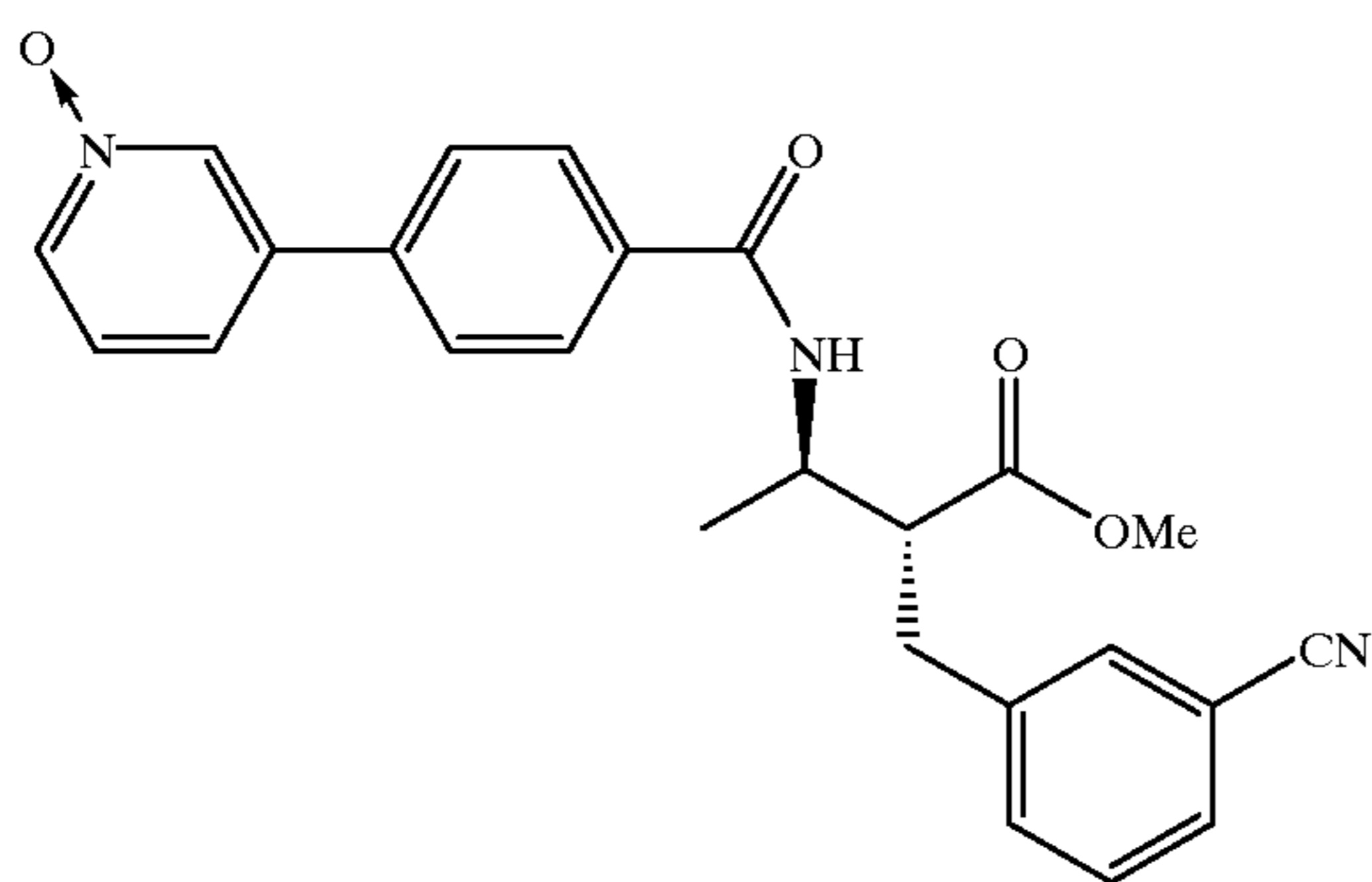
Compound 208
