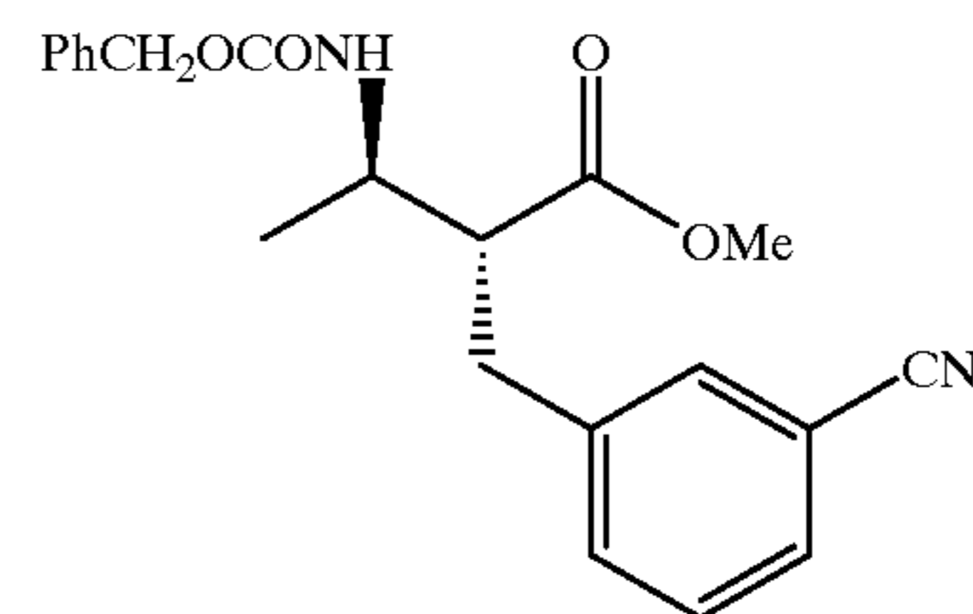
Compound 201
