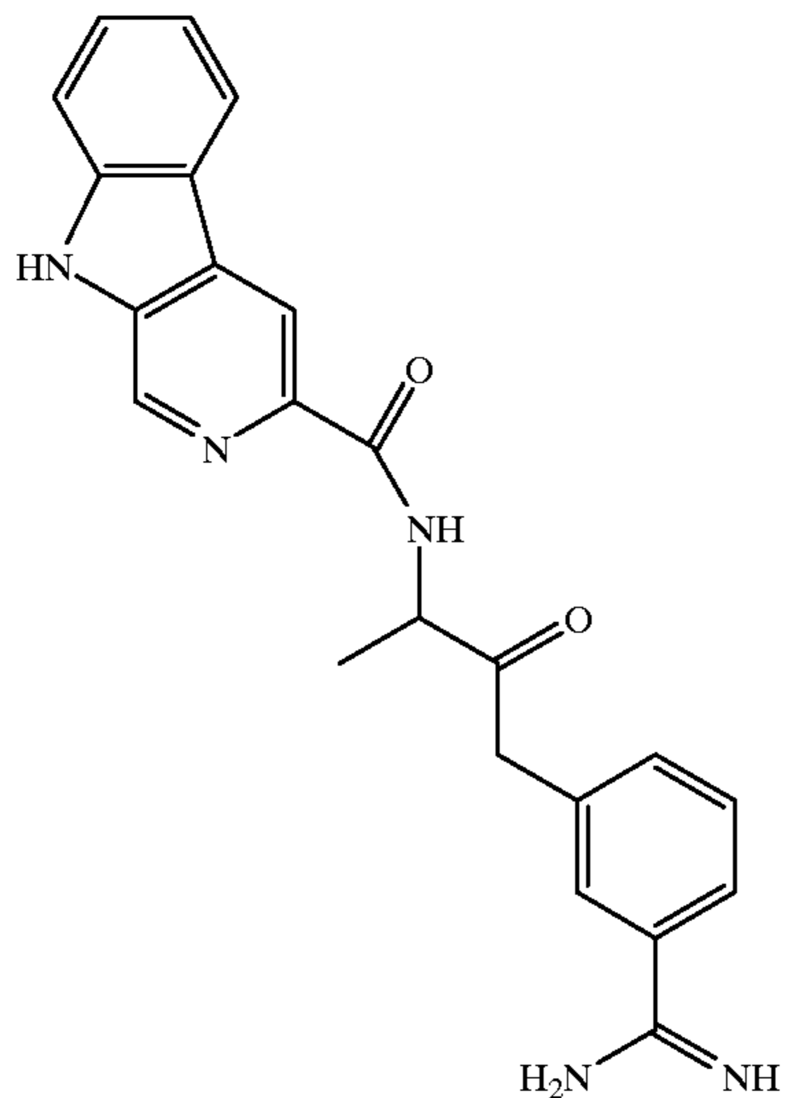
Compound 292
