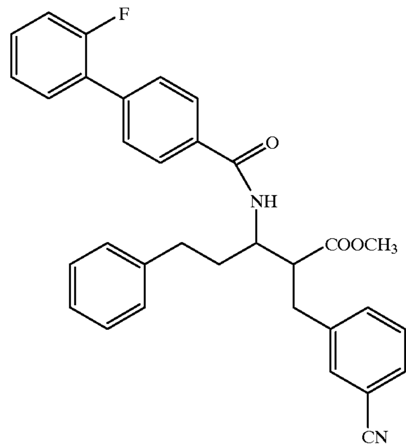
Compound 108
