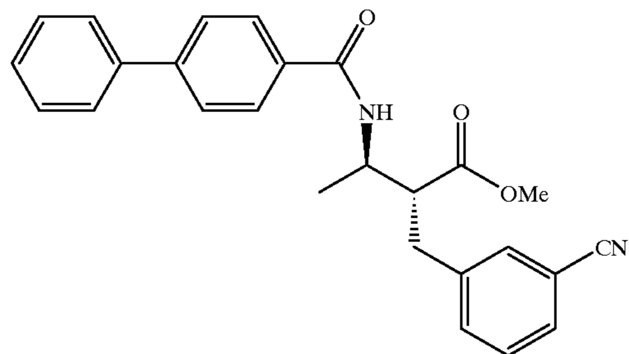
Compound 205
