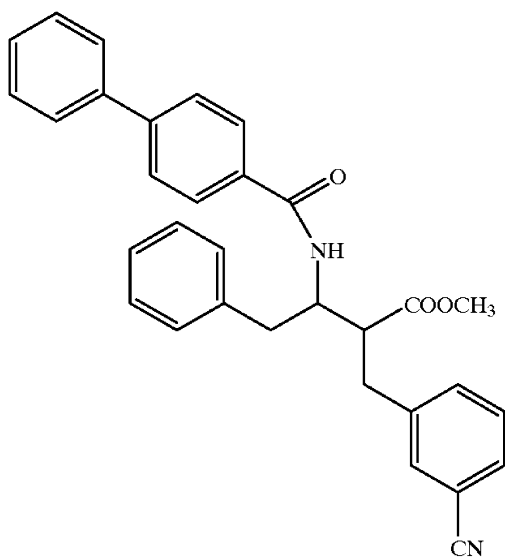
Compound 111
