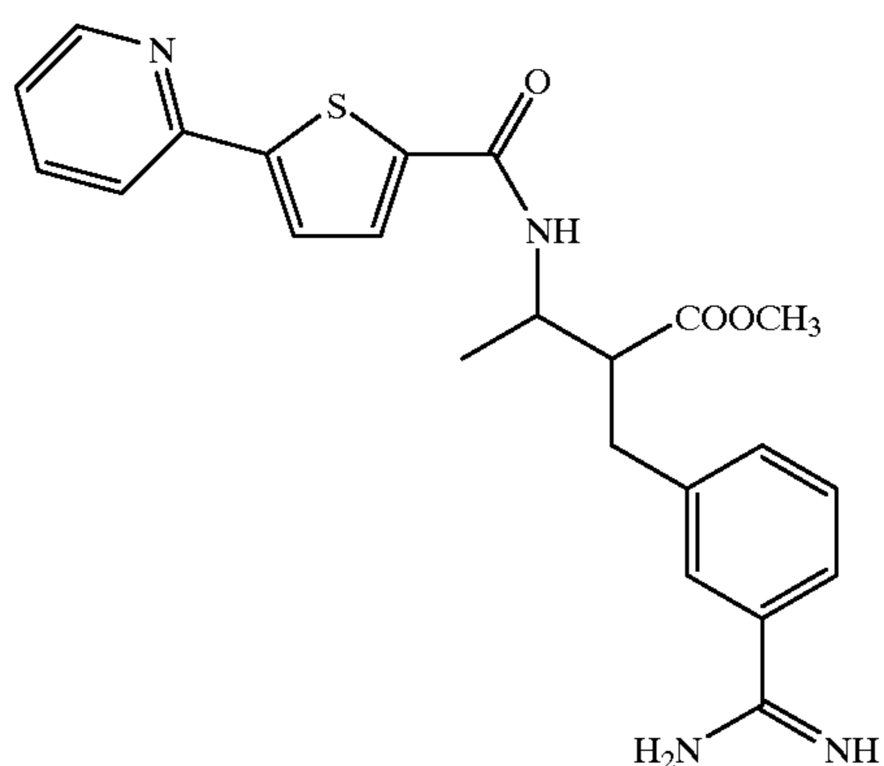
Compound 273
