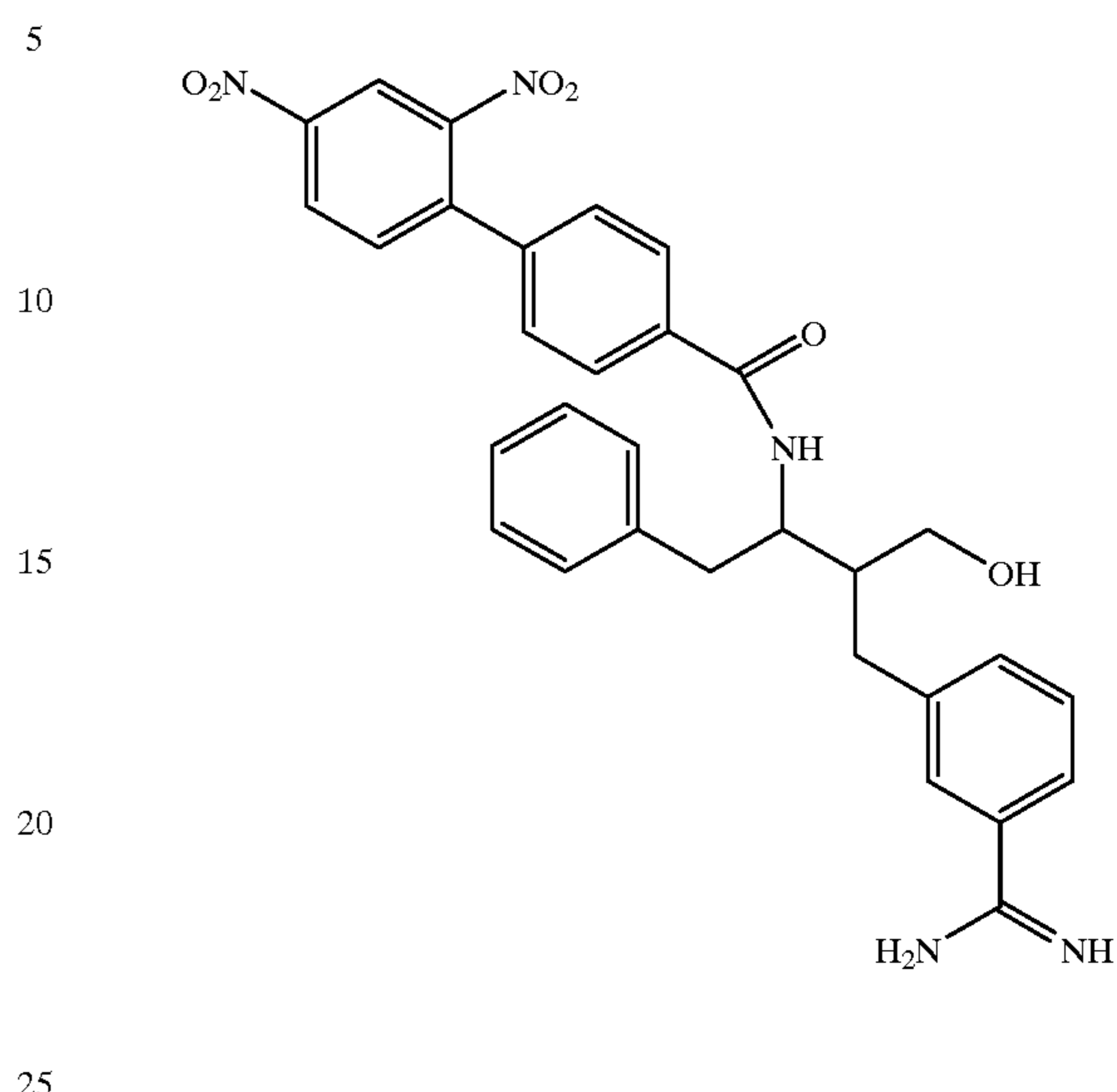
Compound 176
