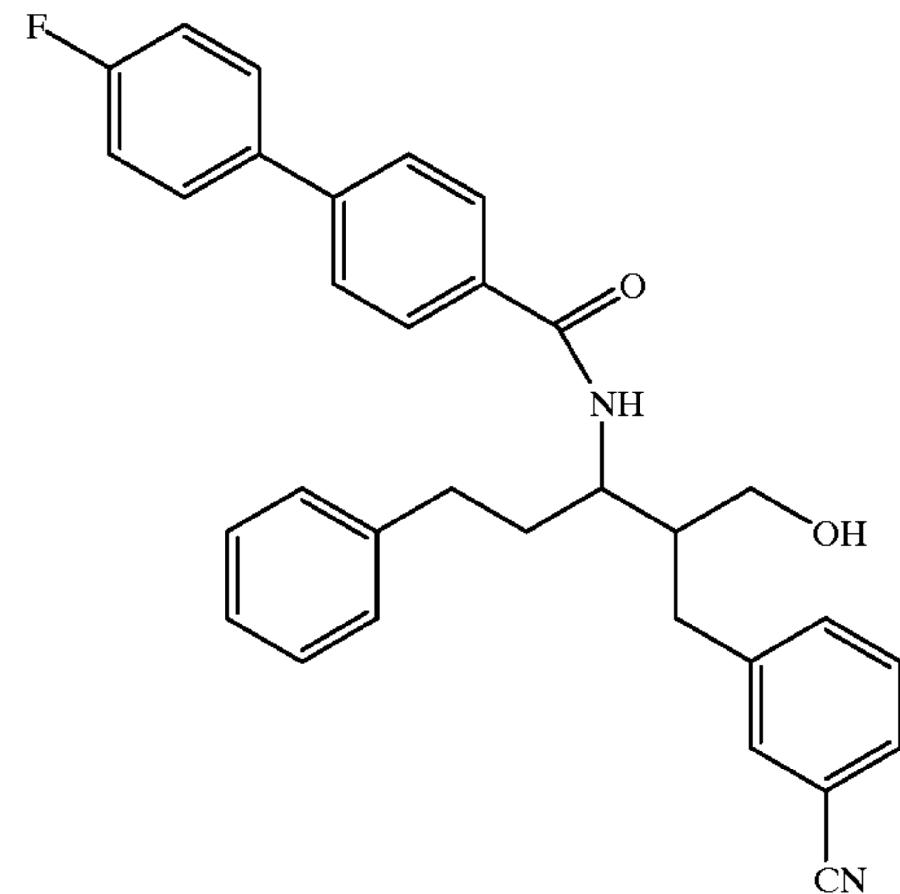
Compound 132
