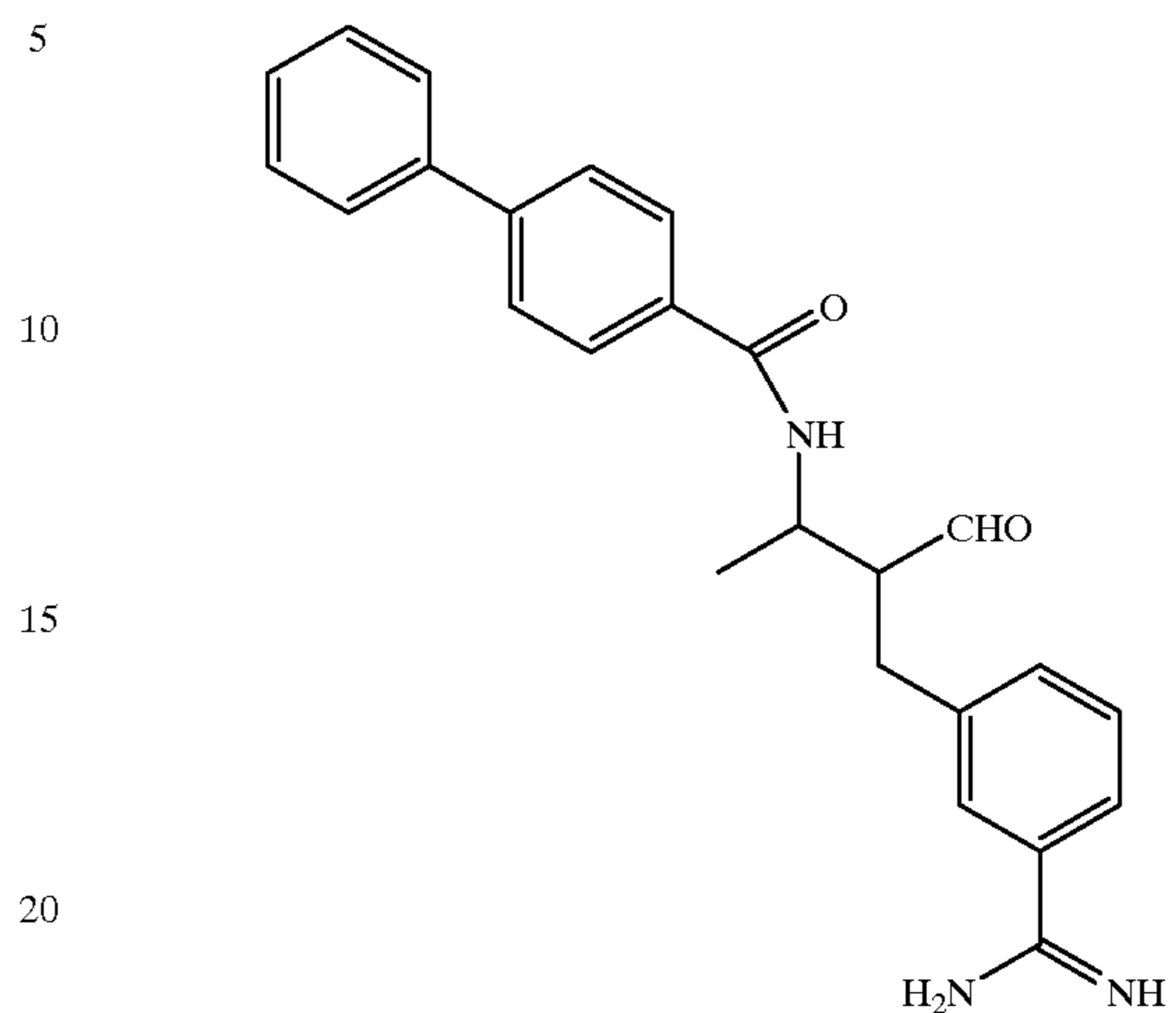
Compound 196
