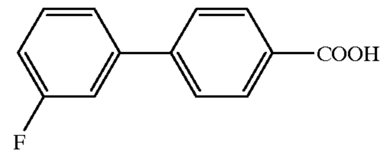
Compound 94
