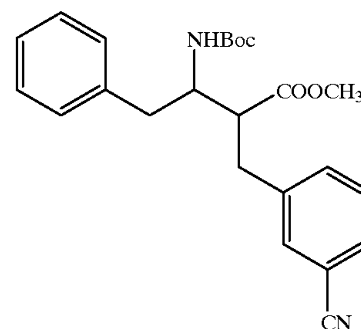
Compound 62
