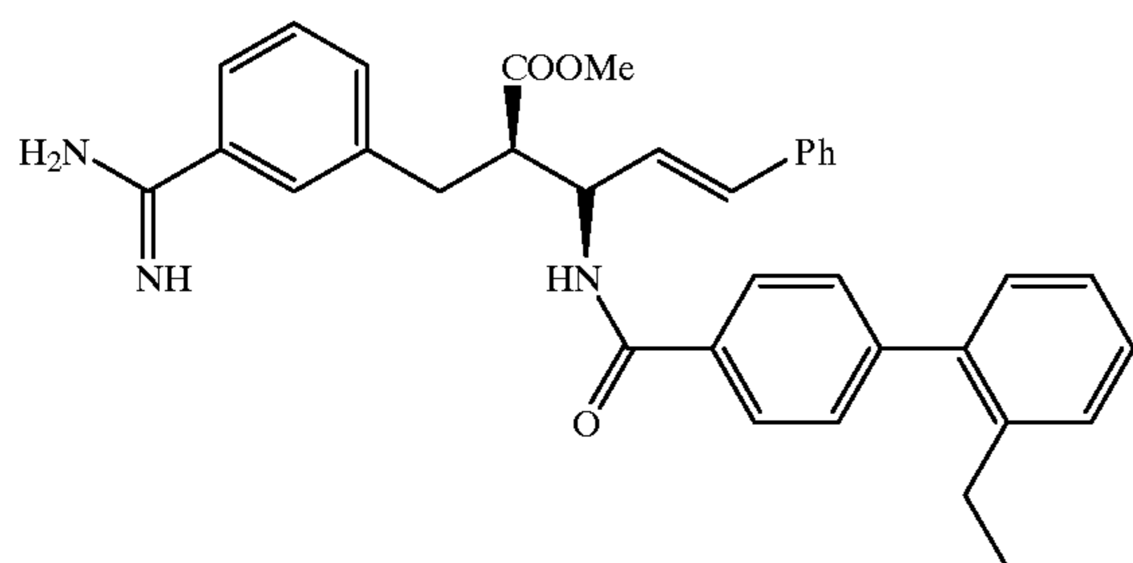
Compound 28
