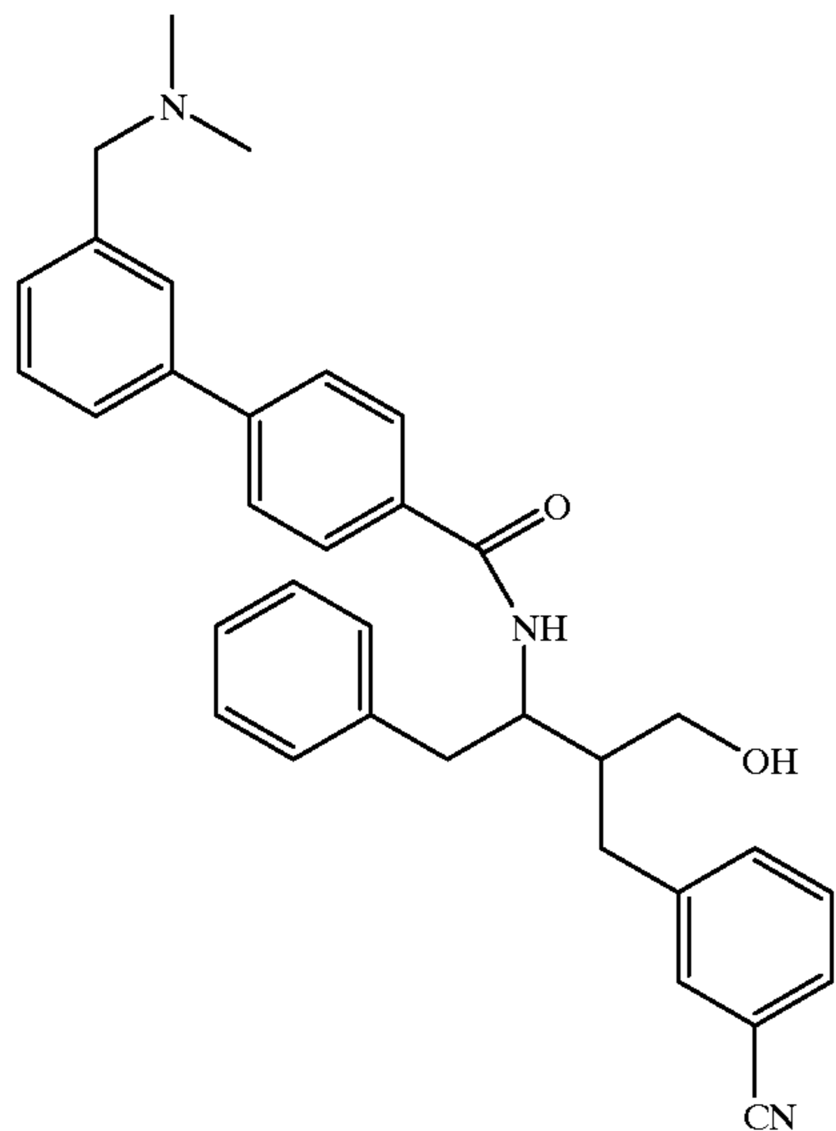
Compound 154
