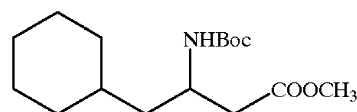
Compound 61
