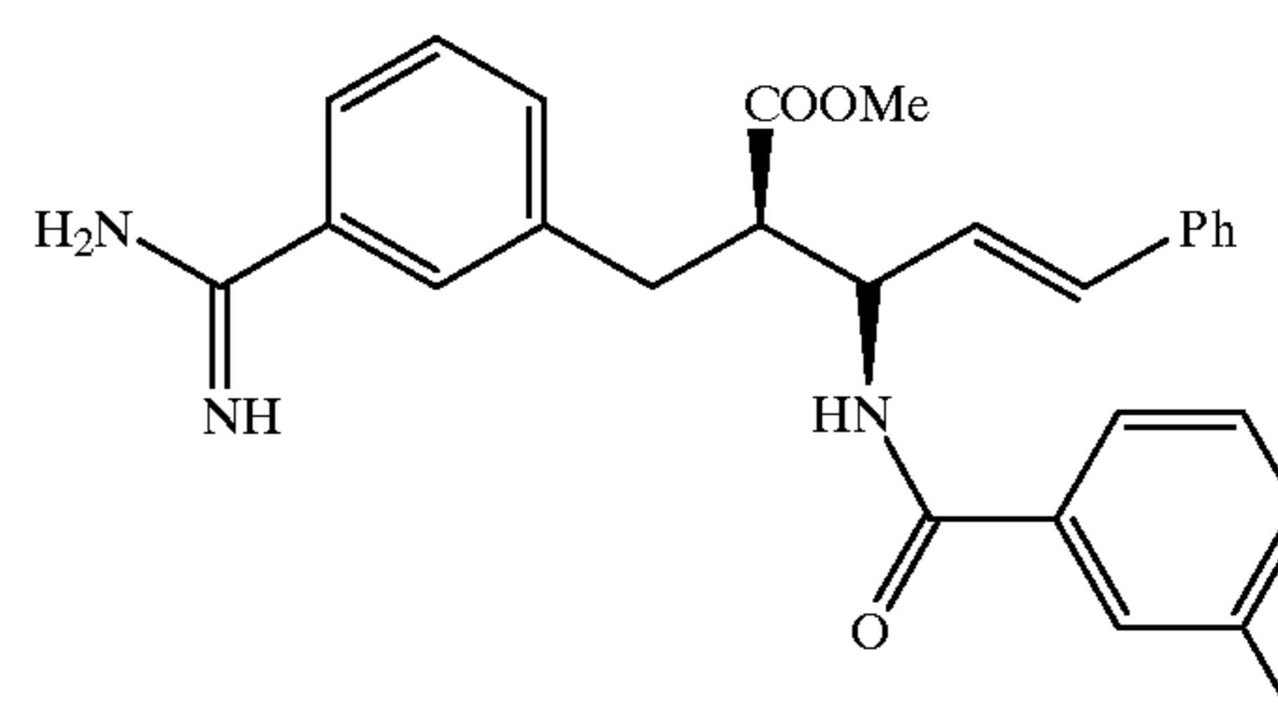
Compound 13
