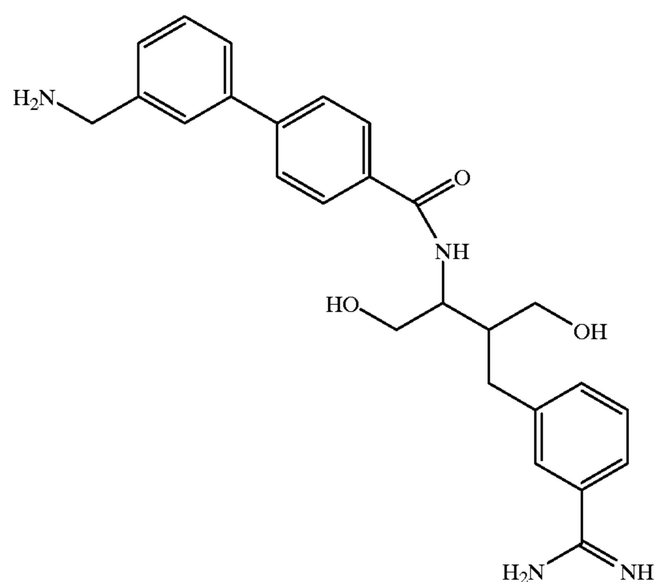
Compound 299
