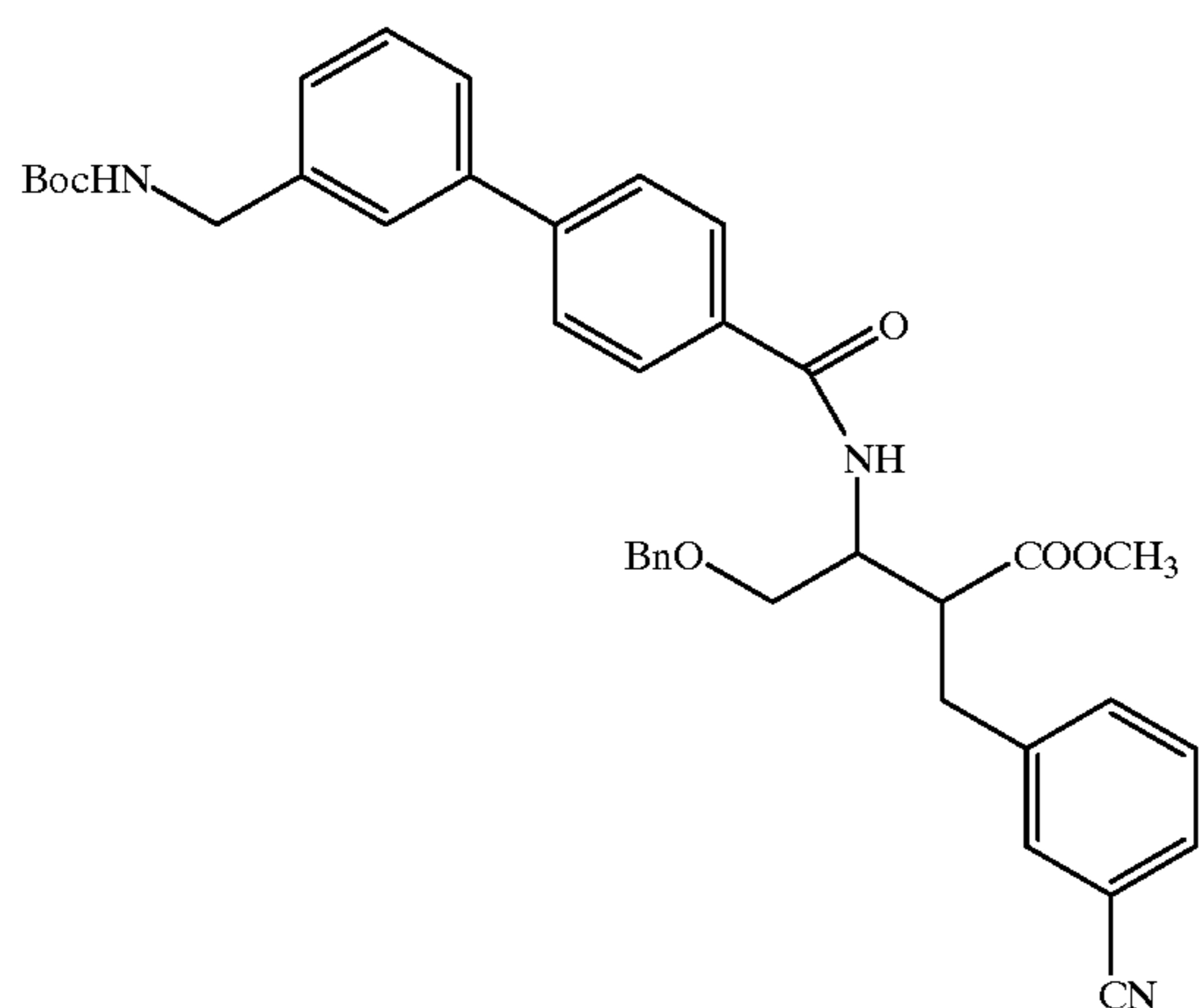
Compound 265
