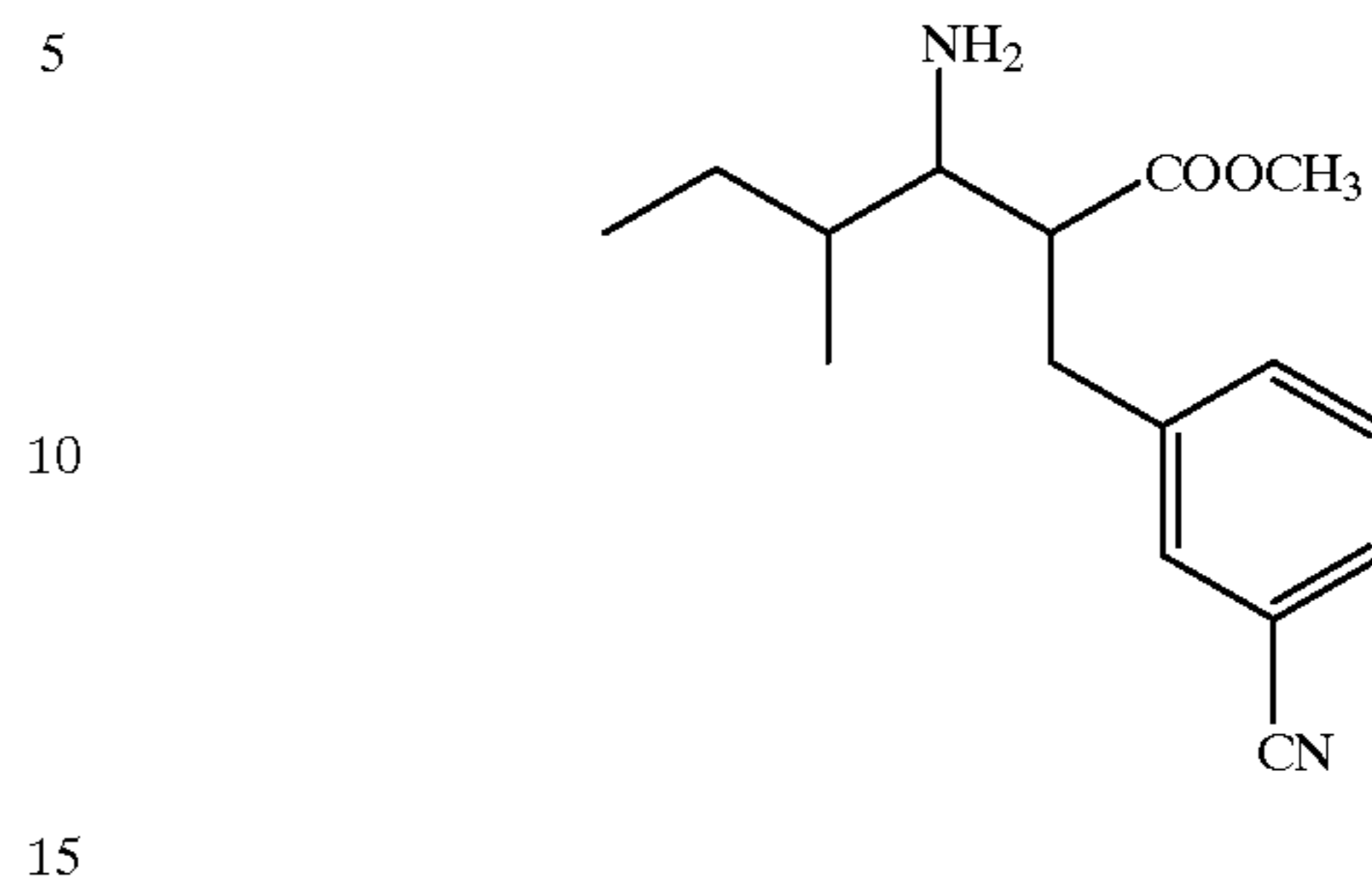
Compound 72
