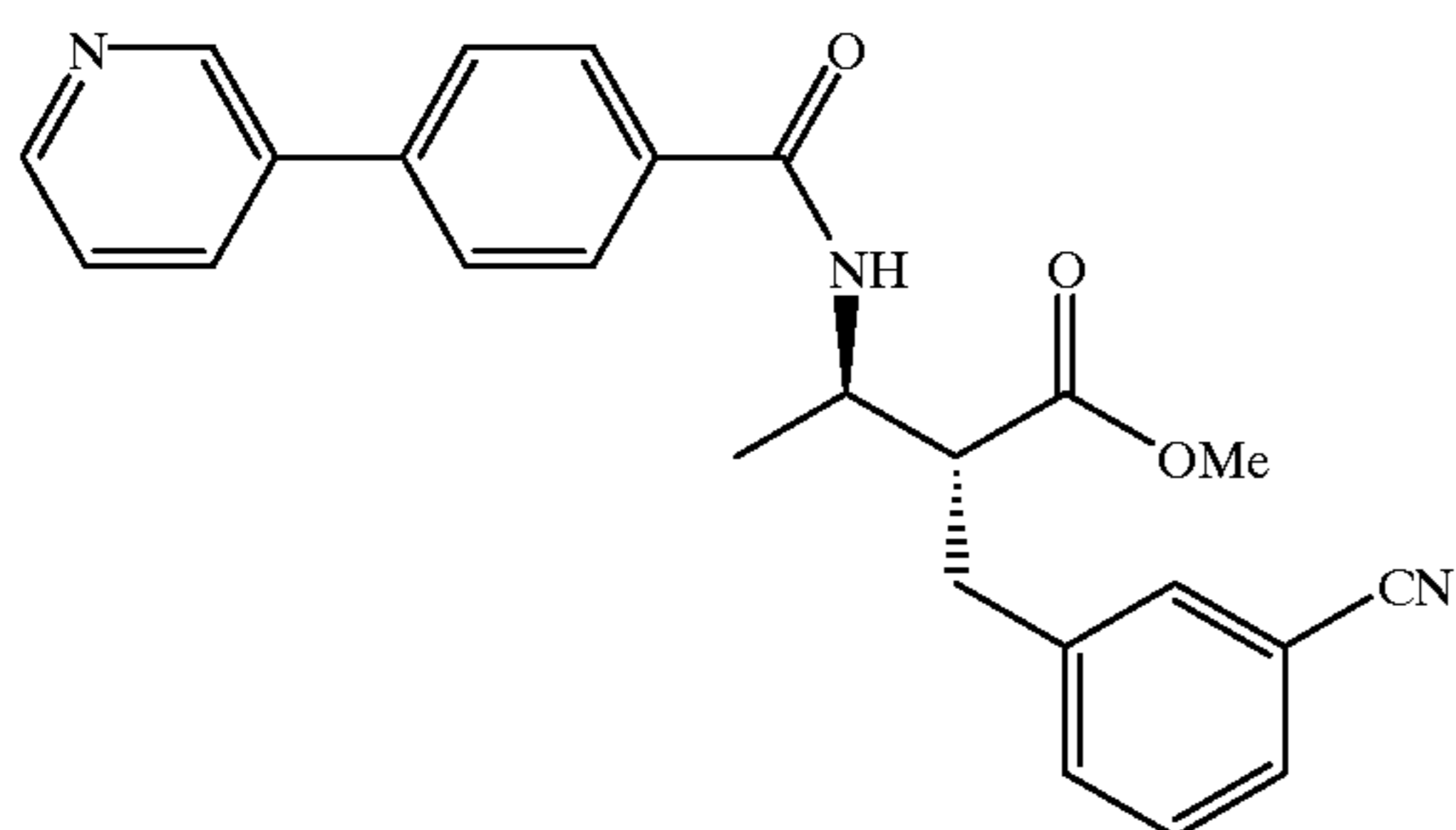
Compound 203
