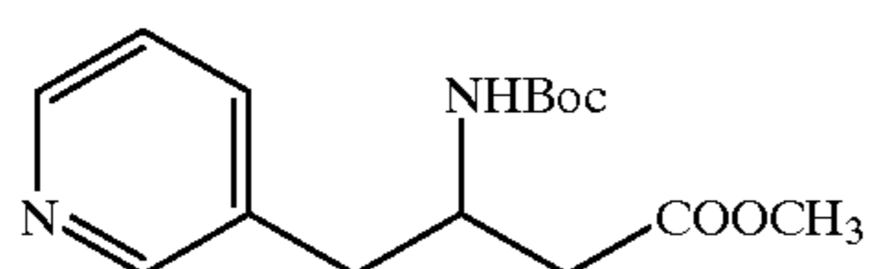
Compound 59
