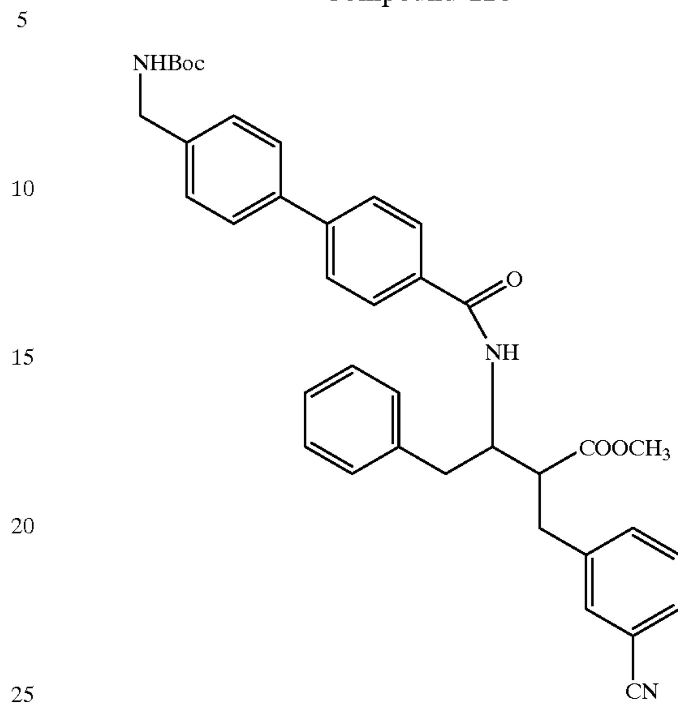
Compound 116
