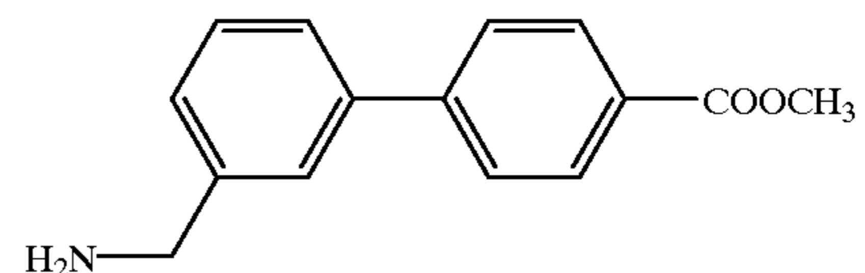
Compound 81
