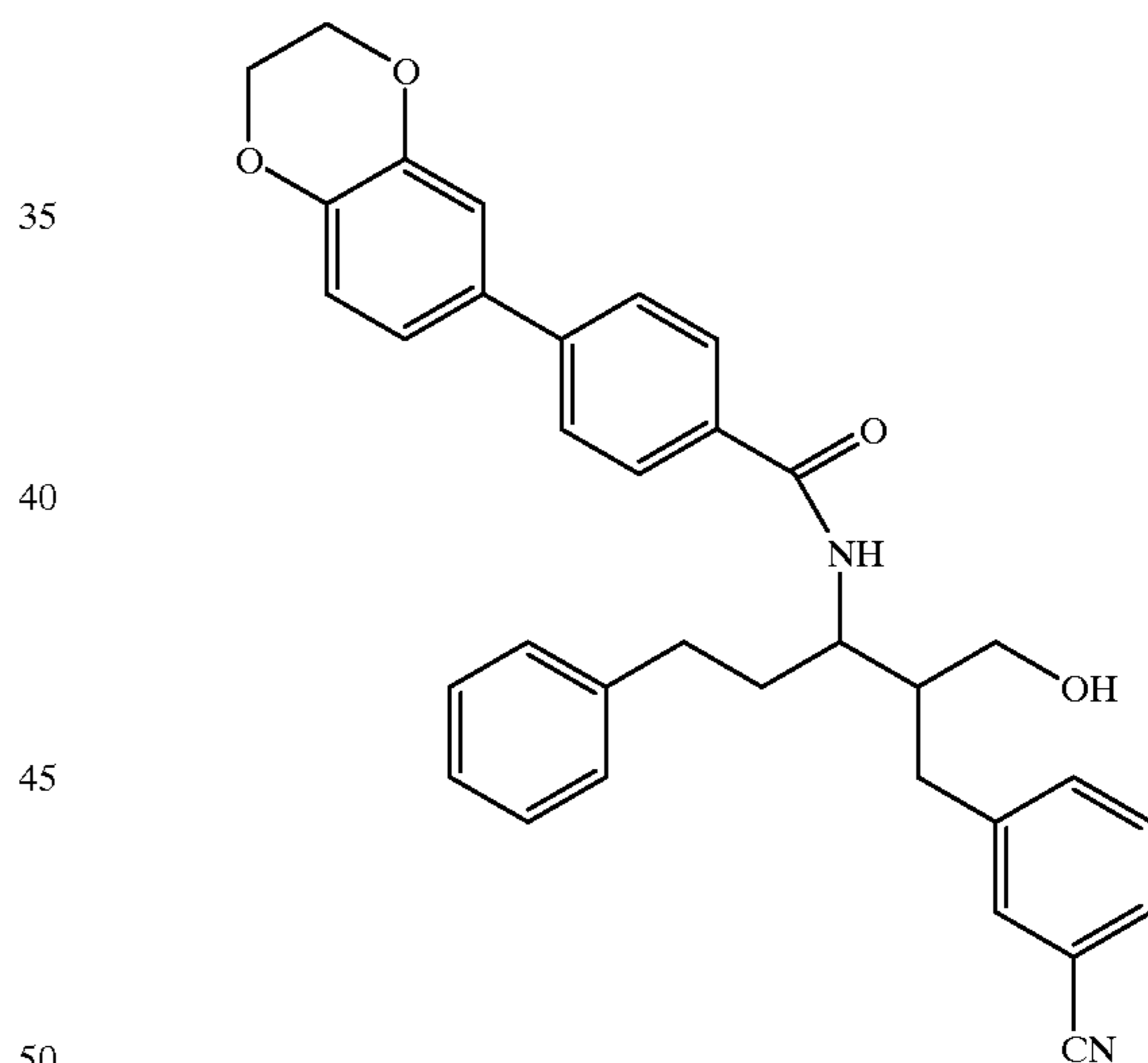
Compound 129
