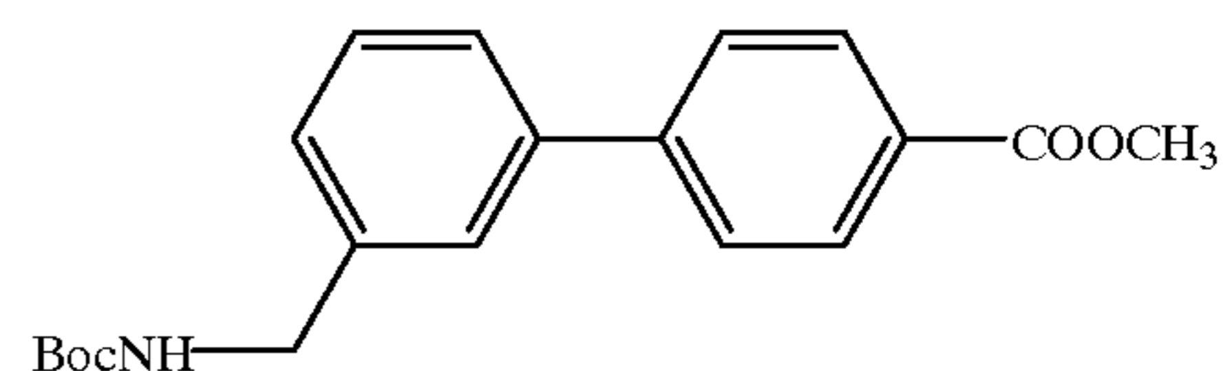
Compound 82
