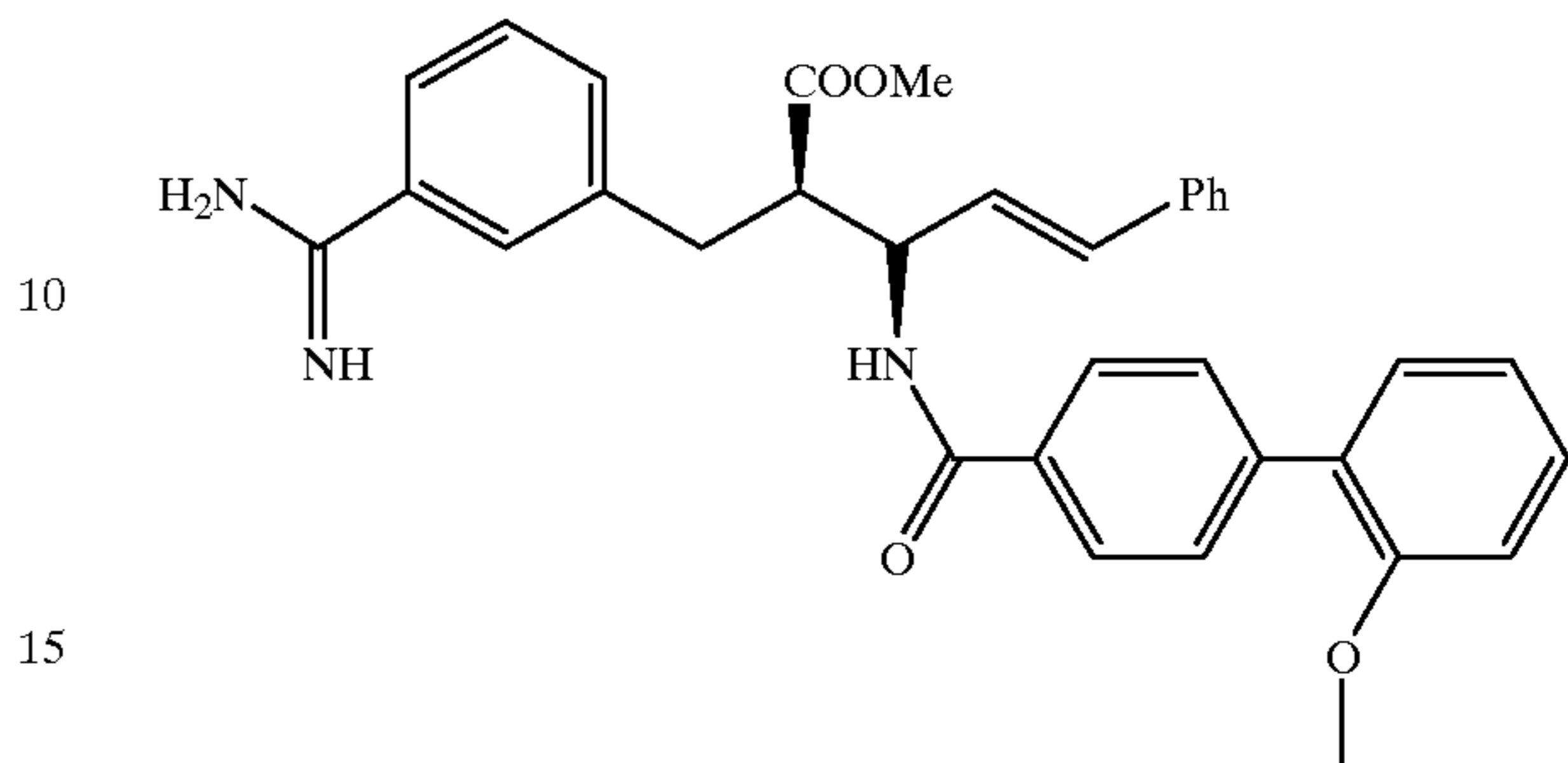
Compound 21
