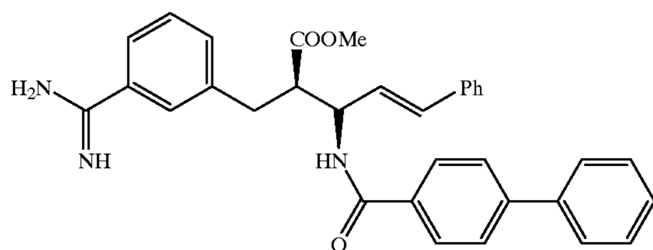
Compound 10
