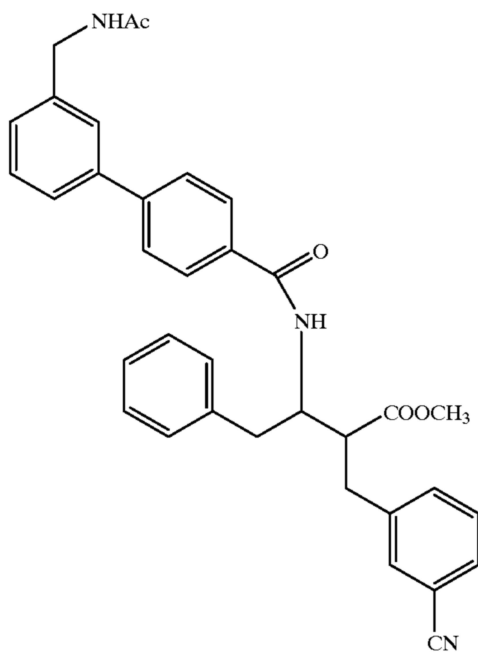
Compound 115
