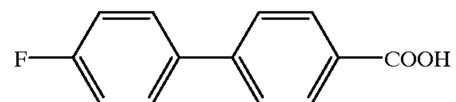
Compound 95
