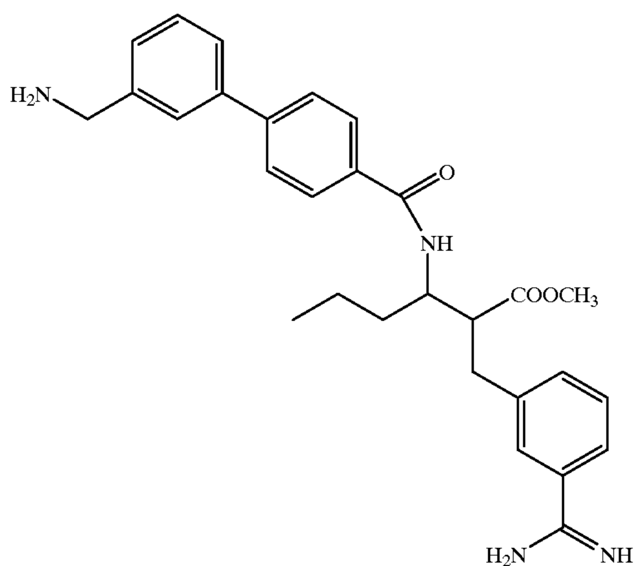
Compound 301
