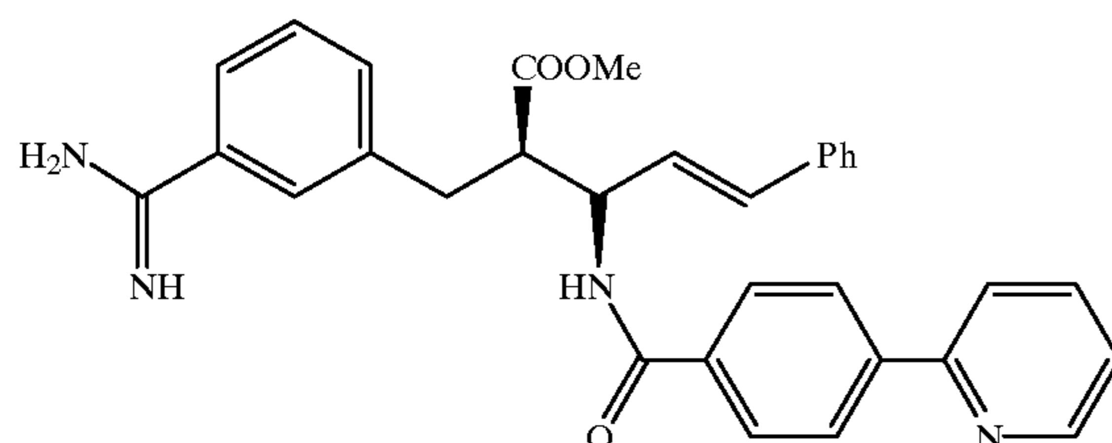
Compound 16
