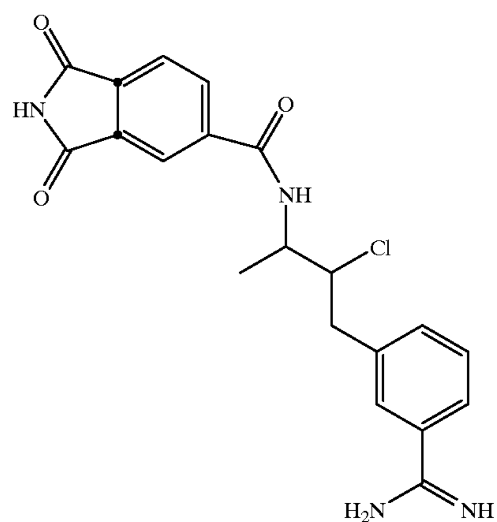
Compound 291
