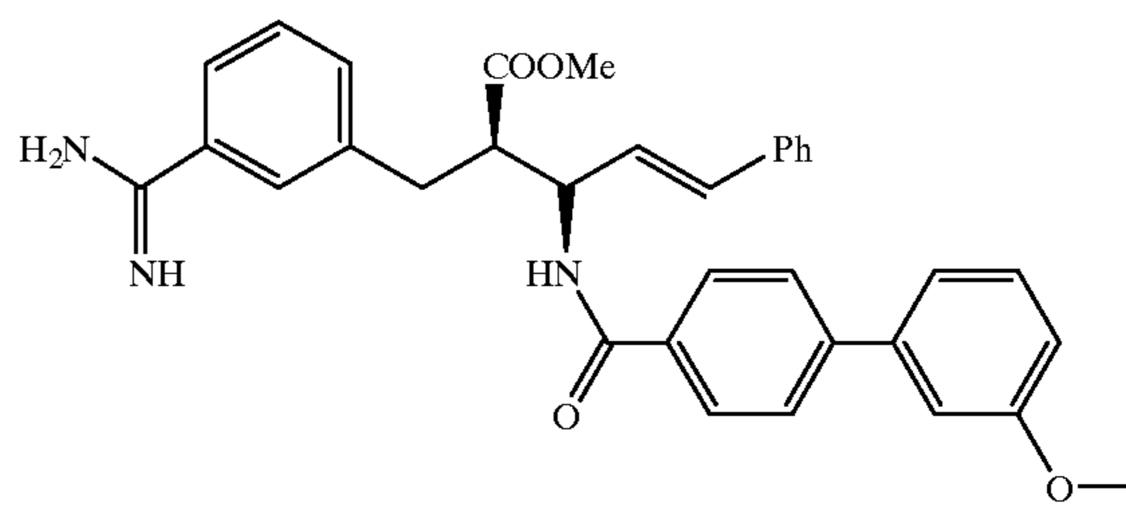
Compound 22
