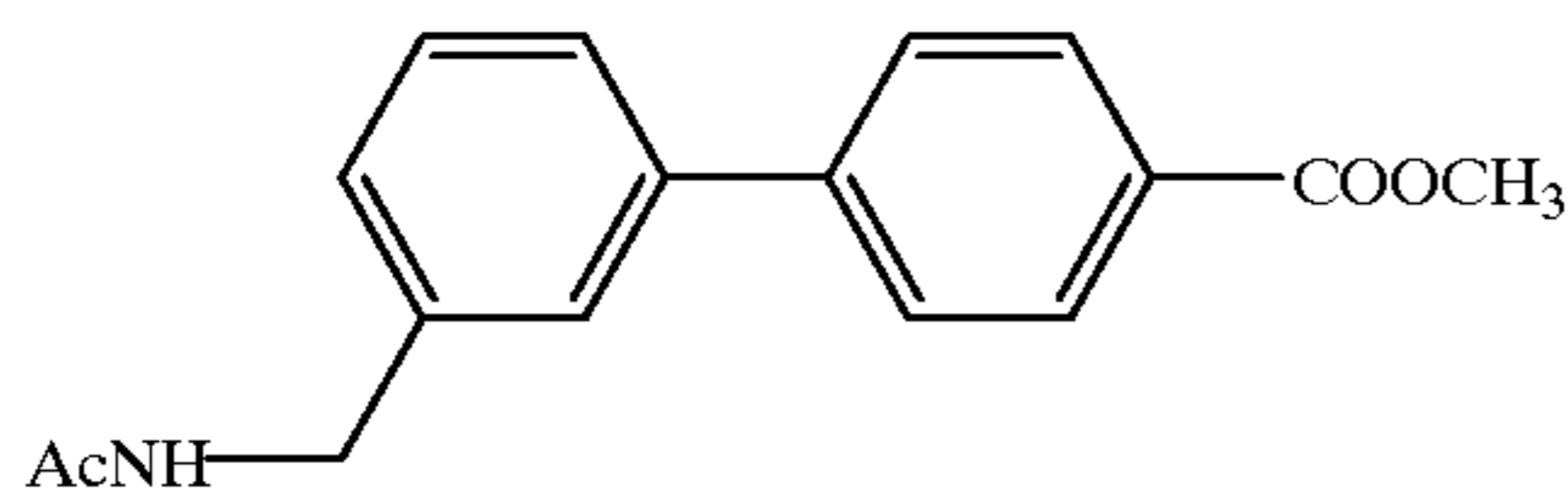
Compound 83
