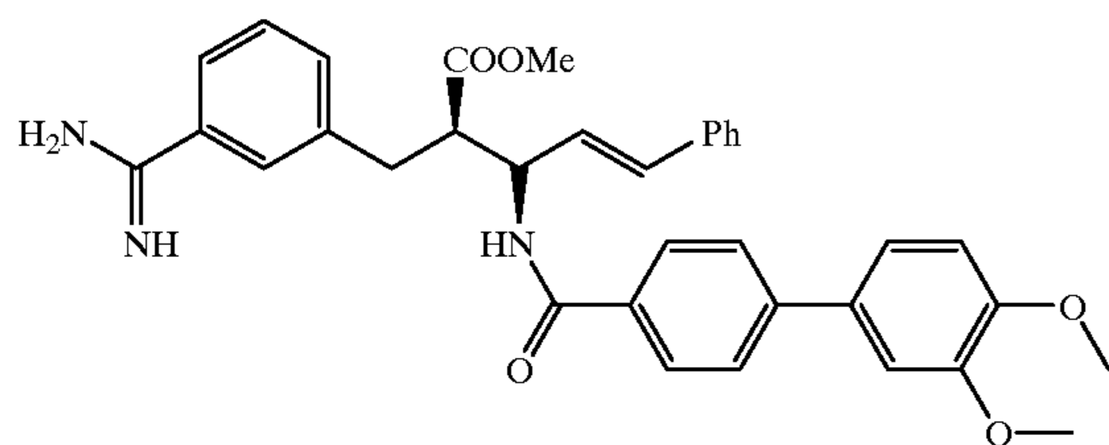
Compound 15
