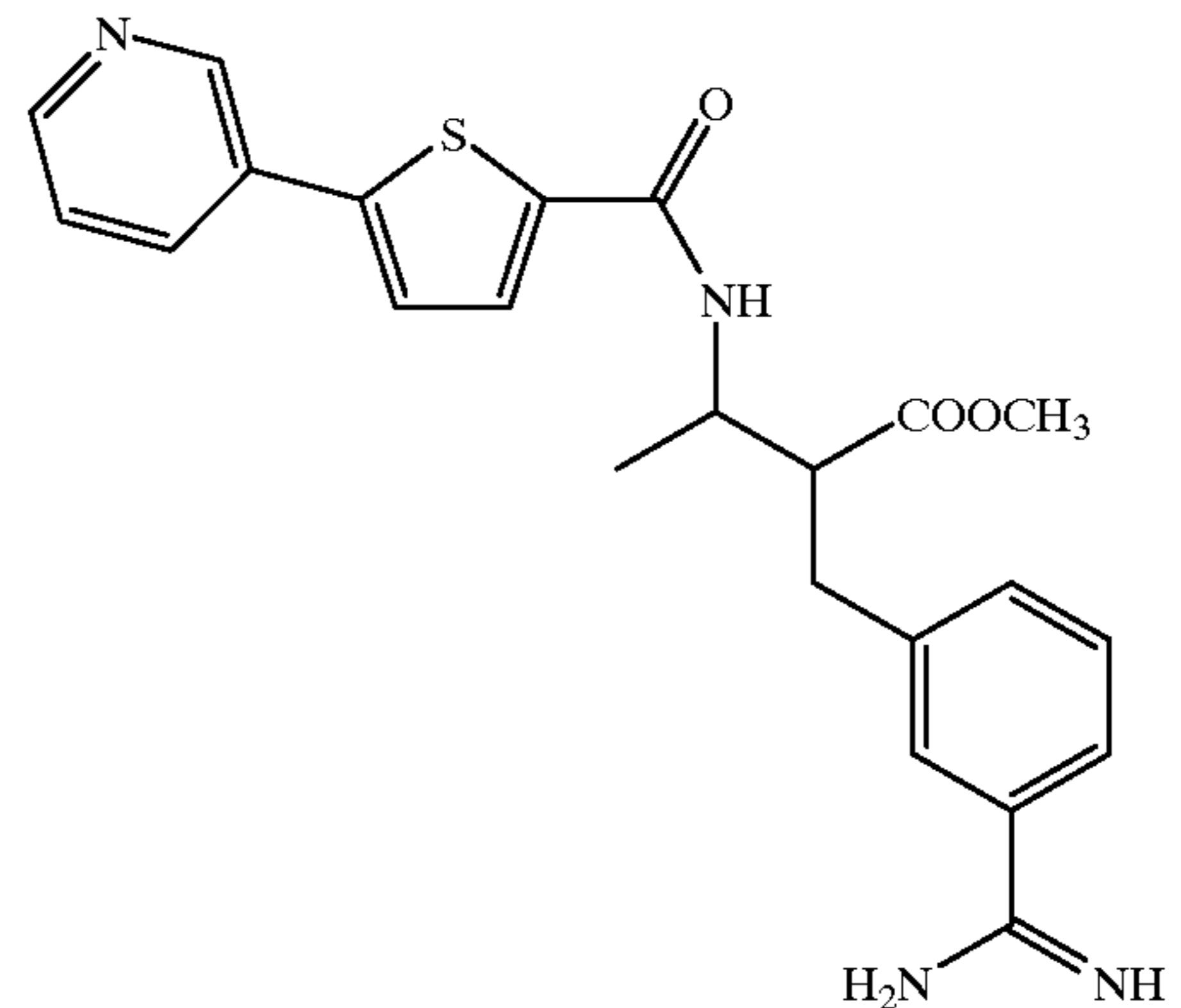
Compound 274
