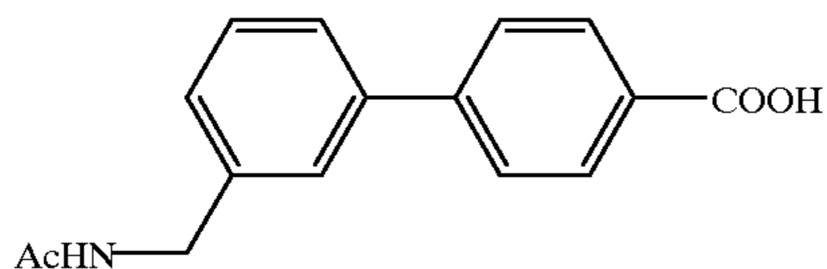
Compound 100
