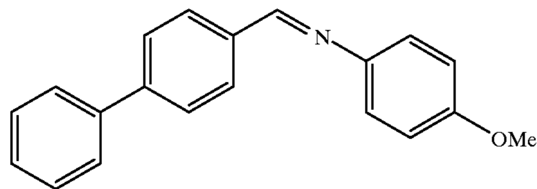
Compound 36
