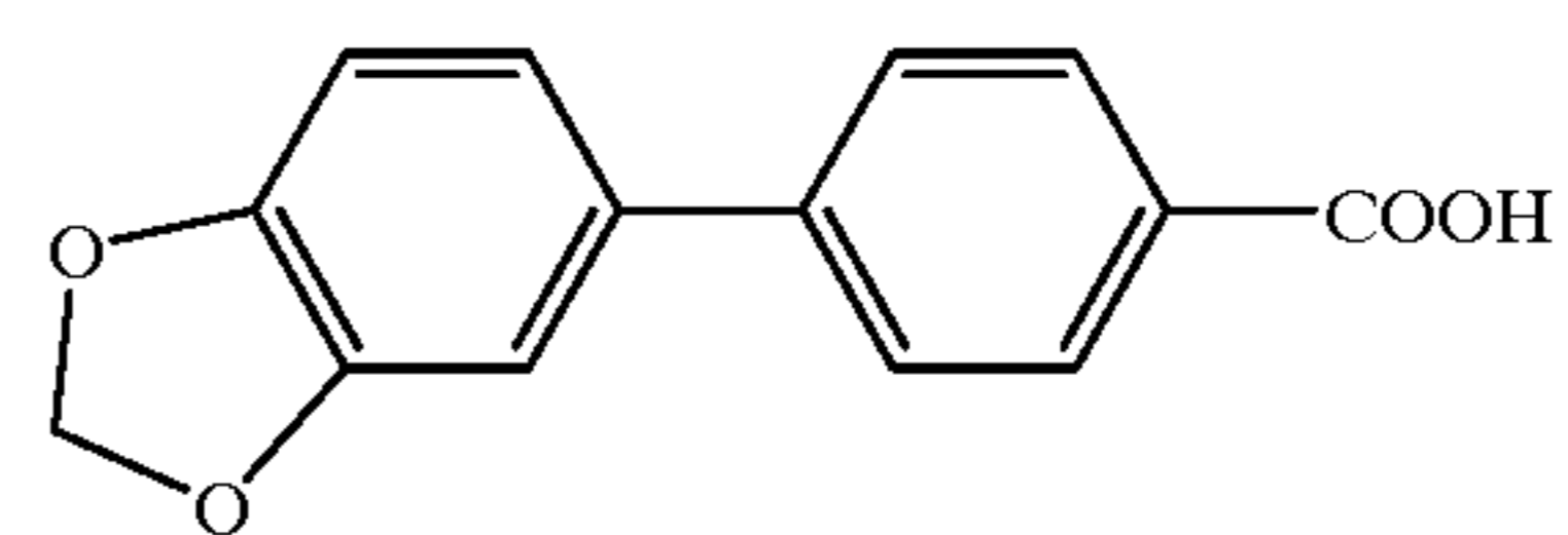
Compound 97
