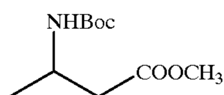
Compound 57
