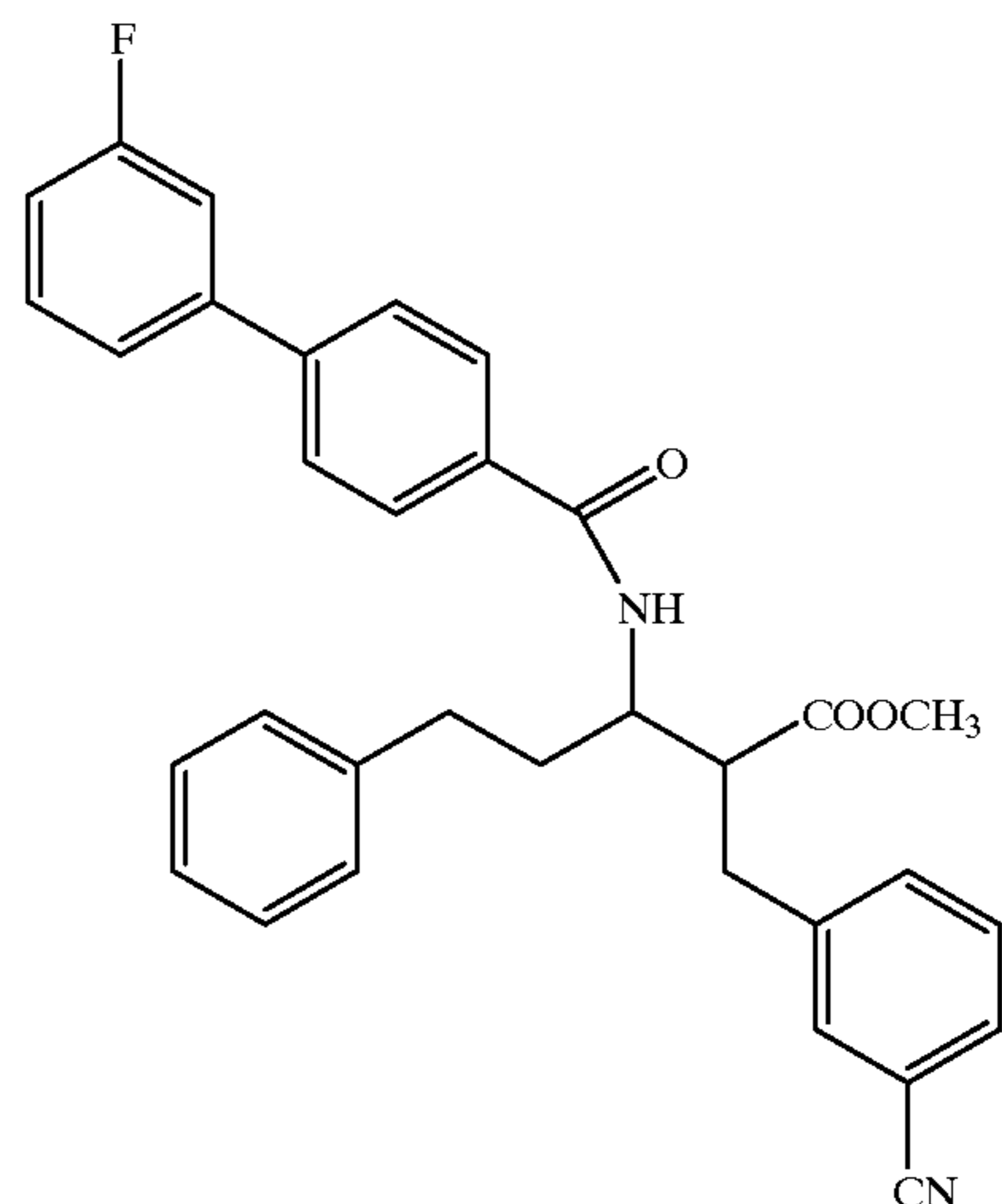
Compound 109
