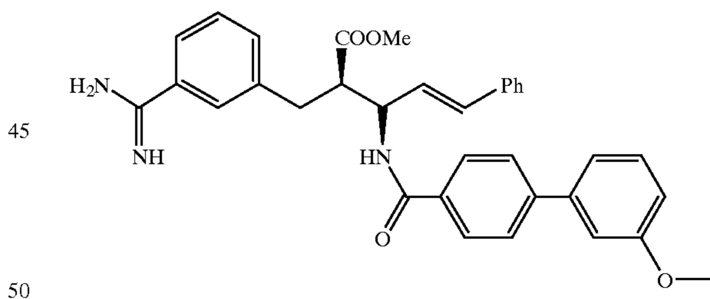
Compound 22
