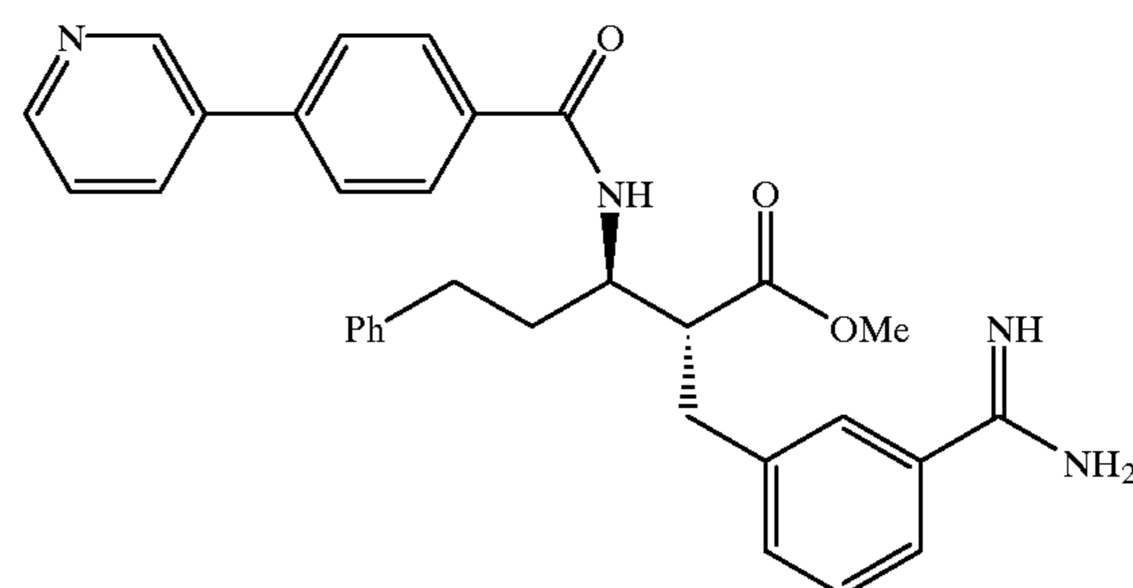
Compound 231
