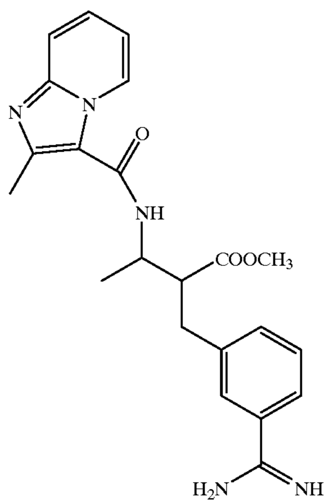
Compound 293
