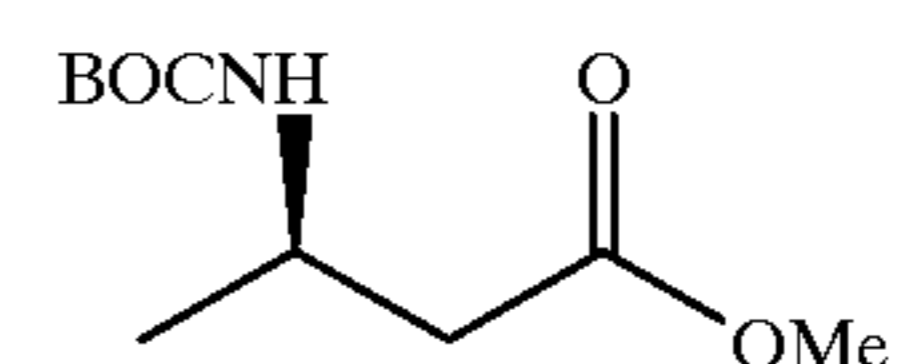
Compound 197
