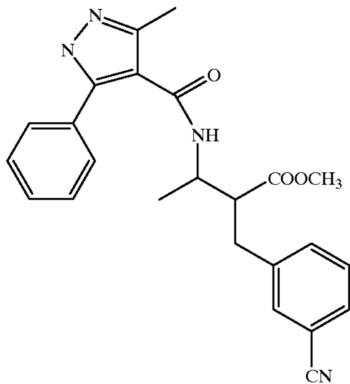
Compound 258
