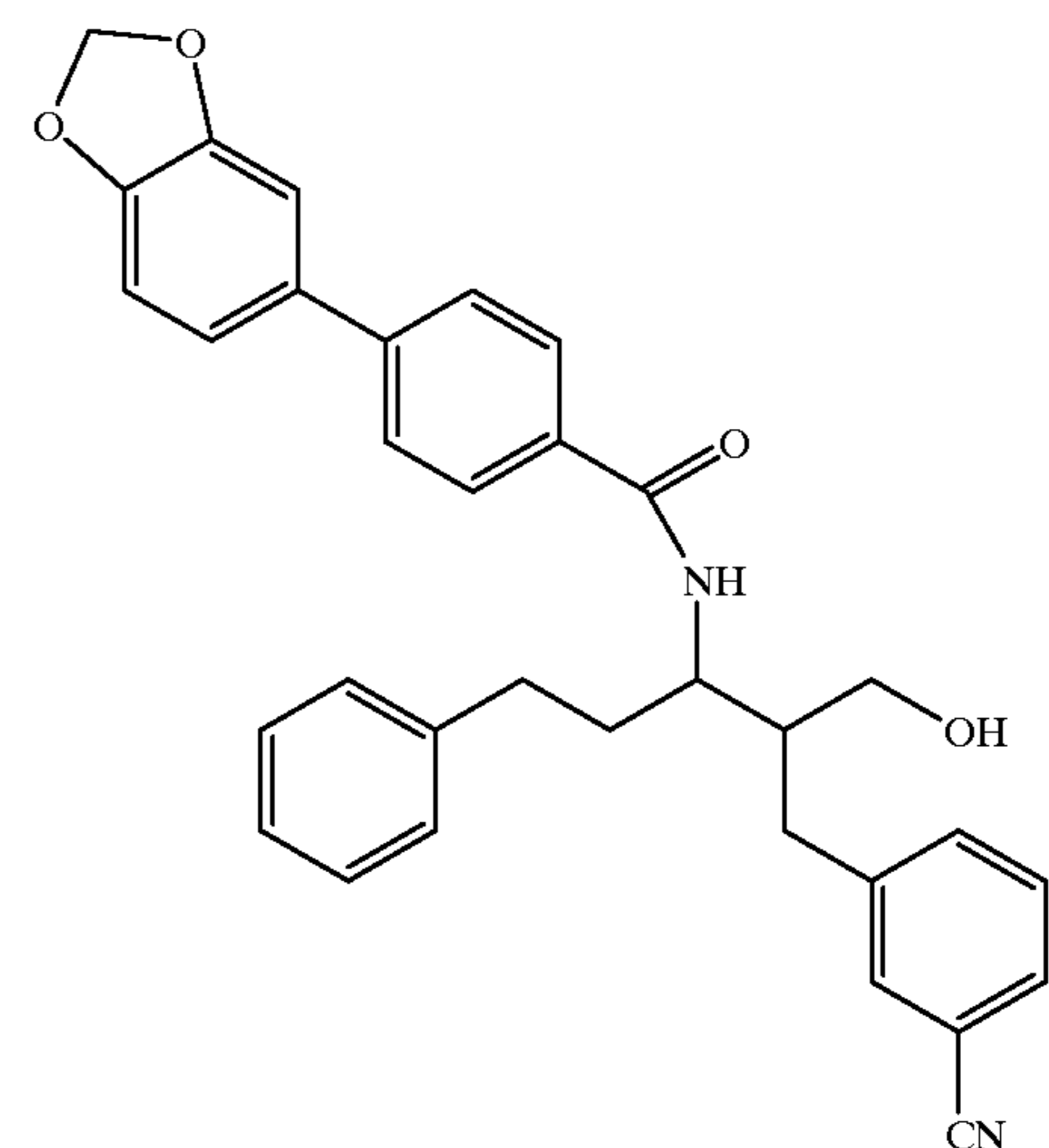
Compound 133
