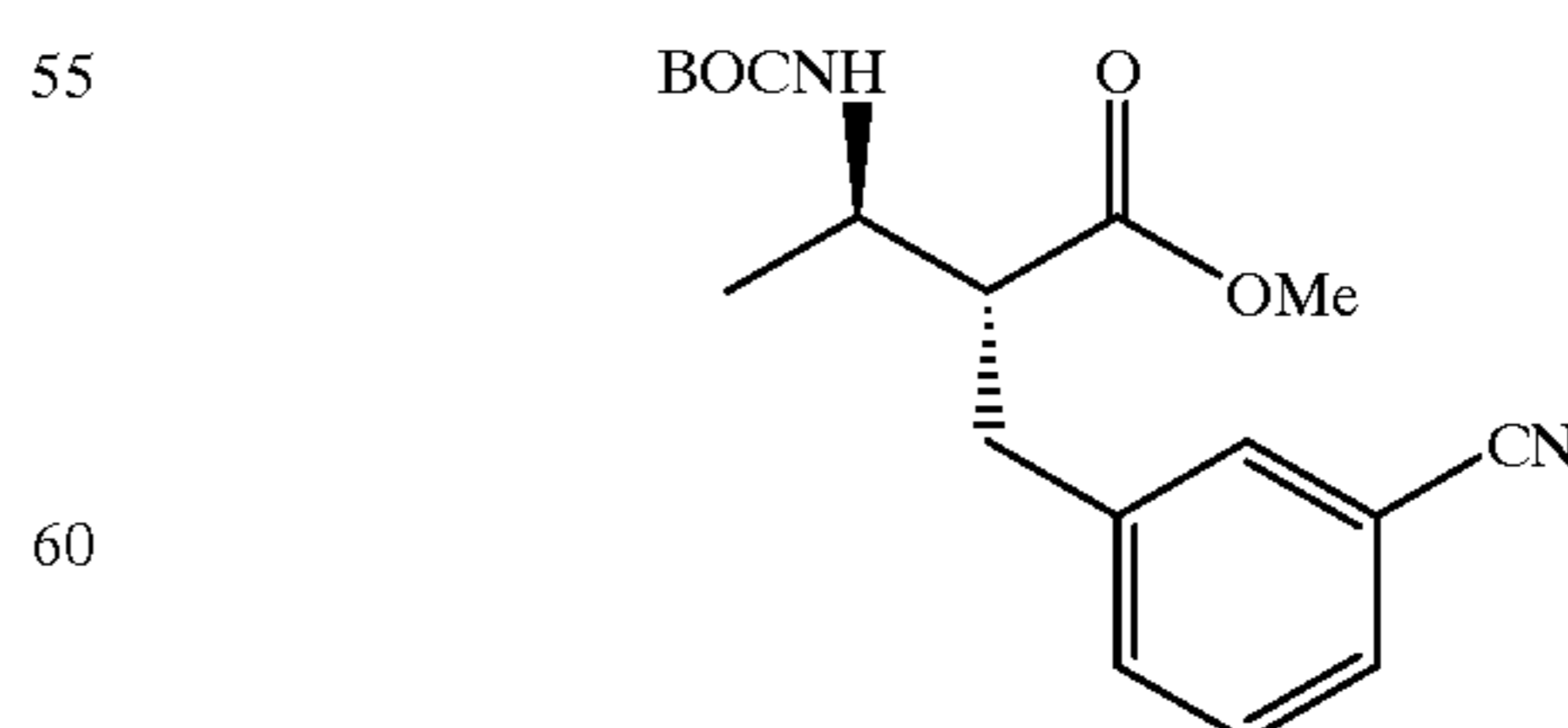
Compound 198
