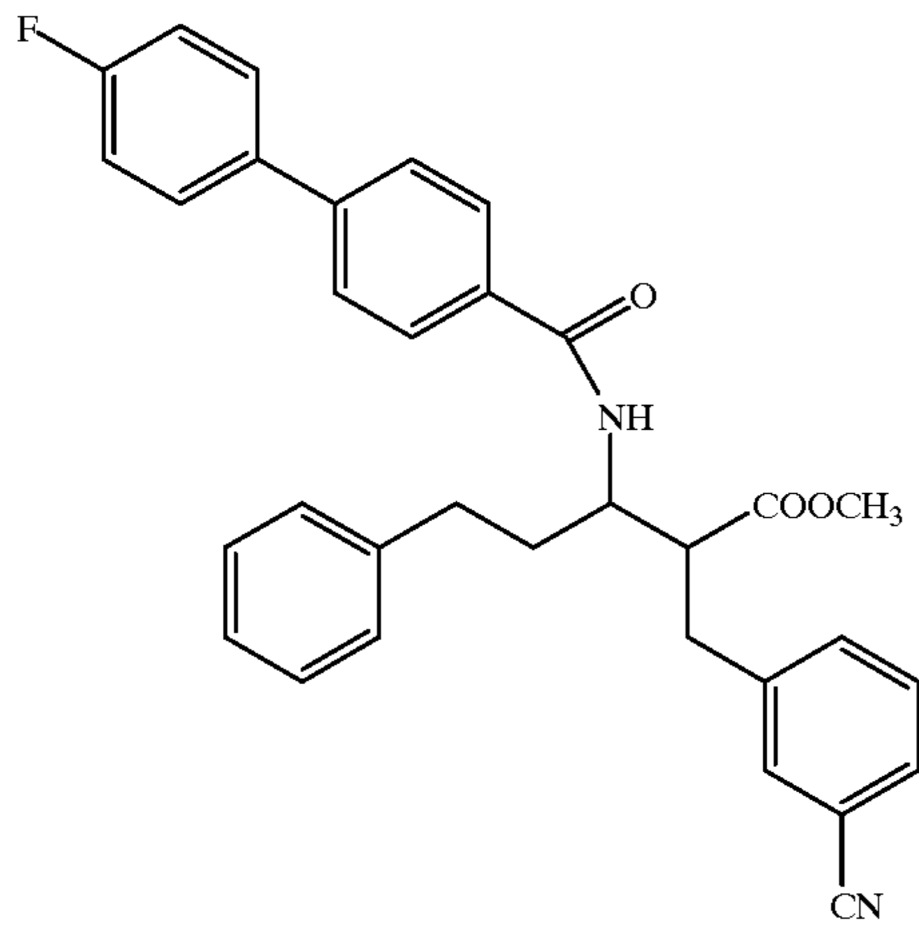
Compound 110
