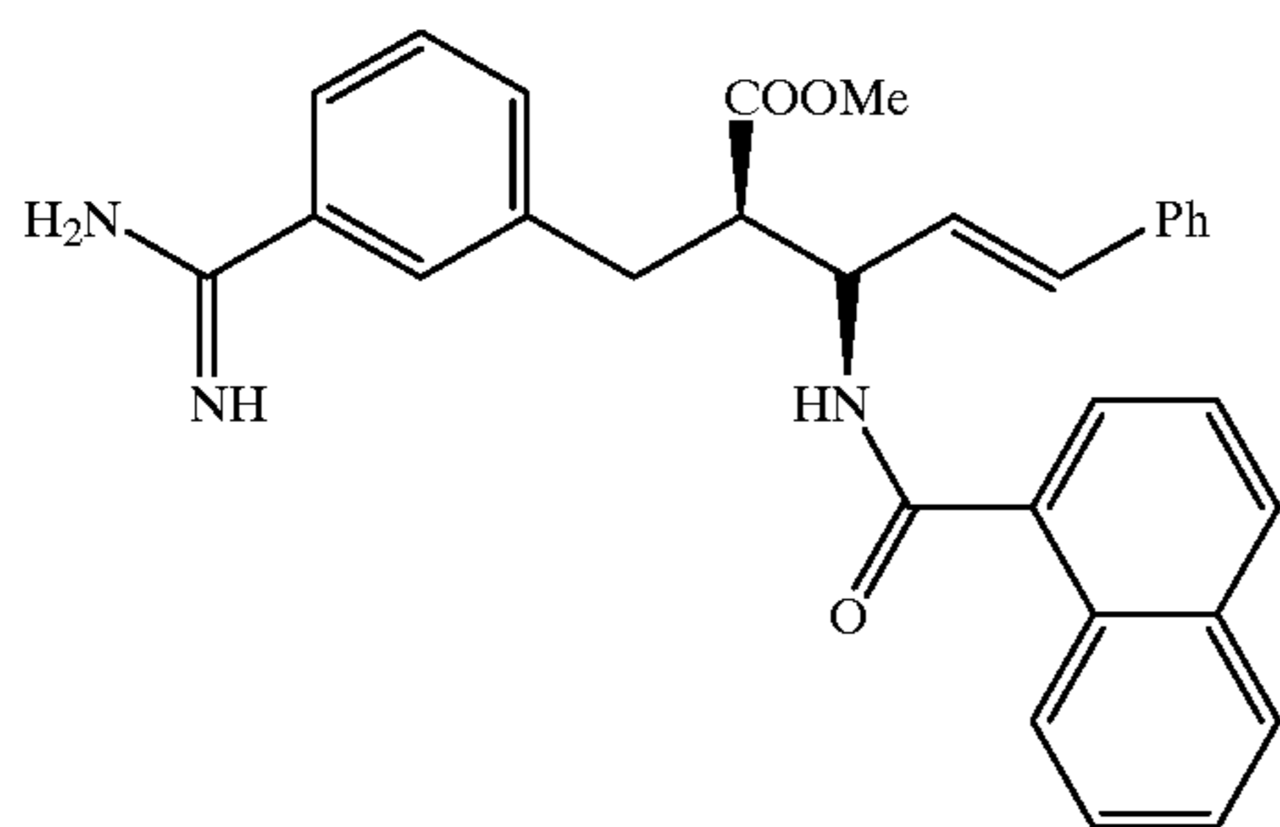
Compound 24
