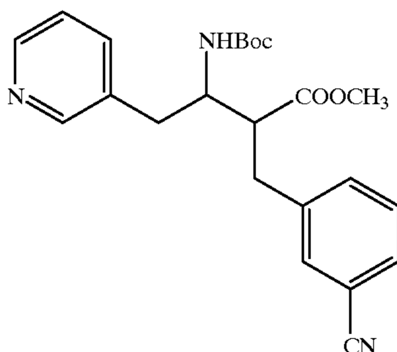
Compound 65
