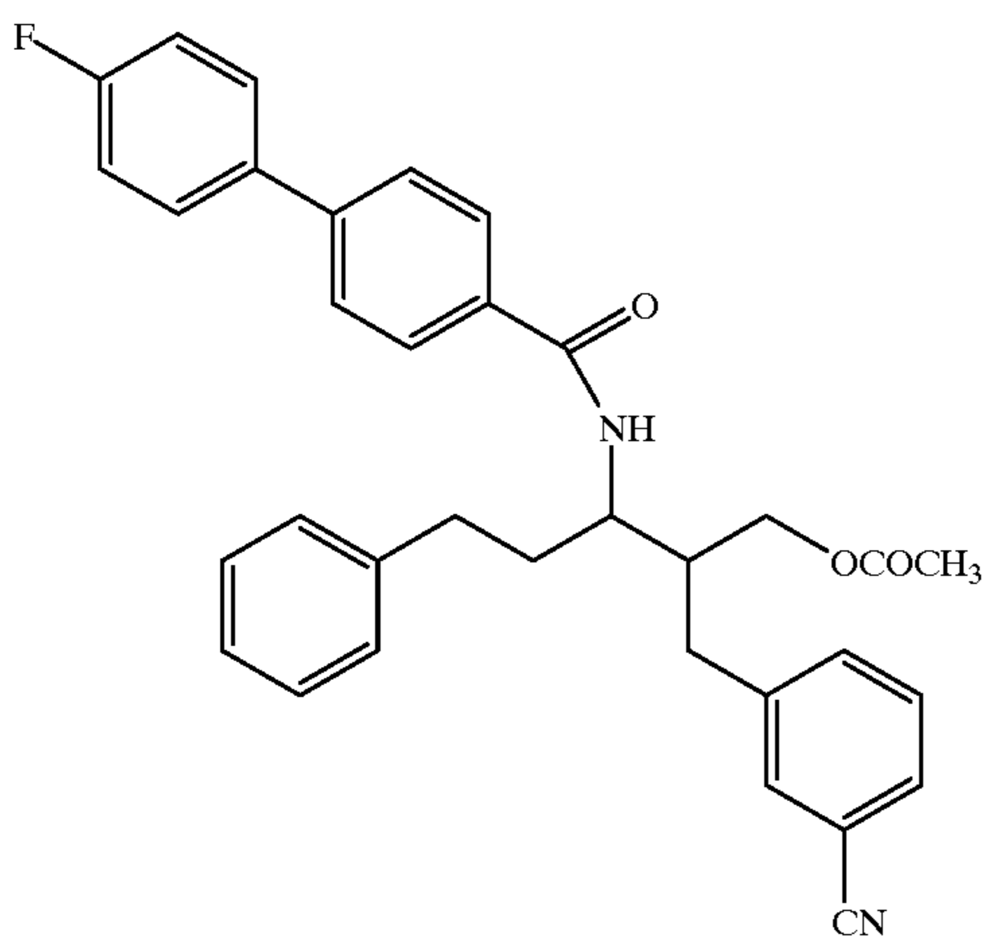
Compound 151
