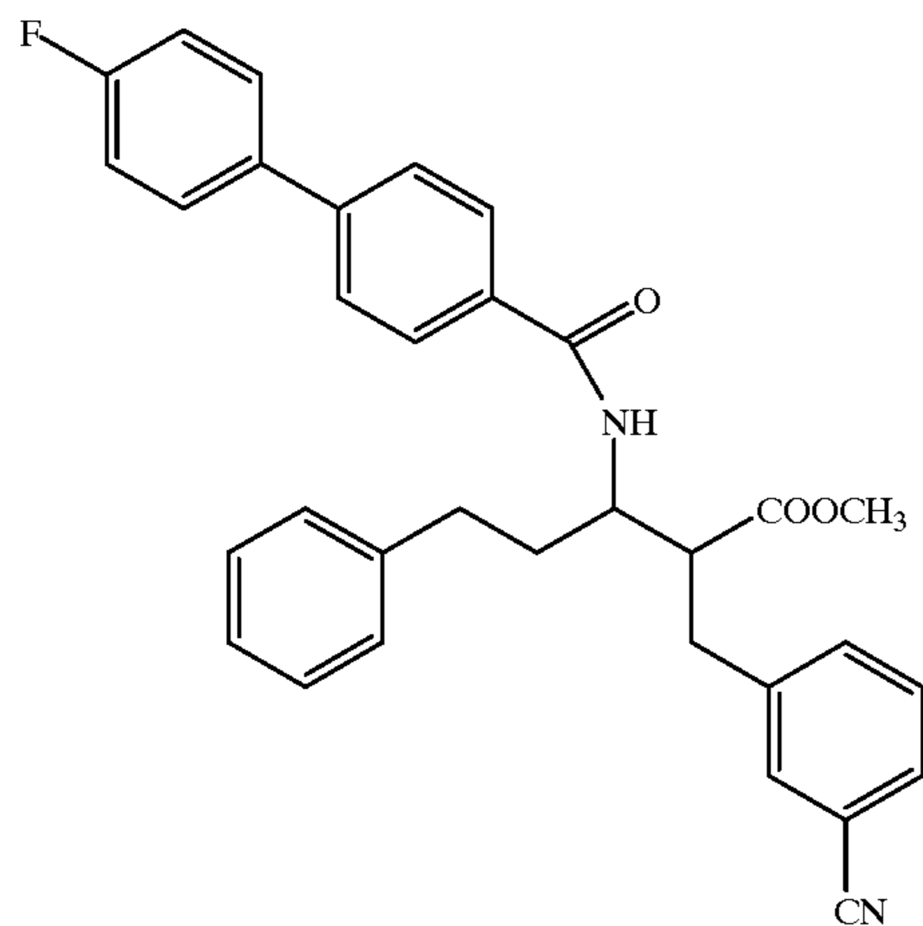
Compound 110
