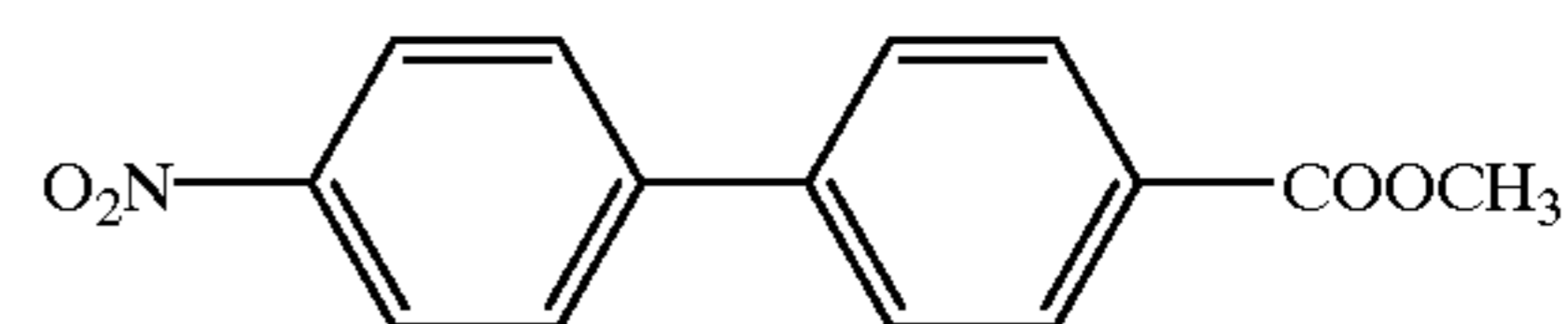
Compound 89
