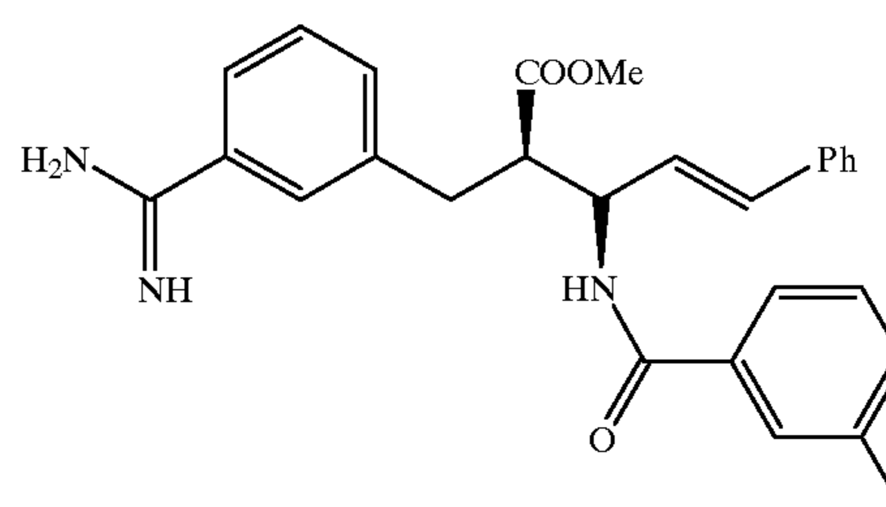
Compound 13
