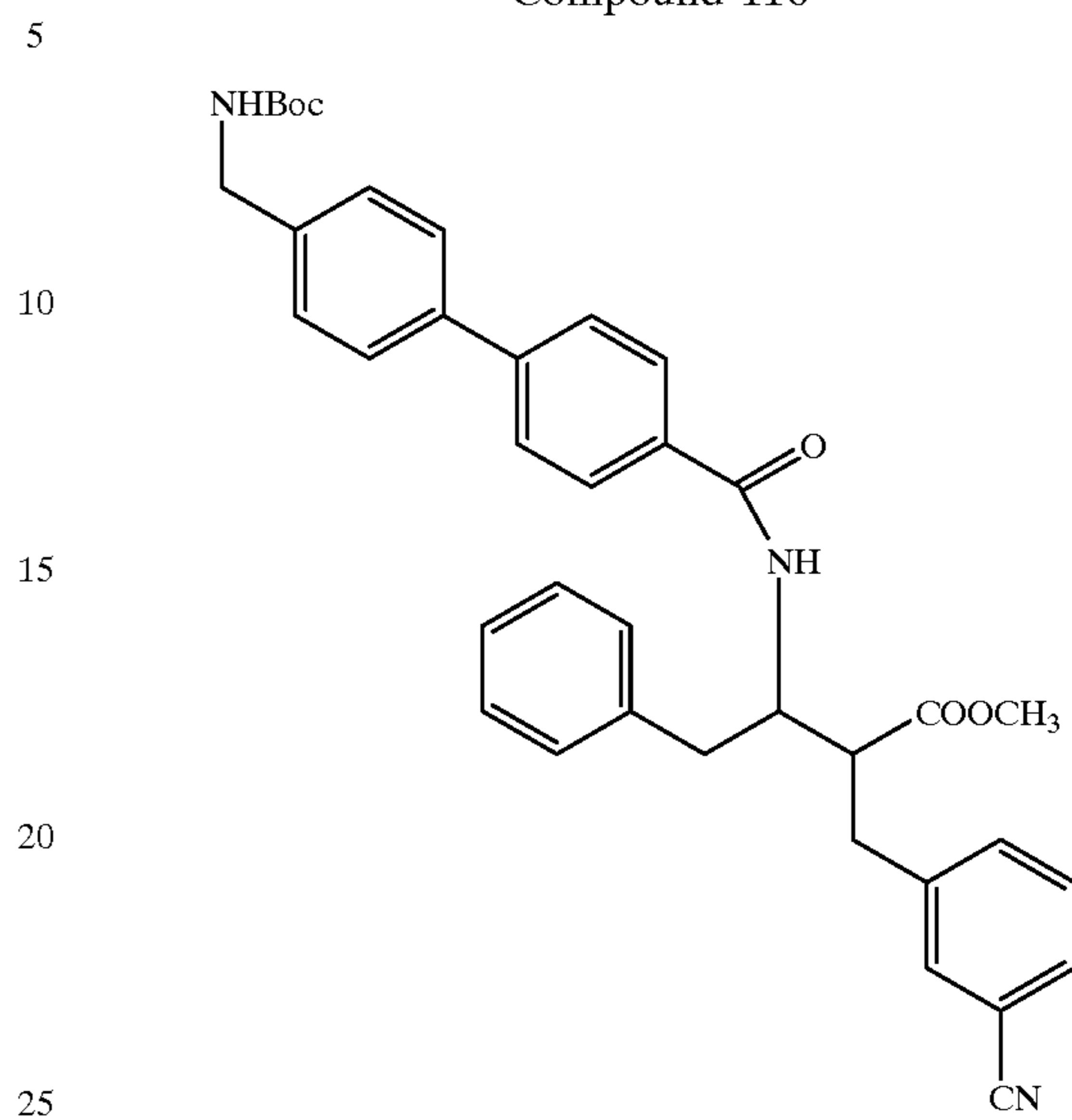
Compound 116
