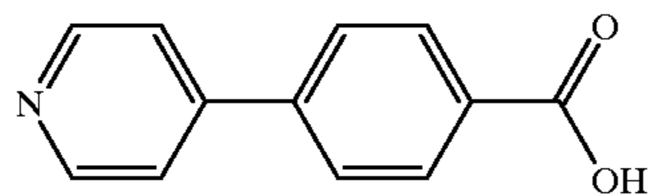
Compound 226
