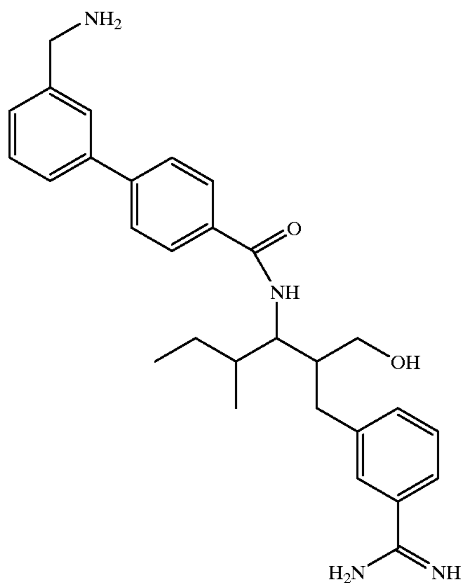
Compound 194
