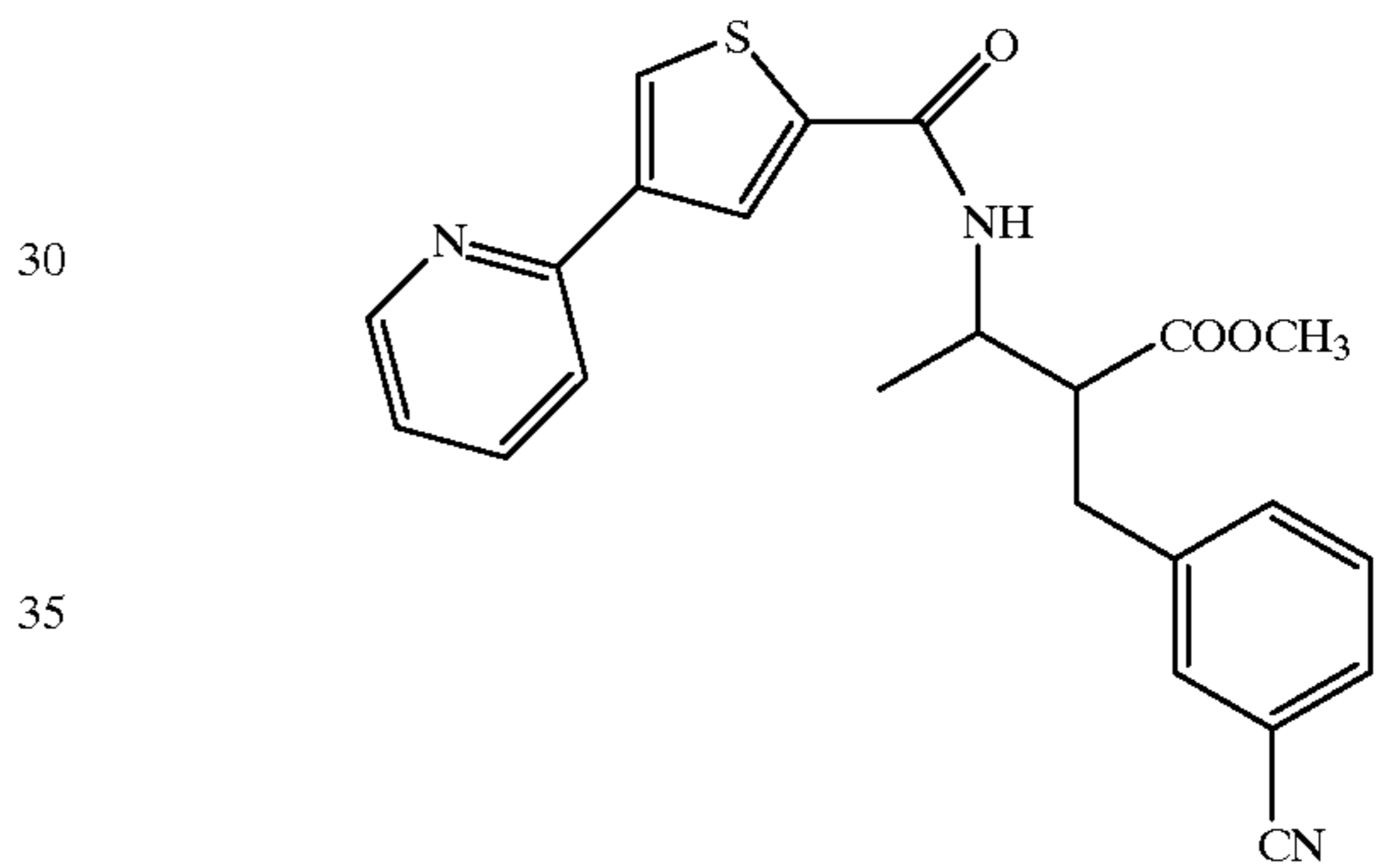
Compound 244
