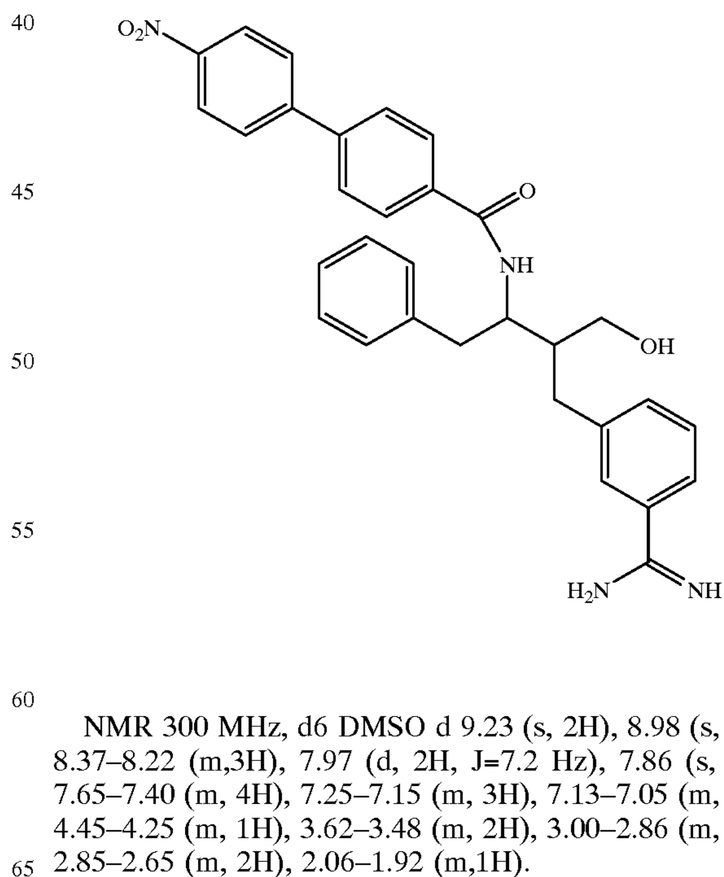
Compound 177
