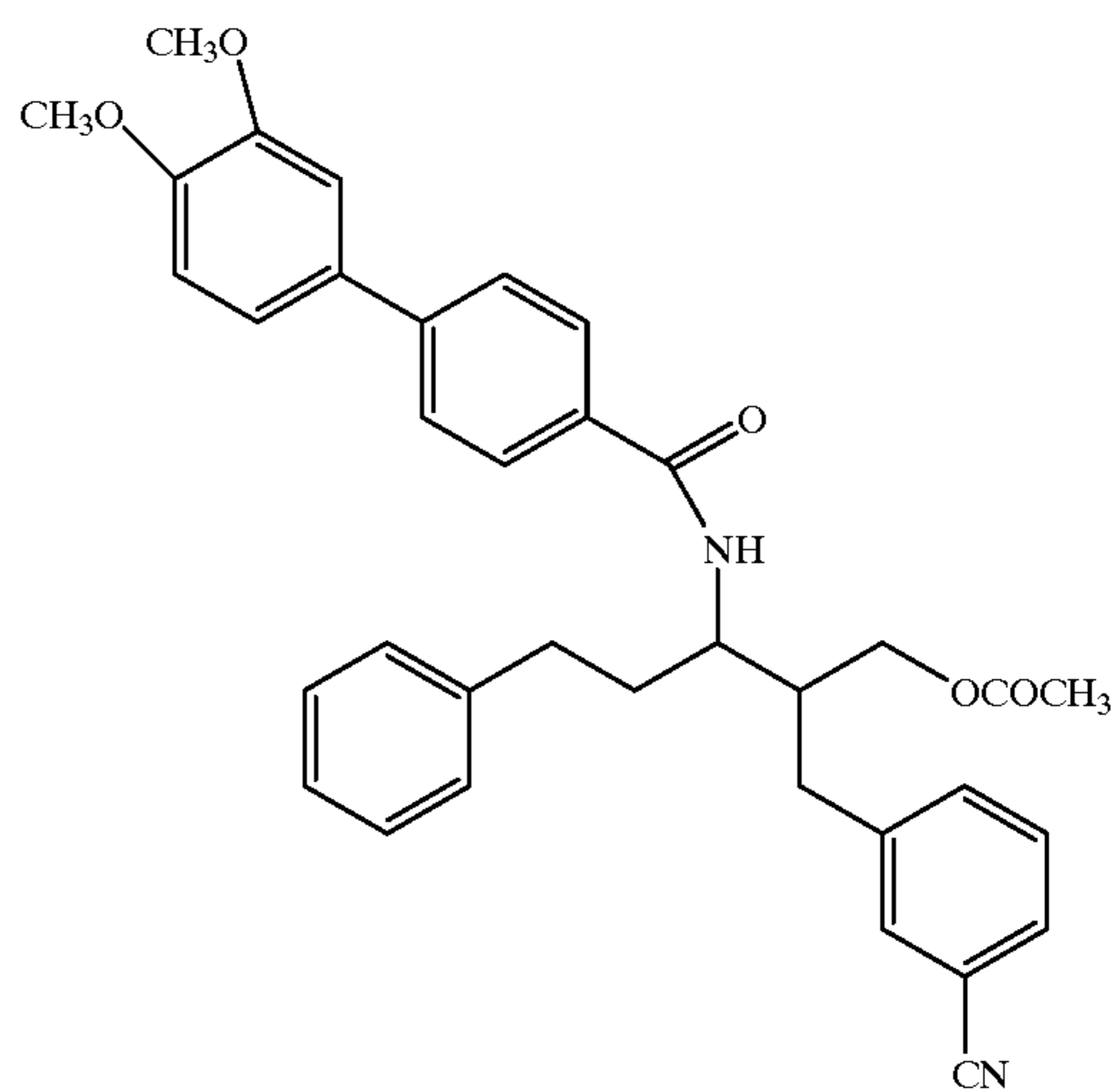
Compound 153
