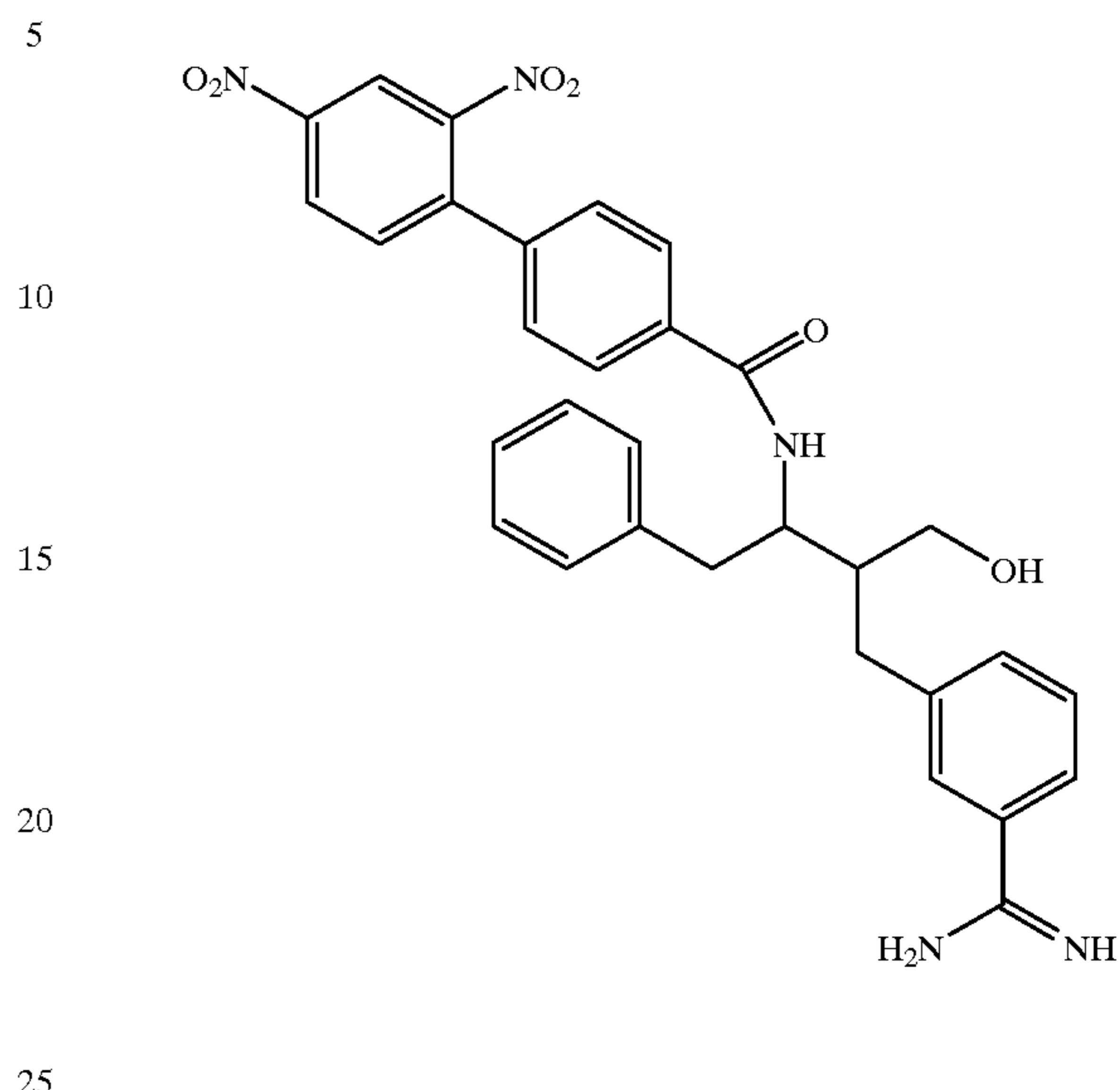
Compound 176
