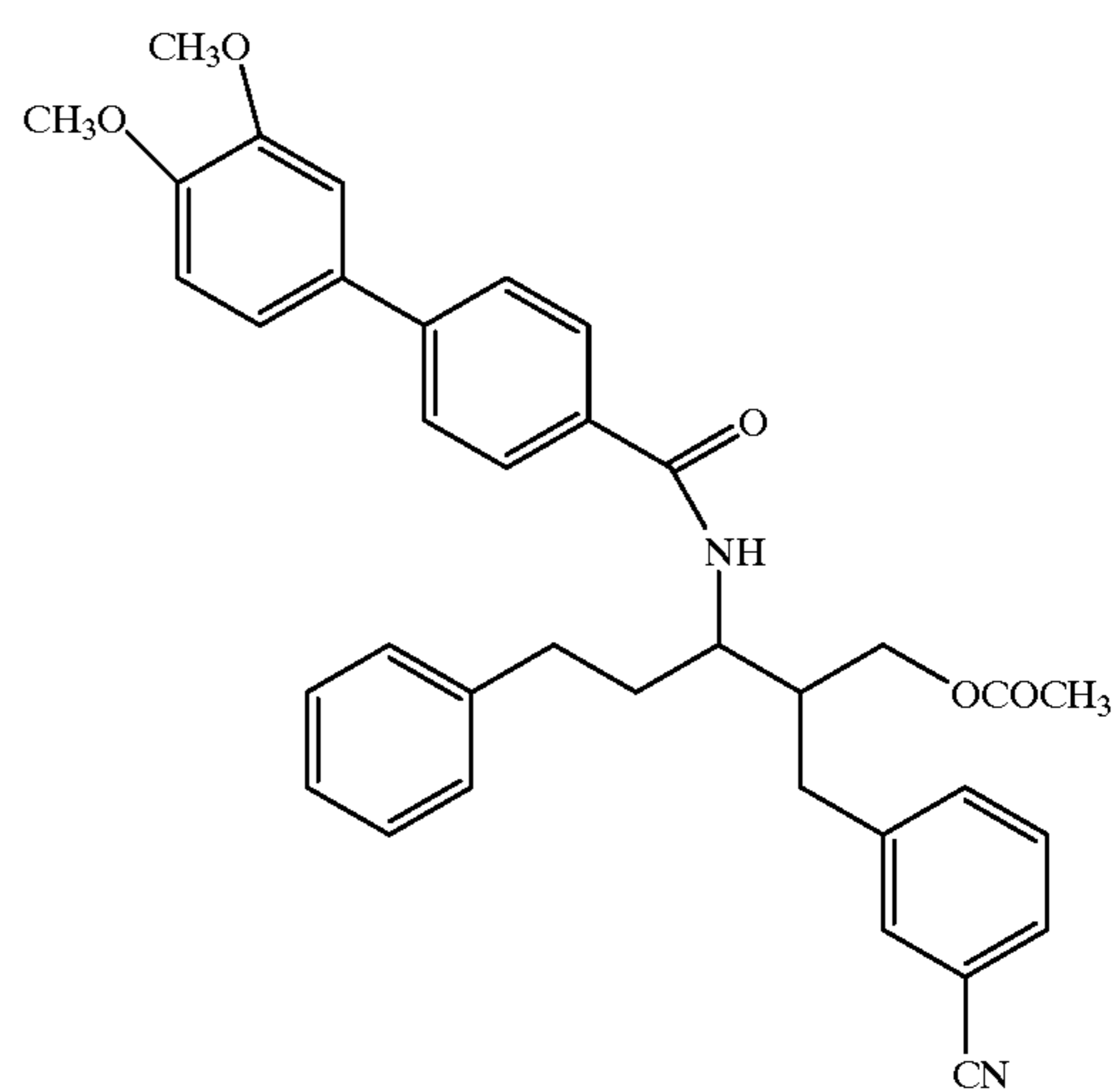
Compound 153
