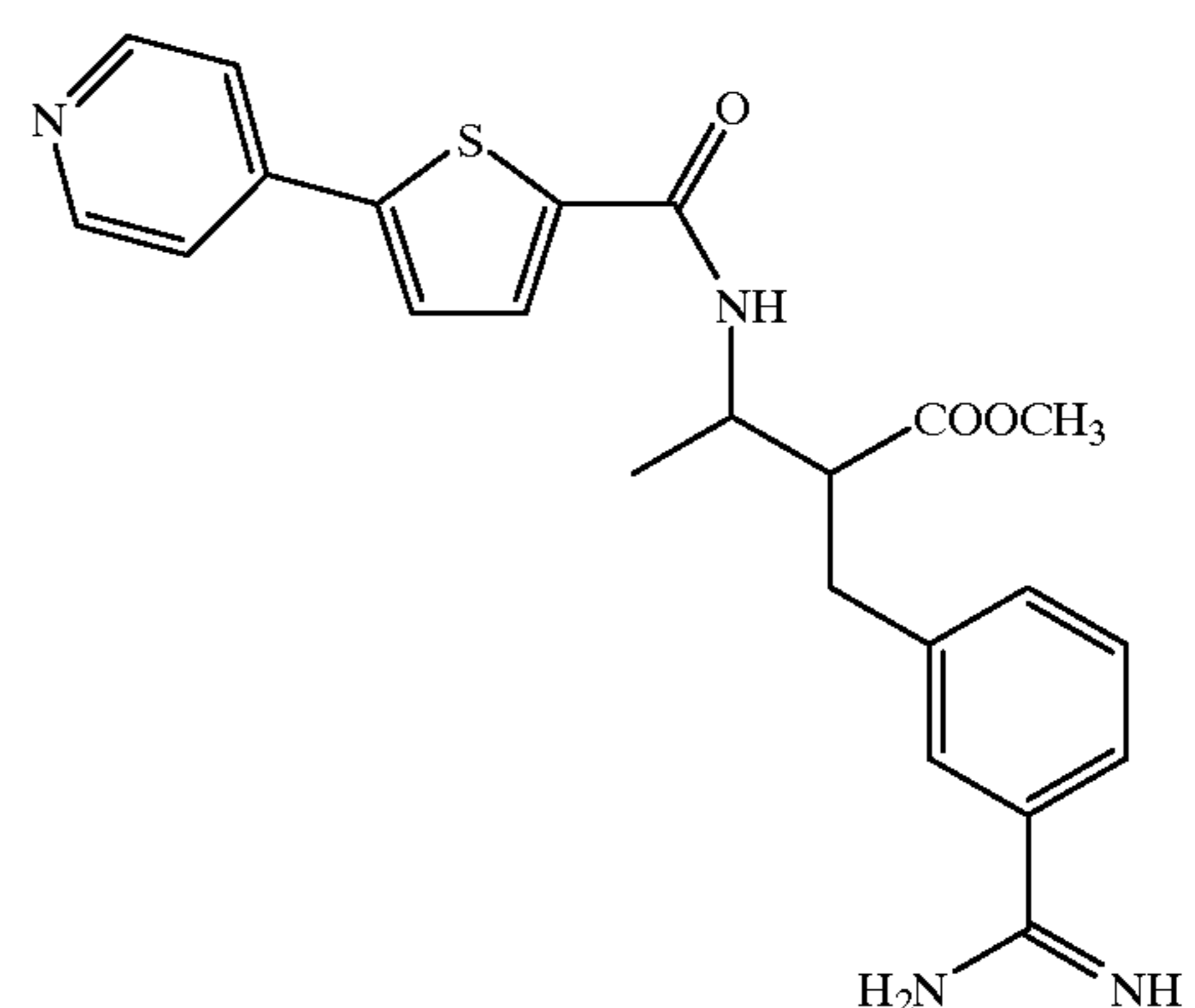
Compound 275
