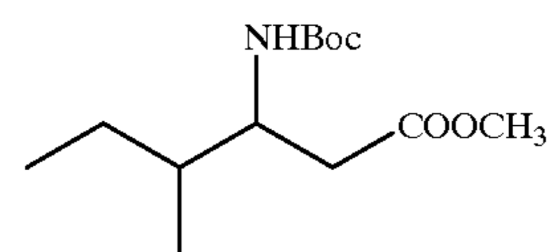
Compound 60
