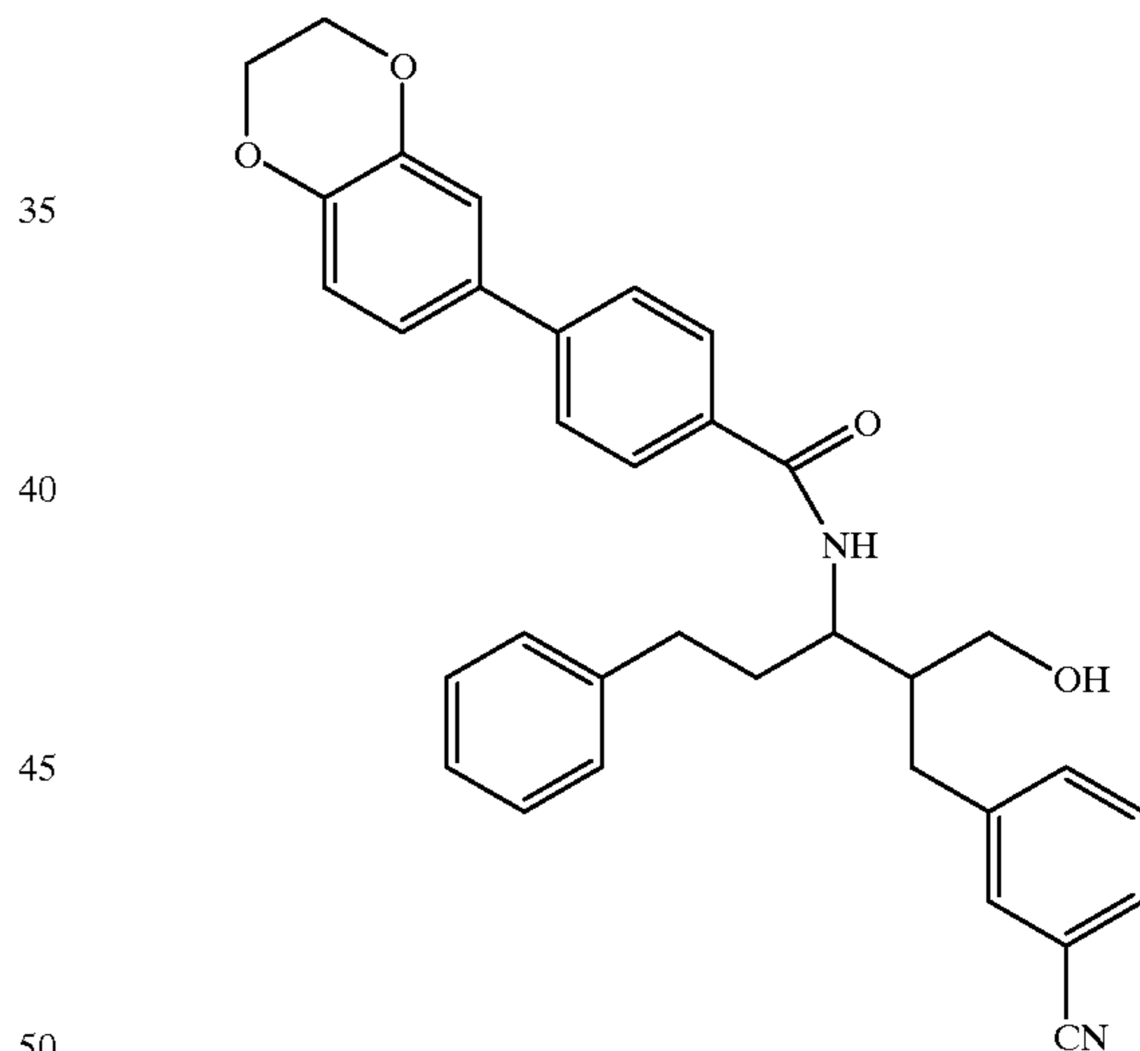
Compound 129
