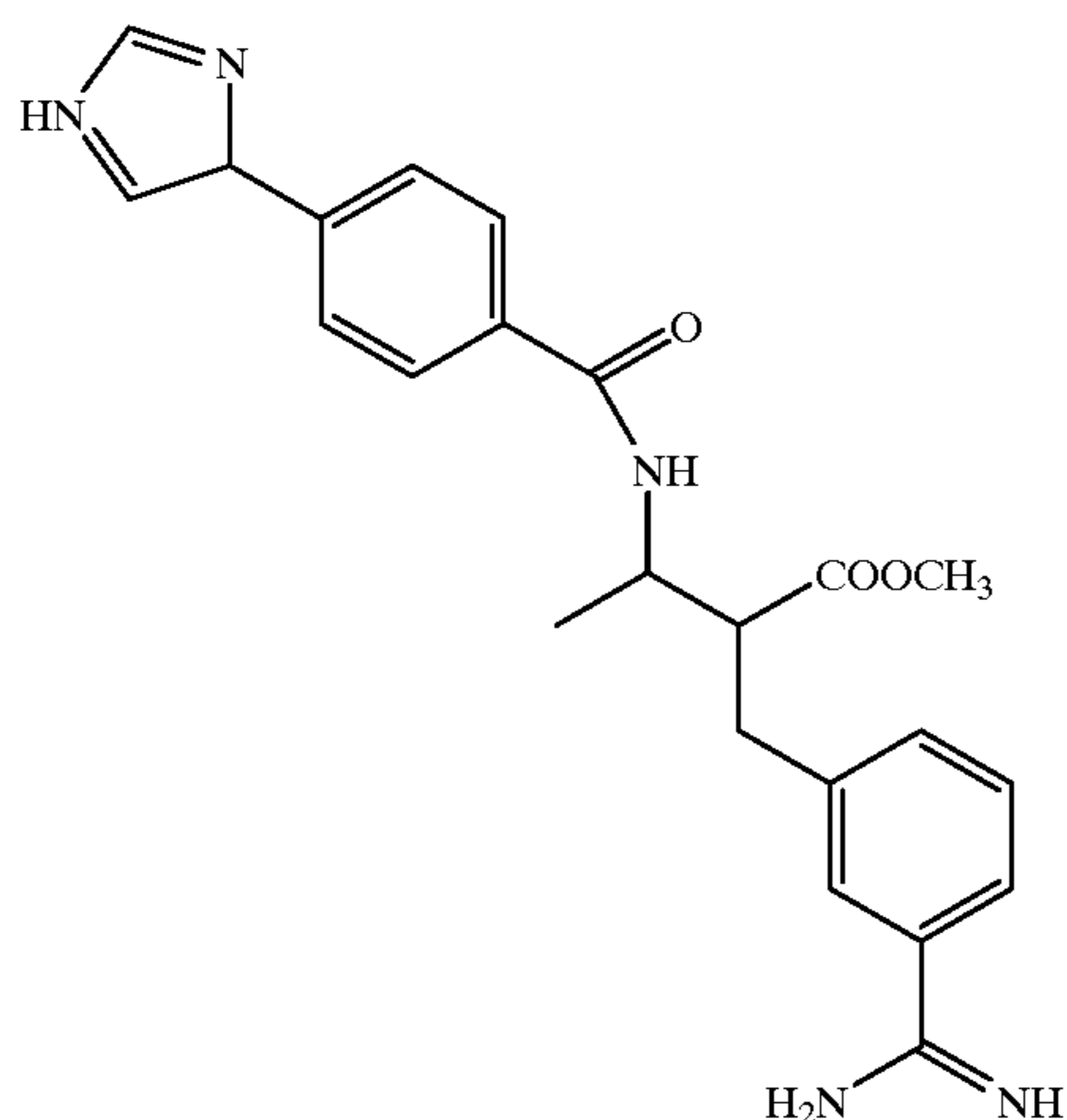
Compound 280
