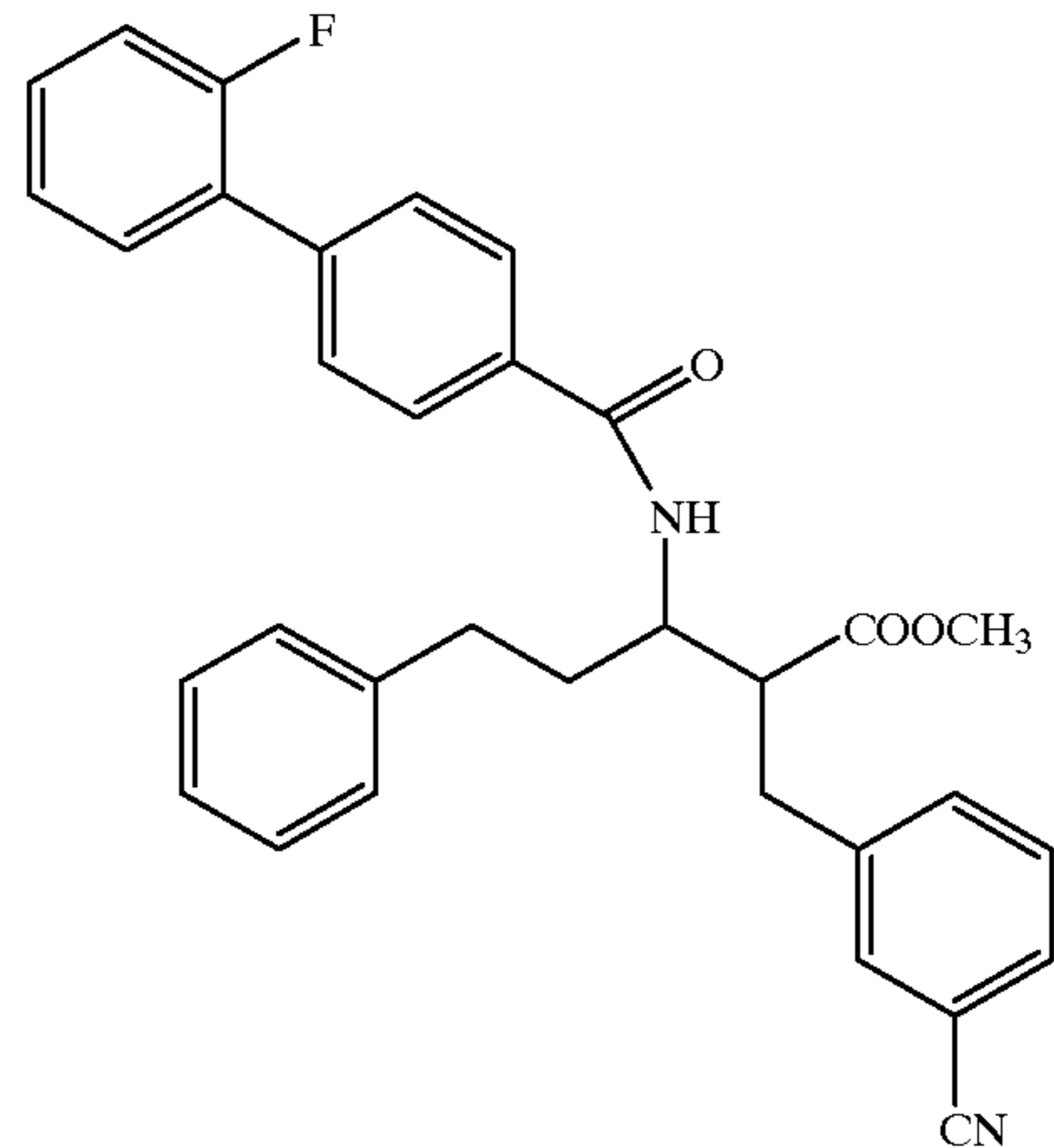
Compound 108
