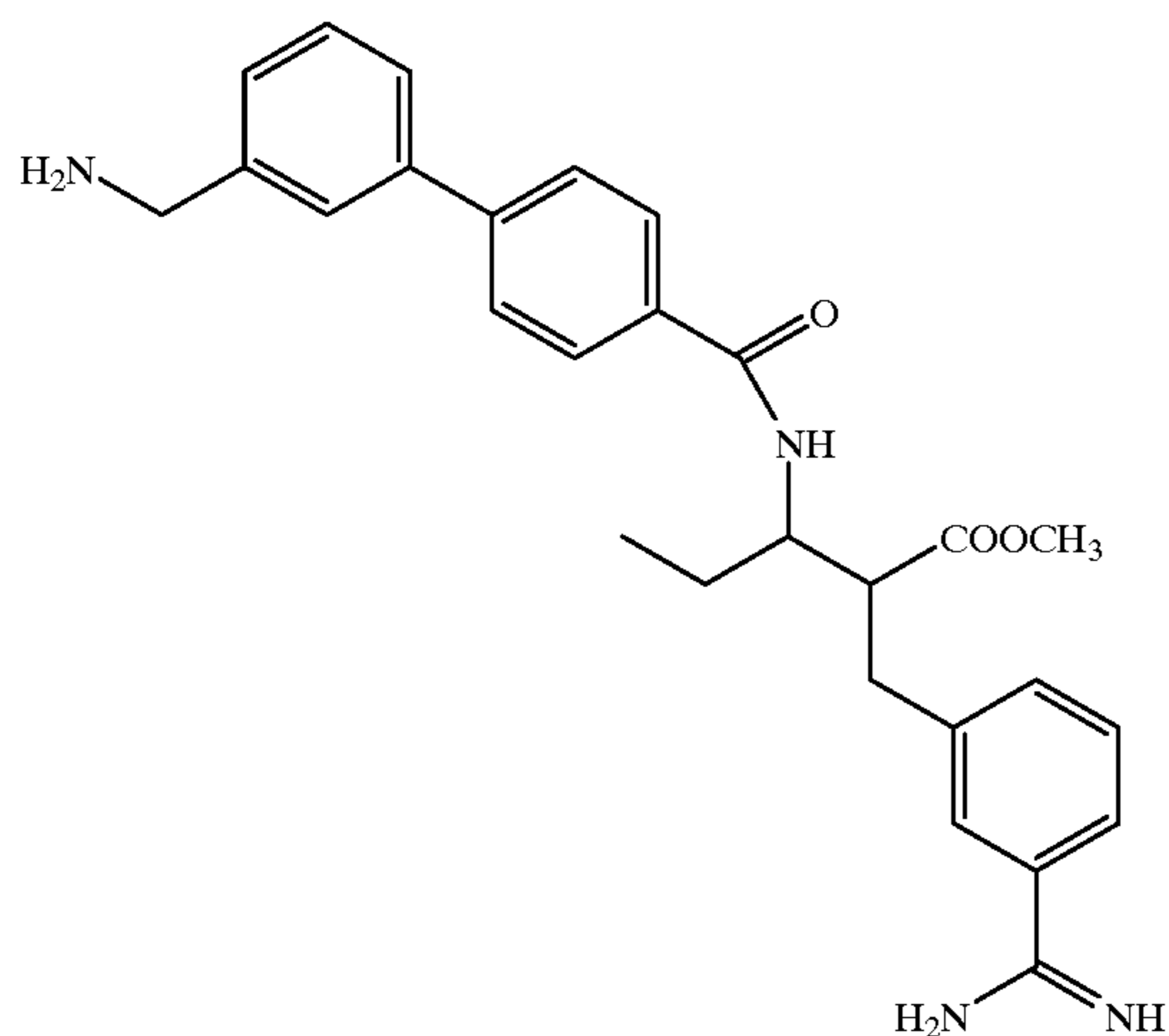
Compound 300
