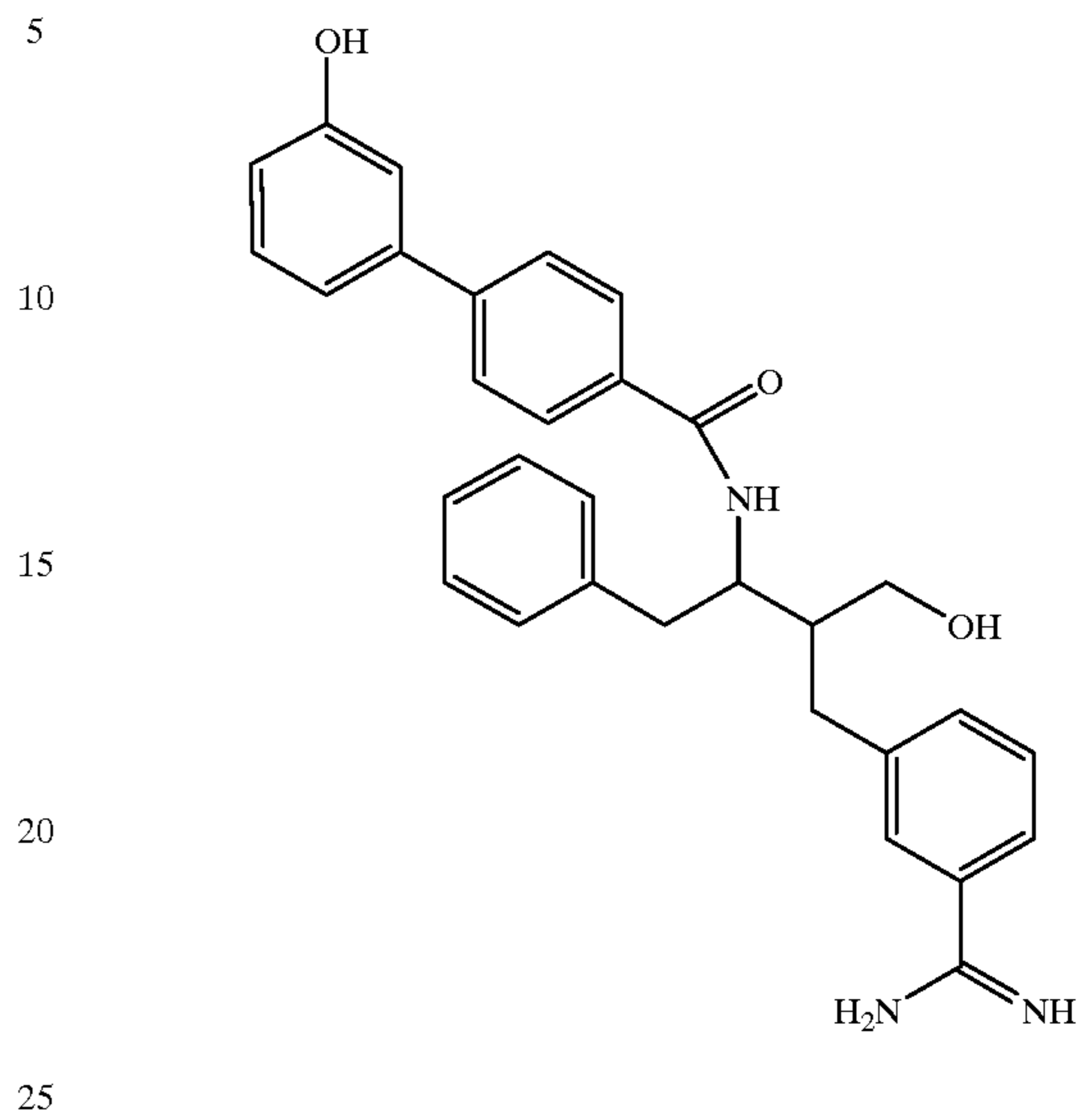
Compound 172
