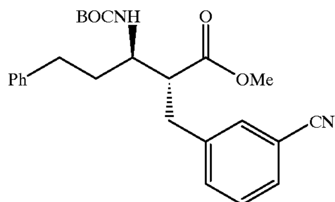
Compound 228
