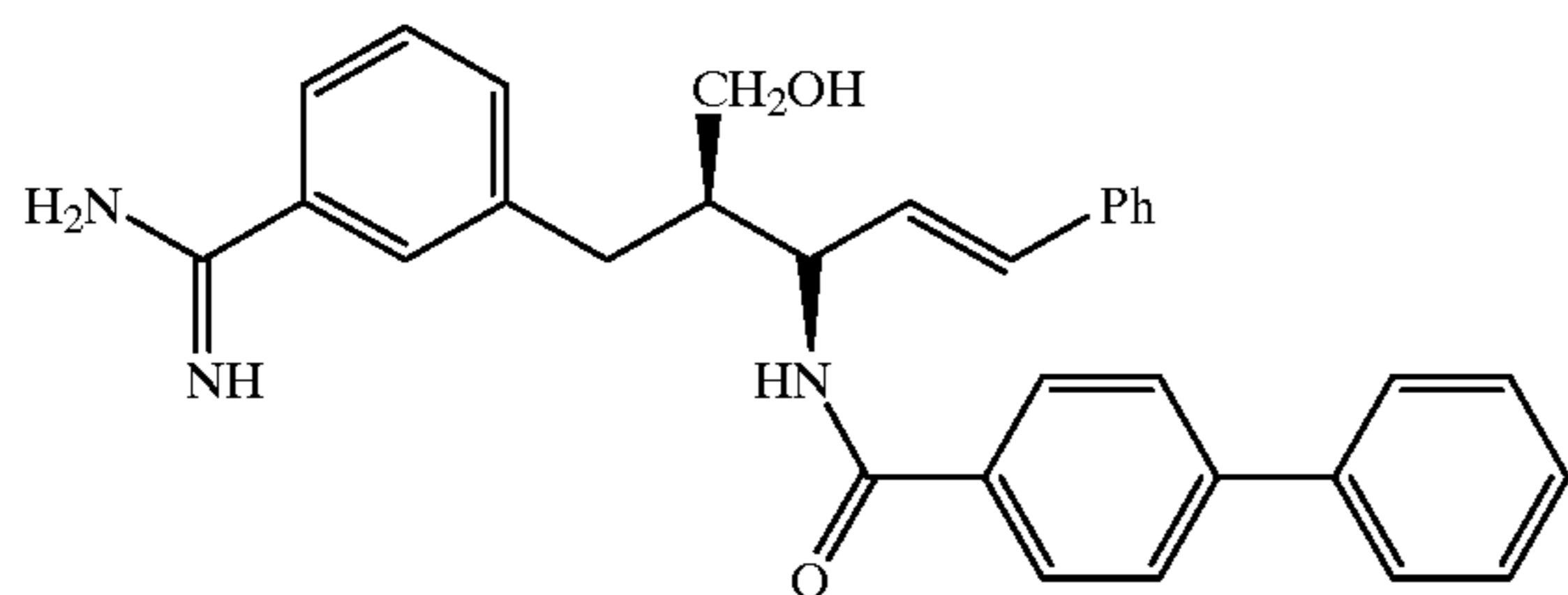
Compound 42
