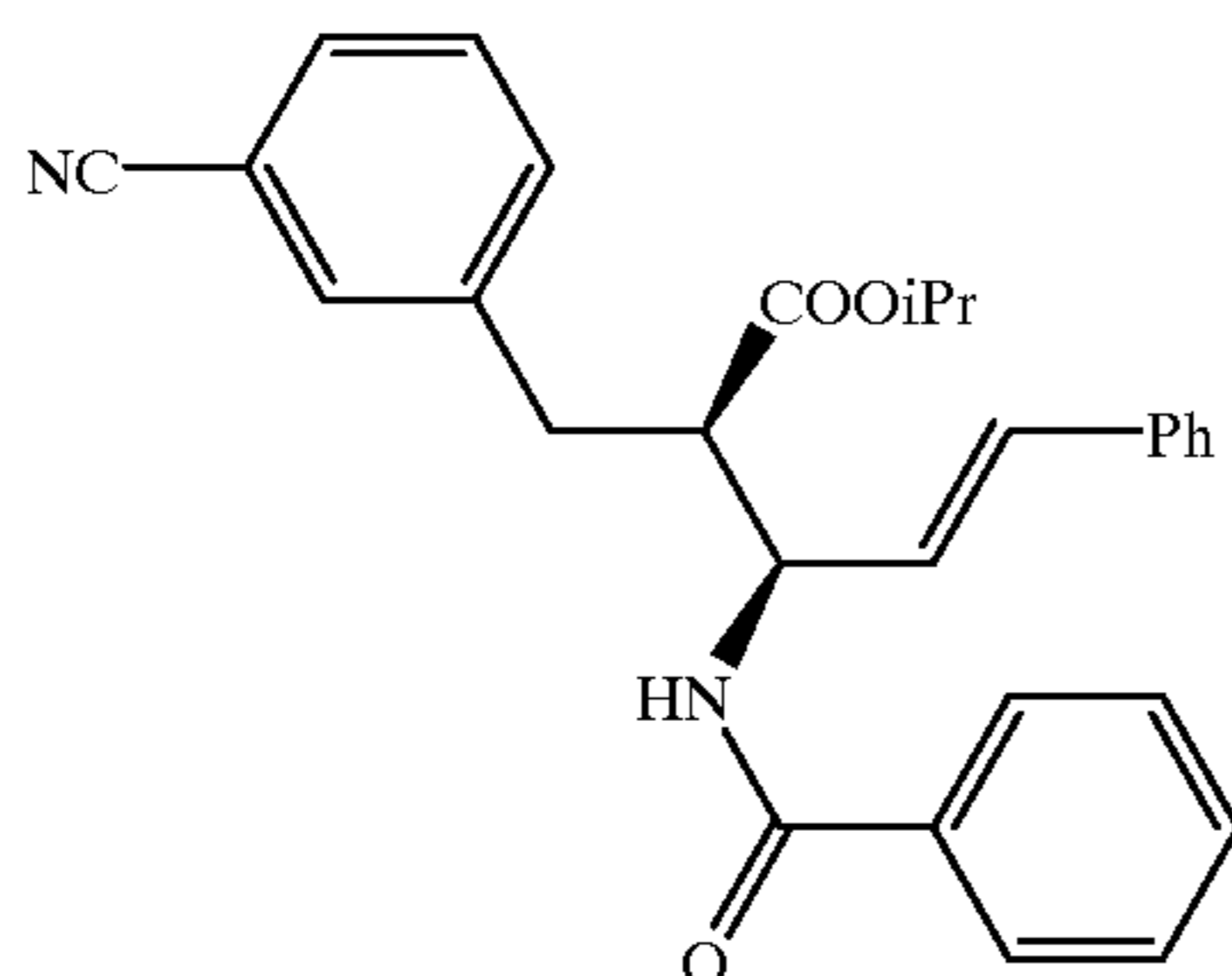
Compound 45
