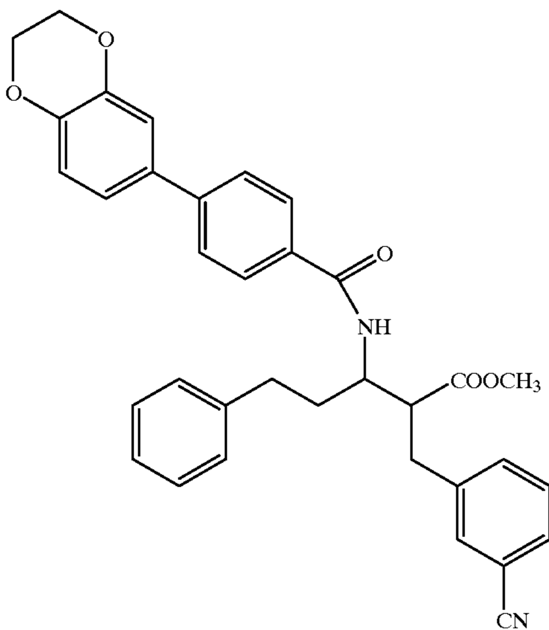
Compound 107
