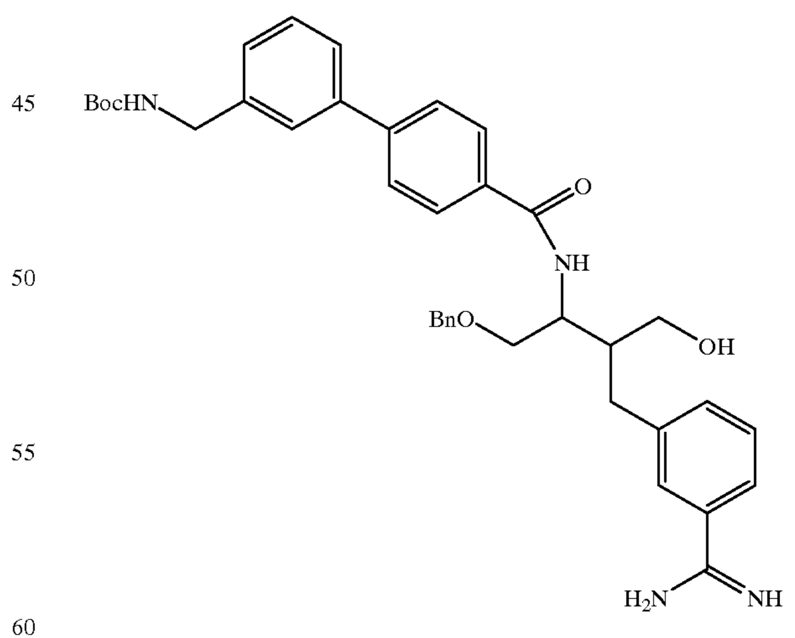
Compound 295
