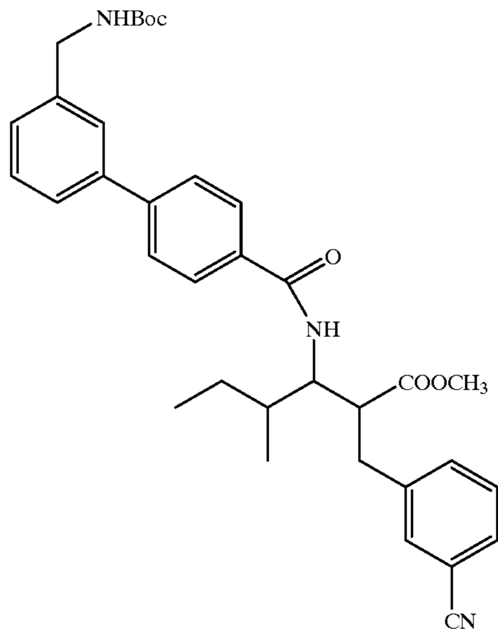
Compound 126
