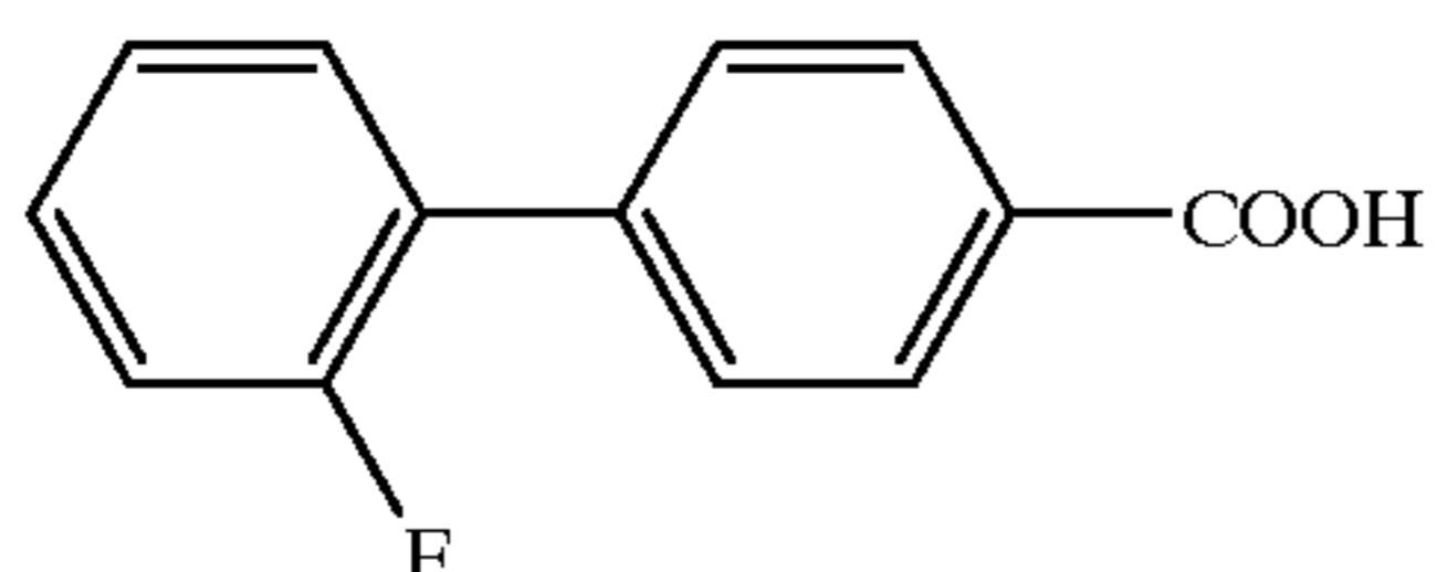
Compound 93
