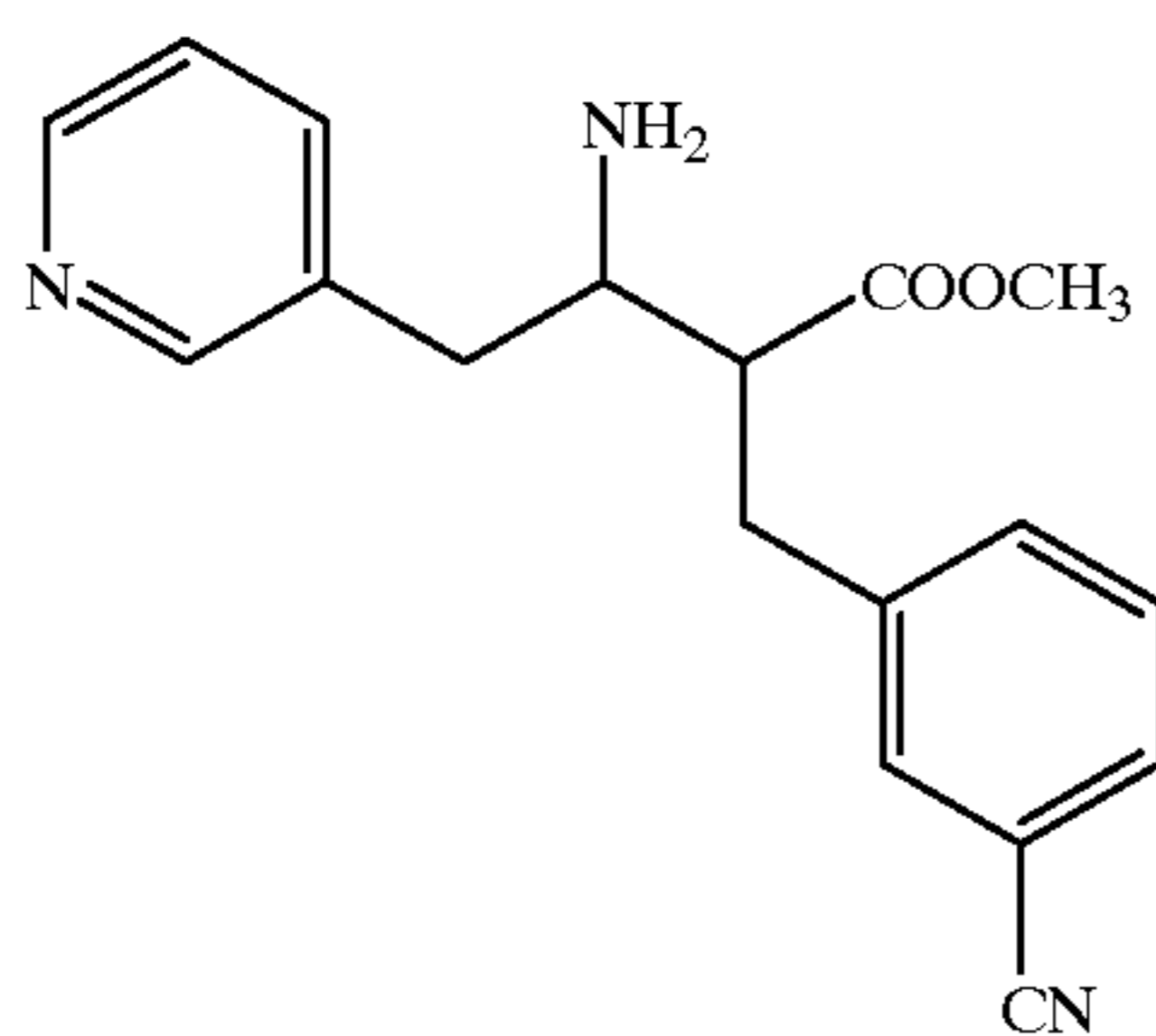
Compound 71
