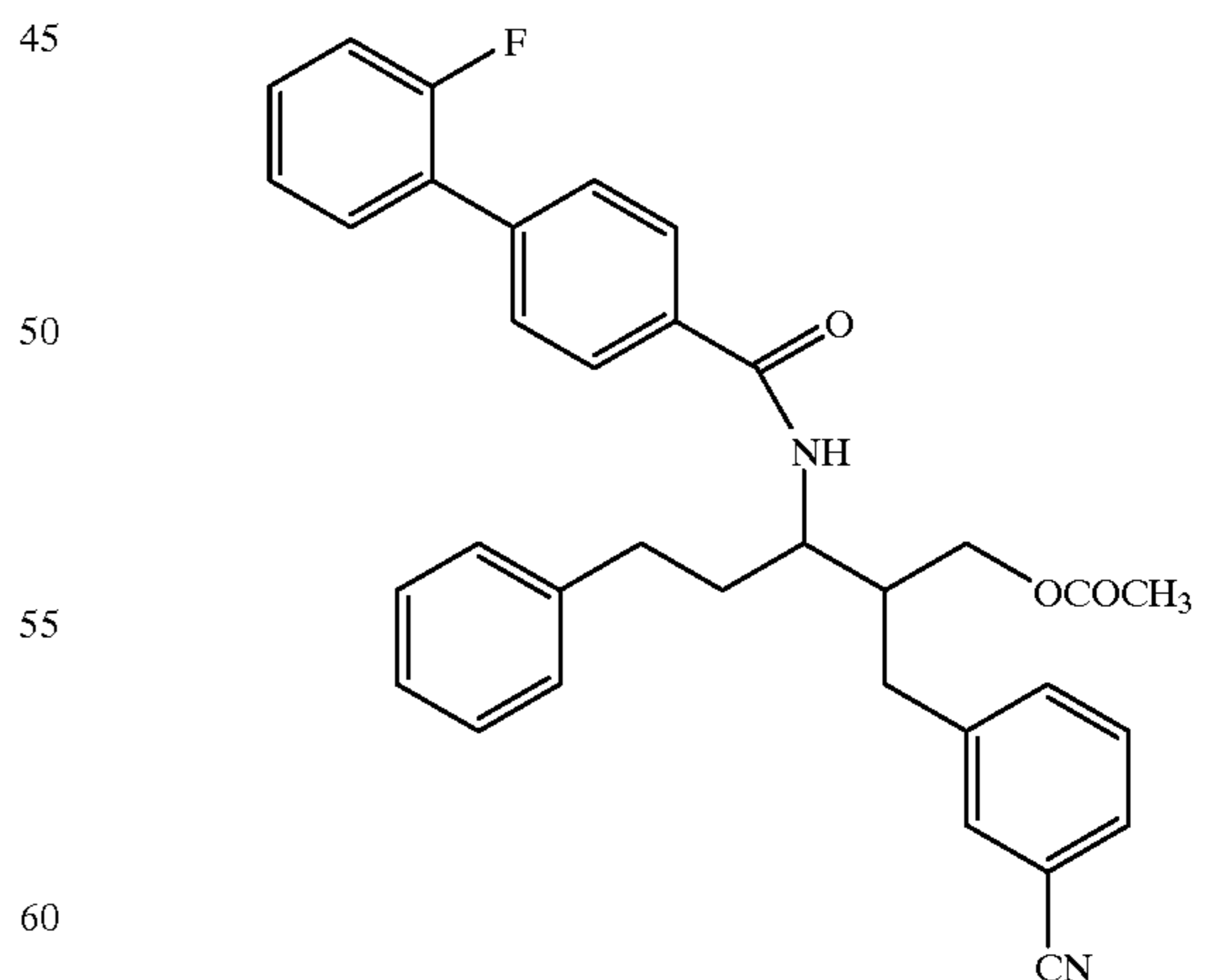
Compound 149
